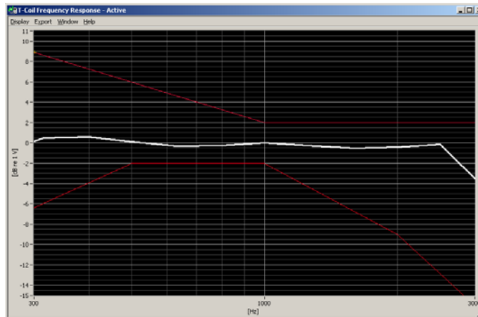
Figure 6-1 Axial Frequency Response
