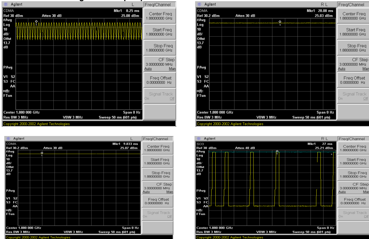
Figure 8-4 Zero-Span Plots
