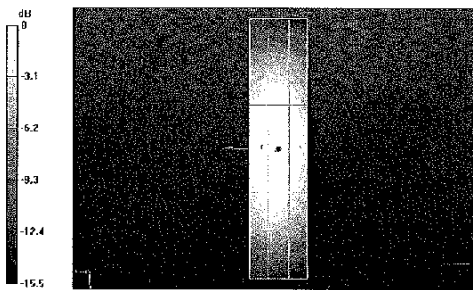
0 dB = 0.475A/m
