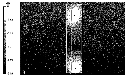
0 dB = 138.2V/m
