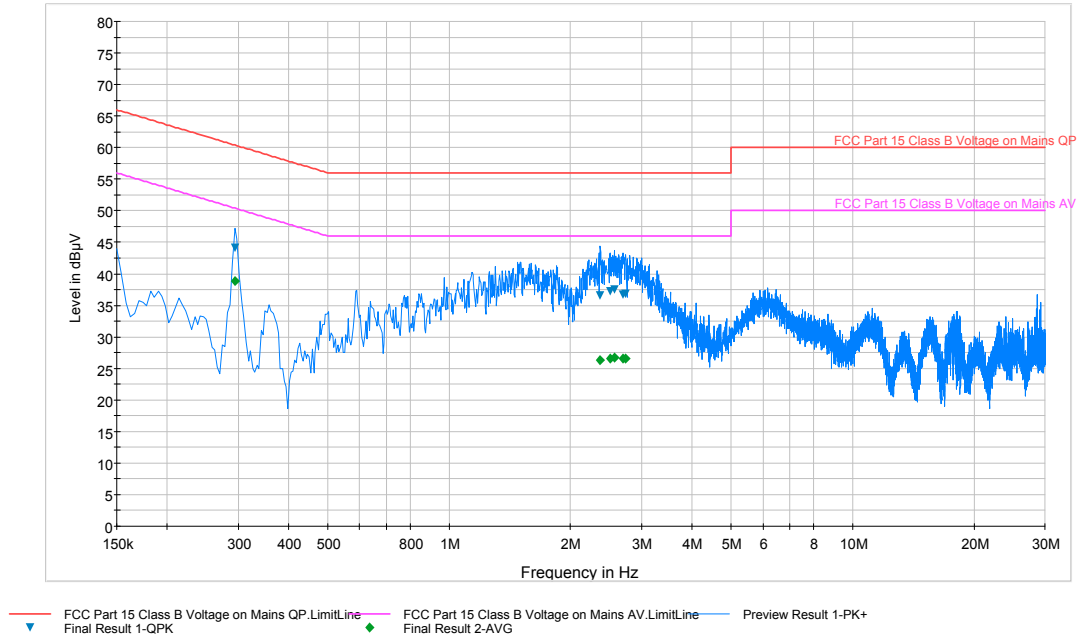
Plot 6-60. Line Conducted Plot with 802.11a (N)
