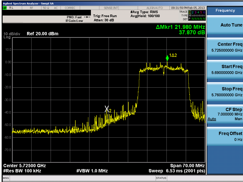
Plot 6-39. Band Edge Plot (20MHz BW 802.11n (5.8GHz) – Ch. 149)
