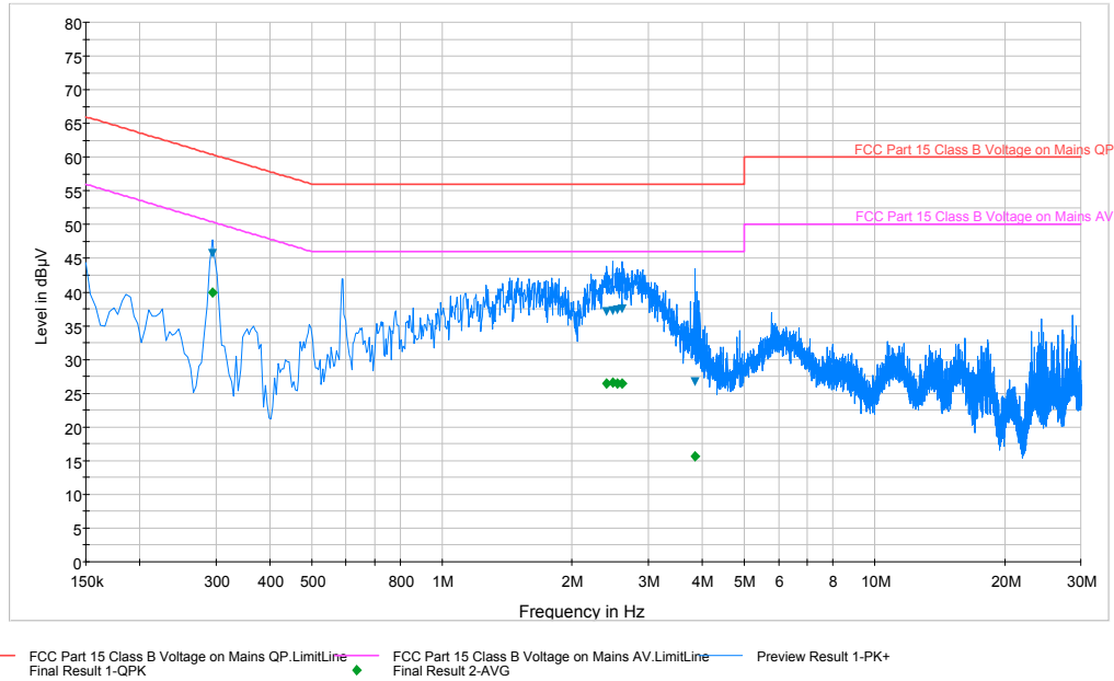
Plot 6-58. Line Conducted Plot with 802.11b (N)
