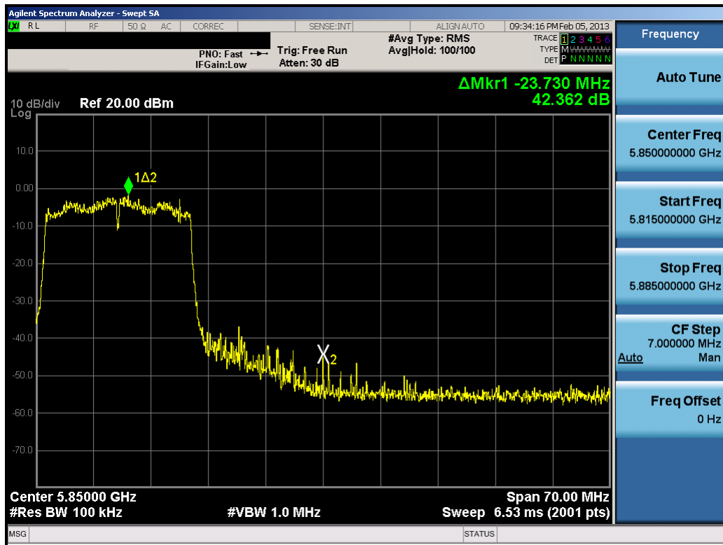
Plot 6-40. Band Edge Plot (20MHz BW 802.11n (5.8GHz) – Ch. 165)
