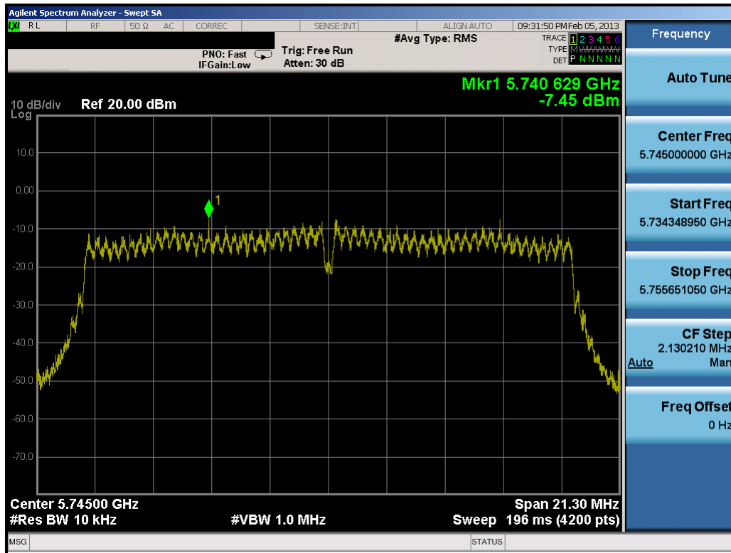
Plot 6-28. Power Spectral Density Plot (20MHz BW 802.11n (5.8GHz) – Ch. 149)
