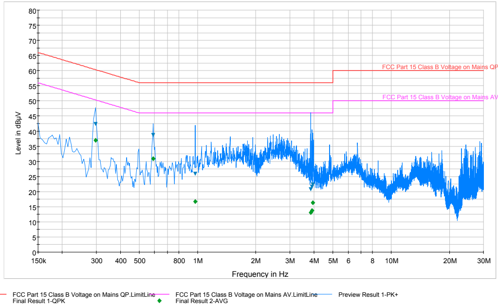
Plot 6-57. Line Conducted Plot with 802.11b (L1)
