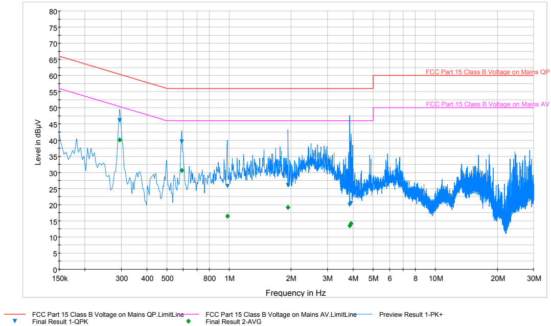
Plot 6-59. Line Conducted Plot with 802.11a (L1)
