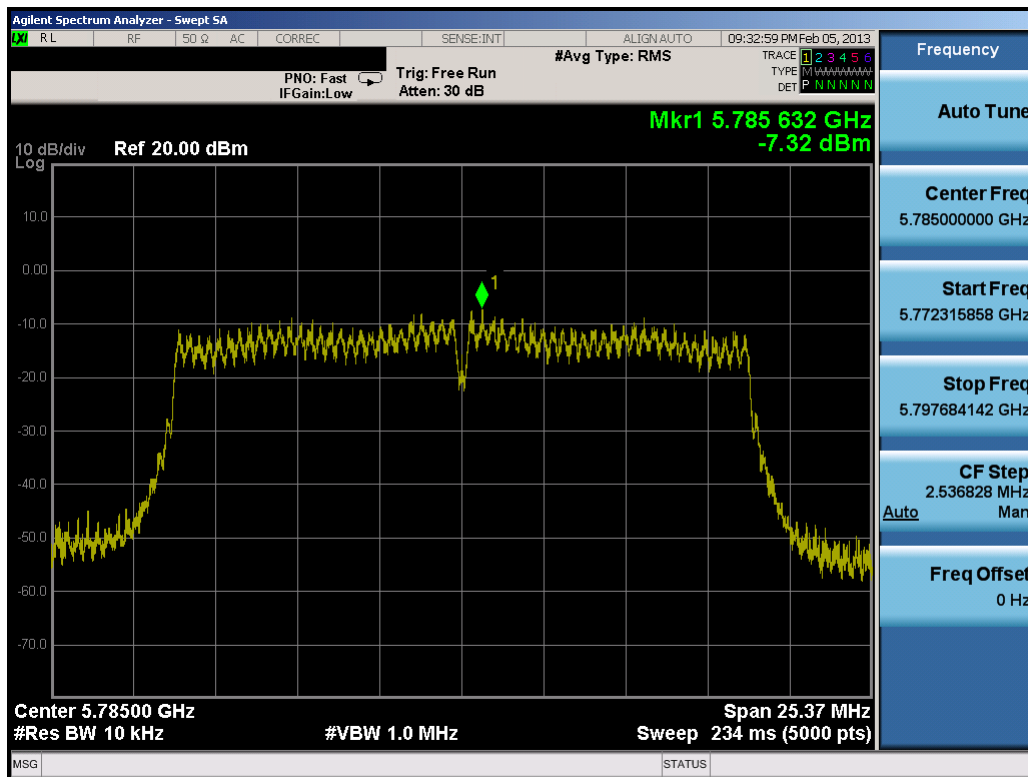
Plot 6-29. Power Spectral Density Plot (20MHz BW 802.11n (5.8GHz) – Ch. 157)
