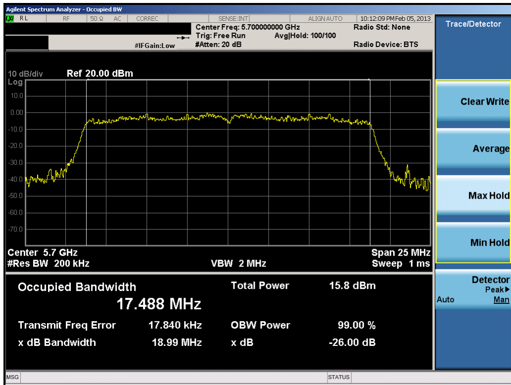
Plot 6-18. 26dB Bandwidth Plot (20MHz BW 802.11n (UNII Band 3) – Ch. 140)
