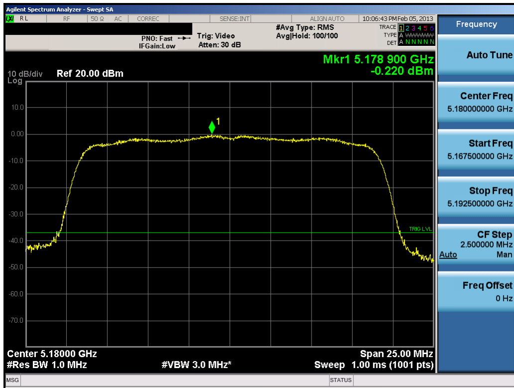
Plot 6-22. Peak Power Spectral Density Plot (20MHz BW 802.11n (UNII Band 1) – Ch. 36)
