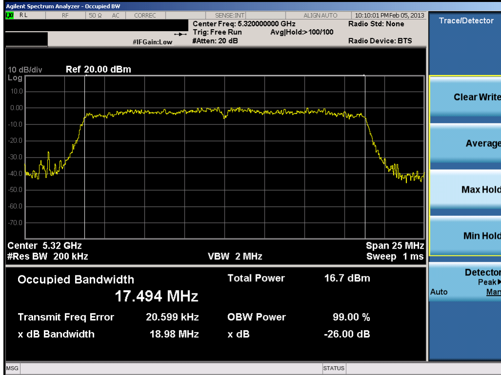
Plot 6-12. 26dB Bandwidth Plot (20MHz BW 802.11n (UNII Band 2) – Ch. 64)
