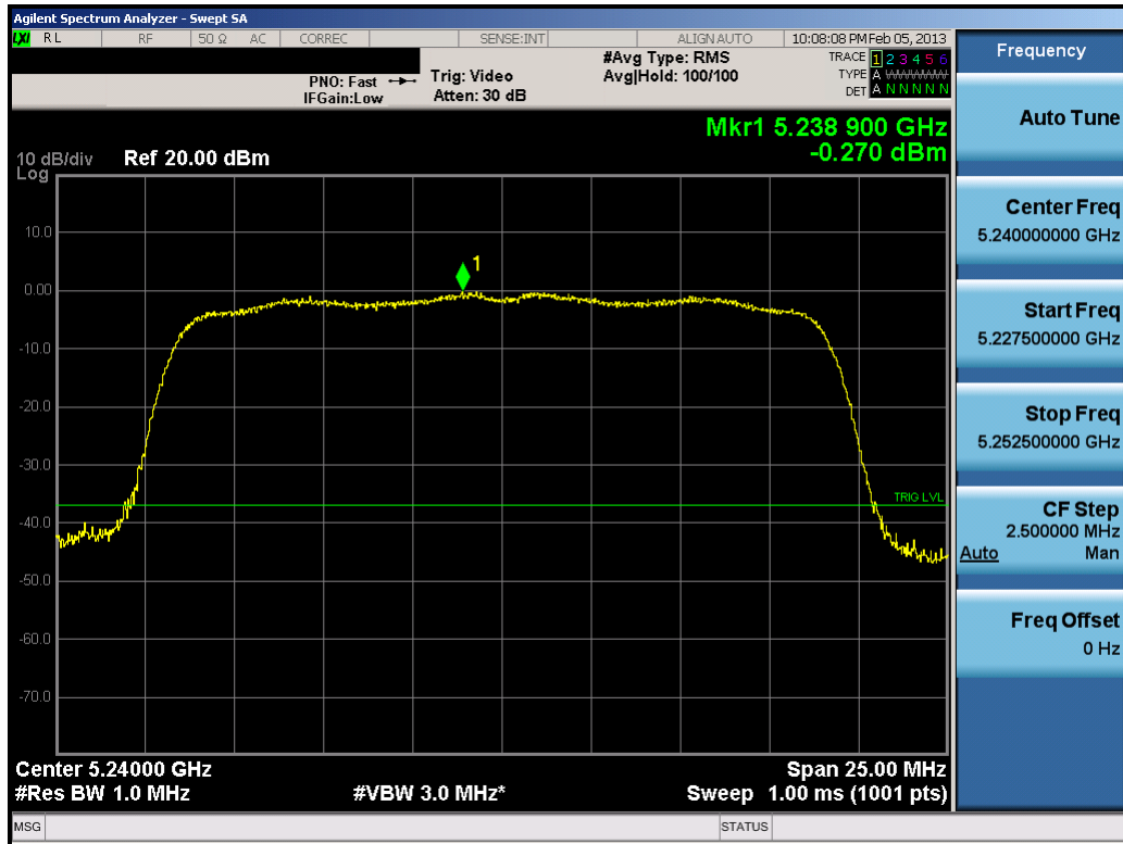
Plot 6-24. Peak Power Spectral Density Plot (20MHz BW 802.11n (UNII Band 1) – Ch. 48)
