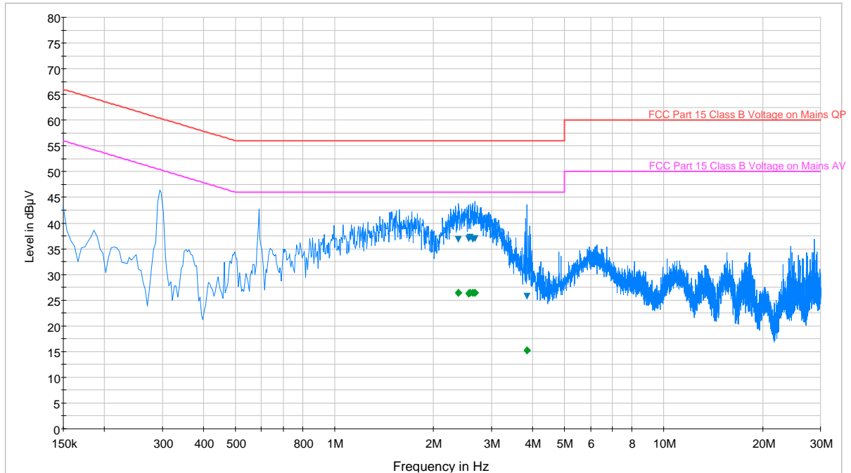
— FCC Part 15 Class B Voltage on Mains QP.LimitLine — FCC Part 15 Class B Voltage on Mains AV.LimitLine — Preview Result 1-PK+ Final Result 1-QPK ▼ Final Result 1-QPK ◆ Final Result 2-AVG
