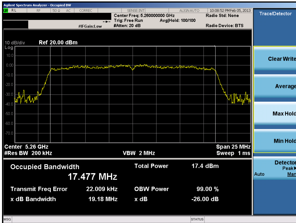
Plot 6-10. 26dB Bandwidth Plot (20MHz BW 802.11n (UNII Band 2) – Ch. 52)
