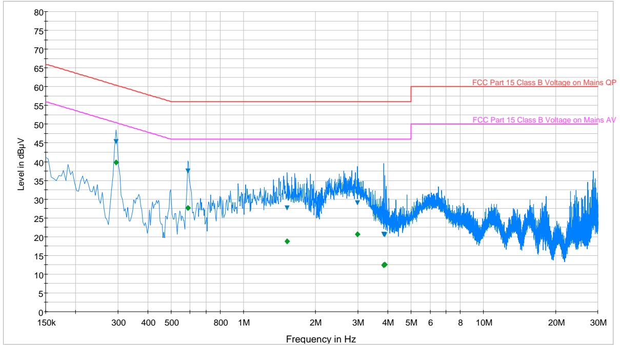
Plot 6-46. Line Conducted Plot with 802.11a UNII Band 1 (L1)
