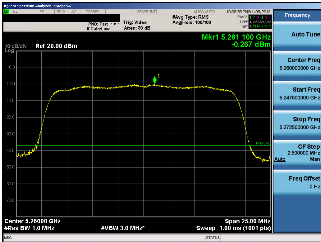
Plot 6-28. Peak Power Spectral Density Plot (20MHz BW 802.11n (UNII Band 2) – Ch. 52)
