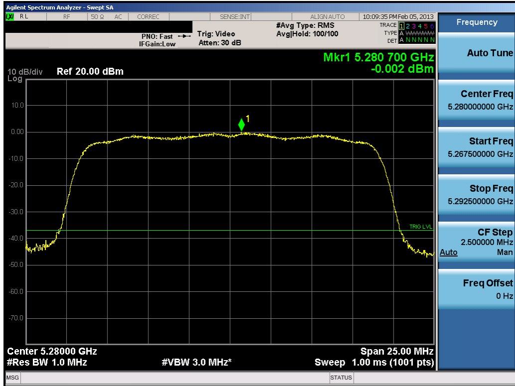
Plot 6-29. Peak Power Spectral Density Plot (20MHz BW 802.11n (UNII Band 2) – Ch. 56)
