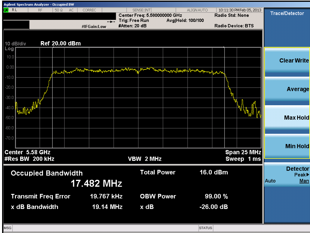
Plot 6-17. 26dB Bandwidth Plot (20MHz BW 802.11n (UNII Band 3) – Ch. 116)
