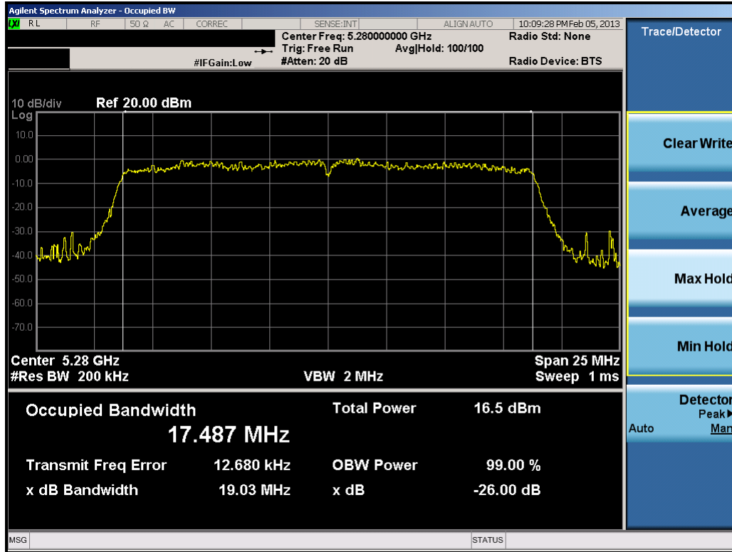
Plot 6-11. 26dB Bandwidth Plot (20MHz BW 802.11n (UNII Band 2) – Ch. 56)
