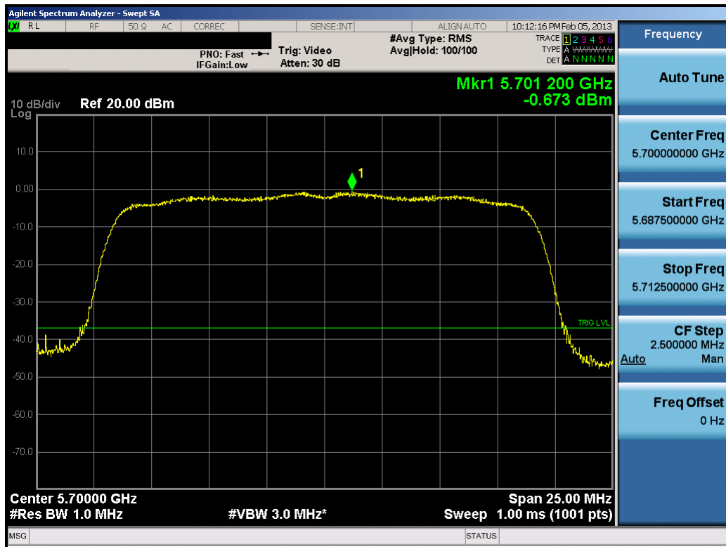
Plot 6-36. Peak Power Spectral Density Plot (20MHz BW 802.11n (UNII Band 3) – Ch. 140)
