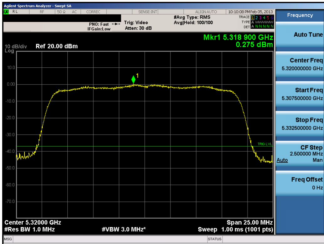
Plot 6-30. Peak Power Spectral Density Plot (20MHz BW 802.11n (UNII Band 2) – Ch. 64)
