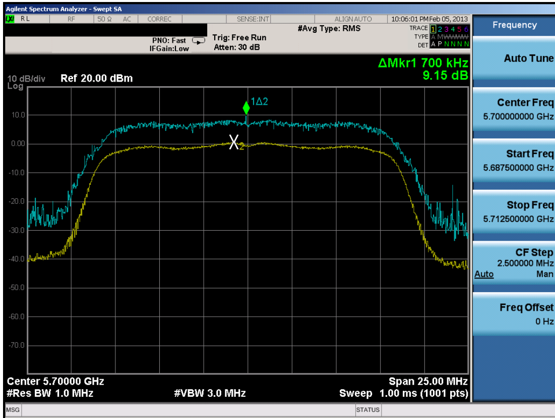
Plot 6-37. Peak Excursion Ratio Plot (802.11a)
