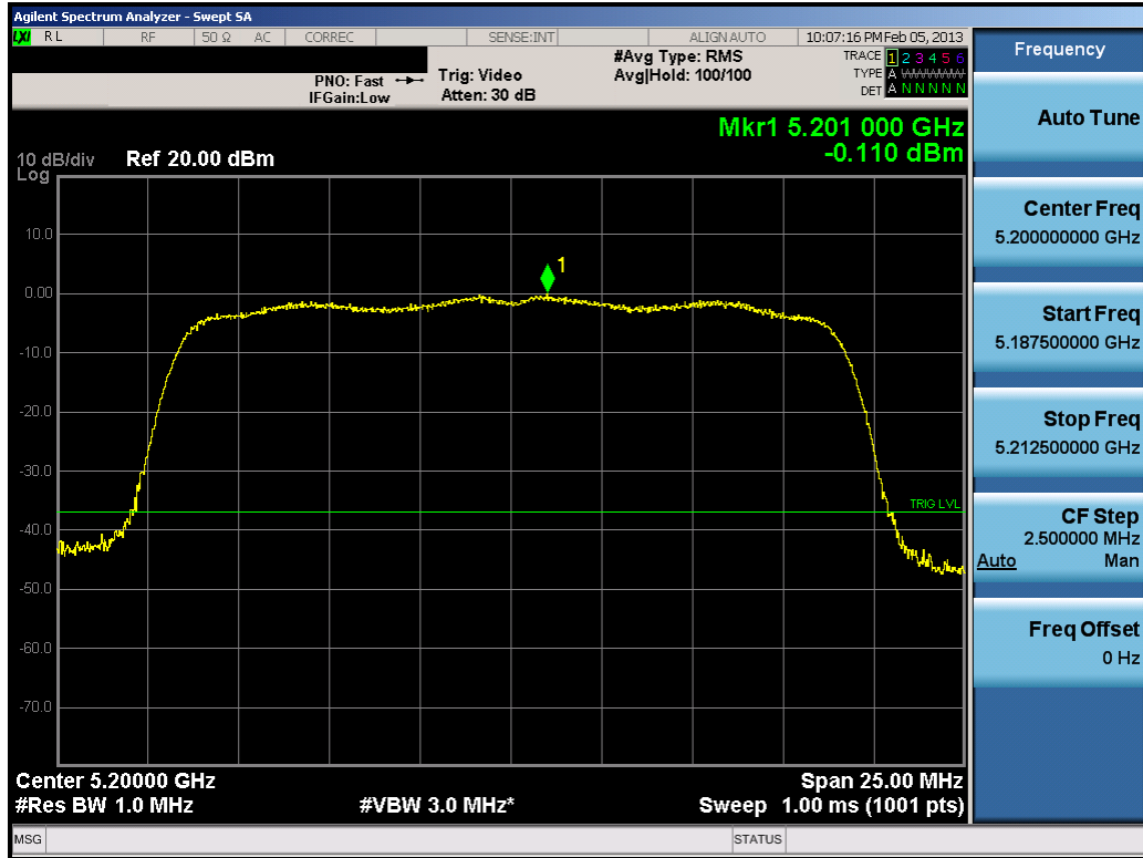
Plot 6-23. Peak Power Spectral Density Plot (20MHz BW 802.11n (UNII Band 1) – Ch. 40)
