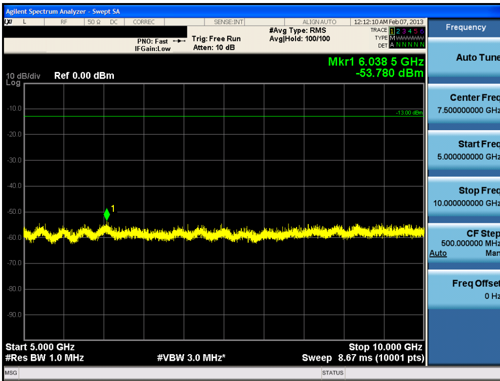
Plot 7-2. Conducted Spurious Plot (Cellular CDMA Mode – Ch. 1013)
