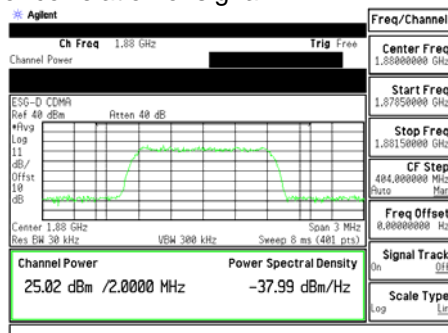
Figure 20 Signal Generator Modulated Signal
