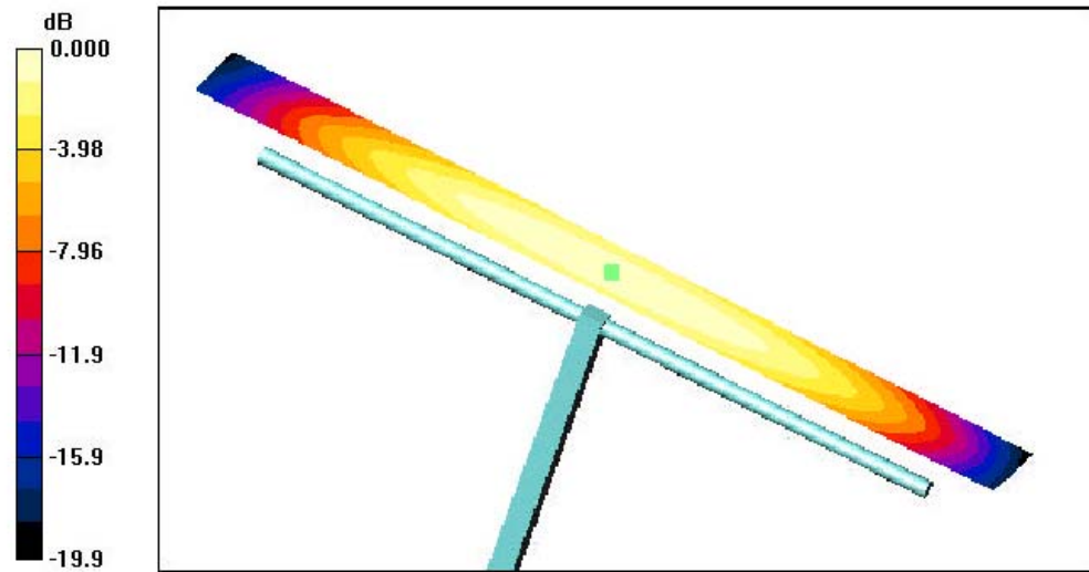
0 dB = 0.487 A/m
