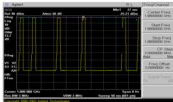
Figure 8-3 CDMA Zero-Span Plots
