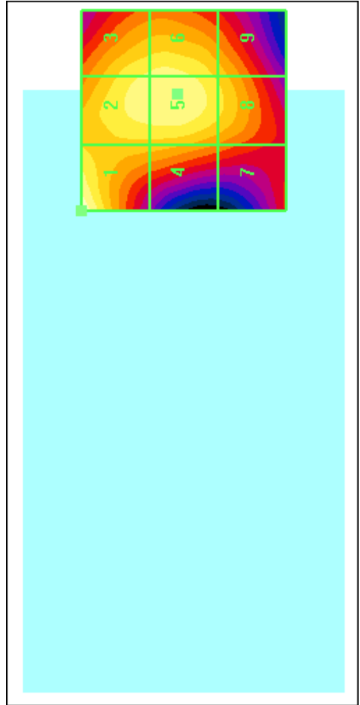
Figure 10-2 Sample H-field Scan Overlay
