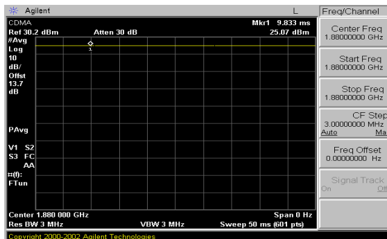
Figure 8-3 CDMA Zero-Span Plots
