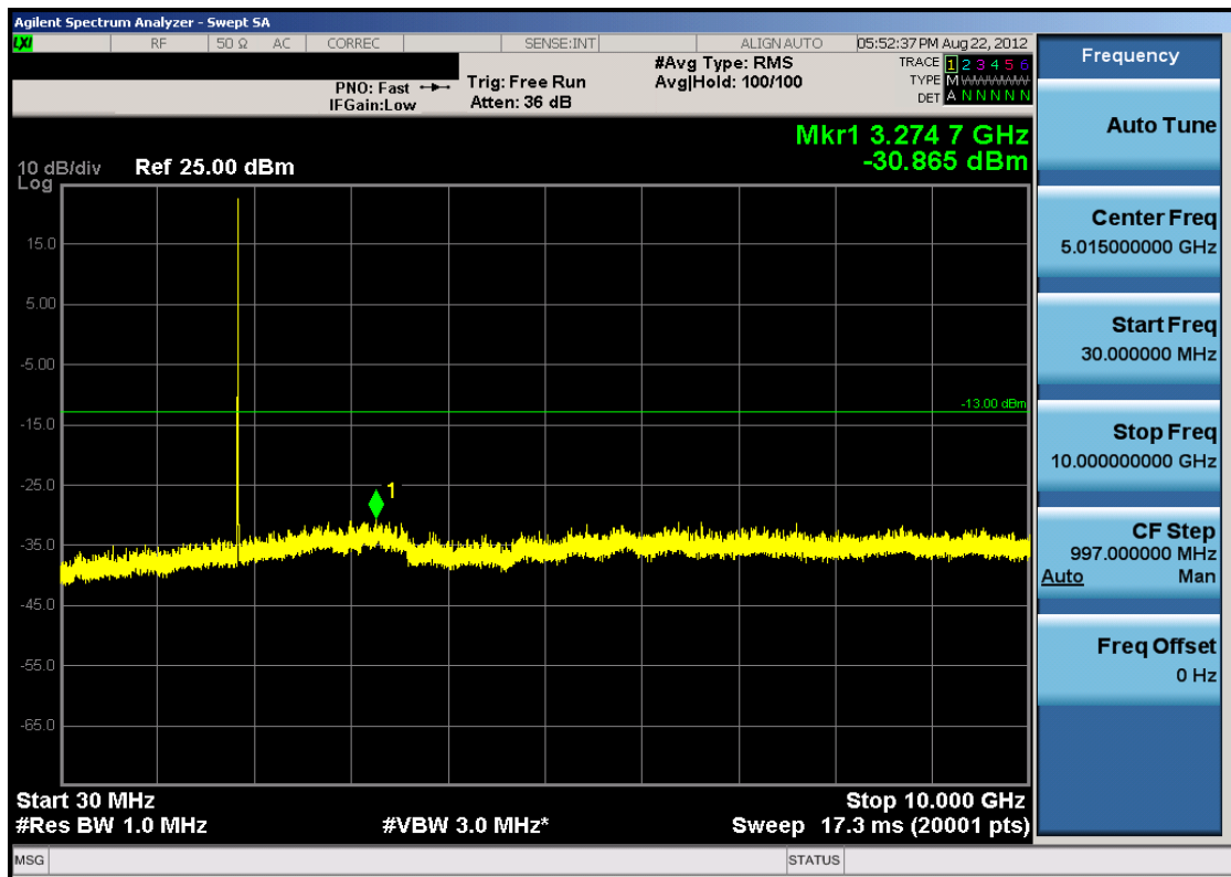
Plot 7-26. Conducted Spurious Plot (PCS WCDMA Mode – Ch. 9262)
