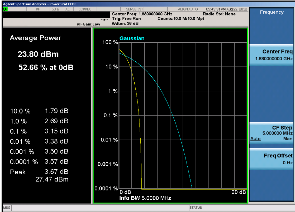
Plot 7-33. Peak-Average Ratio Plot (PCS WCDMA Mode – Ch. 9400)
