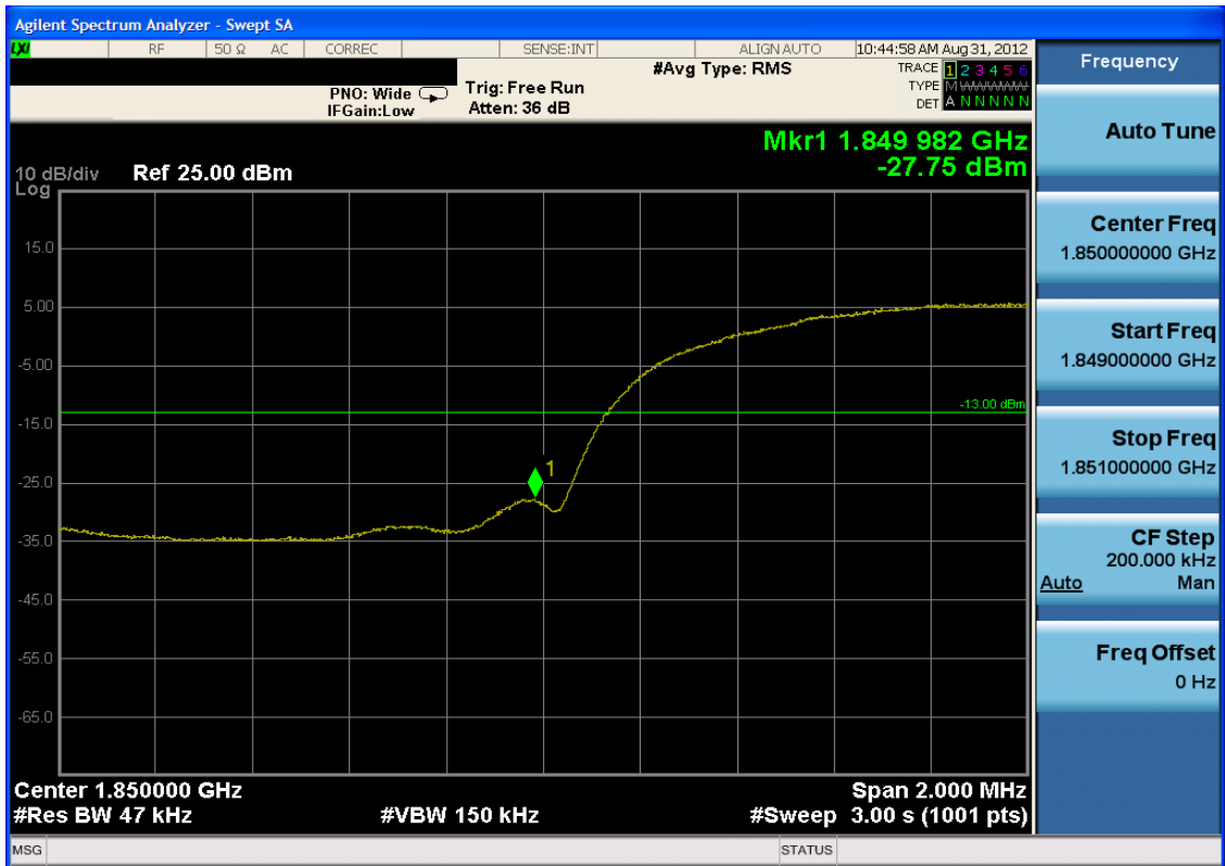
Plot 7-28. Band Edge Plot (PCS WCDMA Mode – Ch. 9262)
