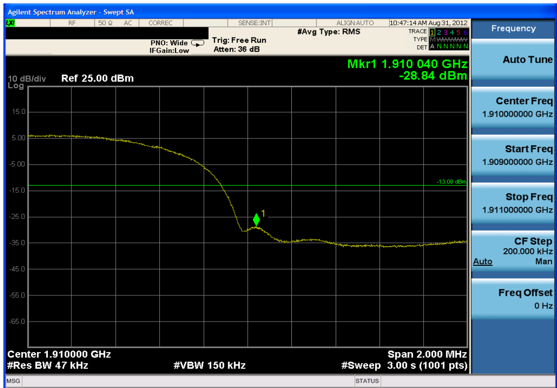
Plot 7-36. Band Edge Plot (PCS WCDMA Mode – Ch. 9538)
