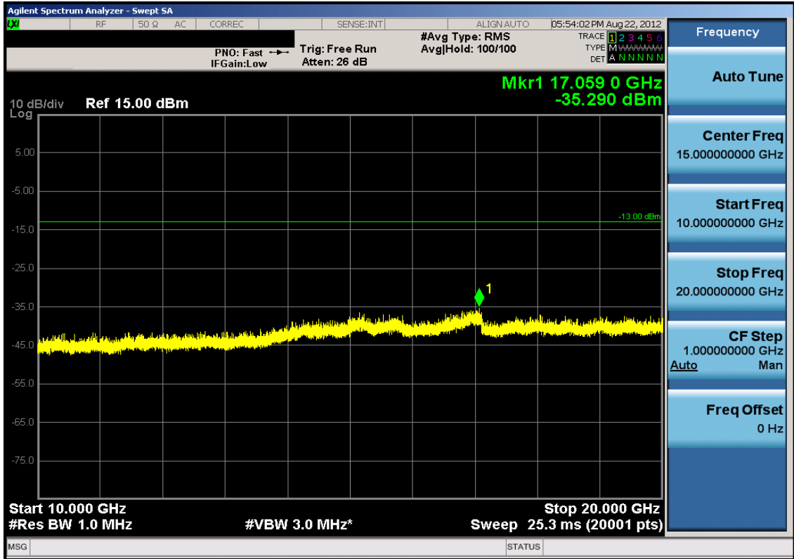
Plot 7-35. Conducted Spurious Plot (PCS WCDMA Mode – Ch. 9538)
