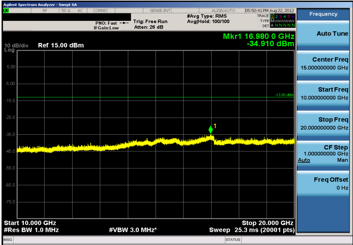
Plot 7-31. Conducted Spurious Plot (PCS WCDMA Mode – Ch. 9400)
