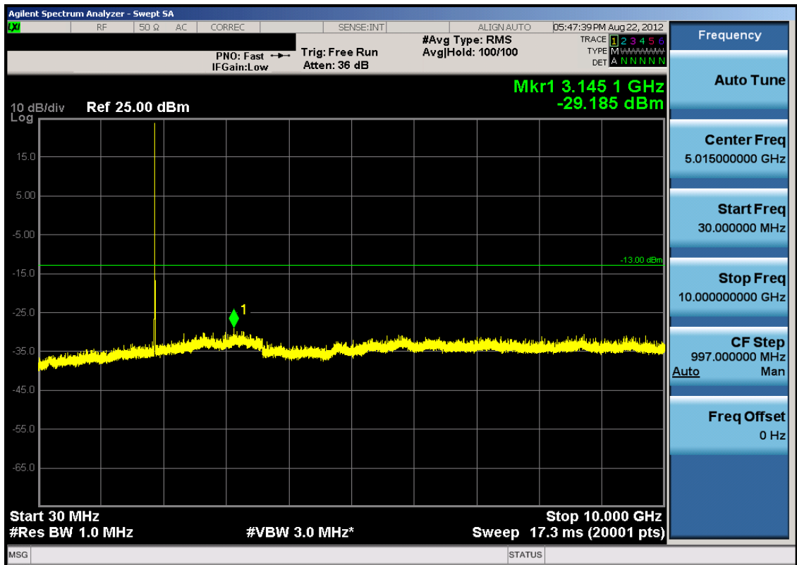
Plot 7-30. Conducted Spurious Plot (PCS WCDMA Mode – Ch. 9400)
