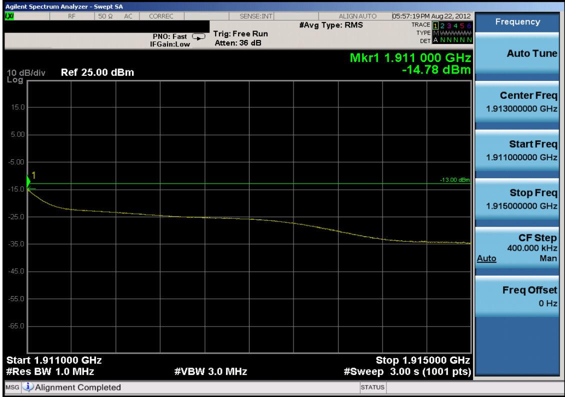
Plot 7-37. 4MHz Span Plot (PCS WCDMA Mode – Ch. 9538)
