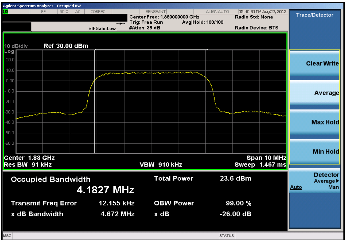
Plot 7-32. Occupied Bandwidth Plot (PCS WCDMA Mode – Ch. 9400)
