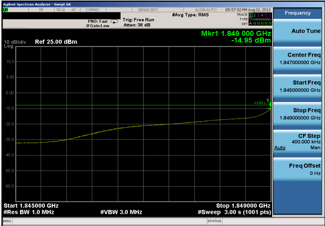
Plot 7-29. 4MHz Span Plot (PCS WCDMA Mode – Ch. 9262)
