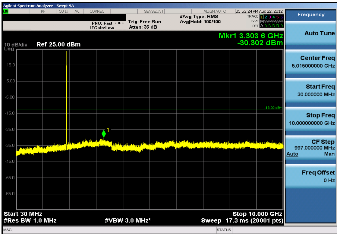
Plot 7-34. Conducted Spurious Plot (PCS WCDMA Mode – Ch. 9538)
