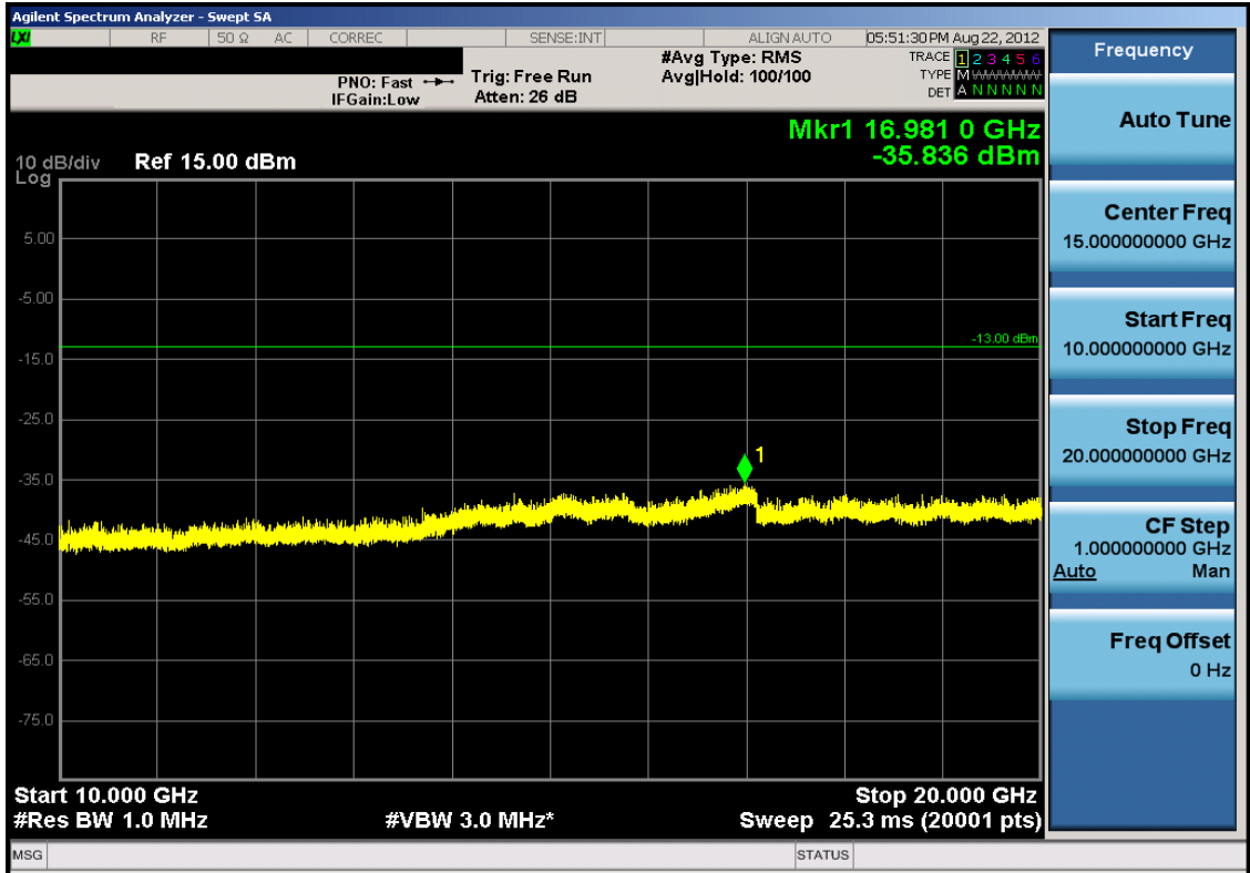
Plot 7-27. Conducted Spurious Plot (PCS WCDMA Mode – Ch. 9262)
