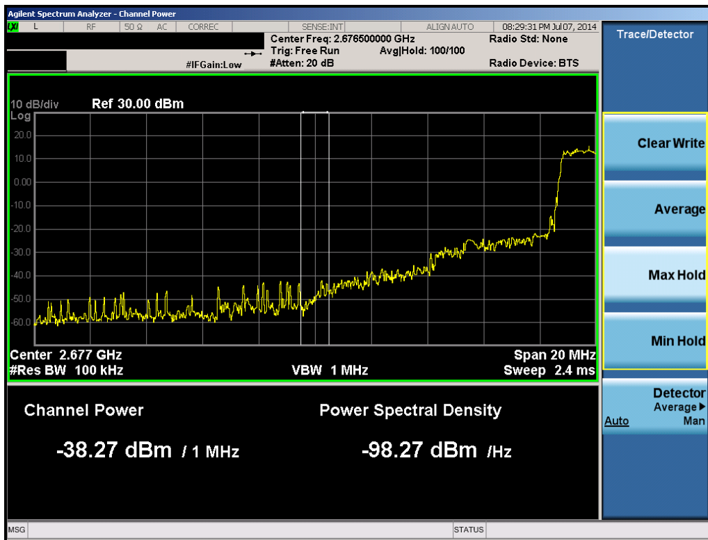
Plot 6-73. 1MHz Integration (Band 41 – 5.0MHz QPSK – RB Size 25, RB Offset 0 – High Channel)
