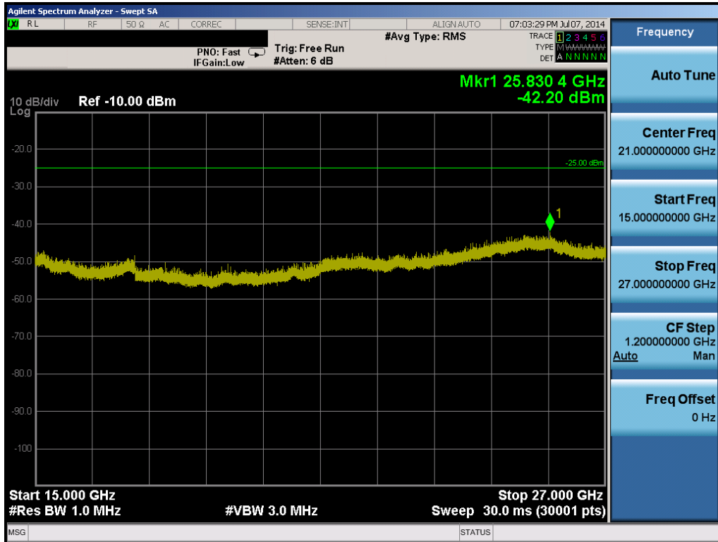
Plot 6-44. Conducted Spurious Plot (Band 41 – 5.0MHz QPSK – RB Size 25, RB Offset 0 – Low Channel)
