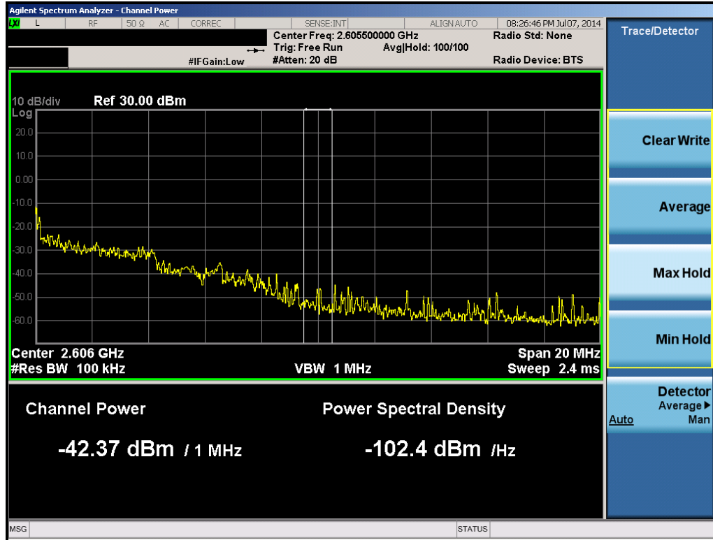
Plot 6-58. 1MHz Integration (Band 41 – 5.0MHz QPSK – RB Size 25, RB Offset 0 – Mid Channel)
