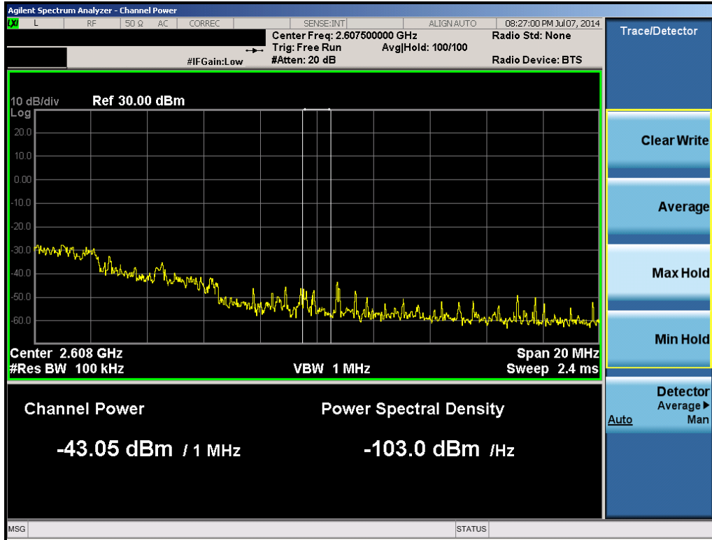
Plot 6-60. 1MHz Integration (Band 41 – 5.0MHz QPSK – RB Size 25, RB Offset 0 – Mid Channel)
