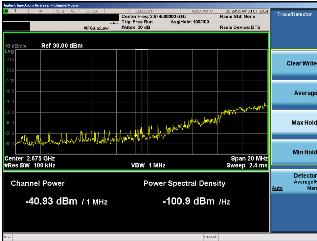
Plot 6-71. 1MHz Integration (Band 41 – 5.0MHz QPSK – RB Size 25, RB Offset 0 – High Channel)
