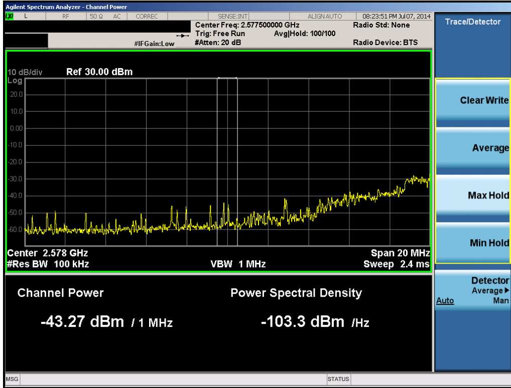
Plot 6-48. 1MHz Integration (Band 41 – 5.0MHz QPSK – RB Size 25, RB Offset 0 – Mid Channel)
