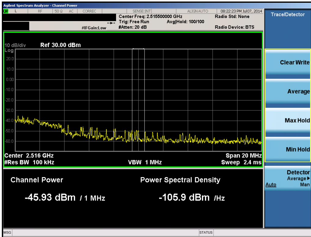
Plot 6-41. 1MHz Integration (Band 41 – 5.0MHz QPSK – RB Size 25, RB Offset 0 – Low Channel)
