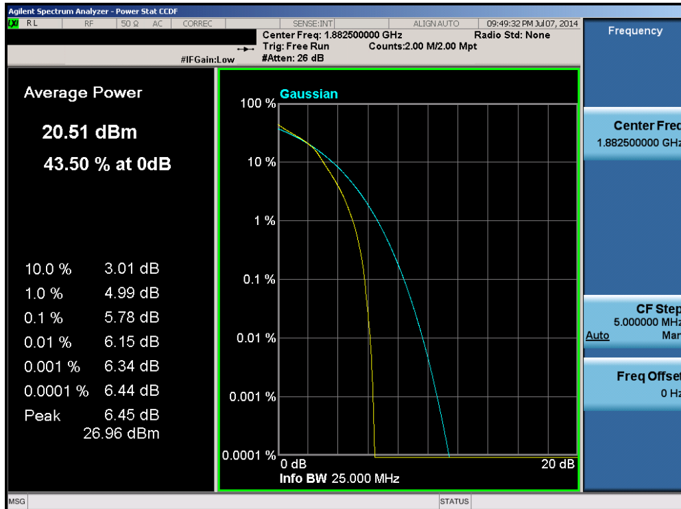
Plot 6-100. PAR Plot (Band 25 – 15.0MHz 16-QAM – RB Size 75)
