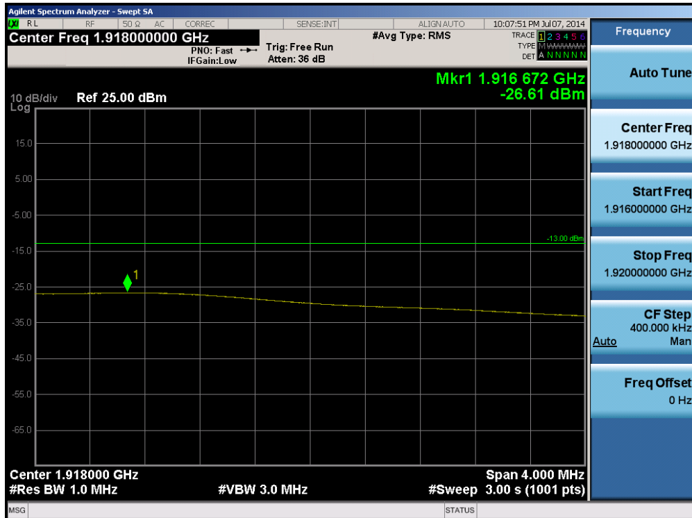
Plot 6-89. Upper Extended Band Edge Plot (Band 25 – 15.0MHz QPSK – RB Size 75)
