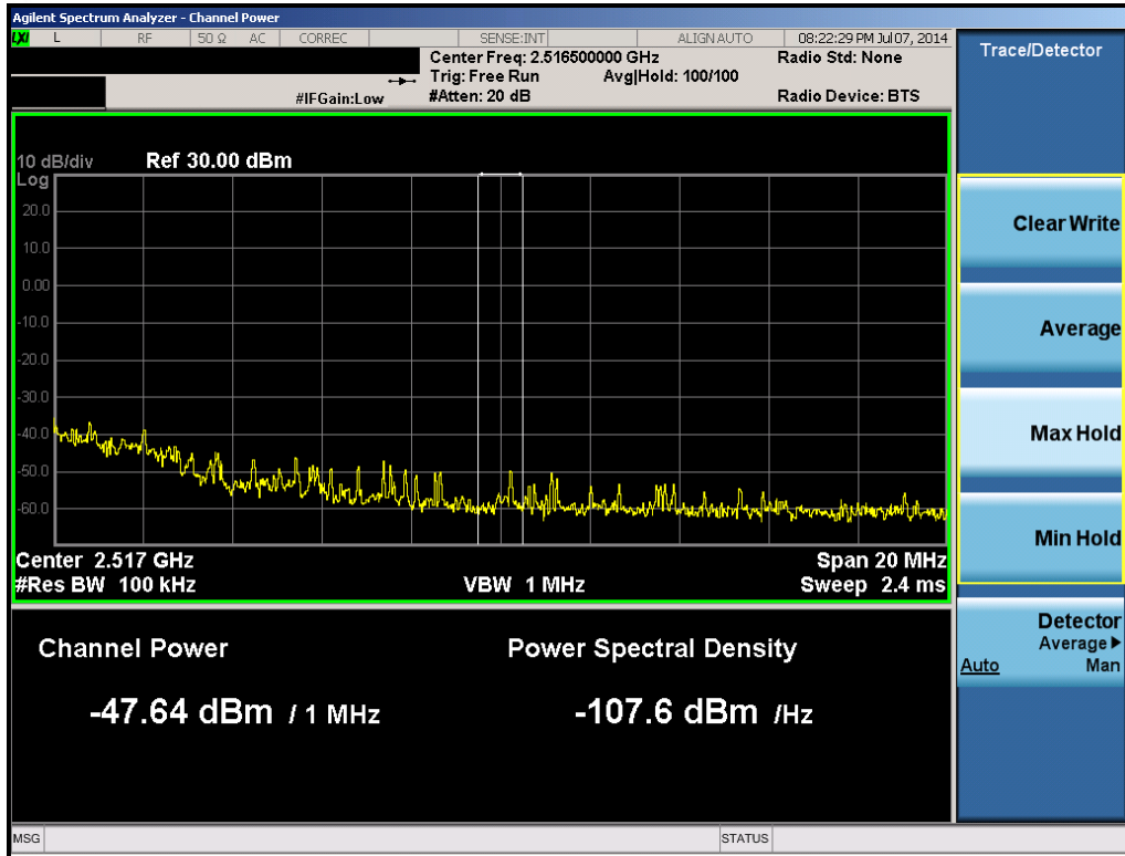
Plot 6-42. 1MHz Integration (Band 41 – 5.0MHz QPSK – RB Size 25, RB Offset 0 – Low Channel)
