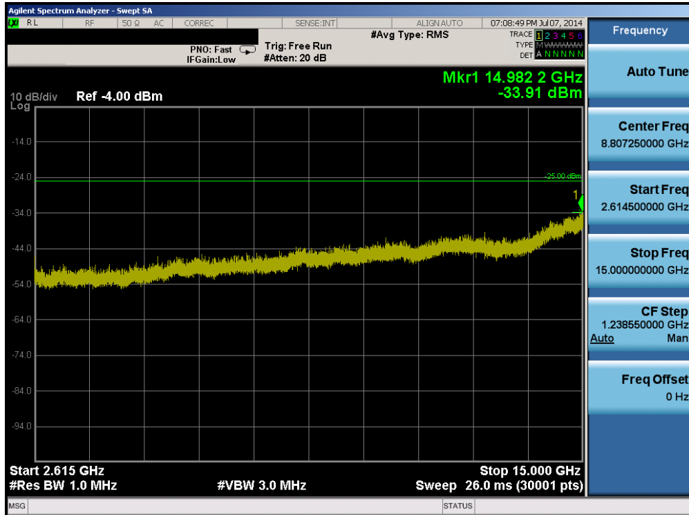
Plot 6-68. Conducted Spurious Plot (Band 41 – 5.0MHz QPSK – RB Size 25, RB Offset 0 – Mid Channel)
