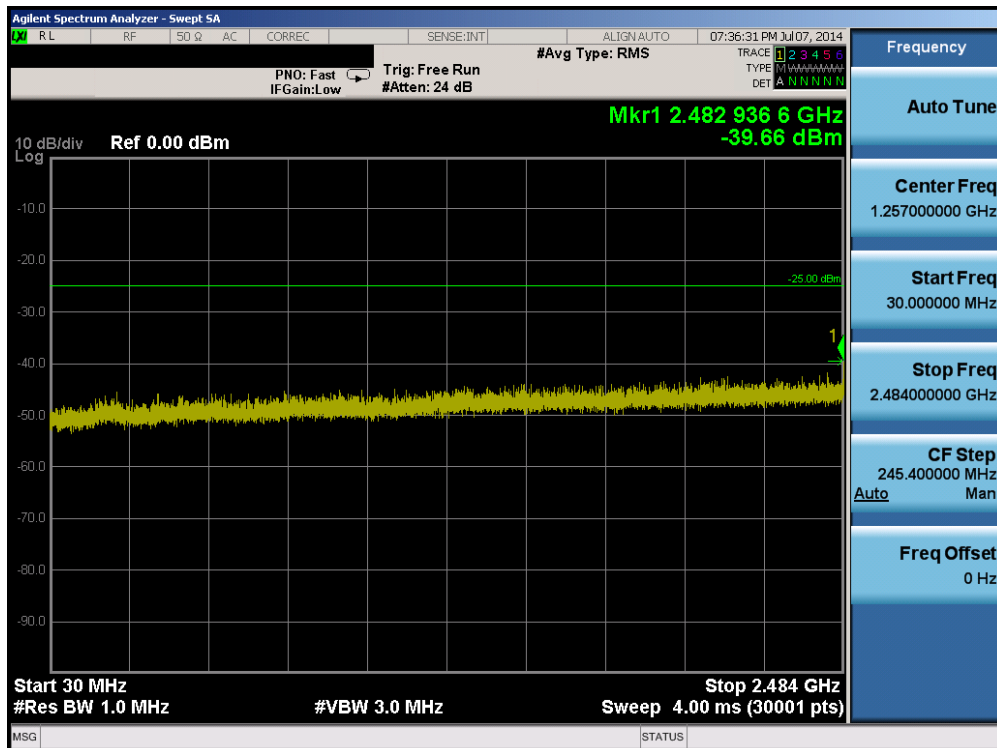
Plot 6-27. Conducted Spurious Plot (Band 41 – 5.0MHz QPSK – RB Size 25, RB Offset 0 – Low Channel)
