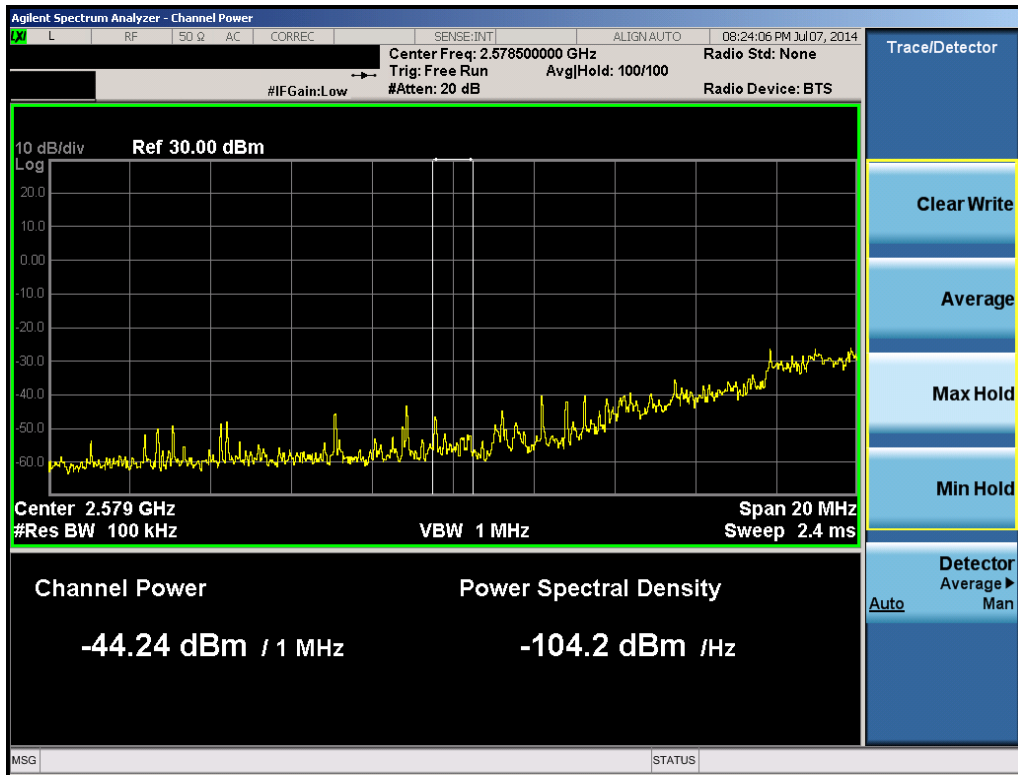
Plot 6-49. 1MHz Integration (Band 41 – 5.0MHz QPSK – RB Size 25, RB Offset 0 – Mid Channel)
