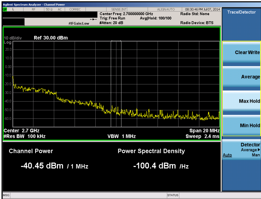
Plot 6-79. 1MHz Integration (Band 41 – 5.0MHz QPSK – RB Size 25, RB Offset 0 – High Channel)
