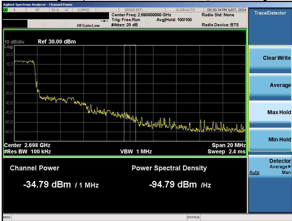
Plot 6-77. 1MHz Integration (Band 41 – 5.0MHz QPSK – RB Size 25, RB Offset 0 – High Channel)
