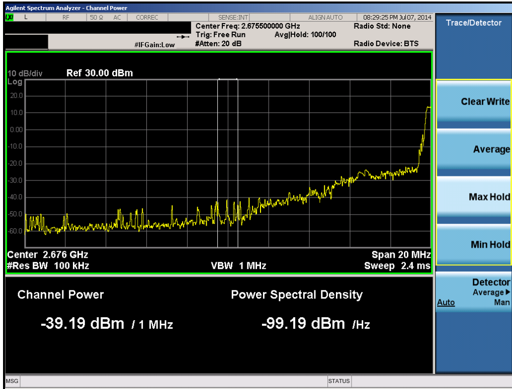
Plot 6-72. 1MHz Integration (Band 41 – 5.0MHz QPSK – RB Size 25, RB Offset 0 – High Channel)
