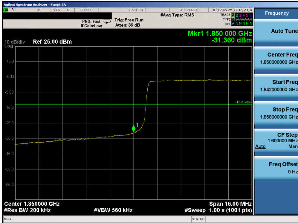
Plot 6-90. Lower Band Edge Plot (Band 25 – 20.0MHz QPSK – RB Size 100)
