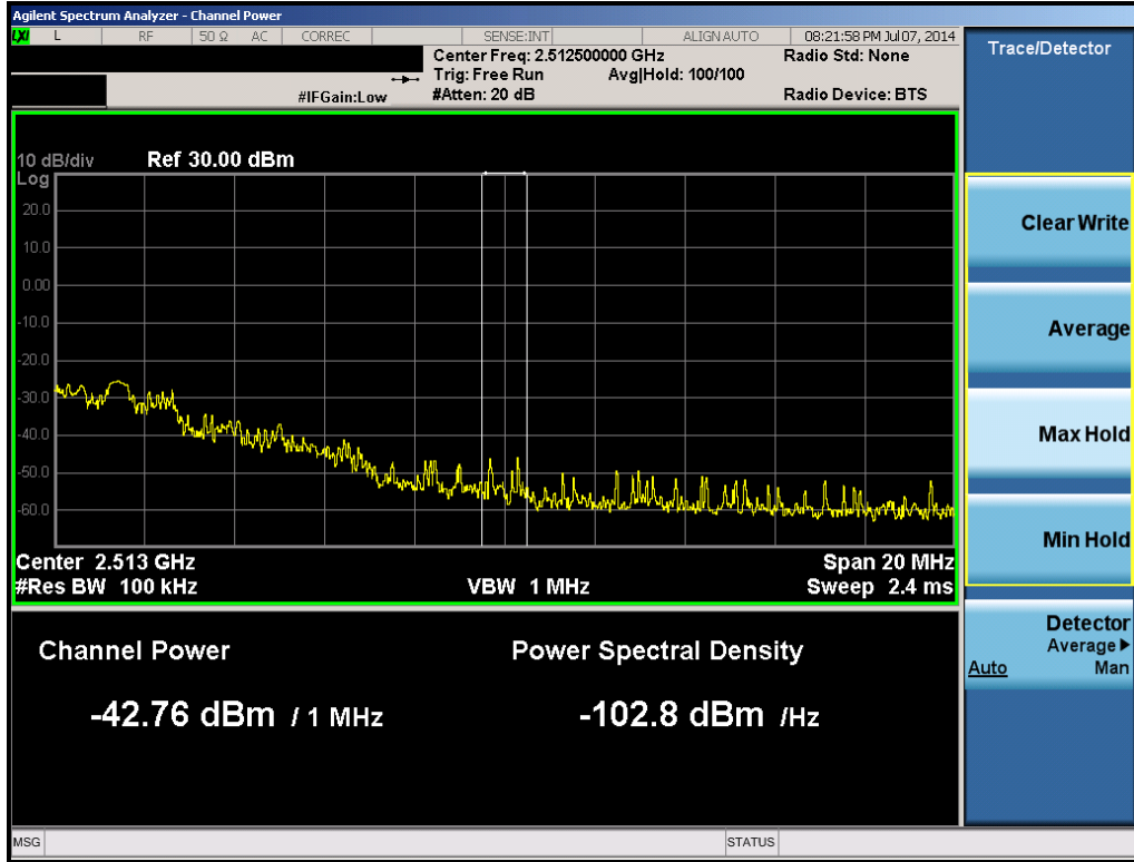
Plot 6-38. 1MHz Integration (Band 41 – 5.0MHz QPSK – RB Size 25, RB Offset 0 – Low Channel)
