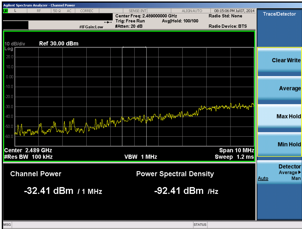
Plot 6-33. 1MHz Integration (Band 41 – 5.0MHz QPSK – RB Size 25, RB Offset 0 – Low Channel)
