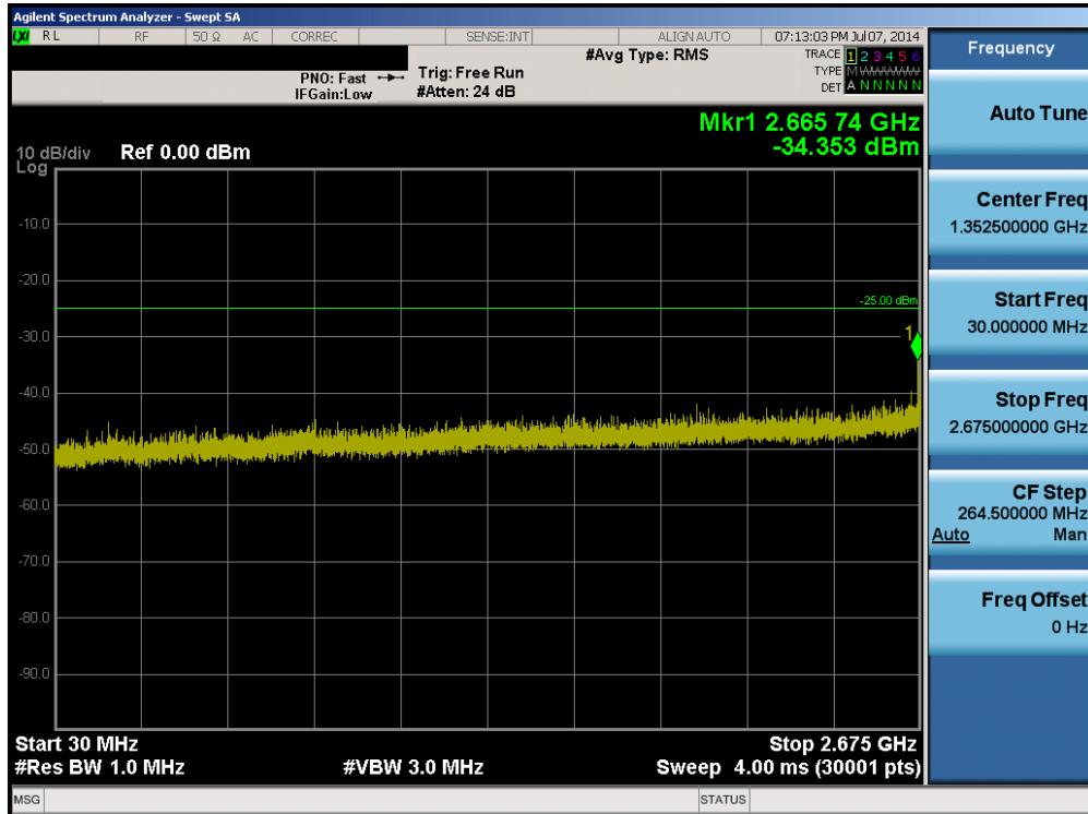
Plot 6-70. Conducted Spurious Plot (Band 41 – 5.0MHz QPSK – RB Size 25, RB Offset 0 – High Channel)
