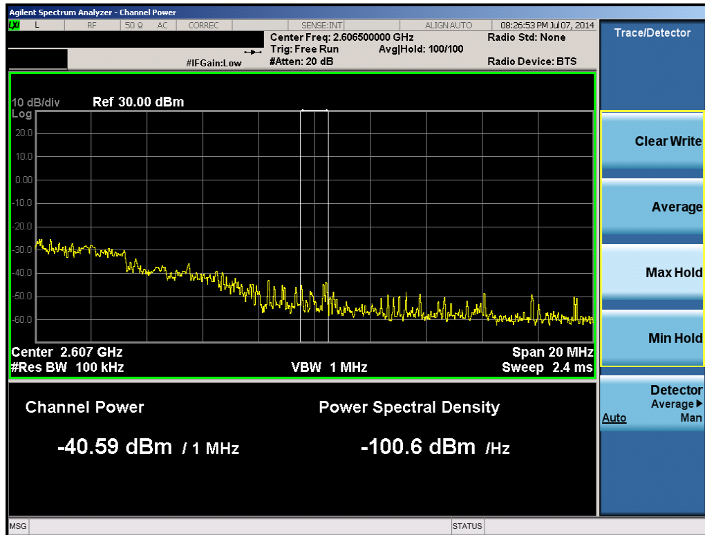
Plot 6-59. 1MHz Integration (Band 41 – 5.0MHz QPSK – RB Size 25, RB Offset 0 – Mid Channel)
