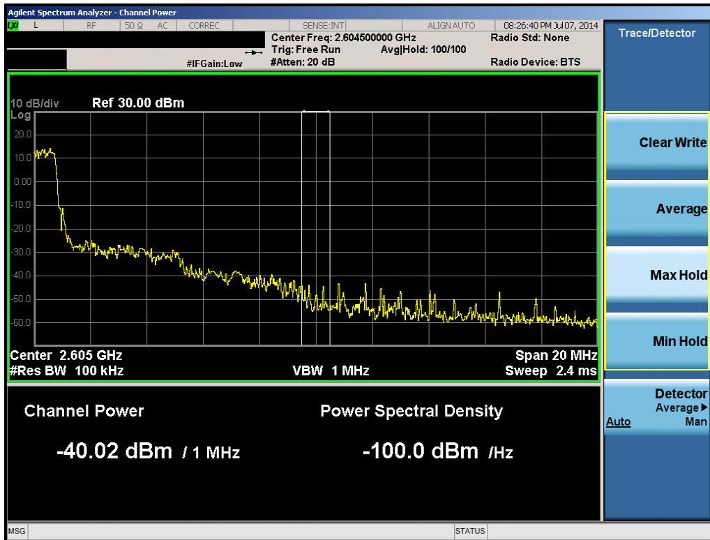
Plot 6-57. 1MHz Integration (Band 41 – 5.0MHz QPSK – RB Size 25, RB Offset 0 – Mid Channel)
