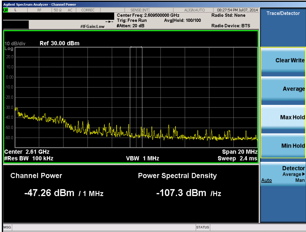
Plot 6-62. 1MHz Integration (Band 41 – 5.0MHz QPSK – RB Size 25, RB Offset 0 – Mid Channel)
