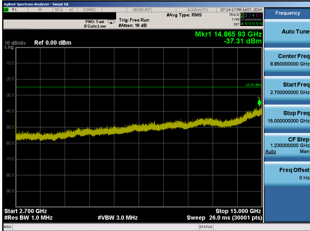
Plot 6-80. Conducted Spurious Plot (Band 41 – 5.0MHz QPSK – RB Size 25, RB Offset 0 – High Channel)
