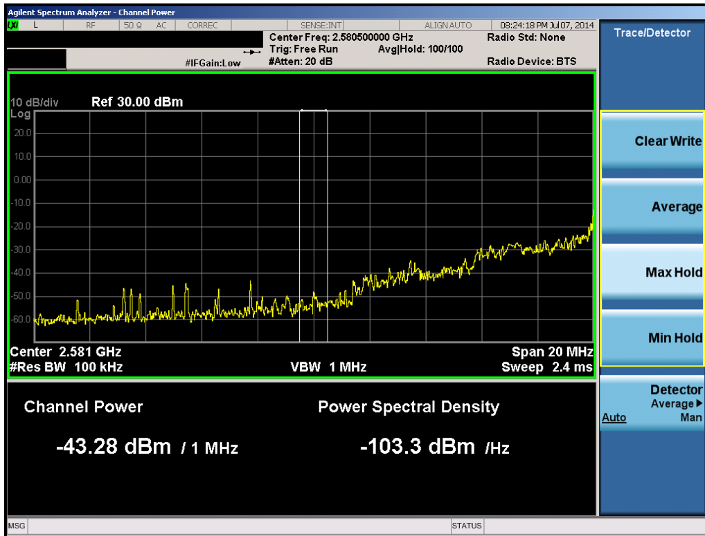
Plot 6-51. 1MHz Integration (Band 41 – 5.0MHz QPSK – RB Size 25, RB Offset 0 – Mid Channel)
