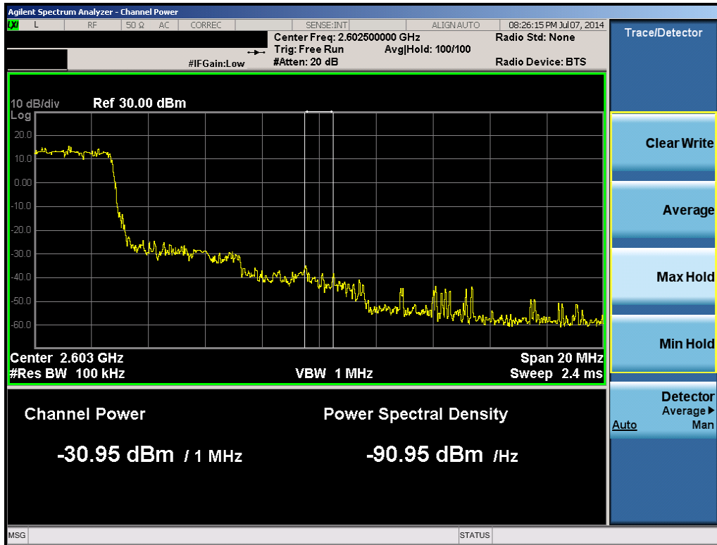
Plot 6-55. 1MHz Integration (Band 41 – 5.0MHz QPSK – RB Size 25, RB Offset 0 – Mid Channel)
