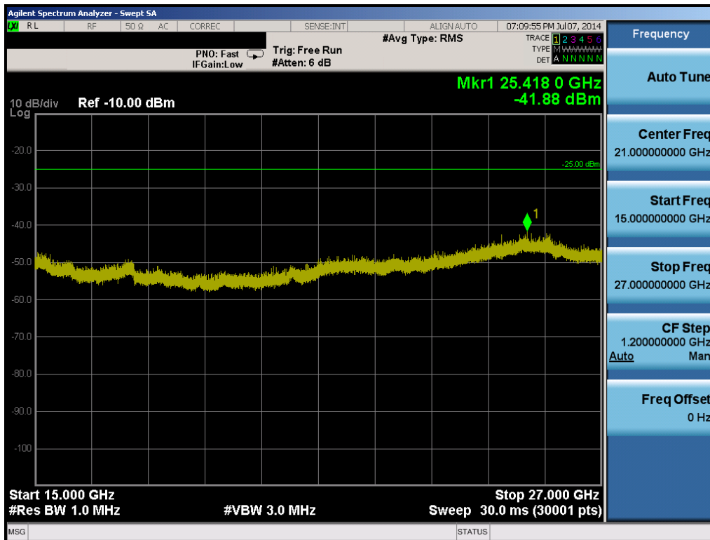
Plot 6-69. Conducted Spurious Plot (Band 41 – 5.0MHz QPSK – RB Size 25, RB Offset 0 – Mid Channel)
