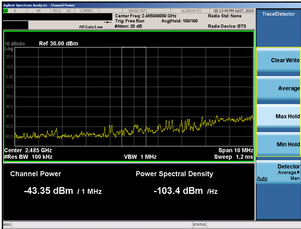
Plot 6-29. 1MHz Integration (Band 41 – 5.0MHz QPSK – RB Size 25, RB Offset 0 – Low Channel)
