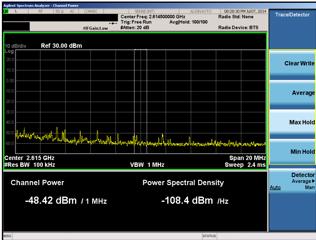
Plot 6-67. 1MHz Integration (Band 41 – 5.0MHz QPSK – RB Size 25, RB Offset 0 – Mid Channel)
