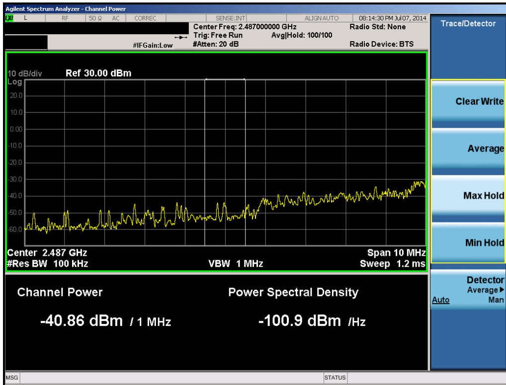
Plot 6-31. 1MHz Integration (Band 41 – 5.0MHz QPSK – RB Size 25, RB Offset 0 – Low Channel)
