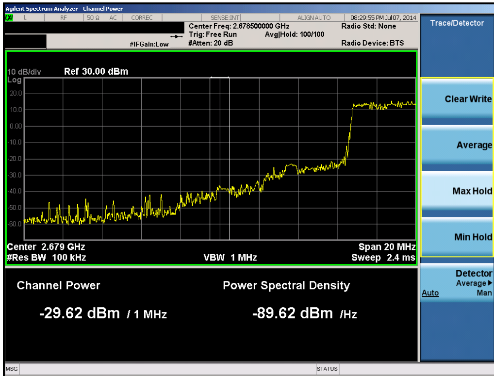
Plot 6-75. 1MHz Integration (Band 41 – 5.0MHz QPSK – RB Size 25, RB Offset 0 – High Channel)
