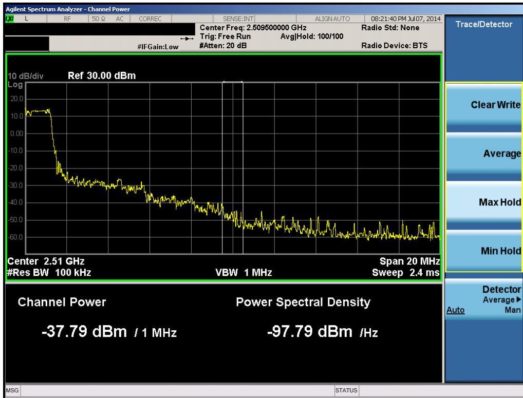
Plot 6-35. 1MHz Integration (Band 41 – 5.0MHz QPSK – RB Size 25, RB Offset 0 – Low Channel)
