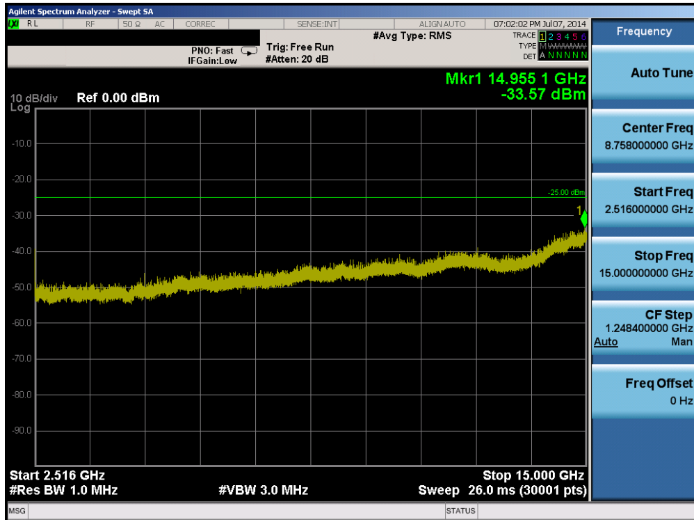
Plot 6-43. Conducted Spurious Plot (Band 41 – 5.0MHz QPSK – RB Size 25, RB Offset 0 – Low Channel)
