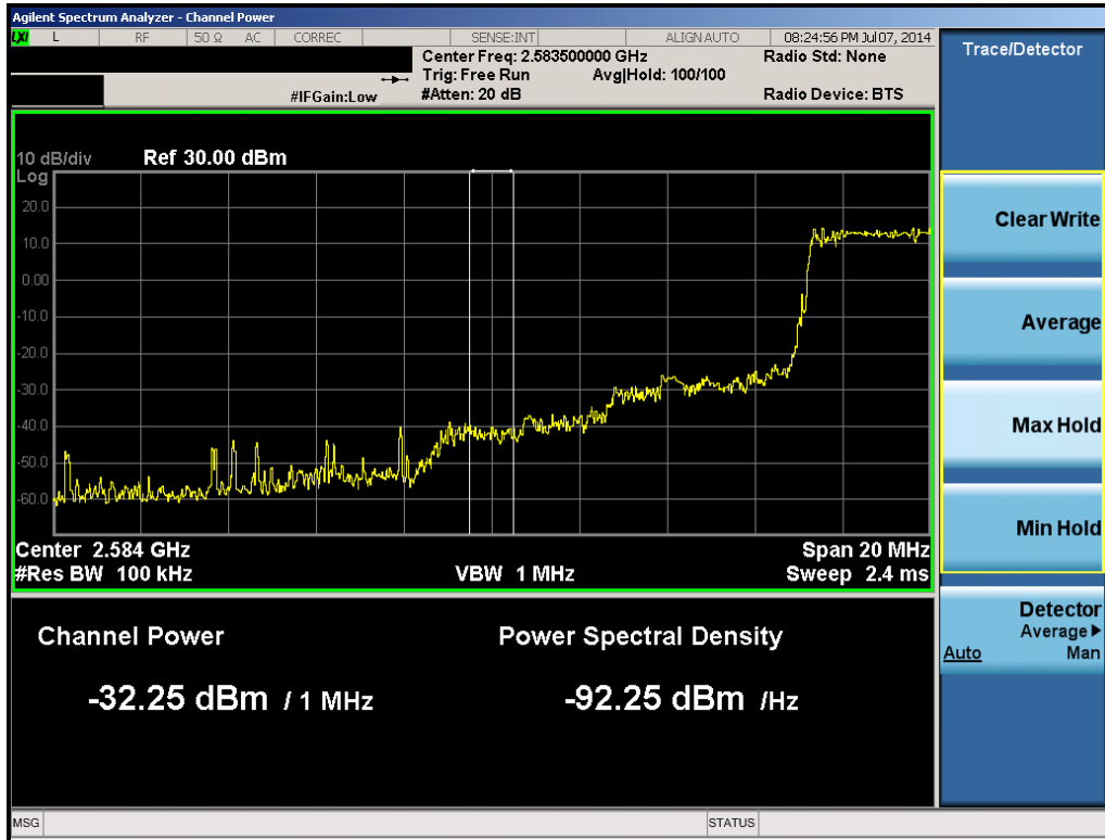
Plot 6-54. 1MHz Integration (Band 41 – 5.0MHz QPSK – RB Size 25, RB Offset 0 – Mid Channel)
