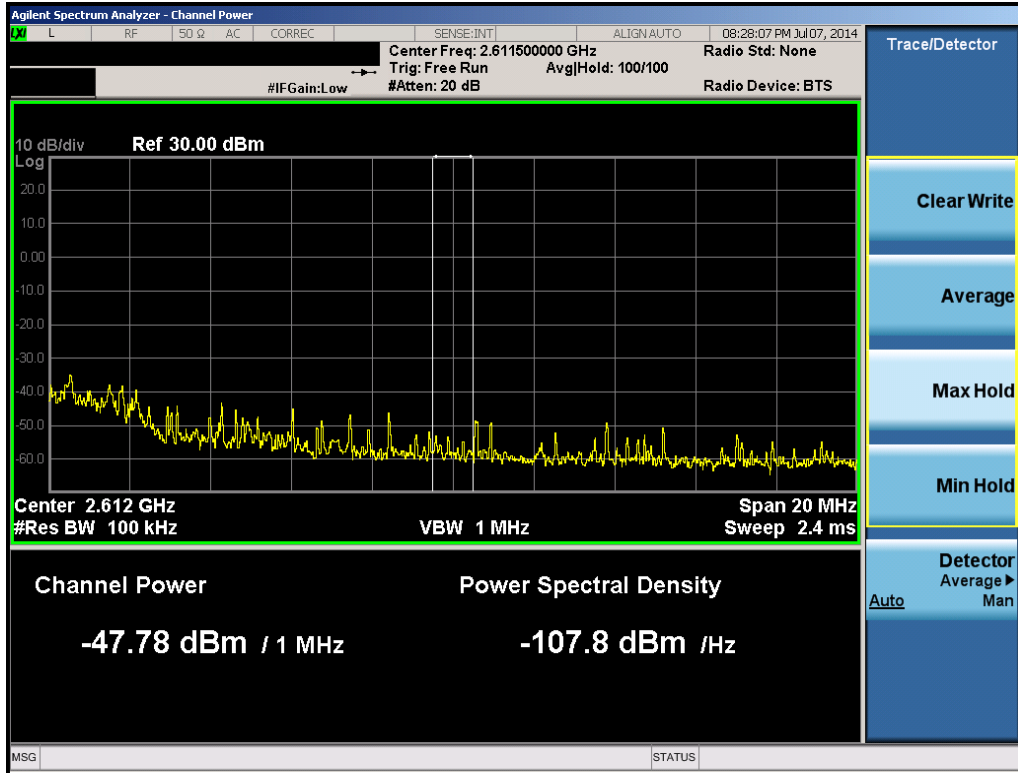
Plot 6-64. 1MHz Integration (Band 41 – 5.0MHz QPSK – RB Size 25, RB Offset 0 – Mid Channel)
