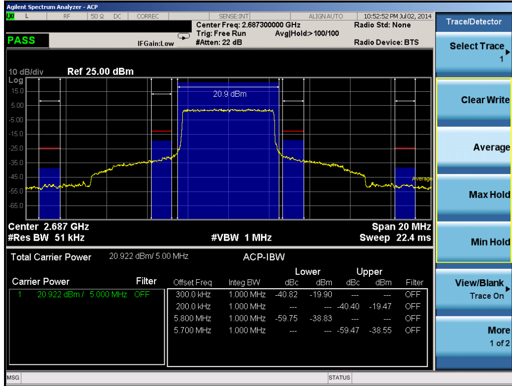
Plot 6-96. Upper ACP Plot (Band 41 – 5.0MHz QPSK – RB Size 25)
