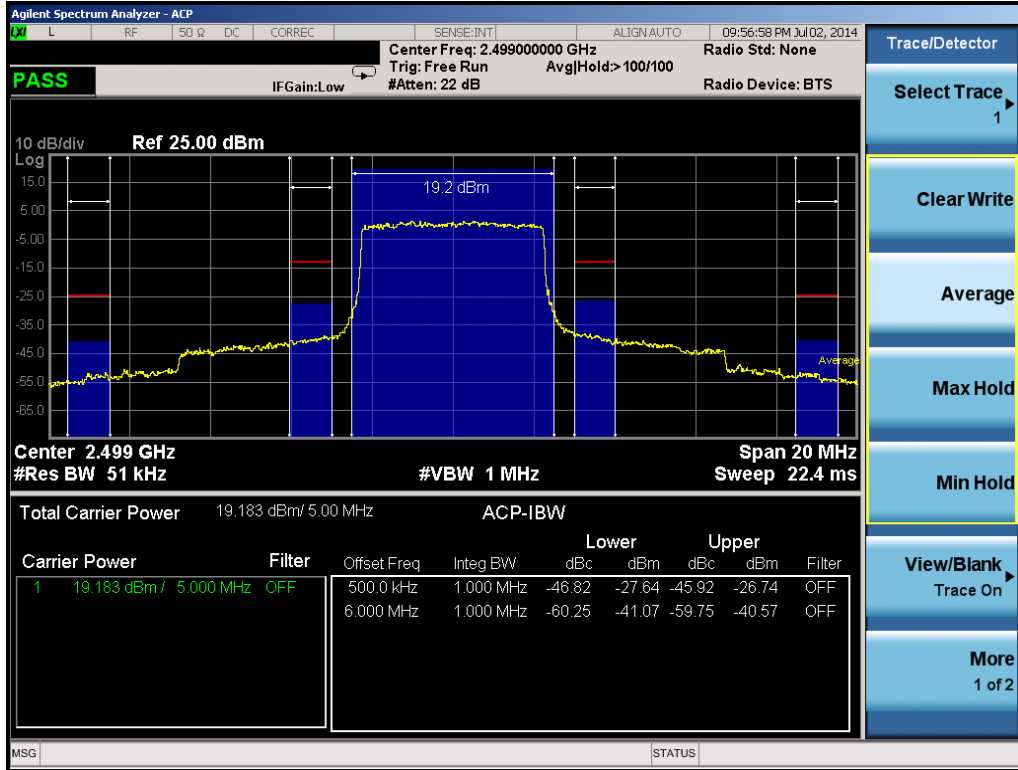
Plot 6-94. Lower ACP Plot (Band 41 – 5.0MHz QPSK – RB Size 25)
