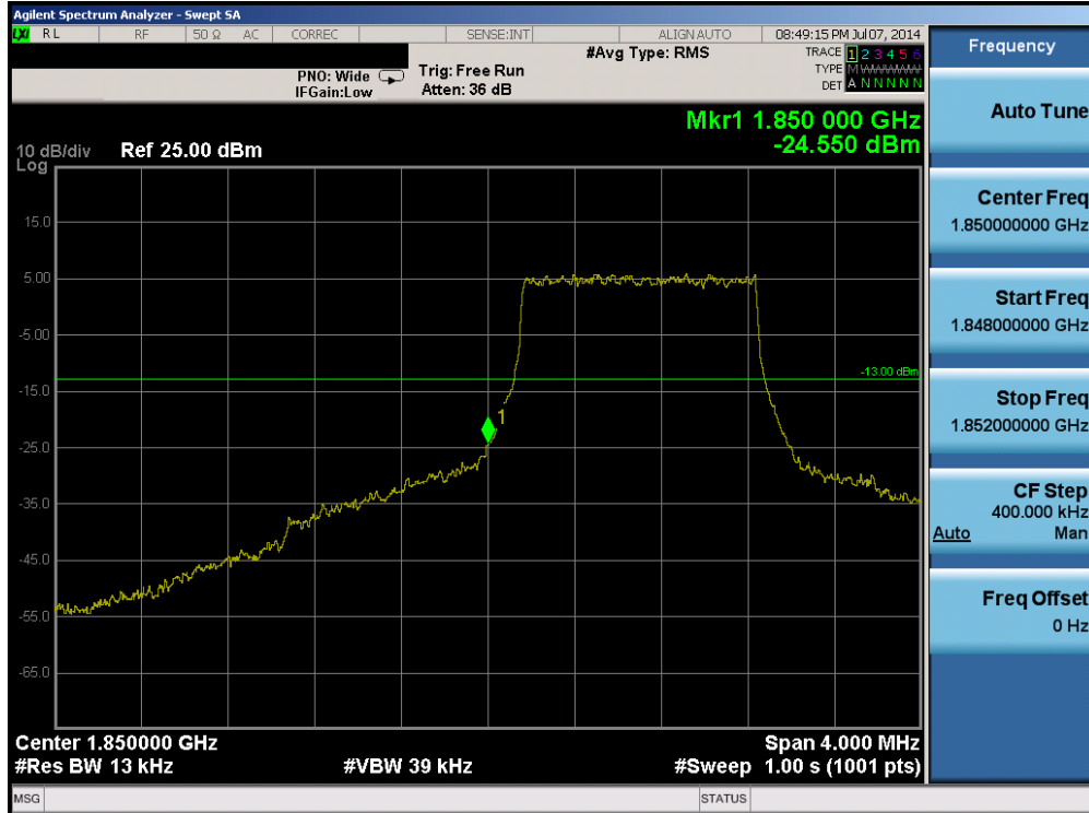
Plot 6-82. Lower Band Edge Plot (Band 25 – 1.4MHz QPSK – RB Size 6)
