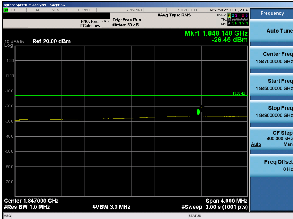
Plot 6-87. Lower Extended Band Edge Plot (Band 25 – 15.0MHz QPSK – RB Size 75)
