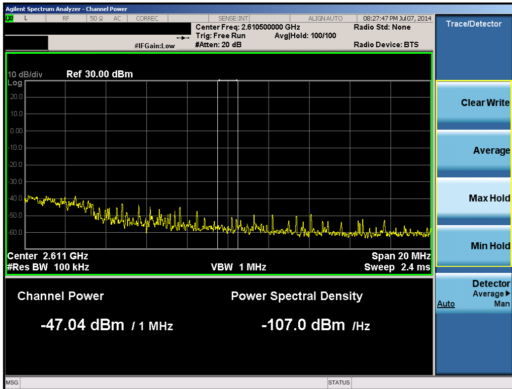
Plot 6-63. 1MHz Integration (Band 41 – 5.0MHz QPSK – RB Size 25, RB Offset 0 – Mid Channel)
