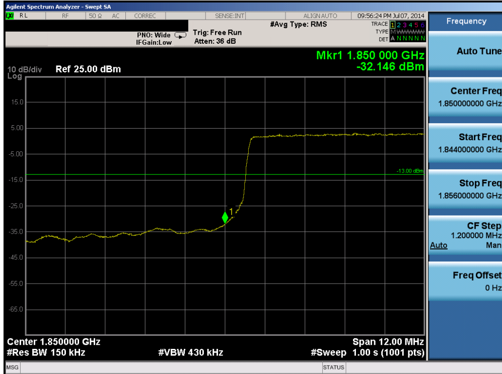
Plot 6-86. Lower Band Edge Plot (Band 25 – 15.0MHz QPSK – RB Size 75)
