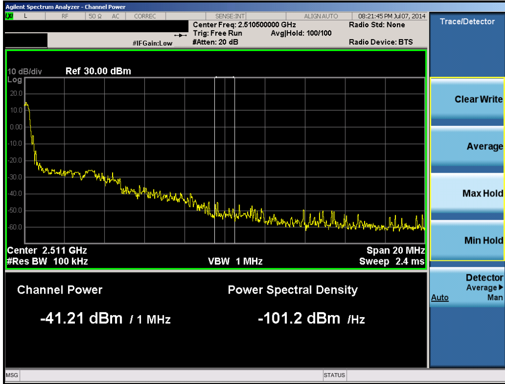
Plot 6-36. 1MHz Integration (Band 41 – 5.0MHz QPSK – RB Size 25, RB Offset 0 – Low Channel)
