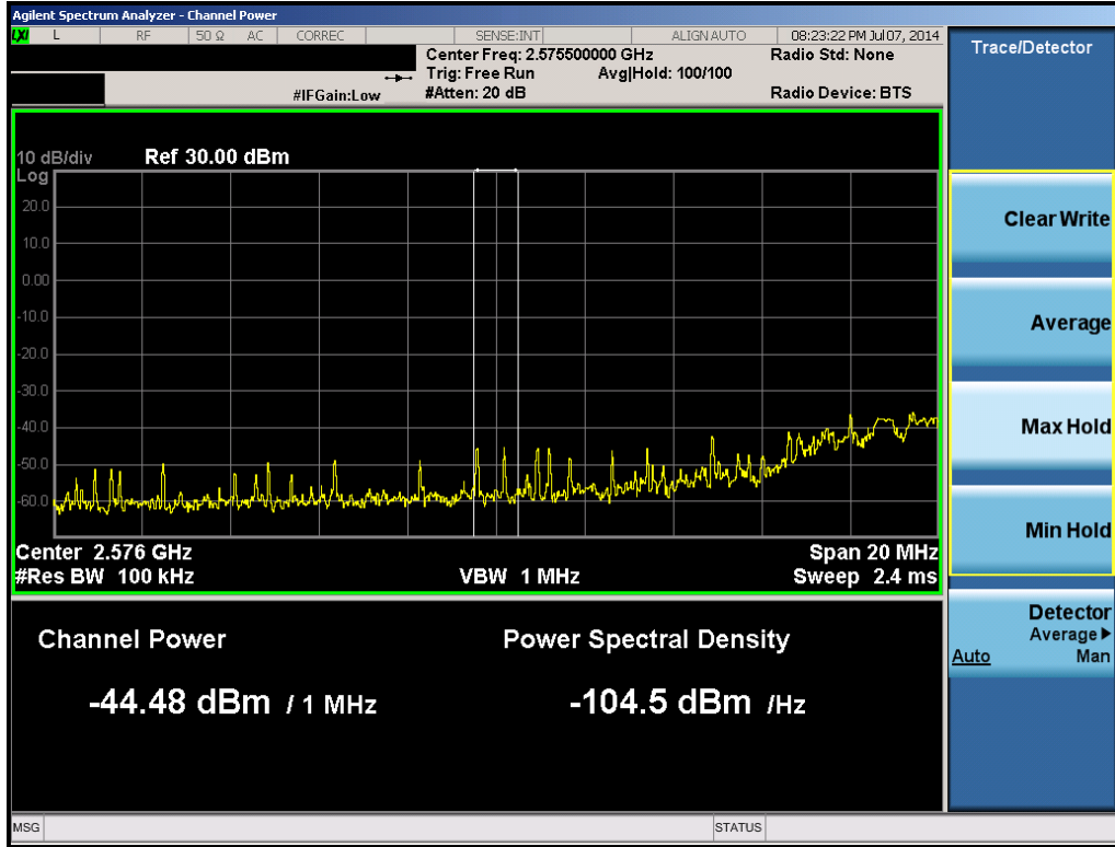
Plot 6-46. 1MHz Integration (Band 41 – 5.0MHz QPSK – RB Size 25, RB Offset 0 – Mid Channel)
