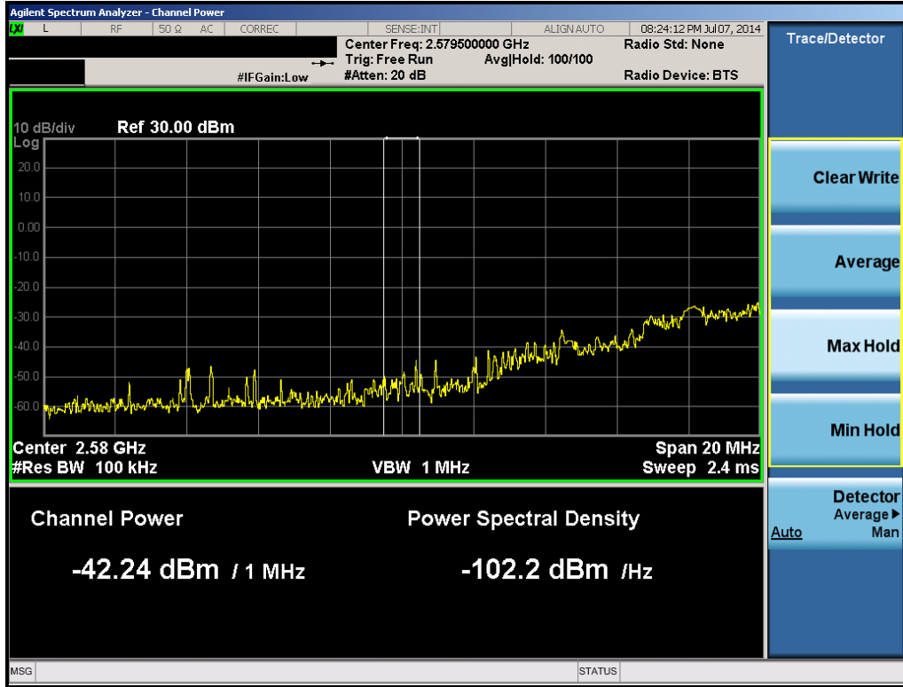
Plot 6-50. 1MHz Integration (Band 41 – 5.0MHz QPSK – RB Size 25, RB Offset 0 – Mid Channel)
