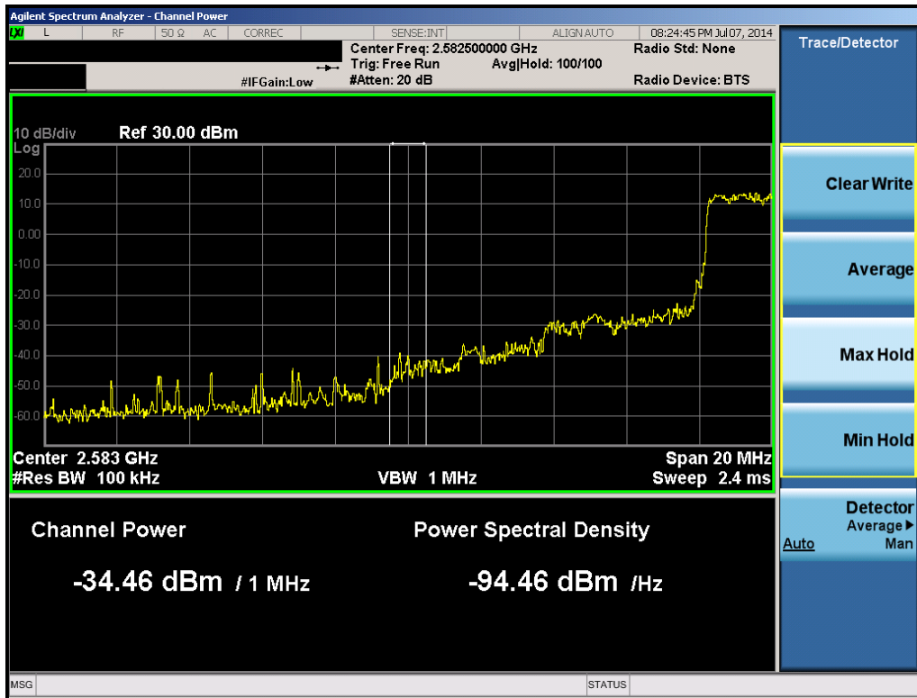
Plot 6-53. 1MHz Integration (Band 41 – 5.0MHz QPSK – RB Size 25, RB Offset 0 – Mid Channel)
