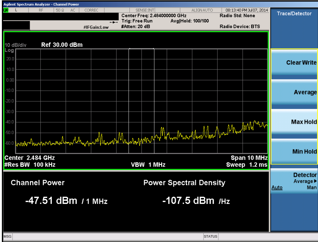
Plot 6-28. 1MHz Integration (Band 41 – 5.0MHz QPSK – RB Size 25, RB Offset 0 – Low Channel)
