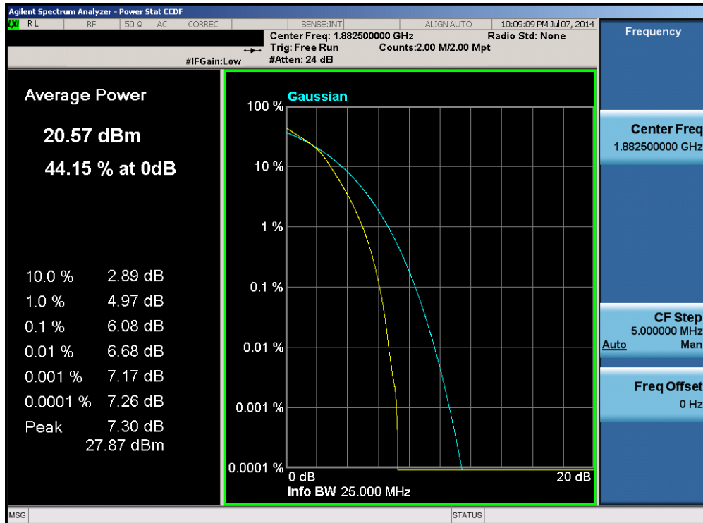
Plot 6-102. PAR Plot (Band 25 – 20.0MHz 16-QAM – RB Size 100)
