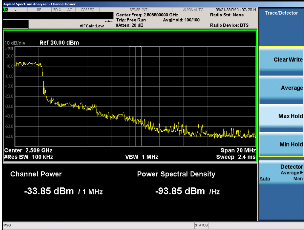
Plot 6-34. 1MHz Integration (Band 41 – 5.0MHz QPSK – RB Size 25, RB Offset 0 – Low Channel)
