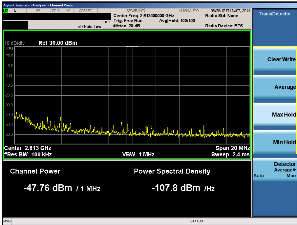
Plot 6-65. 1MHz Integration (Band 41 – 5.0MHz QPSK – RB Size 25, RB Offset 0 – Mid Channel)
