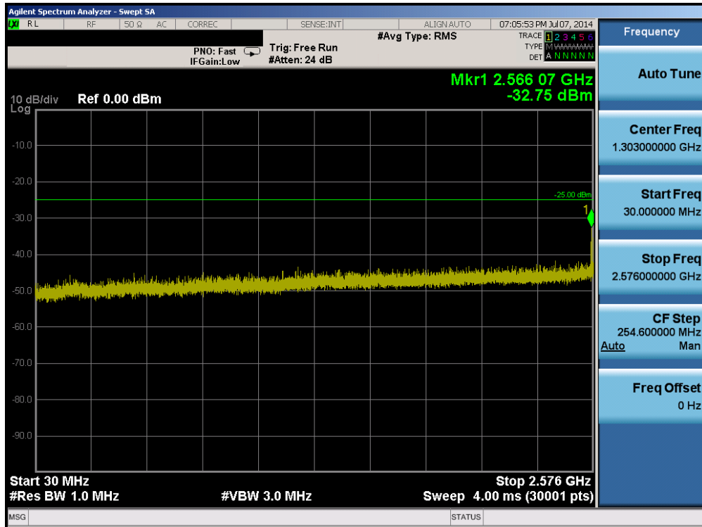
Plot 6-45. Conducted Spurious Plot (Band 41 – 5.0MHz QPSK – RB Size 25, RB Offset 0 – Mid Channel)
