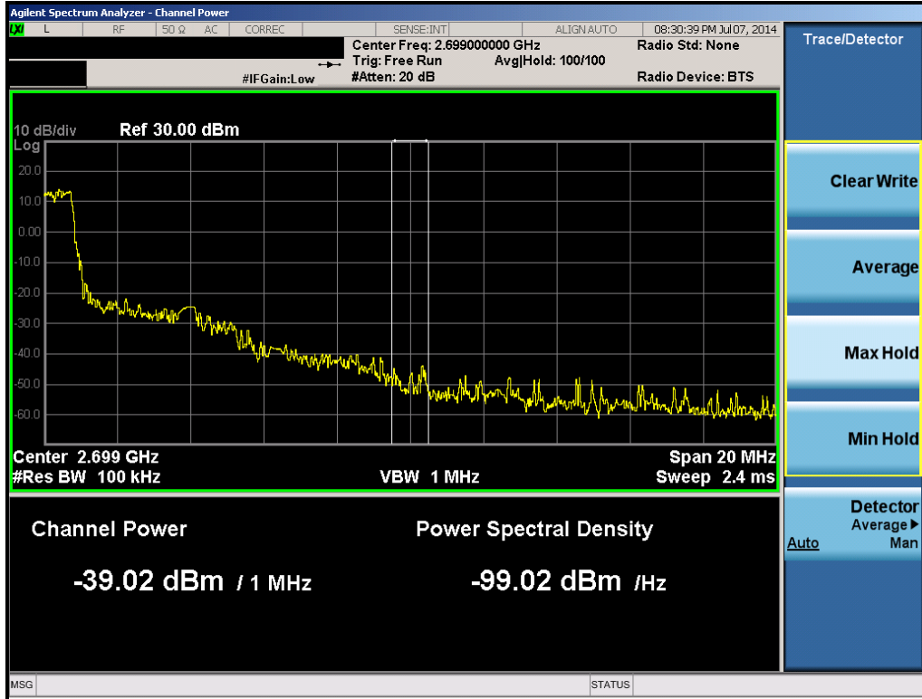
Plot 6-78. 1MHz Integration (Band 41 – 5.0MHz QPSK – RB Size 25, RB Offset 0 – High Channel)
