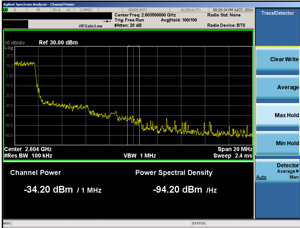
Plot 6-56. 1MHz Integration (Band 41 – 5.0MHz QPSK – RB Size 25, RB Offset 0 – Mid Channel)
