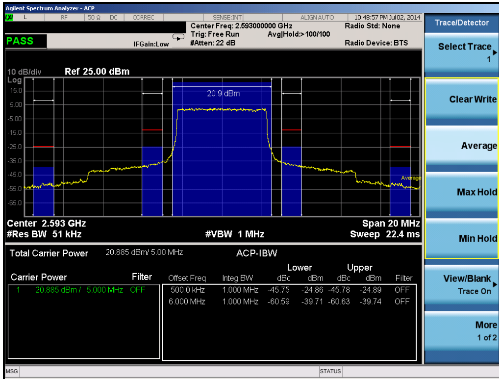
Plot 6-95. Mid ACP Plot (Band 41 – 5.0MHz QPSK – RB Size 25)
