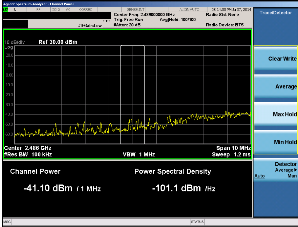
Plot 6-30. 1MHz Integration (Band 41 – 5.0MHz QPSK – RB Size 25, RB Offset 0 – Low Channel)
