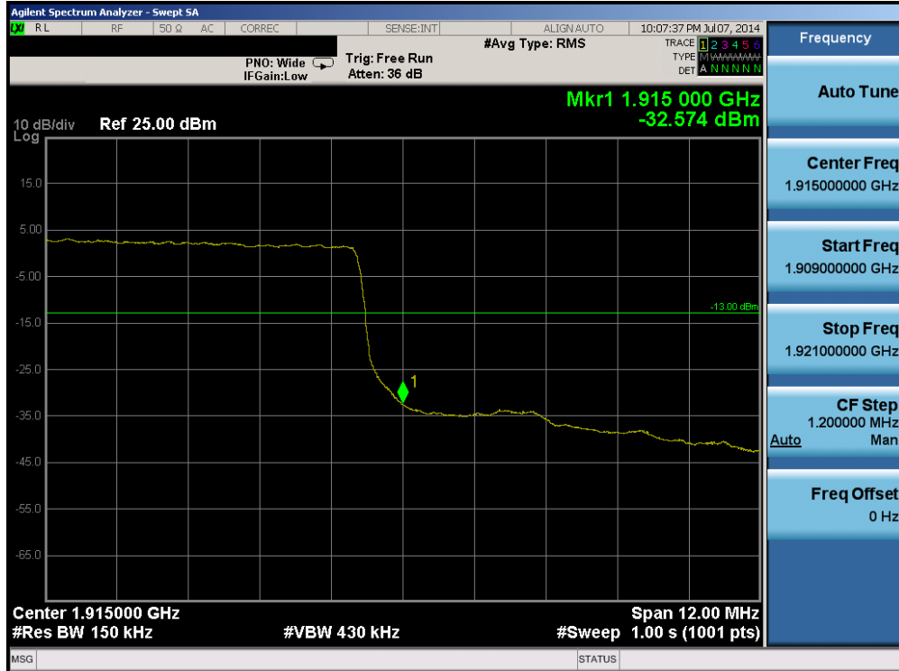
Plot 6-88. Upper Band Edge Plot (Band 25 – 15.0MHz QPSK – RB Size 75)
