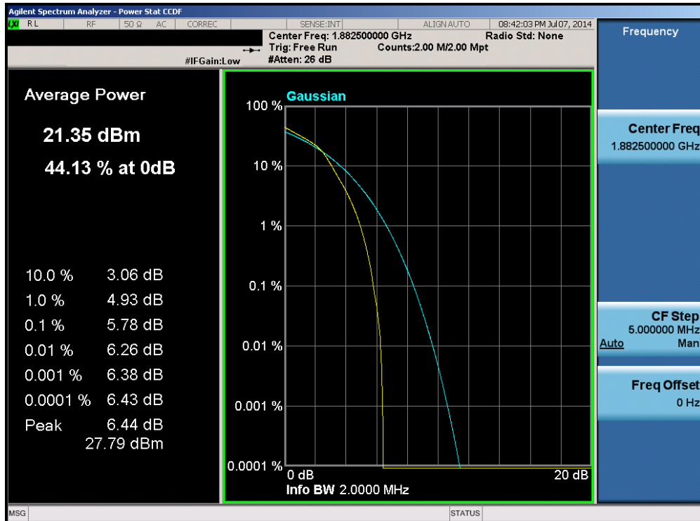
Plot 6-98. PAR Plot (Band 25 – 1.4MHz 16-QAM – RB Size 6)
