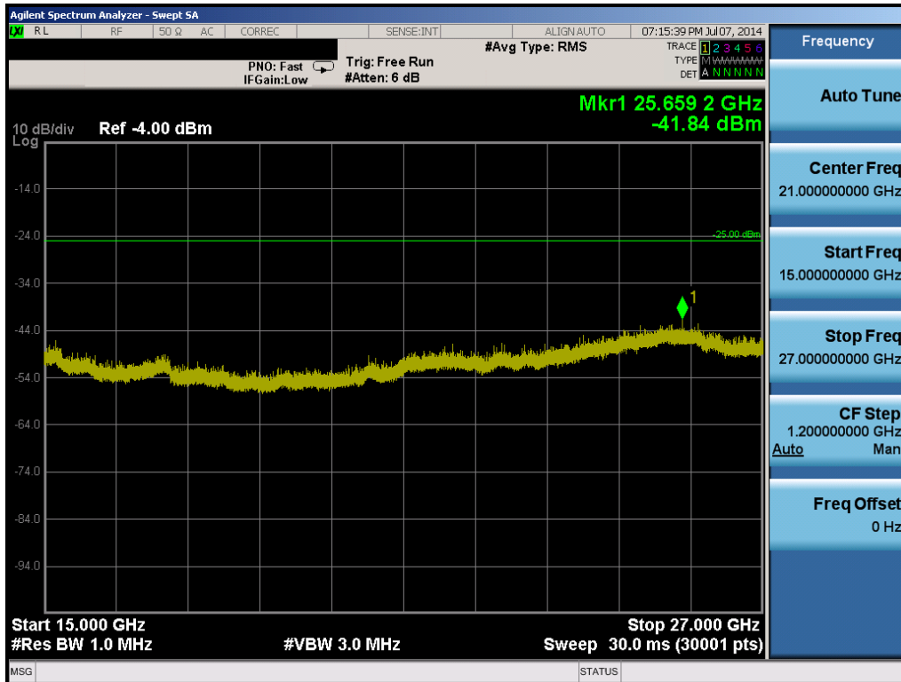
Plot 6-81. Conducted Spurious Plot (Band 41 – 5.0MHz QPSK – RB Size 25, RB Offset 0 – High Channel)
