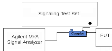
Figure 6-2. Test Instrument & Measurement Setup
