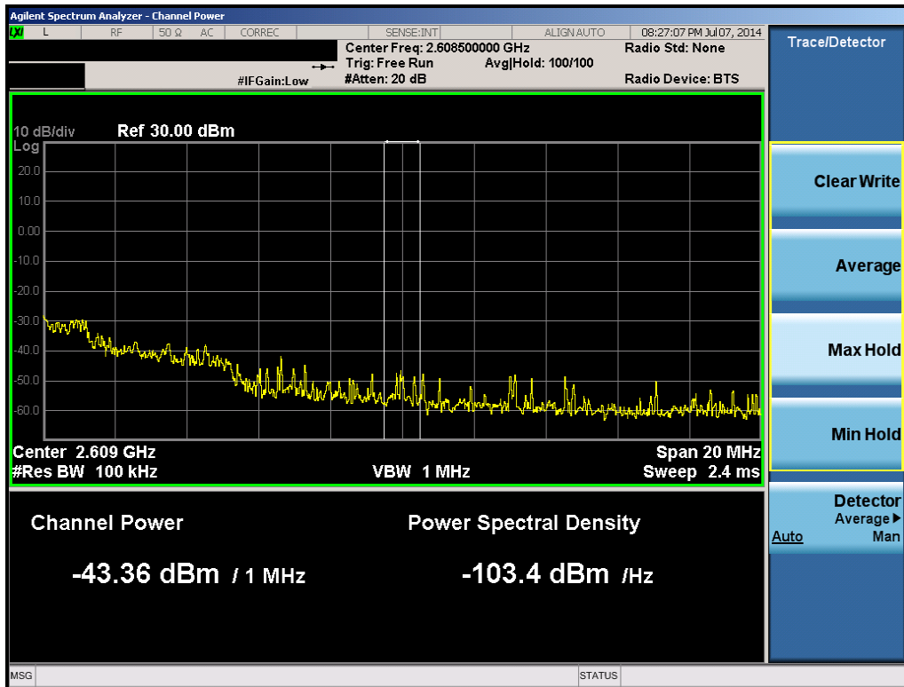
Plot 6-61. 1MHz Integration (Band 41 – 5.0MHz QPSK – RB Size 25, RB Offset 0 – Mid Channel)
