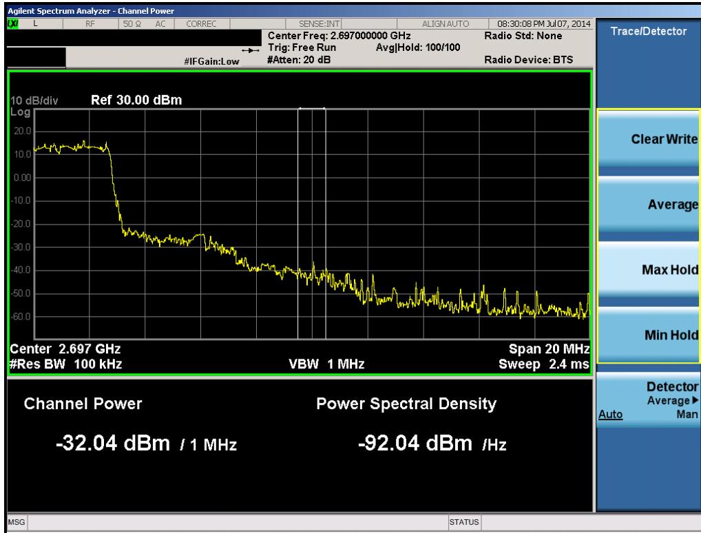
Plot 6-76. 1MHz Integration (Band 41 – 5.0MHz QPSK – RB Size 25, RB Offset 0 – High Channel)
