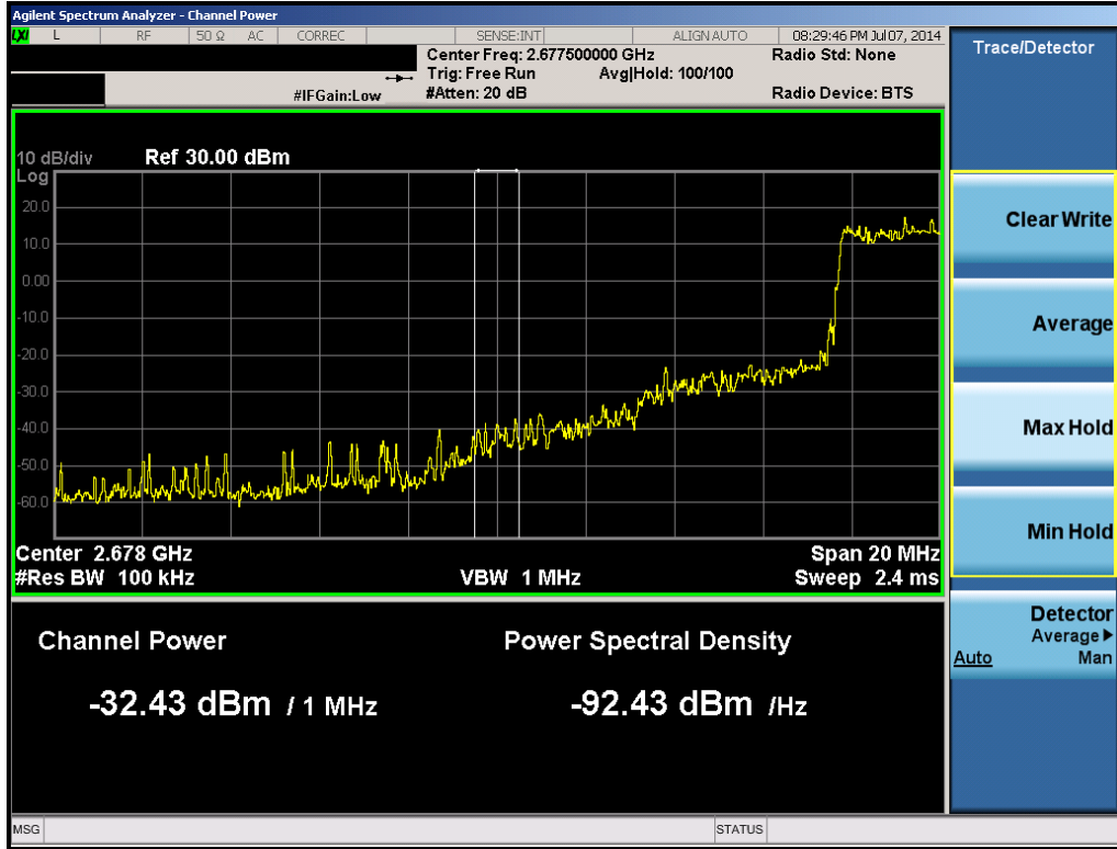
Plot 6-74. 1MHz Integration (Band 41 – 5.0MHz QPSK – RB Size 25, RB Offset 0 – High Channel)
