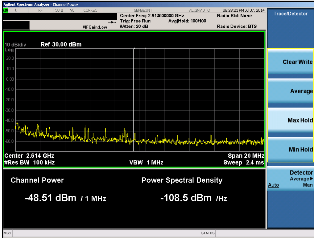
Plot 6-66. 1MHz Integration (Band 41 – 5.0MHz QPSK – RB Size 25, RB Offset 0 – Mid Channel)
