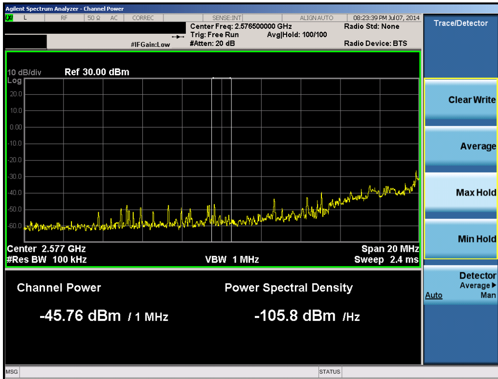
Plot 6-47. 1MHz Integration (Band 41 – 5.0MHz QPSK – RB Size 25, RB Offset 0 – Mid Channel)
