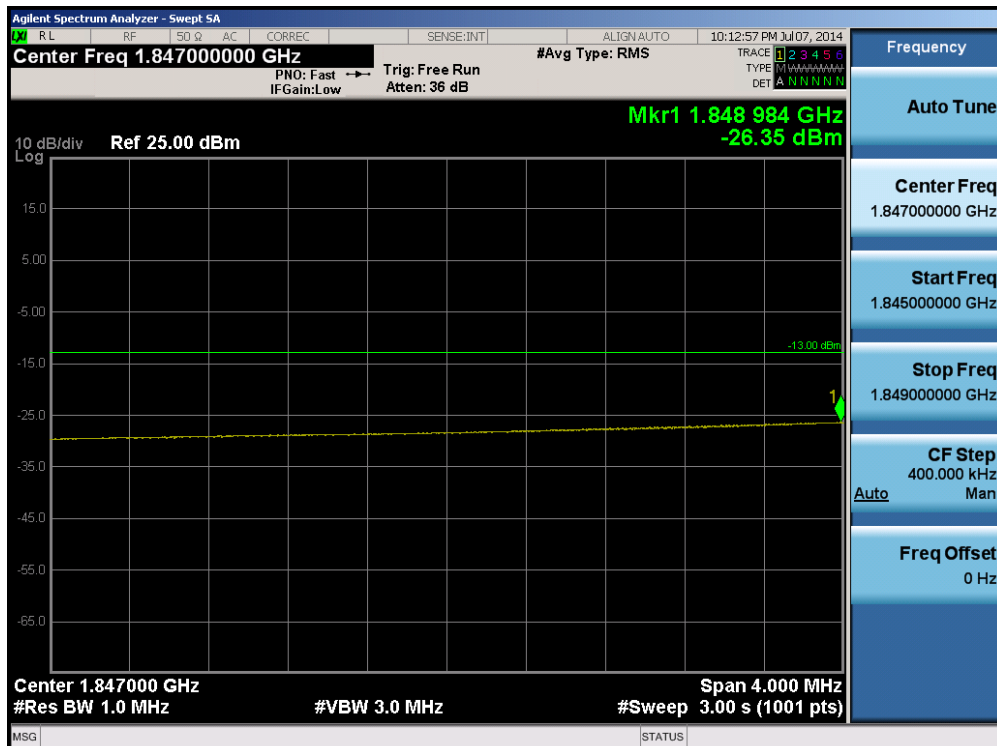
Plot 6-91. Lower Extended Band Edge Plot (Band 25 – 20.0MHz QPSK – RB Size 100)
