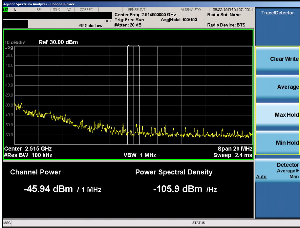
Plot 6-40. 1MHz Integration (Band 41 – 5.0MHz QPSK – RB Size 25, RB Offset 0 – Low Channel)
