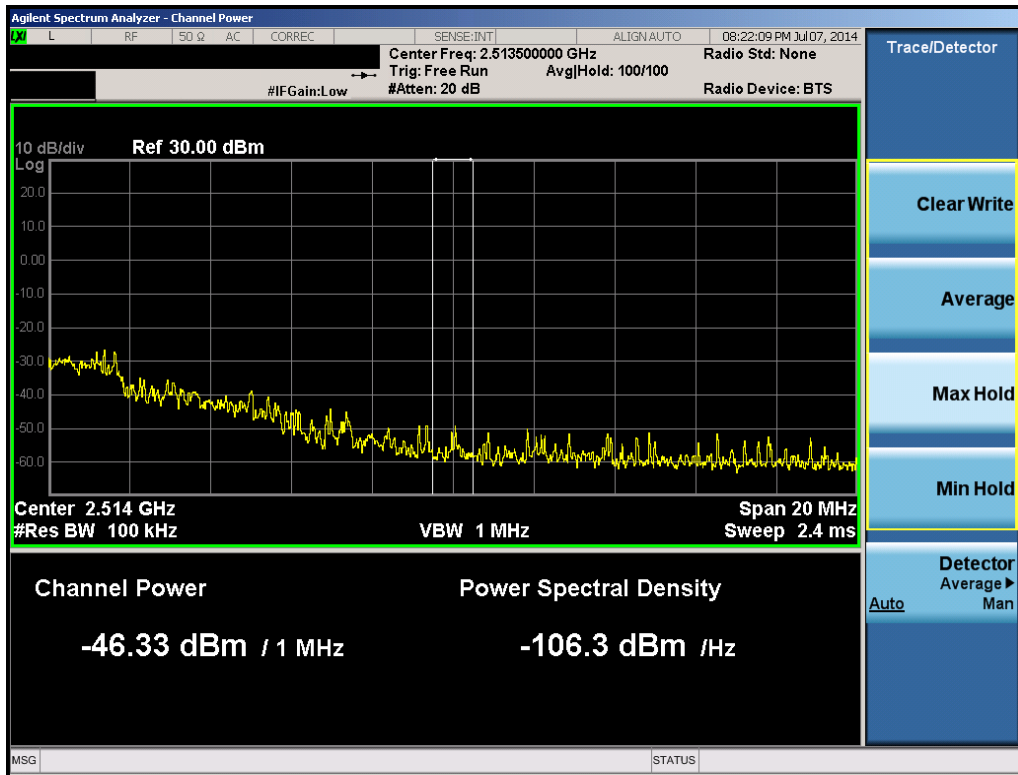
Plot 6-39. 1MHz Integration (Band 41 – 5.0MHz QPSK – RB Size 25, RB Offset 0 – Low Channel)
