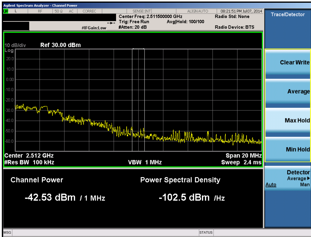
Plot 6-37. 1MHz Integration (Band 41 – 5.0MHz QPSK – RB Size 25, RB Offset 0 – Low Channel)
