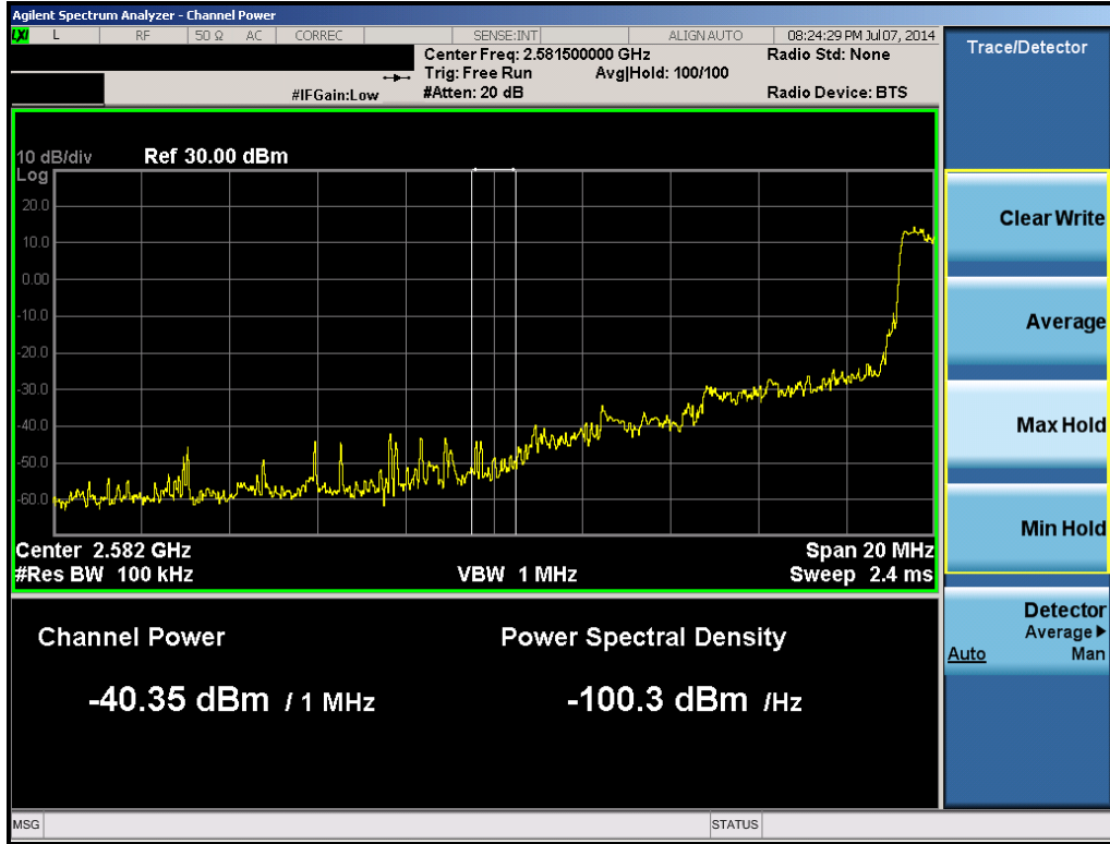
Plot 6-52. 1MHz Integration (Band 41 – 5.0MHz QPSK – RB Size 25, RB Offset 0 – Mid Channel)
