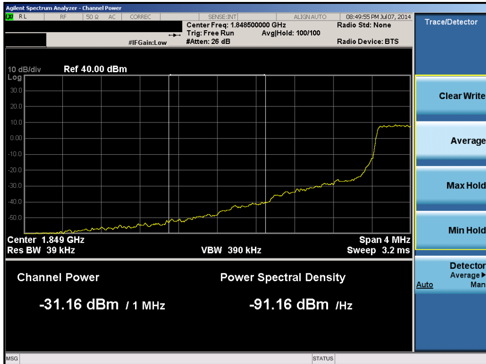
Plot 6-83. Lower Extended Band Edge Plot (Band 25 – 1.4MHz QPSK – RB Size 6)
