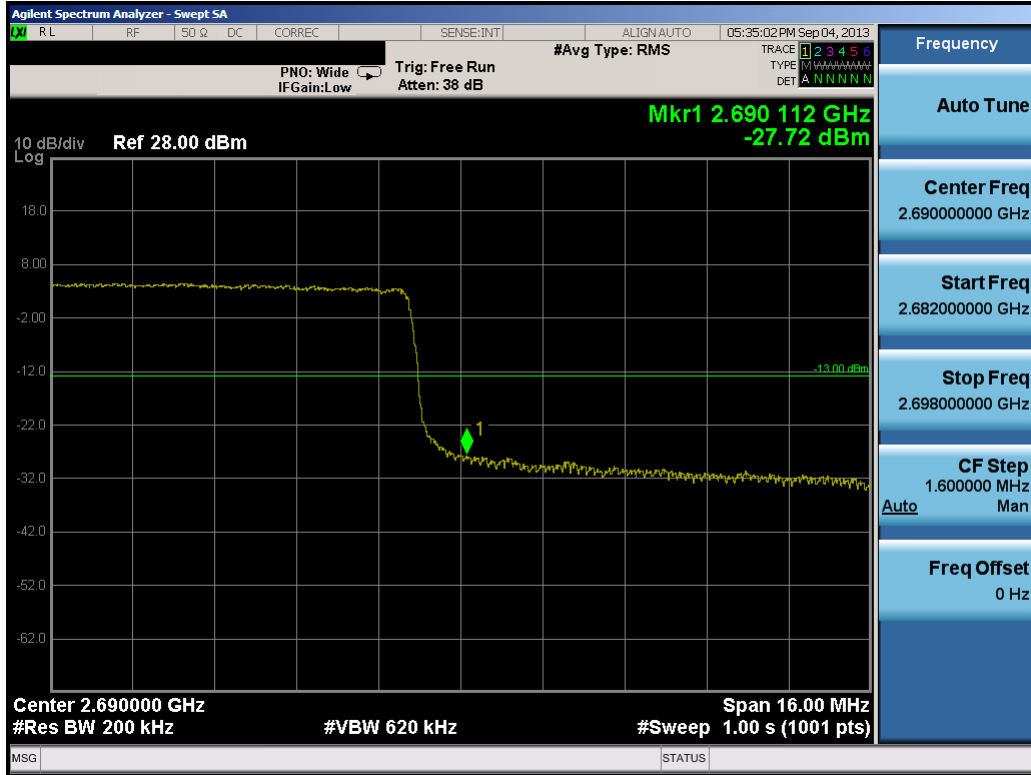
Plot 9-28. Upper Band Edge Plot (20.0MHz QPSK – RB Size 100)
