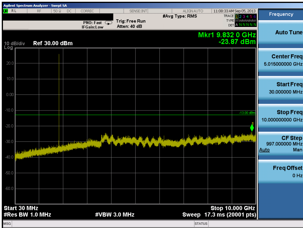
Plot 8-13. Conducted Spurious Plot (5.0MHz QPSK – RB Size 1, RB Offset 0 – Low Channel)
