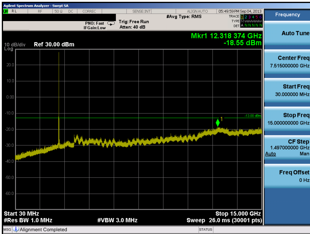
Plot 9-17. Conducted Spurious Plot (15.0MHz QPSK – RB Size 1, RB Offset 0 – High Channel)
