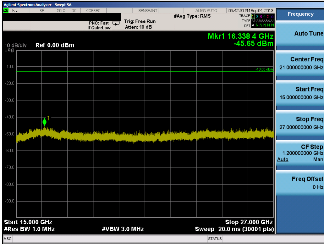
Plot 9-16. Conducted Spurious Plot (15.0MHz QPSK – RB Size 1, RB Offset 0 – Mid Channel)
