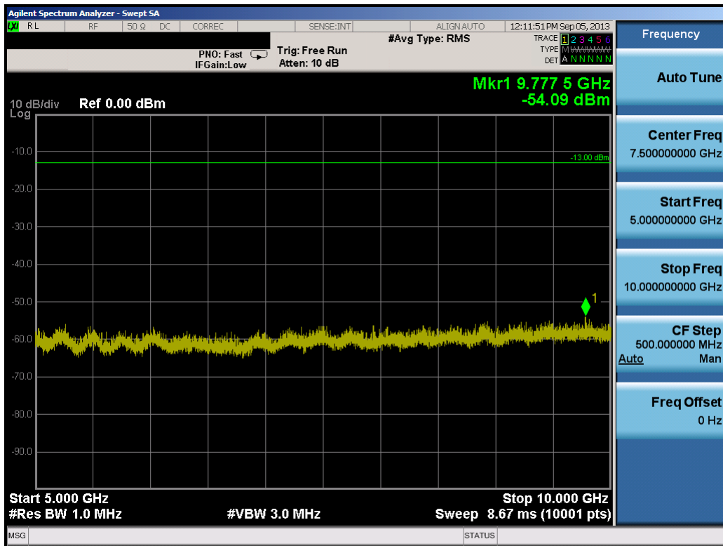
Plot 7-15. Conducted Spurious Plot (5.0MHz QPSK – RB Size 1, RB Offset 0 – Mid Channel)
