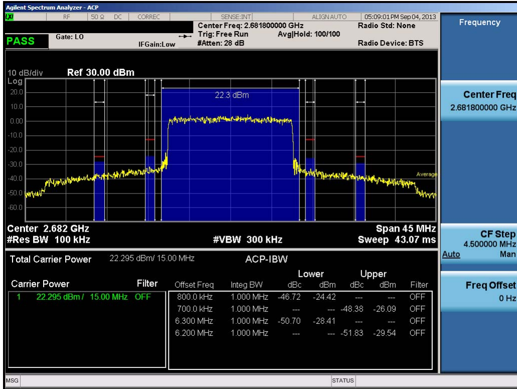
Plot 9-24. ACP Plot (15.0MHz QPSK – RB Size 75 – High Channel)
