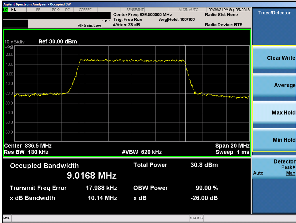
Plot 7-20. Occupied Bandwidth Plot (10.0MHz QPSK – RB Size 50)
