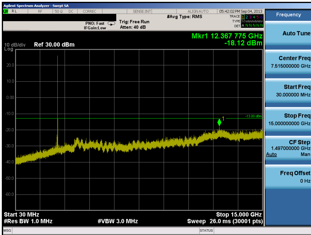
Plot 9-15. Conducted Spurious Plot (15.0MHz QPSK – RB Size 1, RB Offset 0 – Mid Channel)
