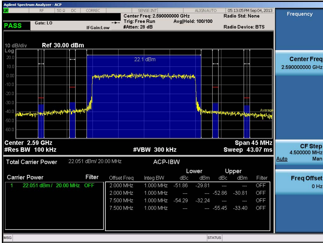
Plot 9-32. ACP Plot (20.0MHz QPSK – RB Size 100 – Mid Channel)
