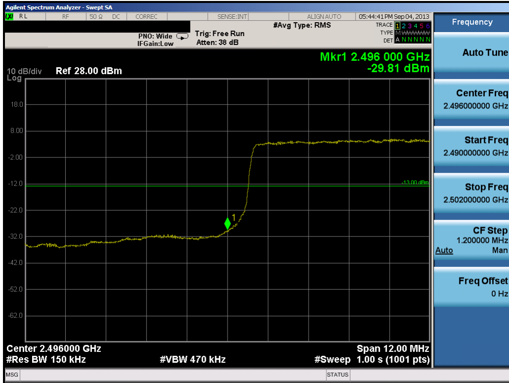
Plot 9-10. Lower Band Edge Plot (15.0MHz QPSK – RB Size 75)
