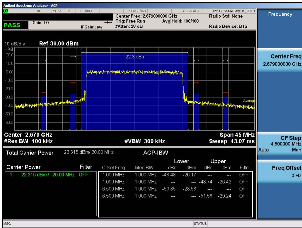
Plot 9-33. ACP Plot (20.0MHz QPSK – RB Size 100 – High Channel)
