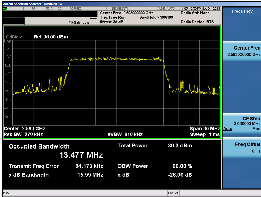
Plot 9-12. Occupied Bandwidth Plot (15.0MHz 16-QAM – RB Size 75)
