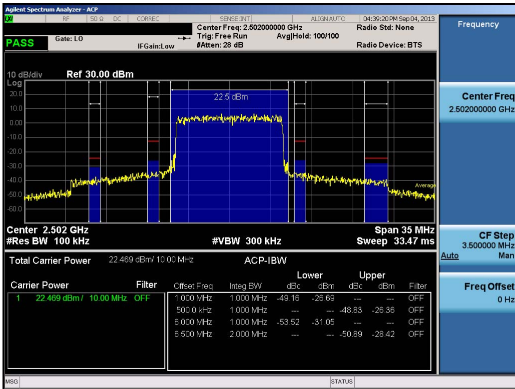
Plot 9-7. ACP Plot (10.0MHz QPSK – RB Size 50 – Low Chanel)
