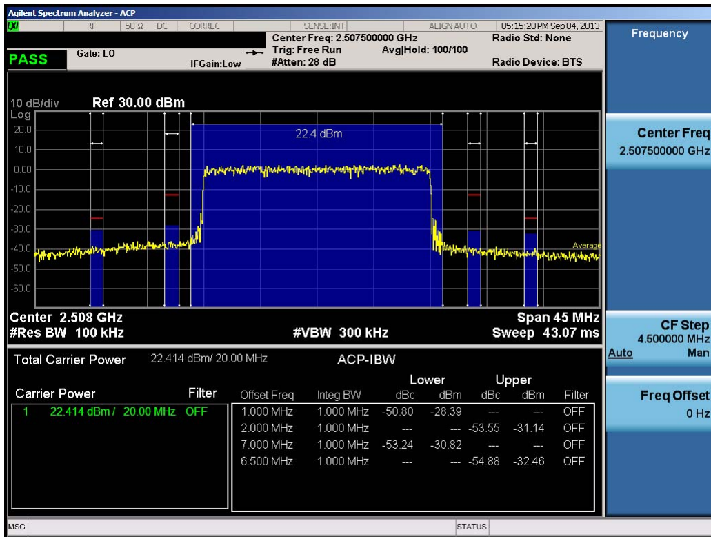
Plot 9-31. ACP Plot (20.0MHz QPSK – RB Size 100 – Low Chanel)
