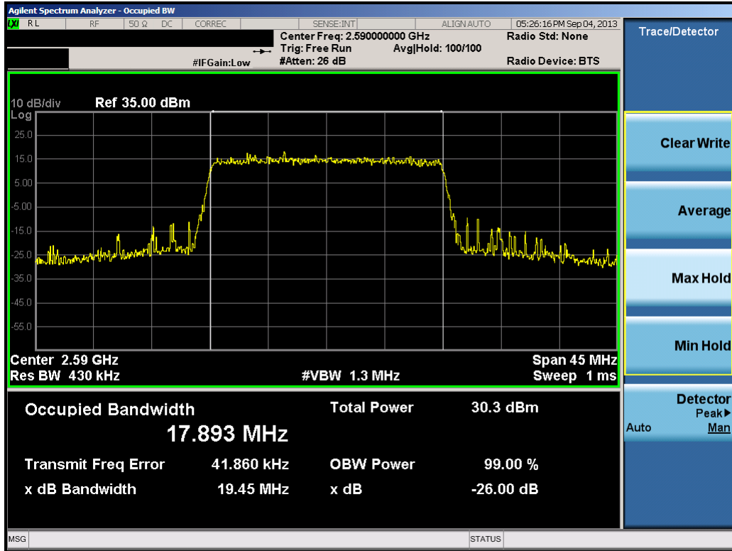
Plot 9-26. Occupied Bandwidth Plot (20.0MHz QPSK – RB Size 100)
