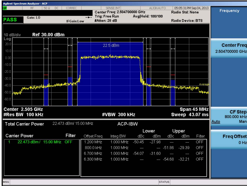
Plot 9-22. ACP Plot (15.0MHz QPSK – RB Size 75 – Low Channel)
