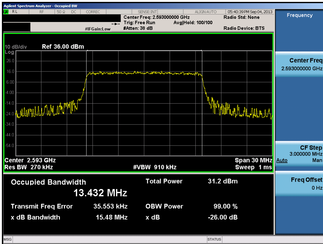
Plot 9-11. Occupied Bandwidth Plot (15.0MHz QPSK – RB Size 75)
