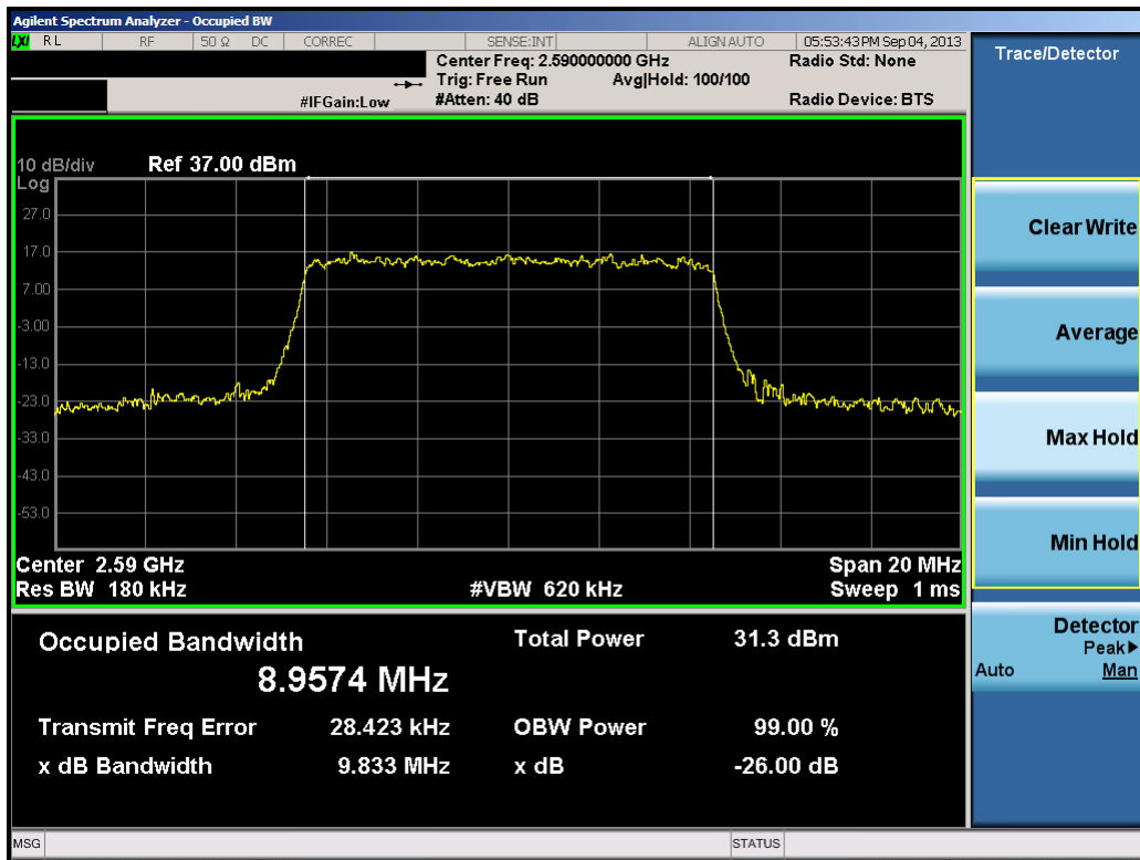
Plot 9-3. Occupied Bandwidth Plot (10.0MHz 16-QAM – RB Size 50)
