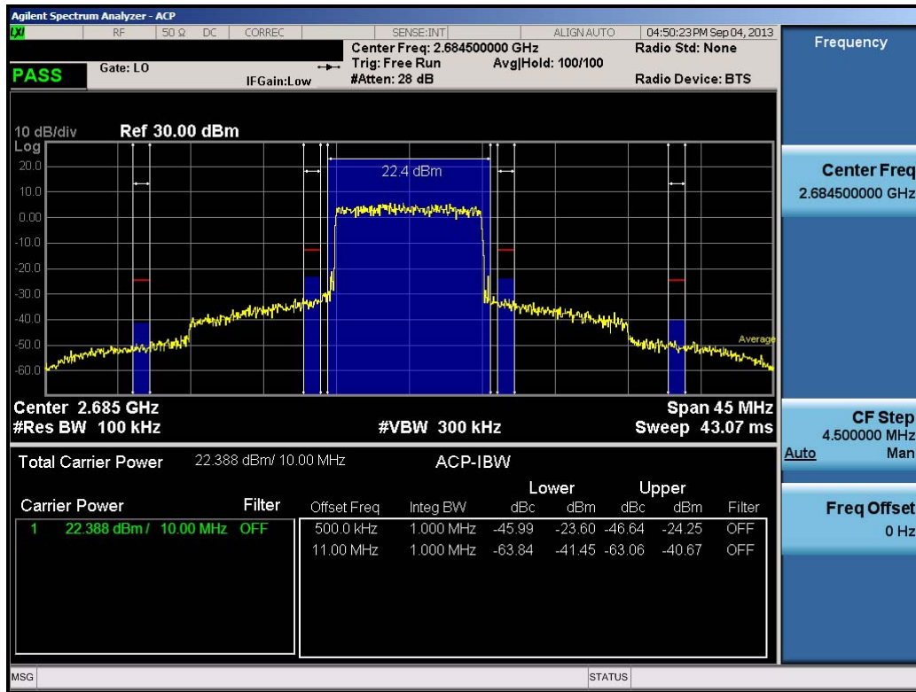
Plot 9-9. ACP Plot (10.0MHz QPSK – RB Size 50 – High Chanel)
