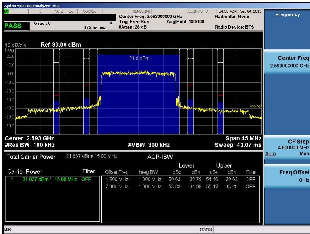
Plot 9-23. ACP Plot (15.0MHz QPSK – RB Size 75 – Mid Channel)
