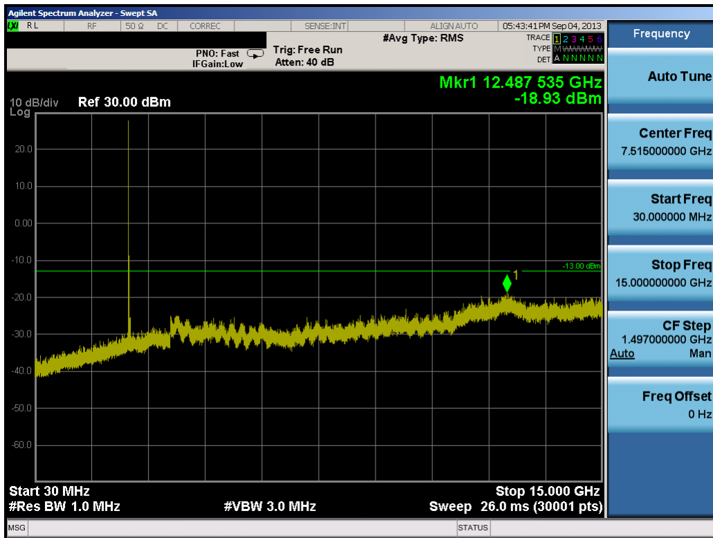
Plot 9-13. Conducted Spurious Plot (15.0MHz QPSK – RB Size 1, RB Offset 0 – Low Channel)
