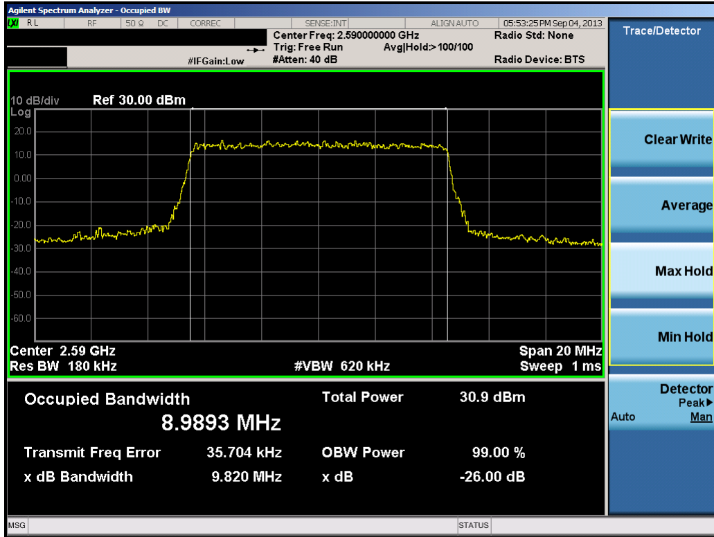
Plot 9-2. Occupied Bandwidth Plot (10.0MHz QPSK – RB Size 50)
