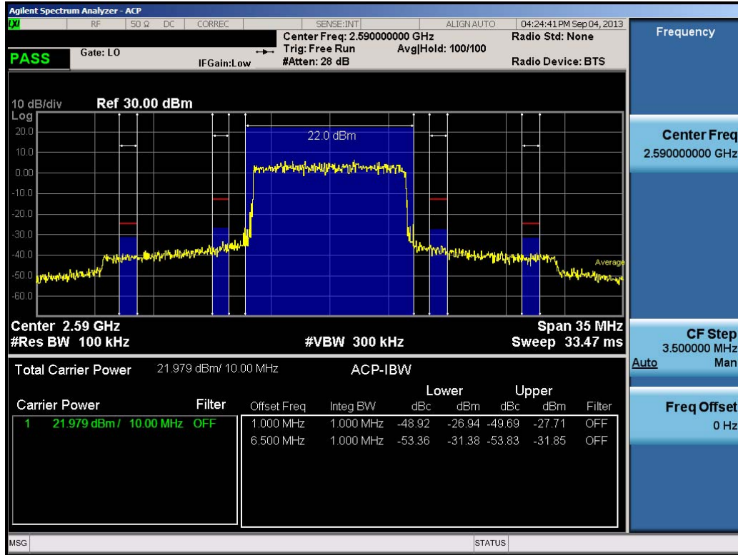
Plot 9-8. ACP Plot (10.0MHz QPSK – RB Size 50 – Mid Chanel)
