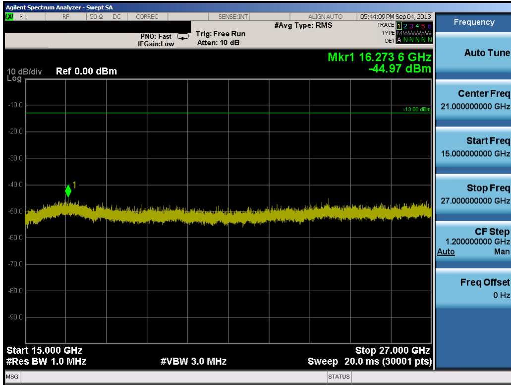
Plot 9-14. Conducted Spurious Plot (15.0MHz QPSK – RB Size 1, RB Offset 0 – Low Channel)
