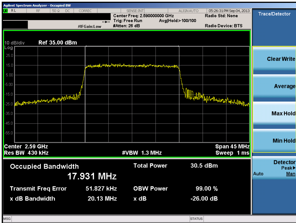
Plot 9-27. Occupied Bandwidth Plot (20.0MHz 16-QAM – RB Size 100)
