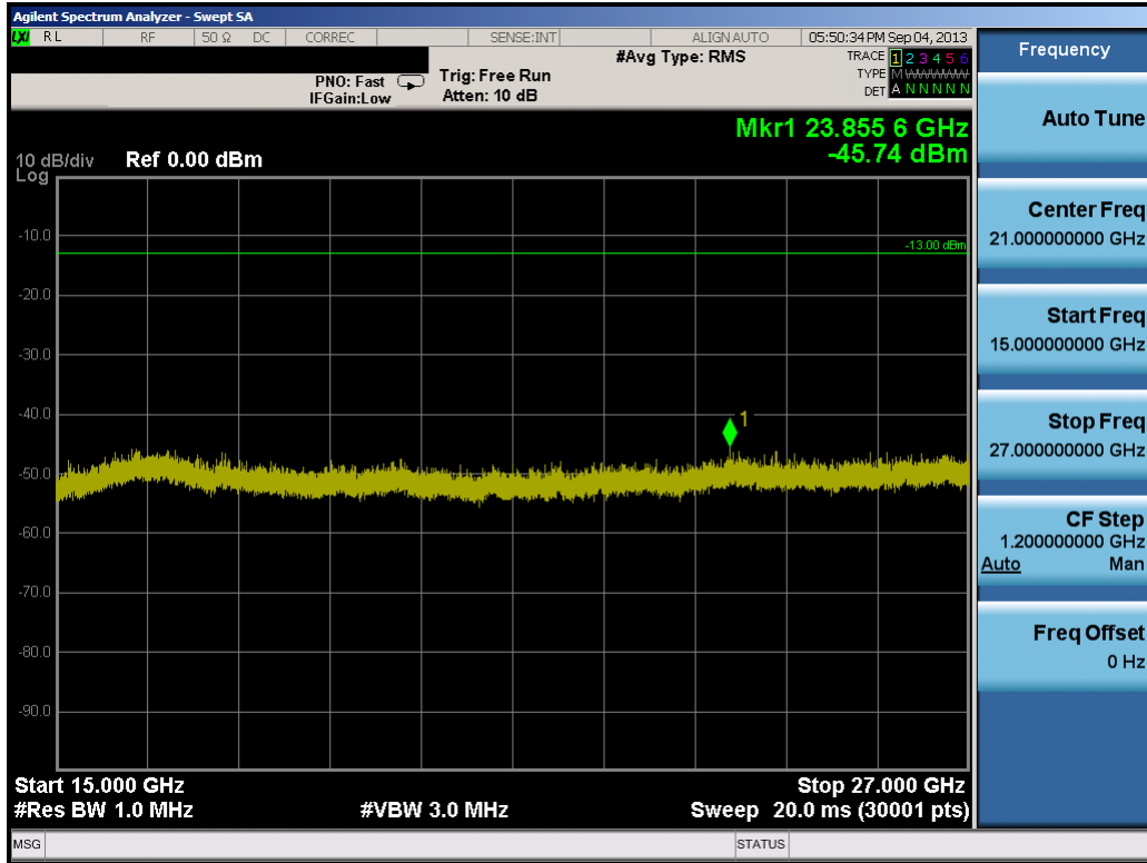
Plot 9-18. Conducted Spurious Plot (15.0MHz QPSK – RB Size 1, RB Offset 0 – High Channel)
