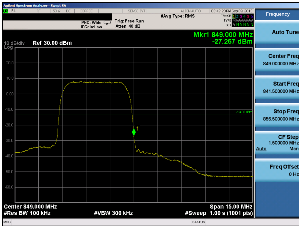
Plot 6-61. Band Edge Plot (Cellular WCDMA Mode – Ch. 4233)
