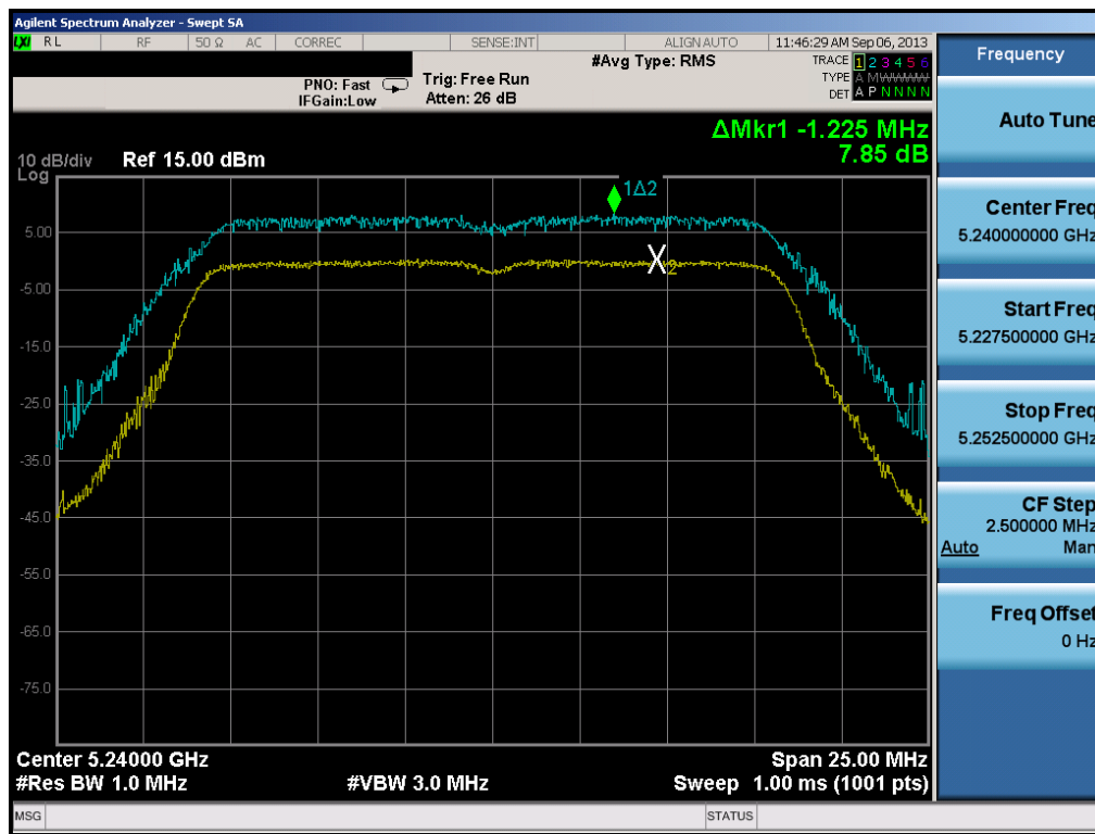
Plot 6-59. Peak Excursion Ratio Plot (802.11a)
