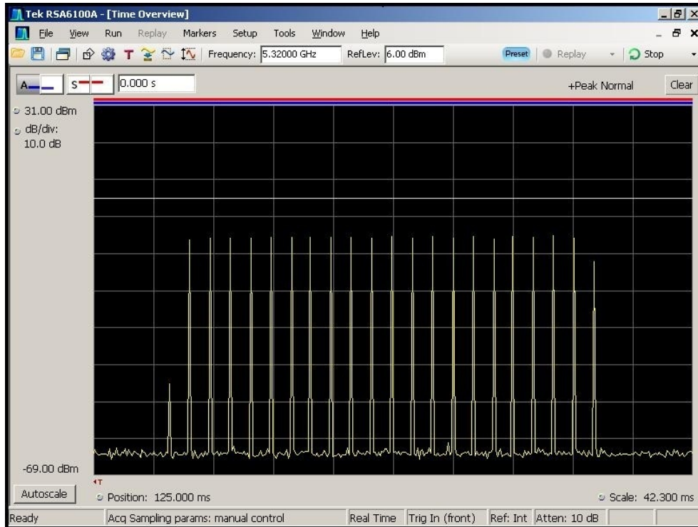
Figure 4-1. Type 1 Radar Pulse
