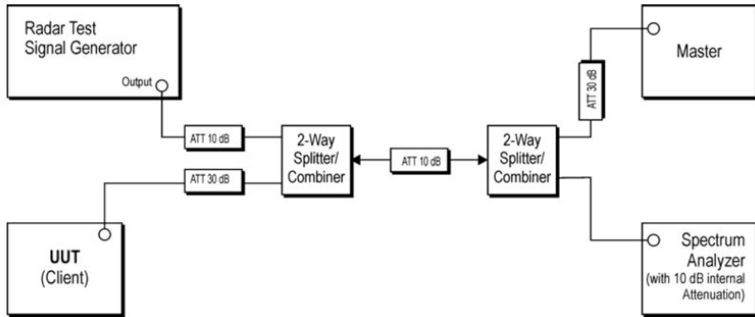
Figure 0-1. Conducted Test Setup for DFS
