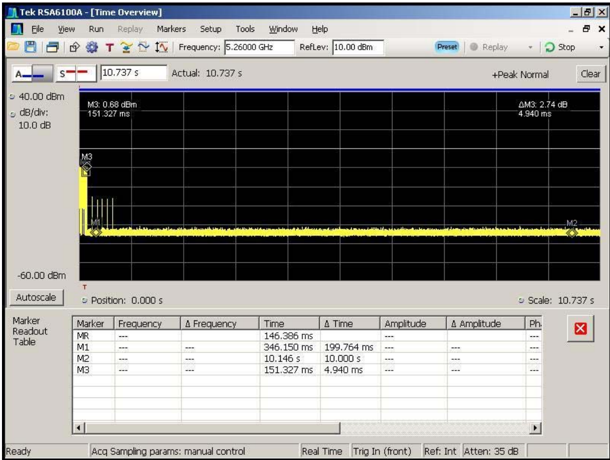
Figure 4-5. Channel Move Time (< 10sec)
