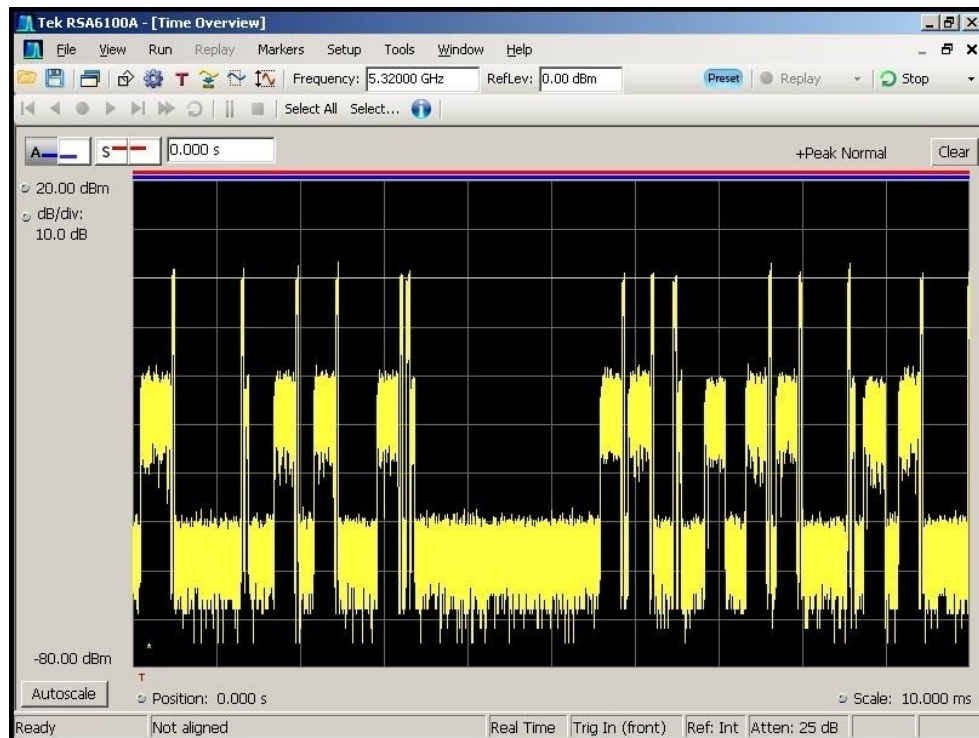
Figure 4-2. Time Display WLAN Channel Traffic (Streaming Video)
