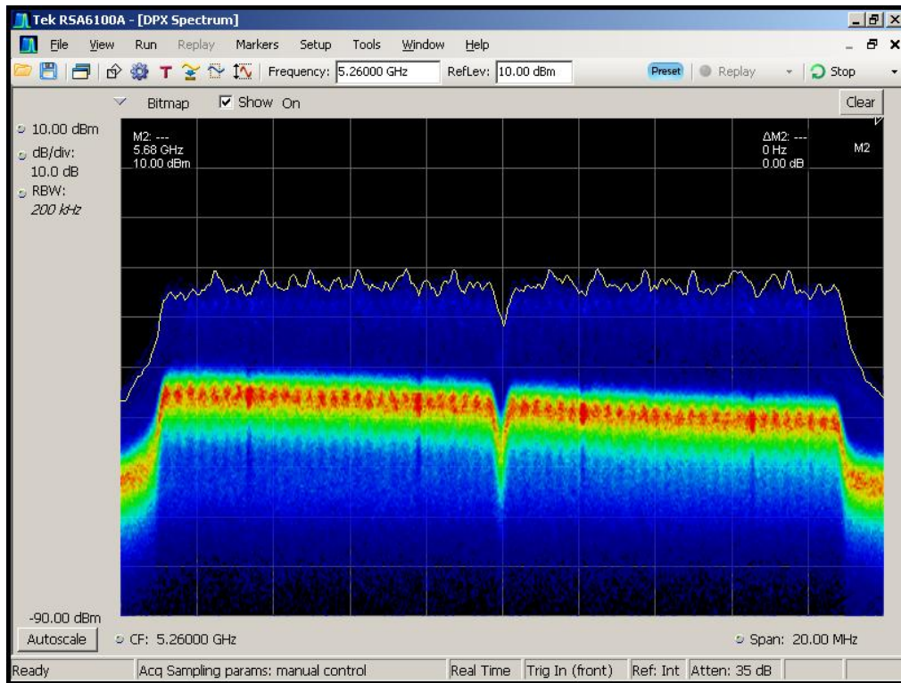
Figure 4-4. Real-Time Spectrum Display, WLAN Traffic (Streaming Video)
