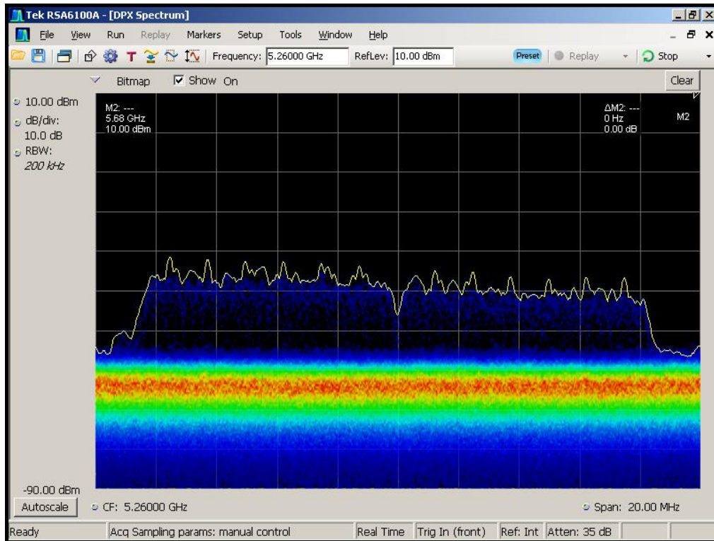
Figure 4-3. Real-Time Spectrum Display, No WLAN Traffic
