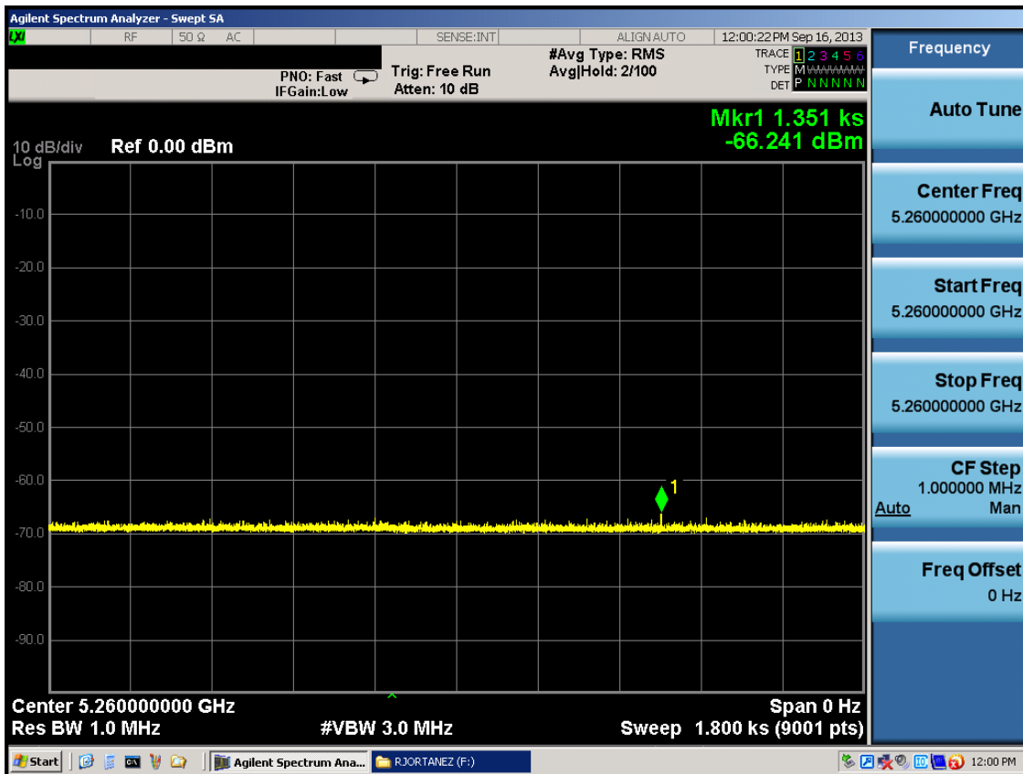
Figure 4-6 Non-occupancy Period - Monitoring live spectrum - Elapse time 30 minutes
