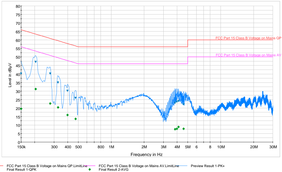
Plot 7-2. Line Conducted Plot (LN)
