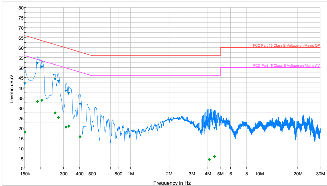
Plot 7-1. Line Conducted Plot (L1)
