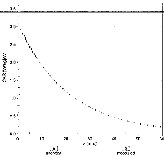
f = 750 MHz, WGLS R9 (H_convF)
