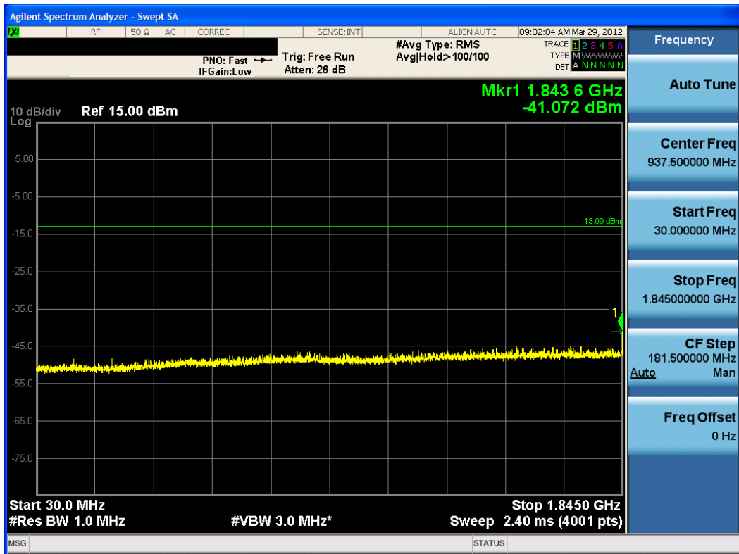
Plot 8-20. Conducted Spurious Plot (PCS EvDO Mode – Ch. 1175)
