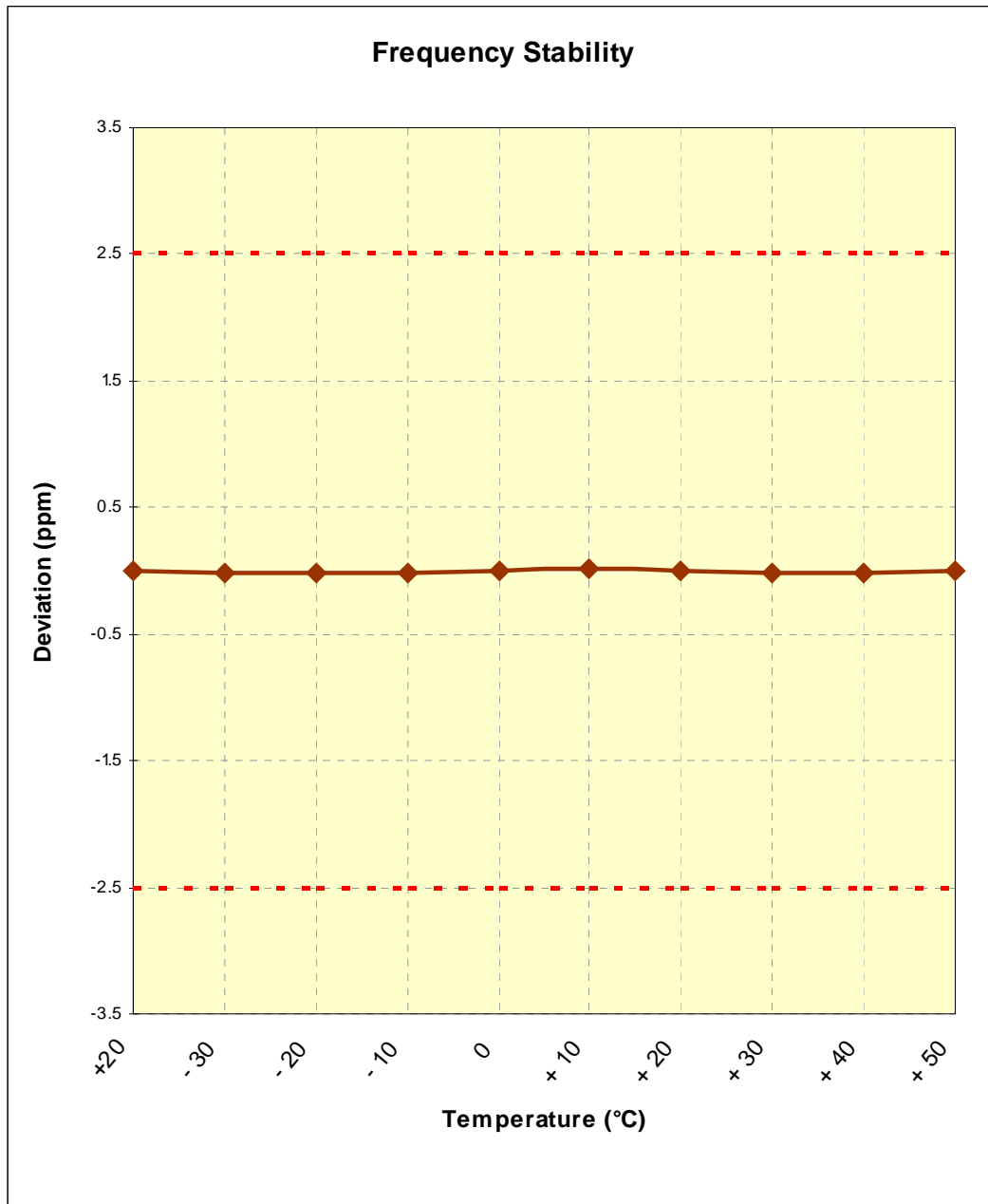
Figure 6-4. Frequency Stability Graph (PCS EvDO Mode – Ch. 600)
