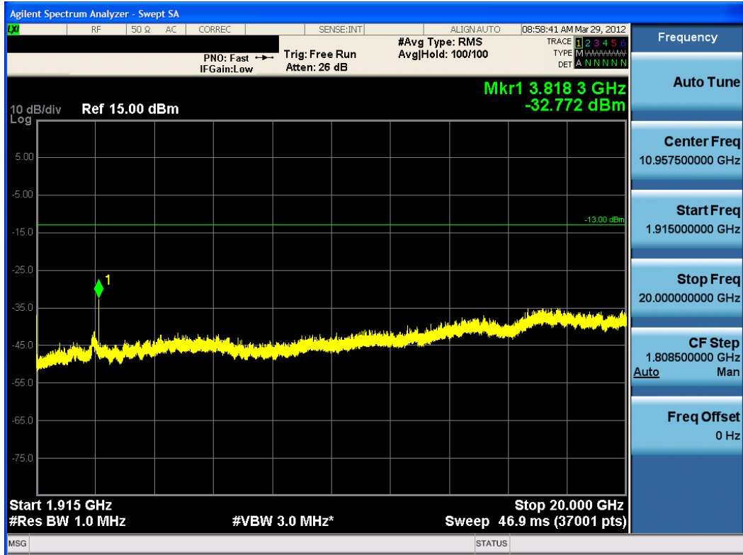
Plot 8-21. Conducted Spurious Plot (PCS EvDO Mode – Ch. 1175)
