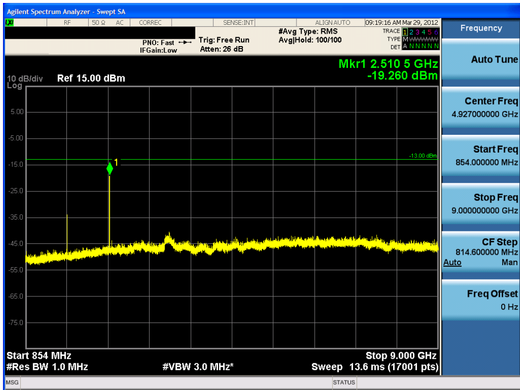
Plot 8-6. Conducted Spurious Plot (Cellular EvDO Mode – Ch. 384)
