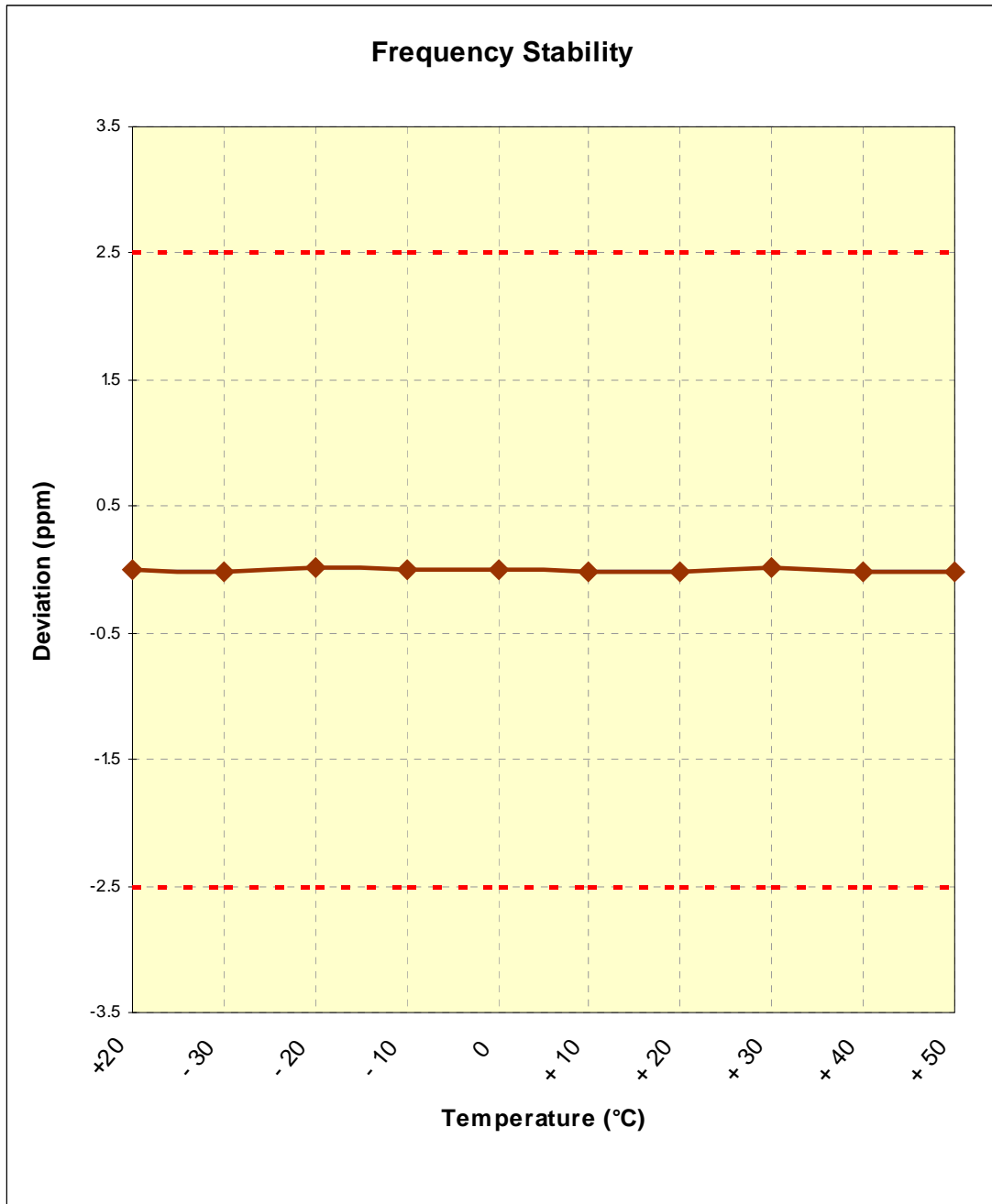
Figure 6-2. Frequency Stability Graph (Cellular EvDO Mode – Ch. 384)
