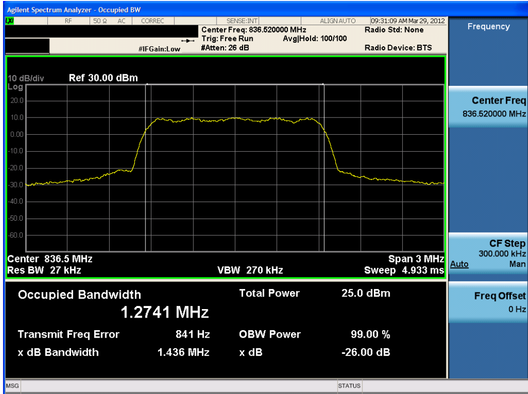
Plot 8-7. Occupied Bandwidth Plot (Cellular EvDO Mode – Ch. 384)
