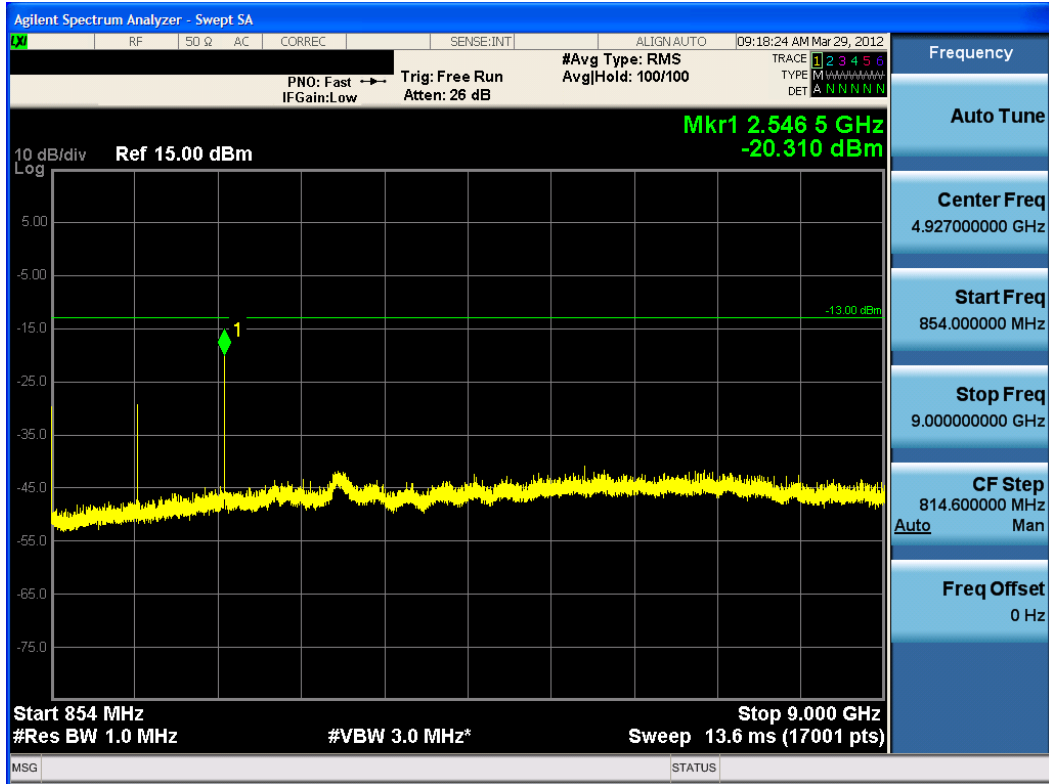
Plot 8-9. Conducted Spurious Plot (Cellular EvDO Mode – Ch. 777)
