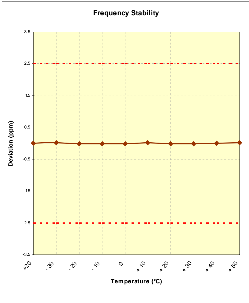
Figure 6-1. Frequency Stability Graph (Cellular 1x CDMA Mode – Ch. 384)
