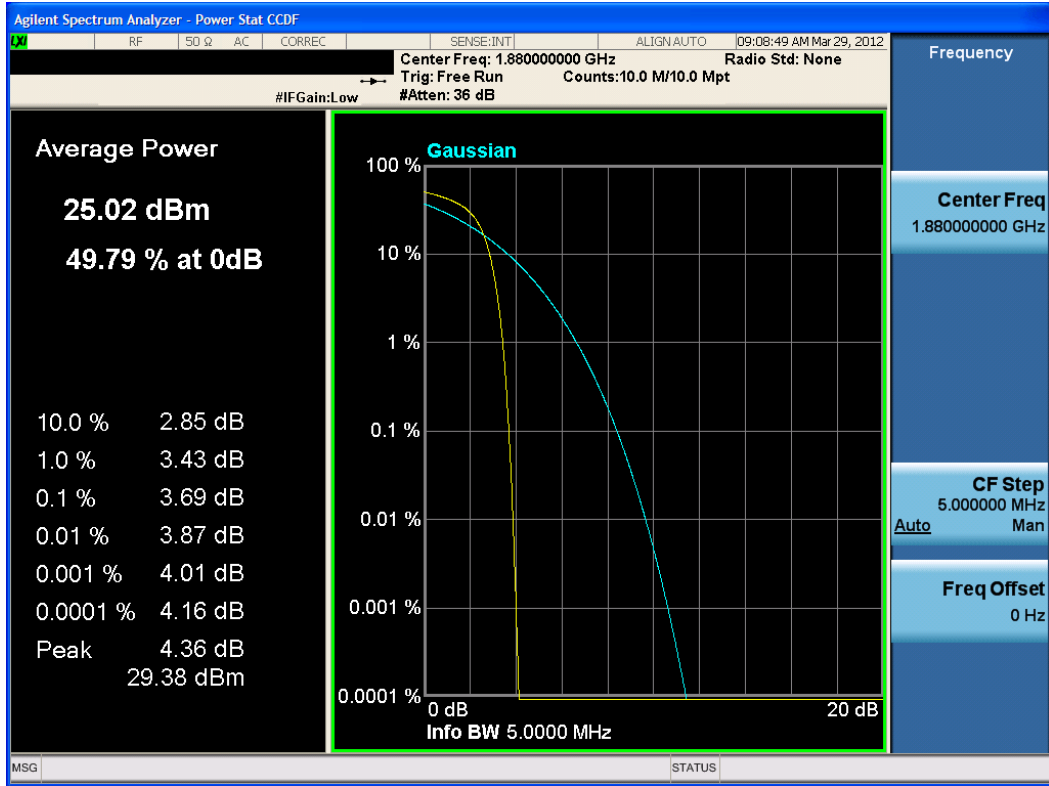
Plot 8-19. Peak-Average Ratio Plot (PCS EvDO Mode – Ch. 600)
