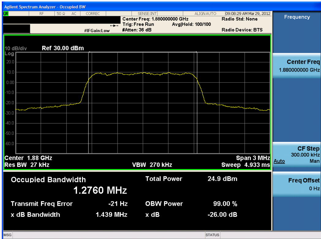
Plot 8-18. Occupied Bandwidth Plot (PCS EvDO Mode – Ch. 600)
