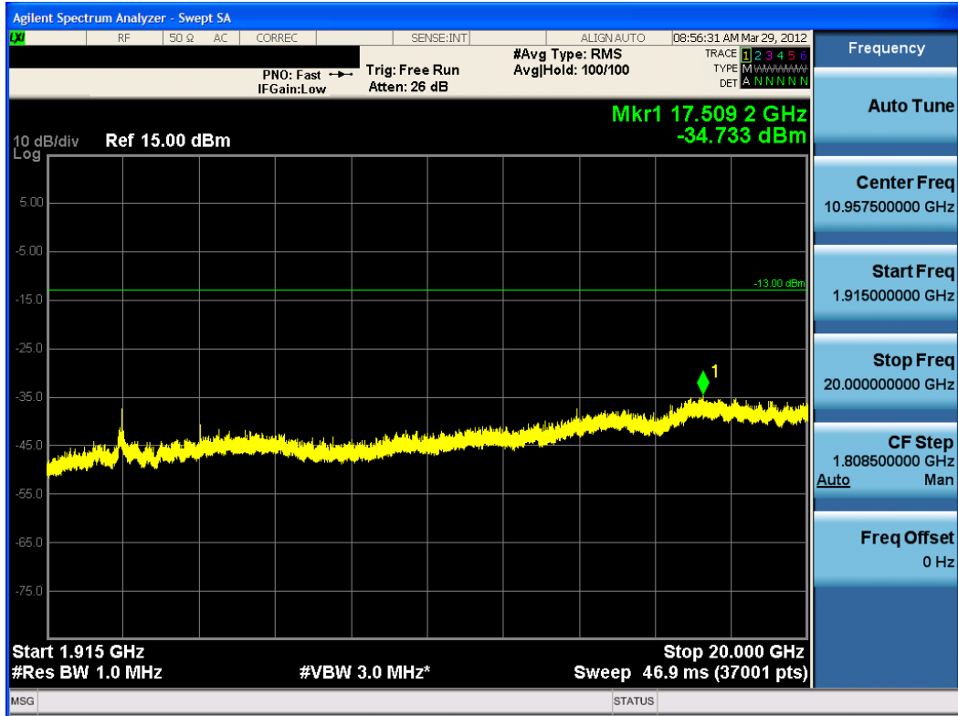
Plot 8-13. Conducted Spurious Plot (PCS EvDO Mode – Ch. 25)
