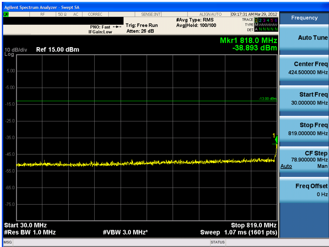
Plot 8-8. Conducted Spurious Plot (Cellular EvDO Mode – Ch. 777)
