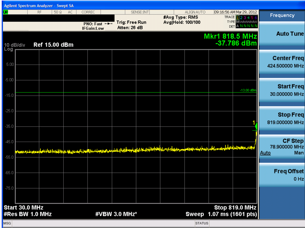
Plot 8-5. Conducted Spurious Plot (Cellular EvDO Mode – Ch. 384)
