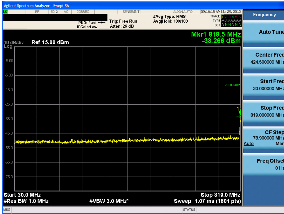
Plot 8-1. Conducted Spurious Plot (Cellular EvDO Mode – Ch. 1013)
