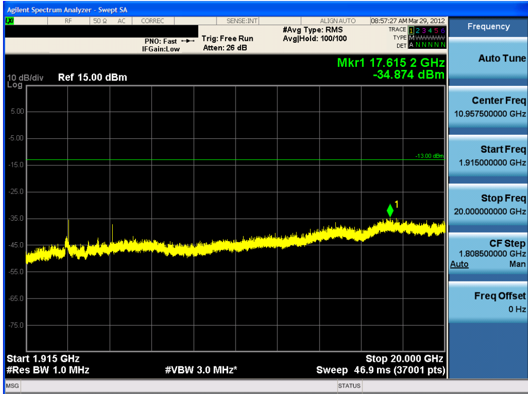
Plot 8-17. Conducted Spurious Plot (PCS EvDO Mode – Ch. 600)
