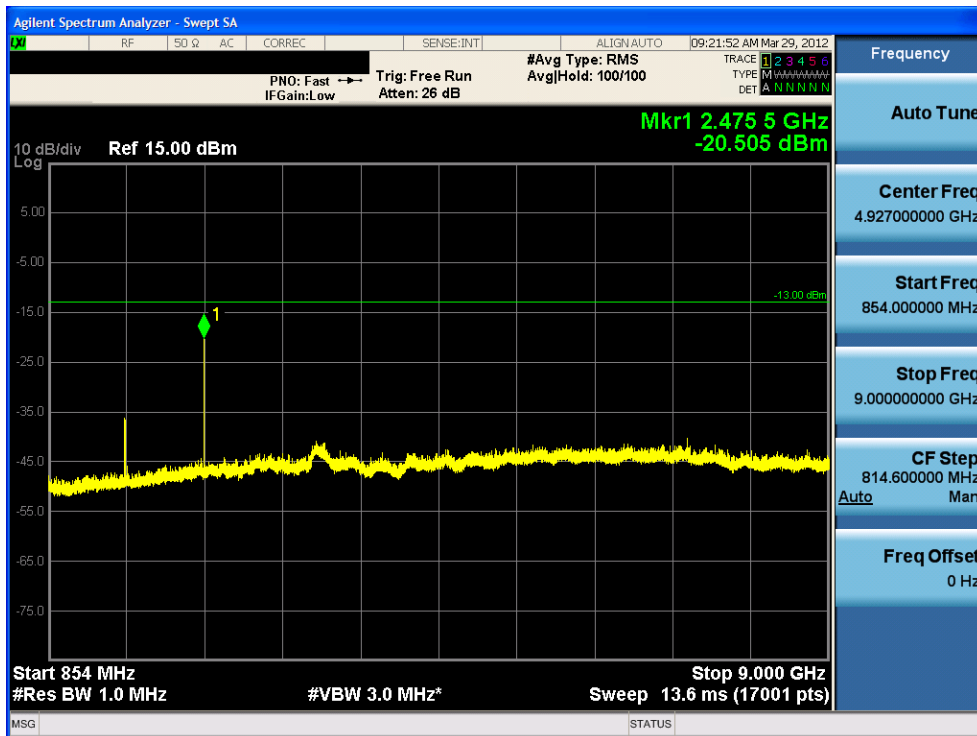
Plot 8-2. Conducted Spurious Plot (Cellular EvDO Mode – Ch. 1013)
