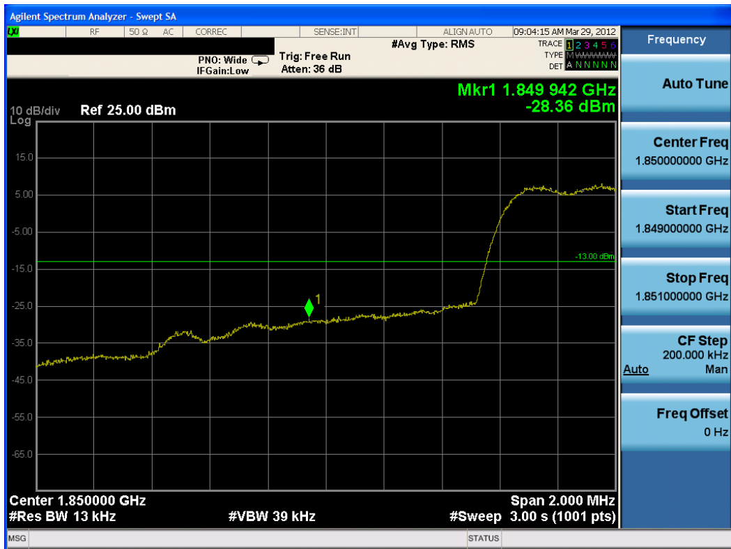
Plot 8-14. Band Edge Plot (PCS EvDO Mode – Ch. 25)
