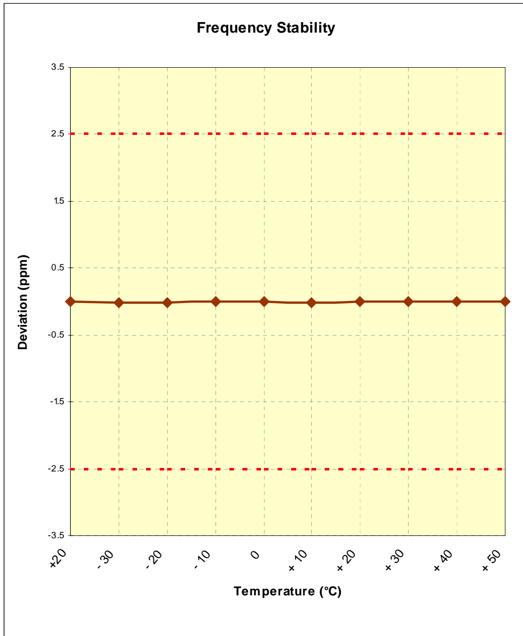
Figure 6-3. Frequency Stability Graph (PCS 1x CDMA Mode – Ch. 600)
