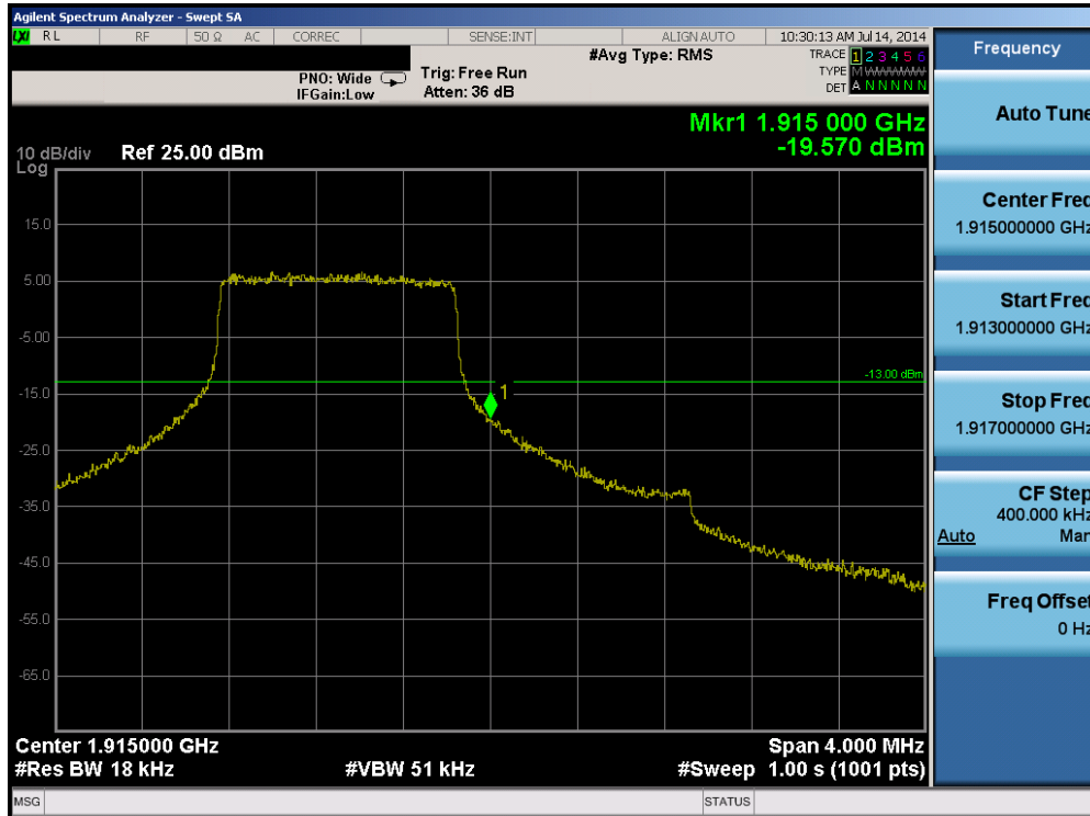
Plot 6-19. Upper Band Edge Plot (Band 25 – 1.4MHz QPSK – RB Size 6)
