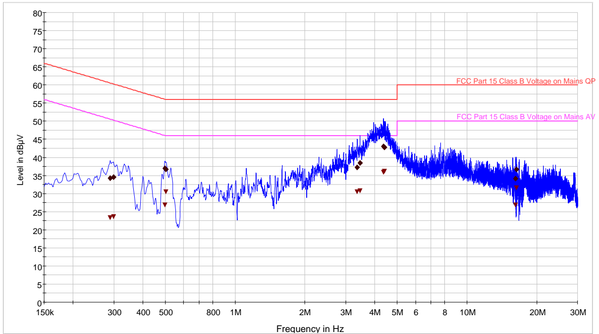
Plot 6-55. Line Conducted Plot with 802.11a (UNII Band 1)
