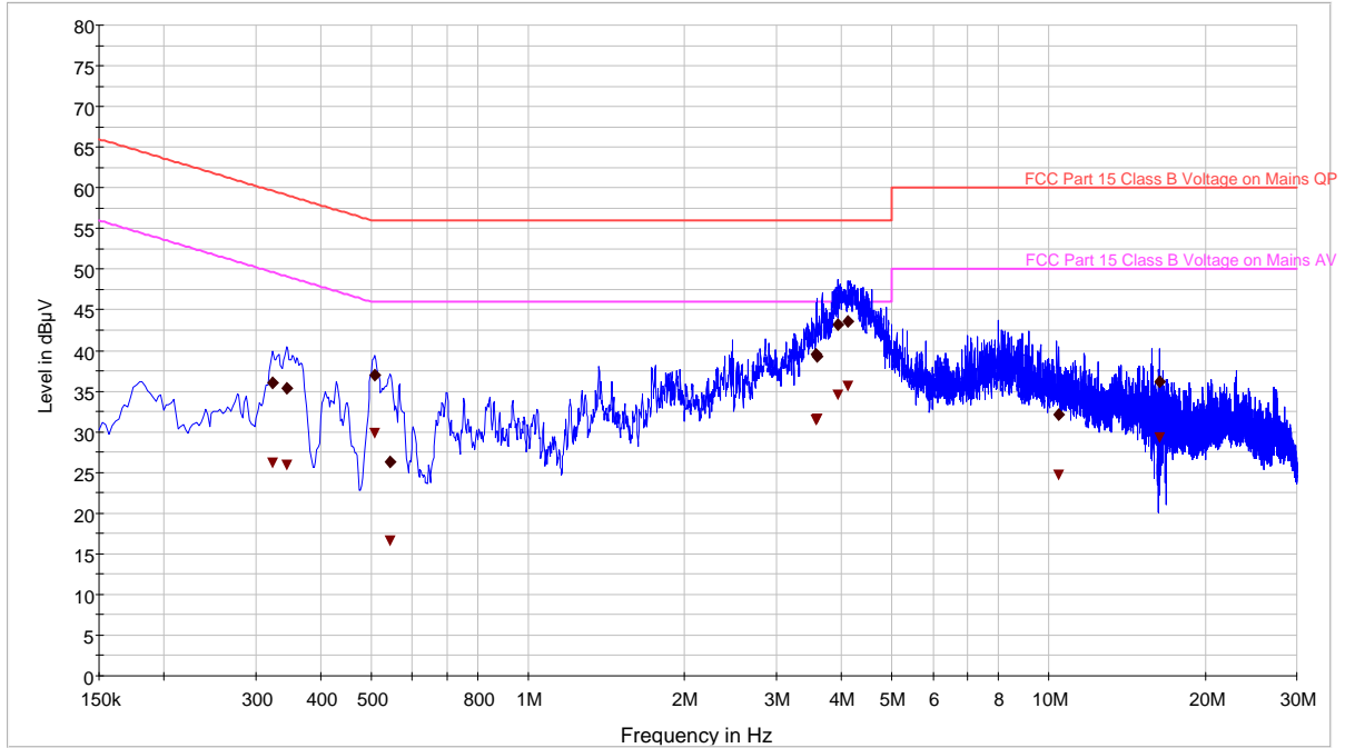
◆ FCC Part 15 Class B Voltage on Mains QP.LimitLine Final Result 1-QPK ▼ FCC Part 15 Class B Voltage on Mains AV.LimitLine Final Result 2-AVG — Preview Result 1-PK+
