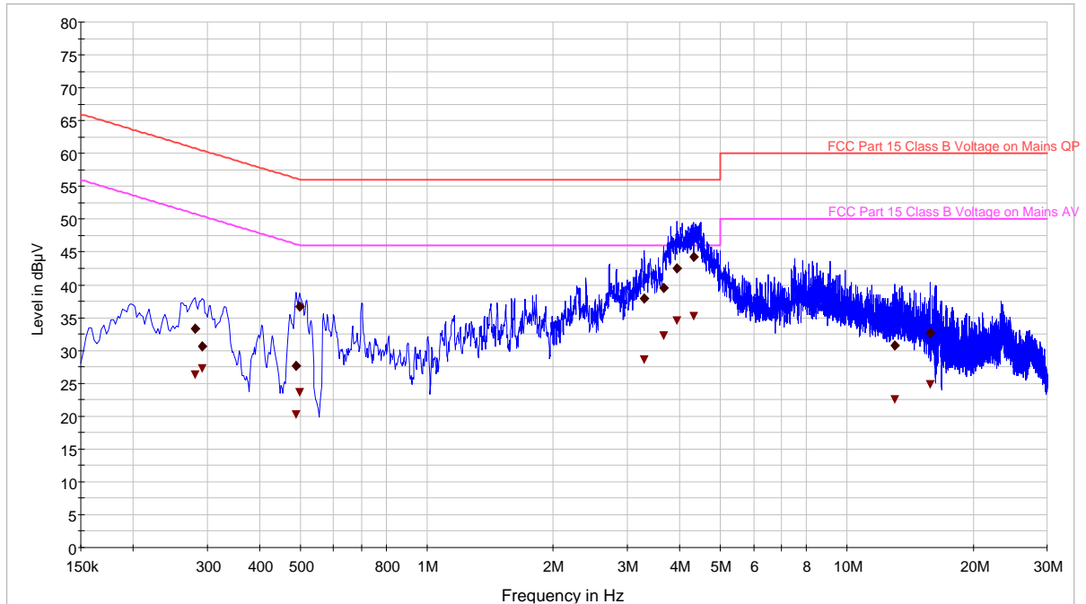
Plot 6-57. Line Conducted Plot with 802.11a (UNII Band 3)
