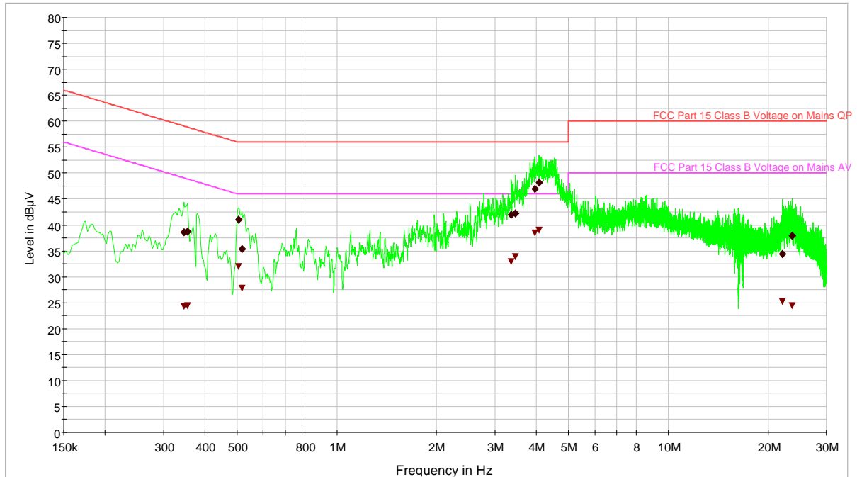
Plot 6-57. Line Conducted Data with 802.11a (UNII Band 2)
