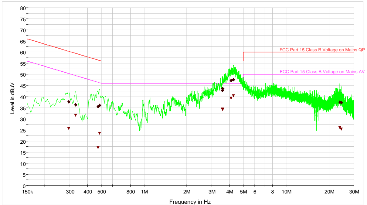
Plot 6-58. Line Conducted Data with 802.11a (UNII Band 3)
