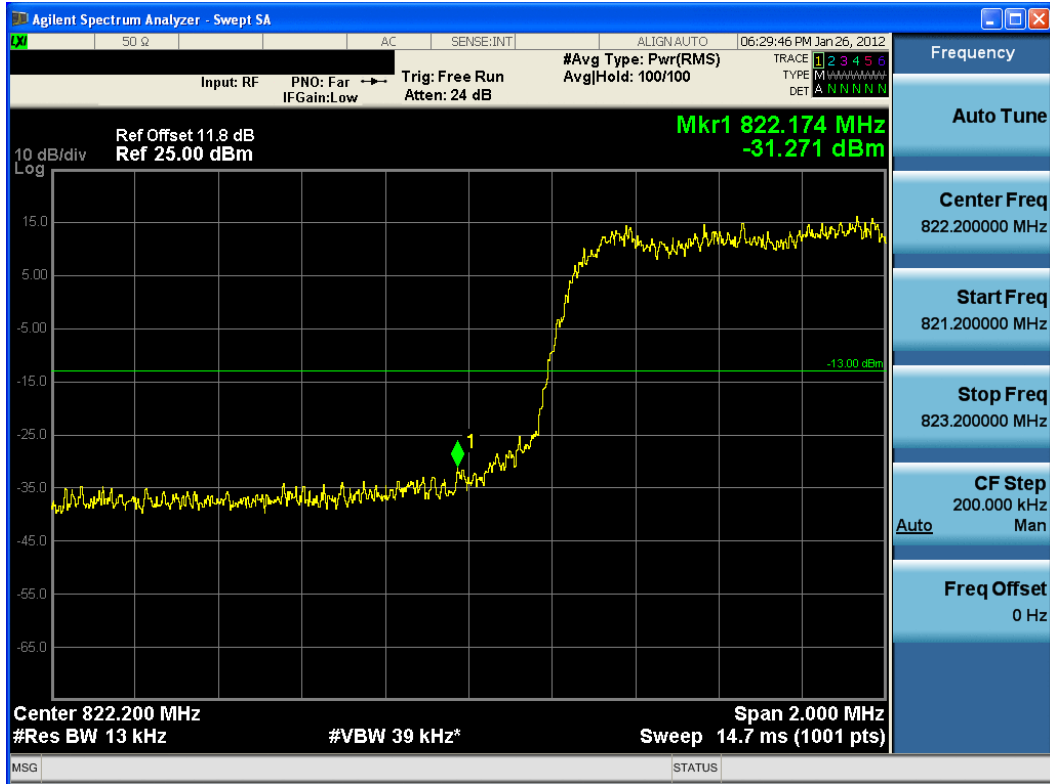
Plot 6-3. Interior Channel Edge Plot (BC10 CDMA Ch. 684) - §90.691
