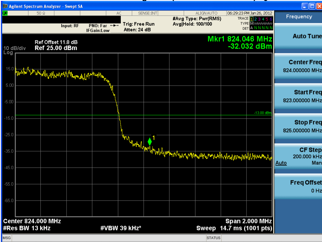
Plot 6-4. Channel Edge Plot (BC10 CDMA Ch. 684) - §90.691
