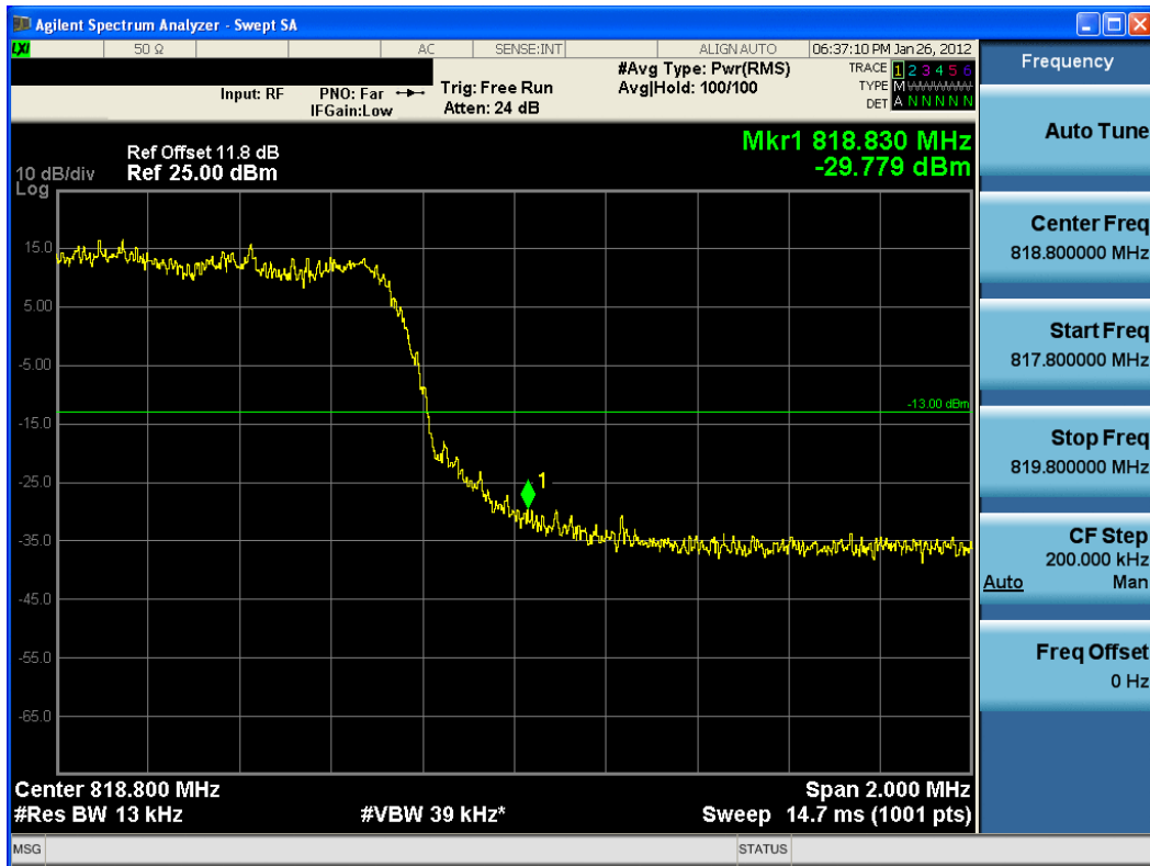
Plot 6-2. Interior Channel Edge Plot (BC10 CDMA Ch. 476) - $90.691
