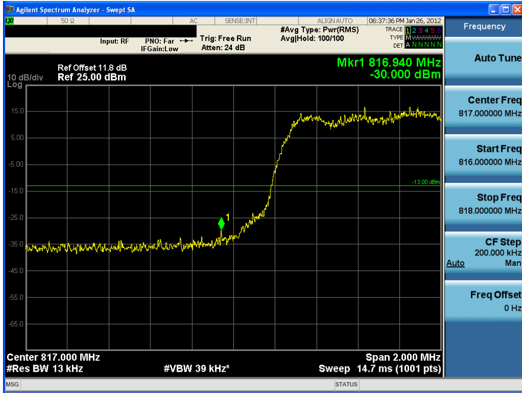
Plot 6-1. Channel Edge Plot (BC10 CDMA Ch. 476) - $90.691
