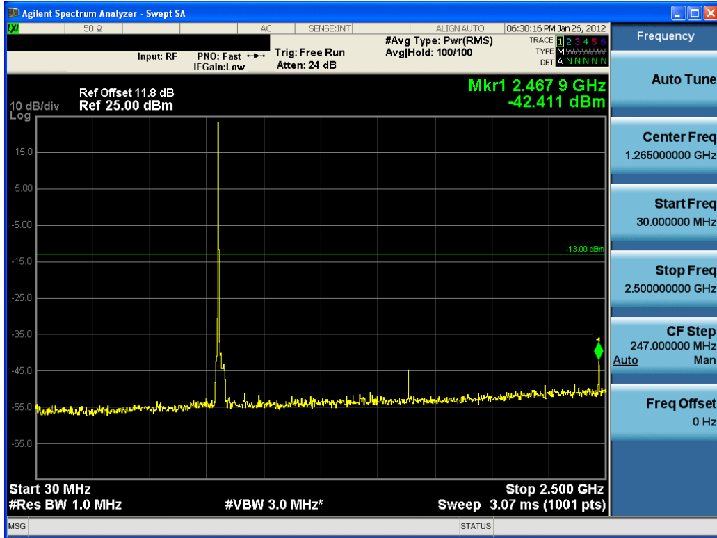
Plot 7-4. Conducted Spurious Plot (BC10 CDMA Ch. 684)
