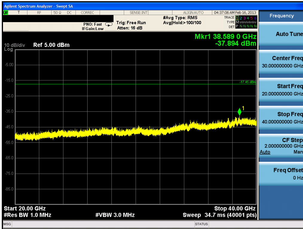
Plot 6-63. Conducted Spurious Plot (802.11a – Ch. 165)
