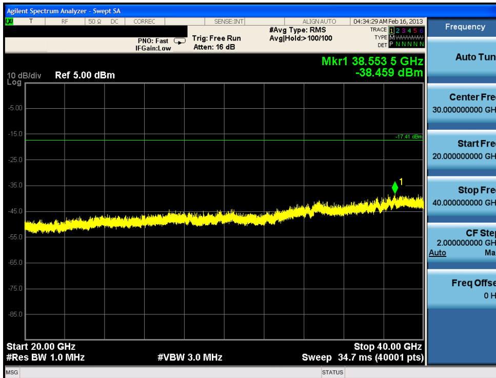
Plot 6-61. Conducted Spurious Plot (802.11a – Ch. 157)
