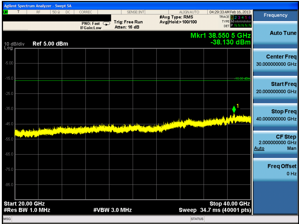
Plot 6-59. Conducted Spurious Plot (802.11a – Ch. 149)
