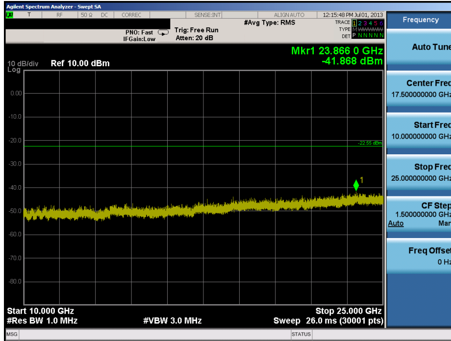
Plot 6-54. Conducted Spurious Plot (802.11b – Ch. 11)
