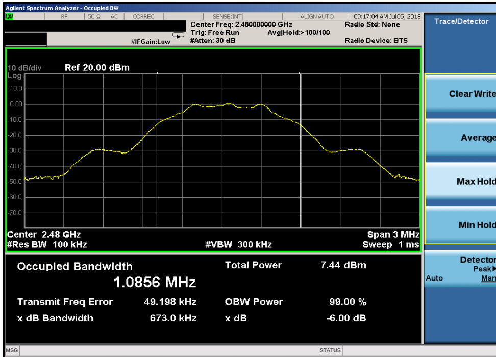
Plot 6-3. 6dB Bandwidth Plot (Bluetooth (LE) – Ch. 39)
