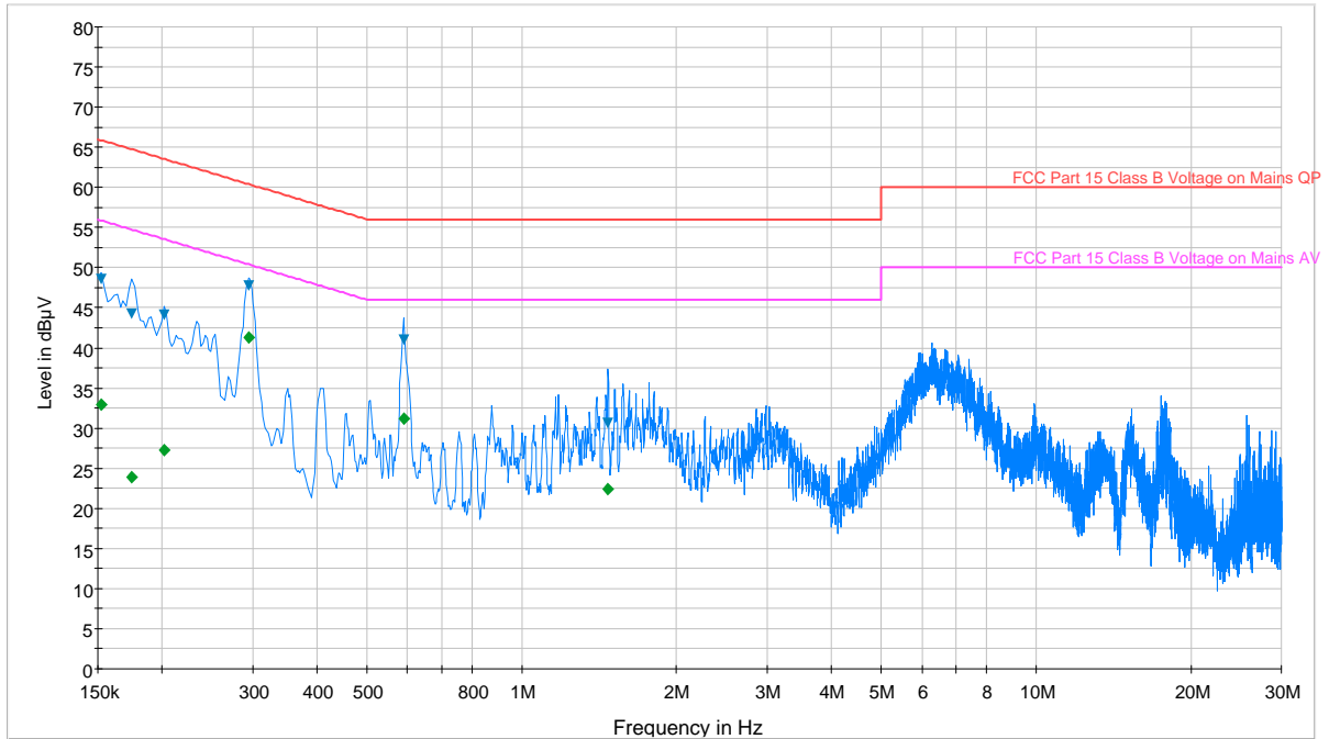
Plot 6-72. Line Conducted Plot with 802.11a UNII Band 2 (N)
