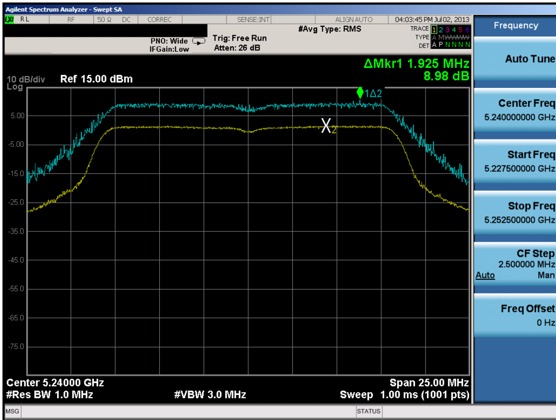
Plot 6-51. Peak Excursion Ratio Plot (802.11a)
