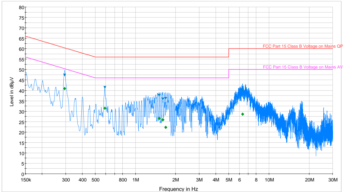
Plot 6-73. Line Conducted Plot with 802.11a UNII Band 3 (L1)
