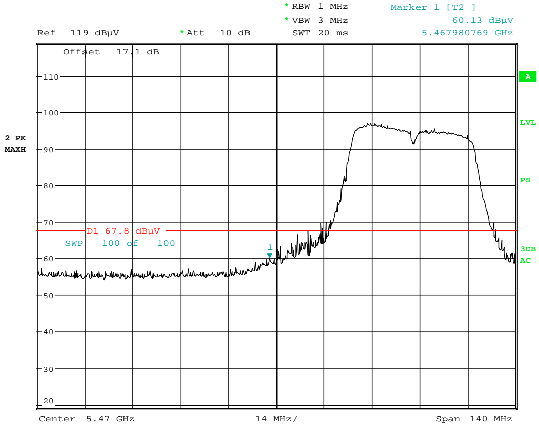
Plot 6-66. Radiated Restricted Lower Band
