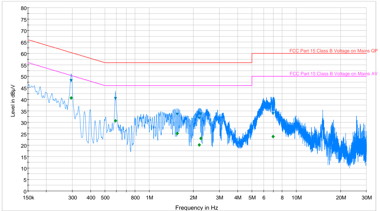
Plot 6-69. Line Conducted Plot with 802.11a UNII Band 1 (L1)
