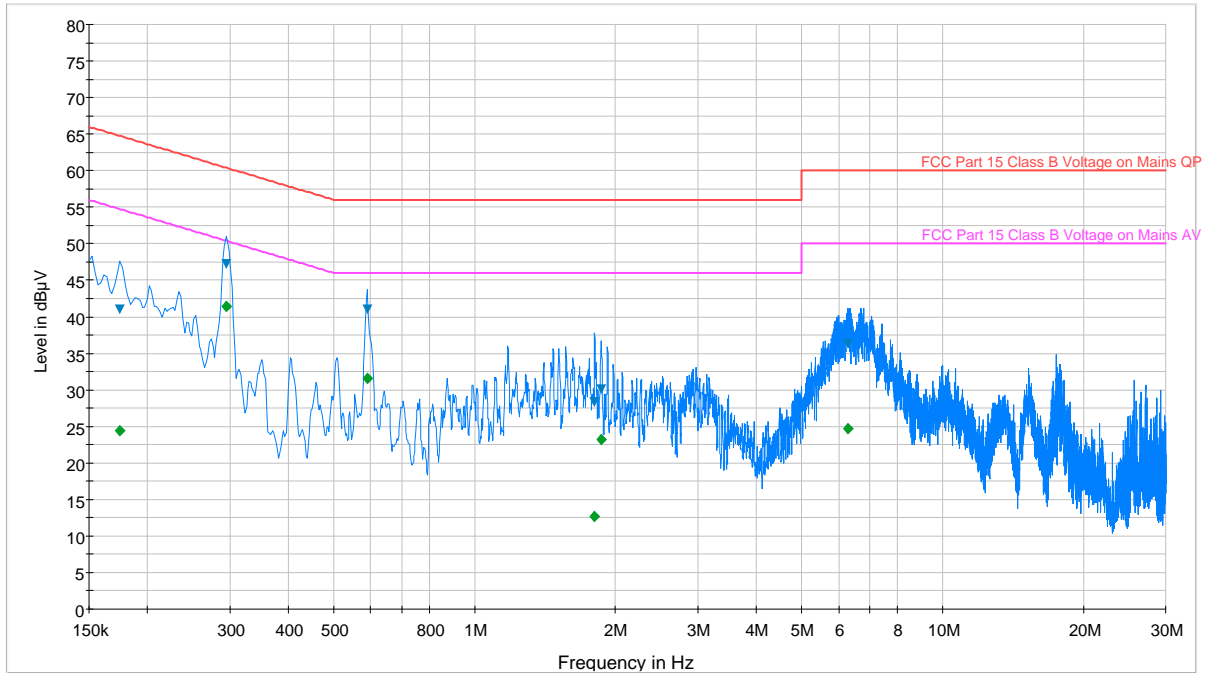
Plot 6-74. Line Conducted Plot with 802.11a UNII Band 3 (N)
