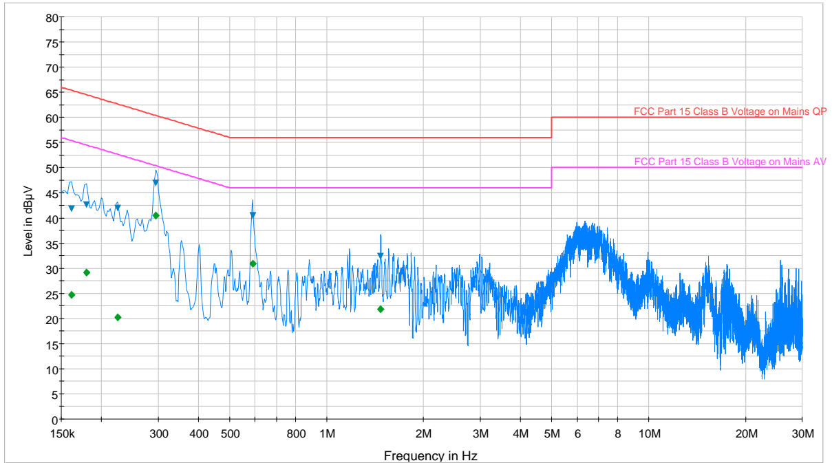
Plot 6-70. Line Conducted Plot with 802.11a UNII Band 1 (N)
