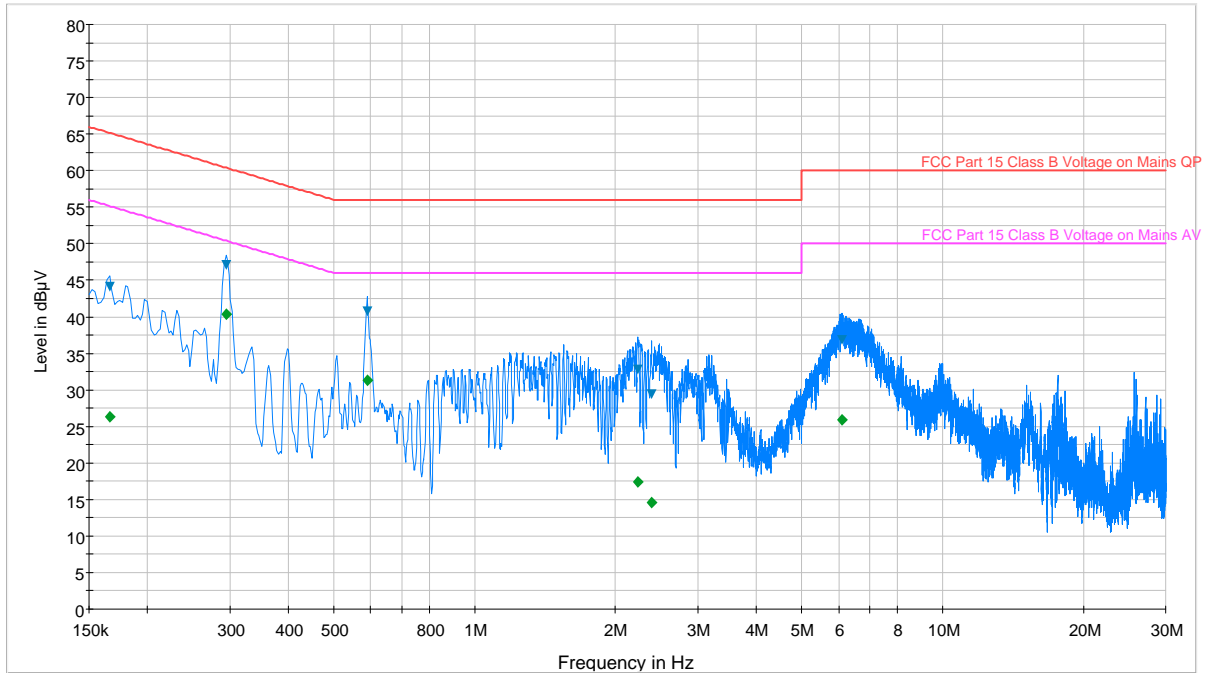
Plot 6-71. Line Conducted Plot with 802.11a UNII Band 2 (L1)
