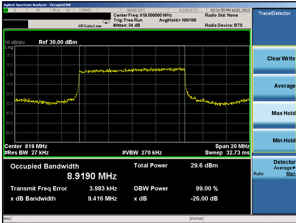
Plot 7-50. Occupied Bandwidth Plot (10MHz QPSK – RB Size 50 – High Channel)
