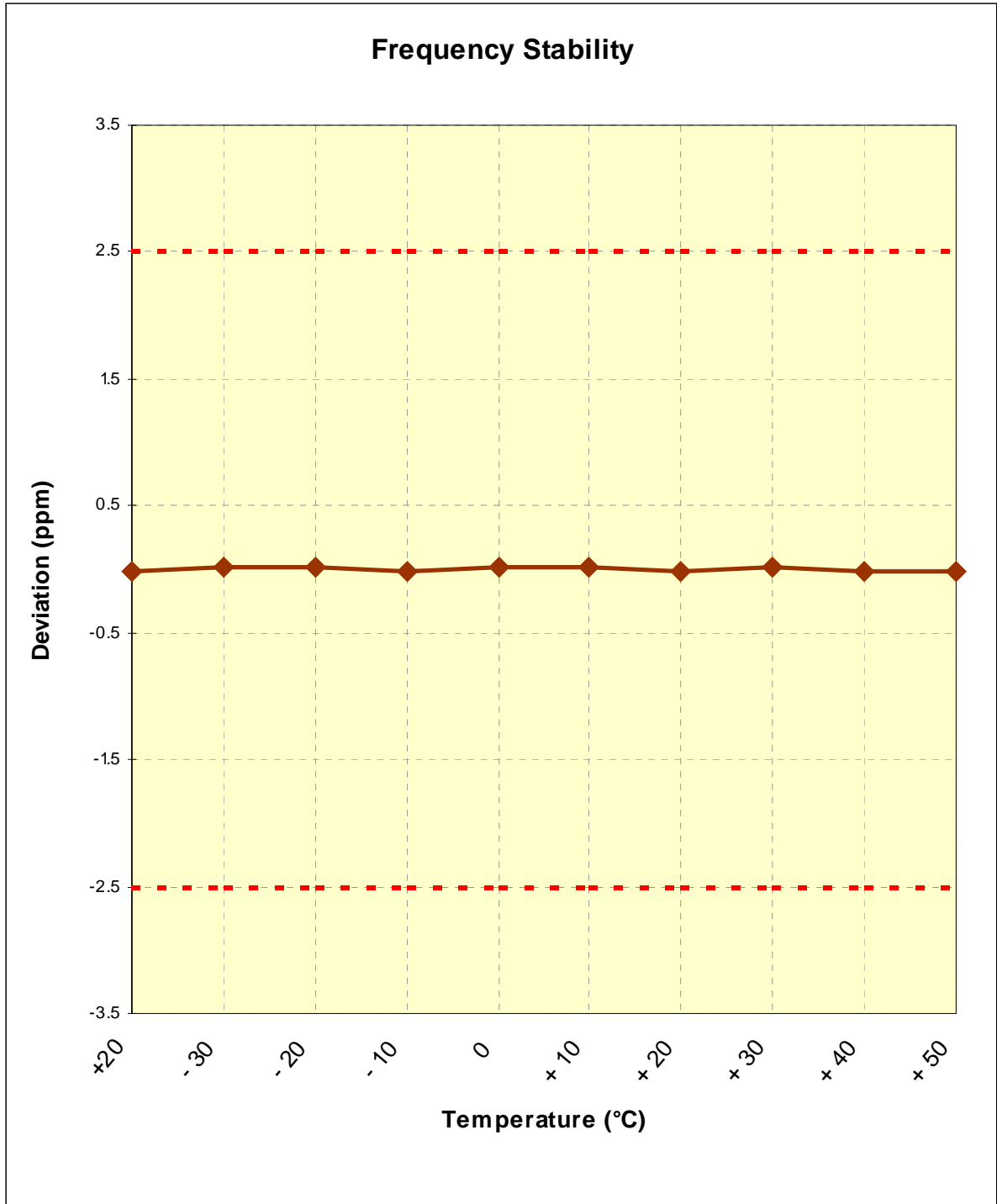
Figure 6-1. Frequency Stability Graph (Ch. 684)
