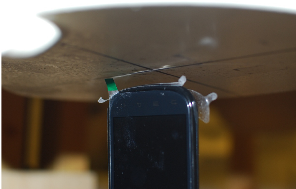
Figure 24-8 SAR Test Setup Photo – Bottom Edge at 1.0cm
