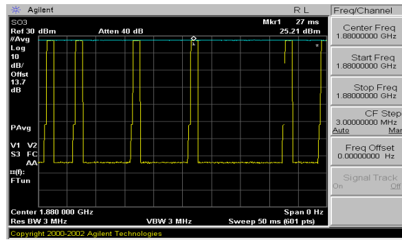
Figure 8-4 Zero-Span Plots
