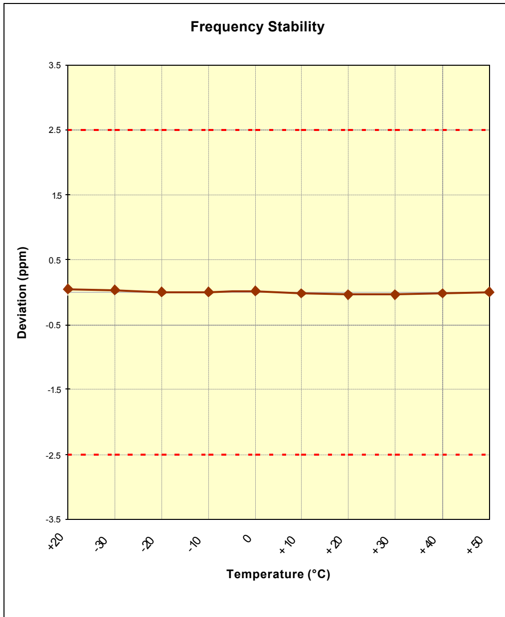
Figure 6-1. Frequency Stability Graph (BC10 CDMA Mode – Ch.684)
