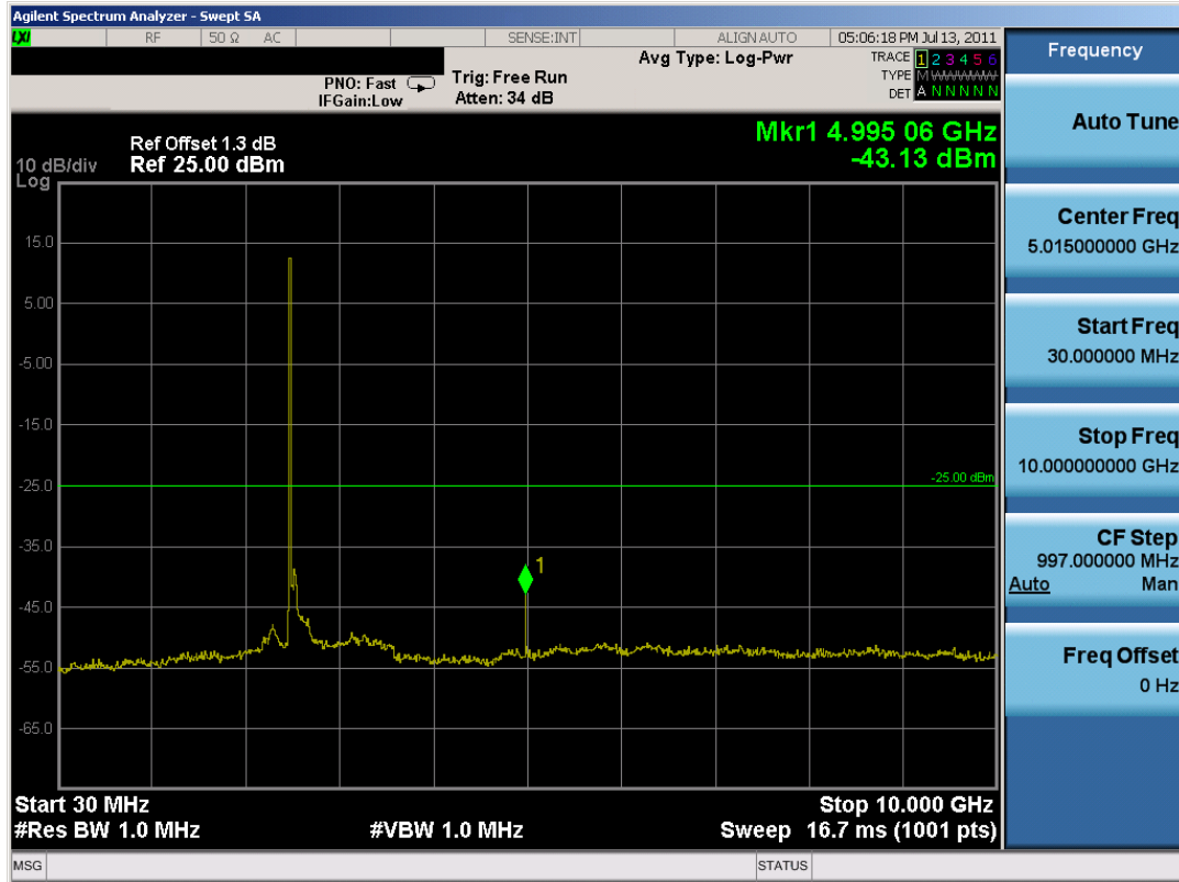
Plot 8-1. Conducted Spurious Plot (WiMAX Mode – Low Channel)
