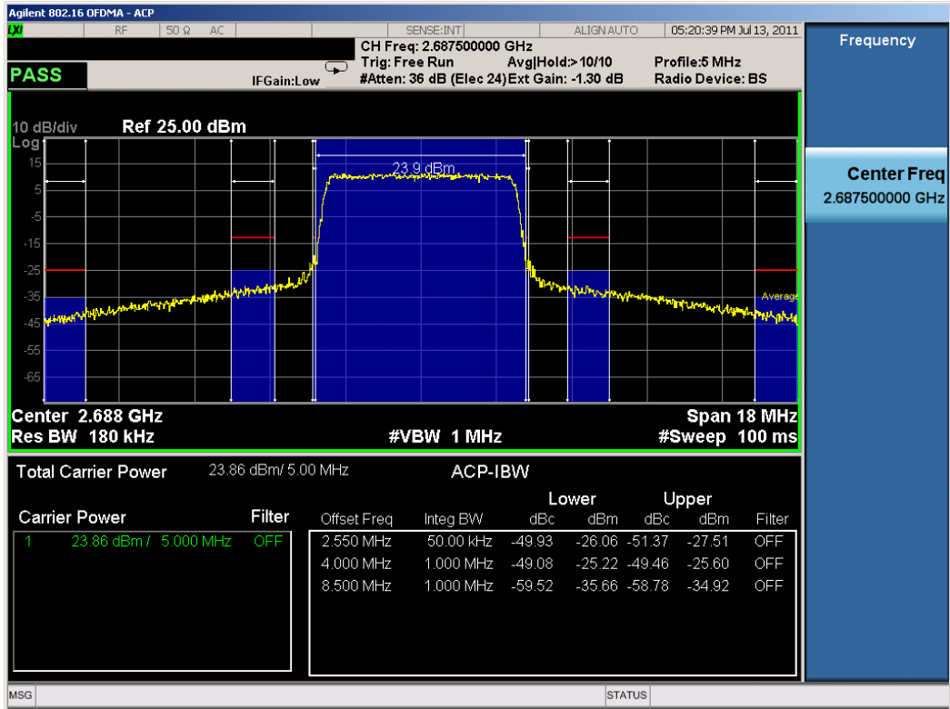
Plot 8-14. Adjacent Channel Power Plot (WiMAX Mode – High Channel – 16QAM)
