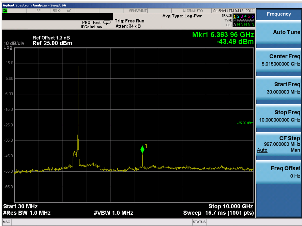
Plot 7-7. Conducted Spurious Plot (WiMAX Mode – High Channel)
