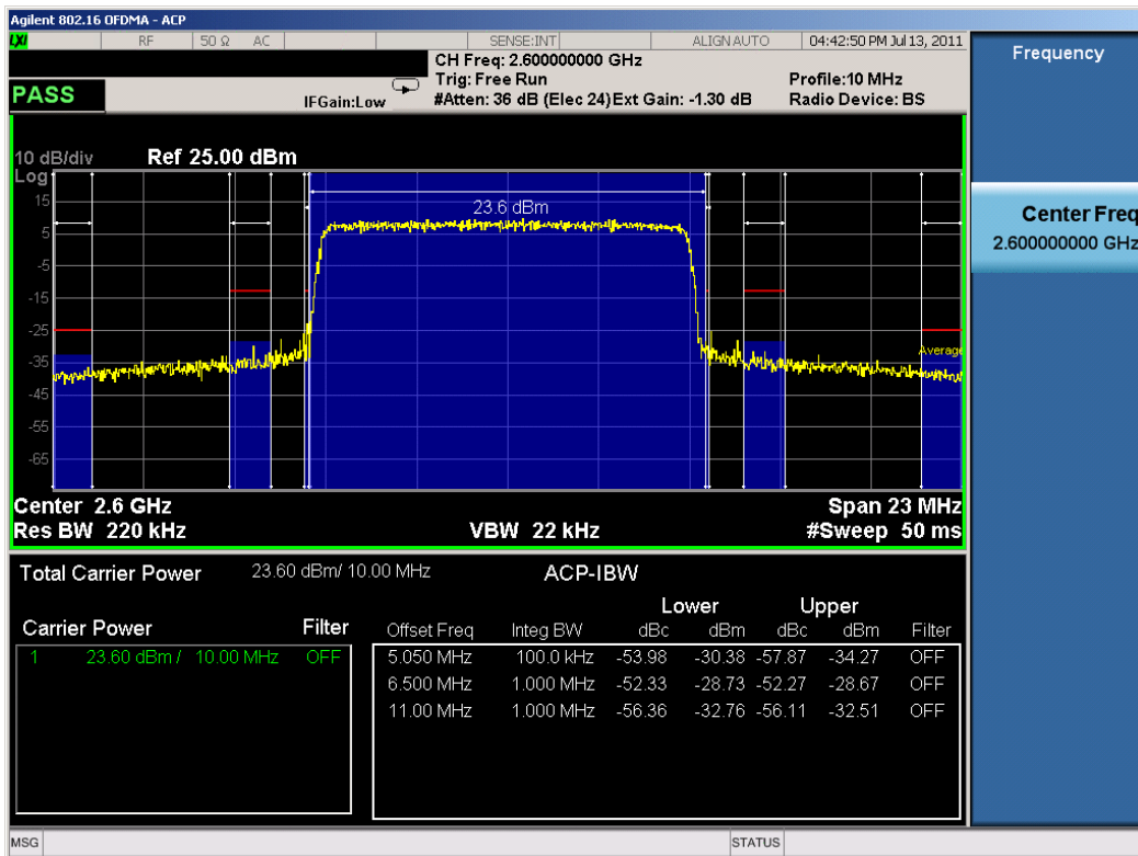
Plot 7-11. Adjacent Channel Power Plot (WiMAX Mode – Mid Channel - QPSK)
