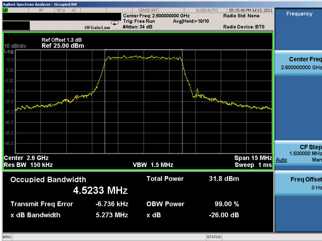
Plot 8-6. Occupied Bandwidth with PUSC 16QAM Modulation Plot (WiMAX Mode – Mid Channel)
