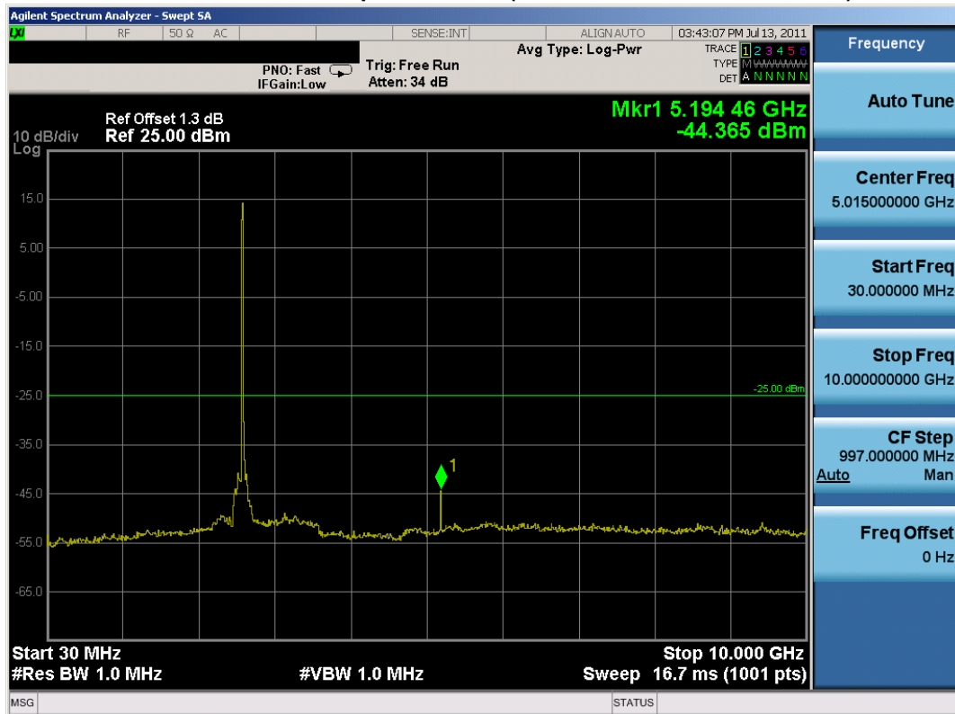
Plot 7-3. Conducted Spurious Plot (WiMAX Mode – Mid Channel)
