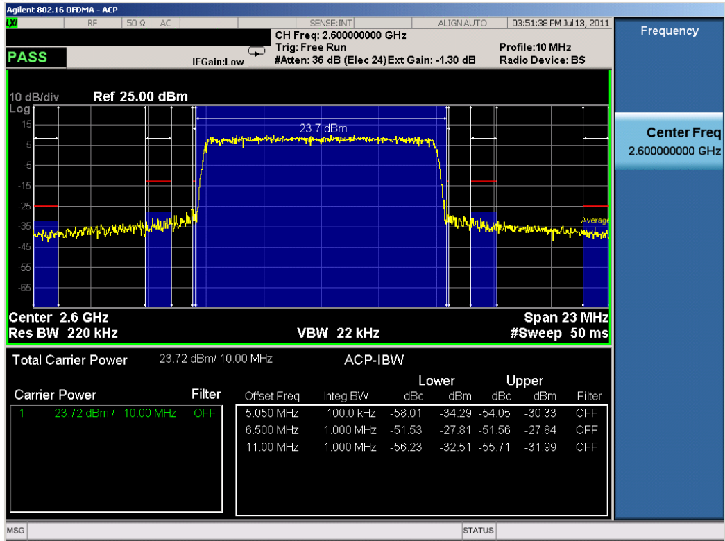
Plot 7-12. Adjacent Channel Power Plot (WiMAX Mode – Mid Channel – 16QAM)
