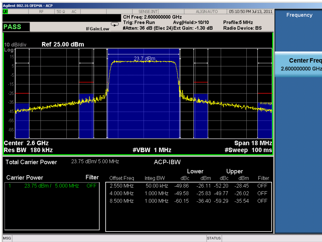
Plot 8-11. Adjacent Channel Power Plot (WiMAX Mode – Mid Channel - QPSK)
