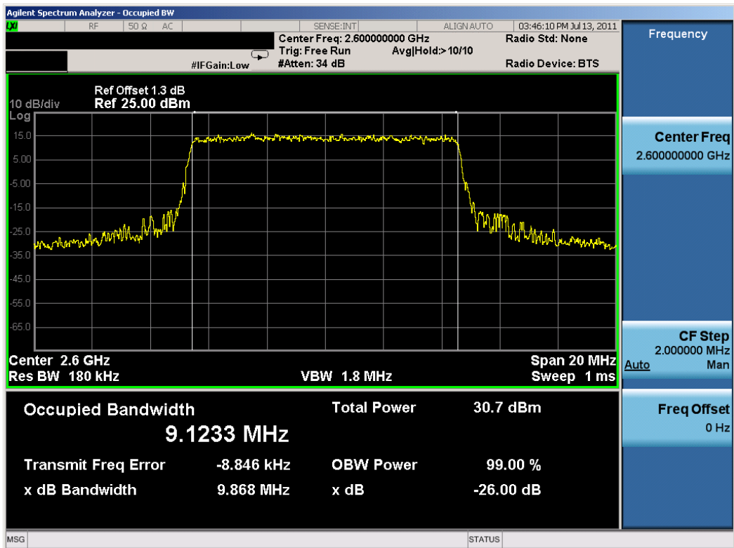
Plot 7-5. Occupied Bandwidth with PUSC QPSK Modulation Plot (WiMAX Mode – Mid Channel)
