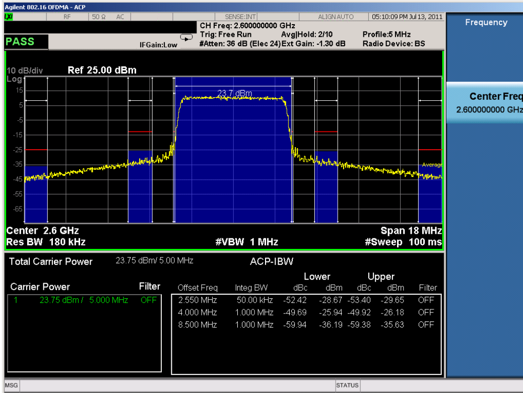
Plot 8-12. Adjacent Channel Power Plot (WiMAX Mode – Mid Channel – 16QAM)
