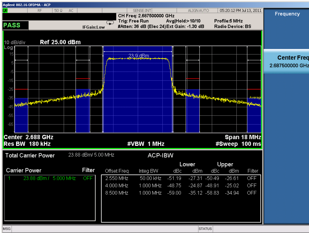
Plot 8-13. Adjacent Channel Power Plot (WiMAX Mode – High Channel - QPSK)
