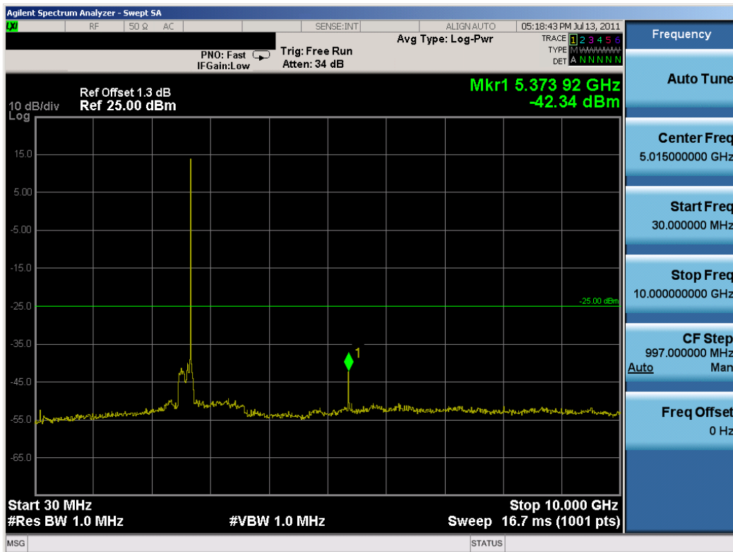
Plot 8-7. Conducted Spurious Plot (WiMAX Mode – High Channel)
