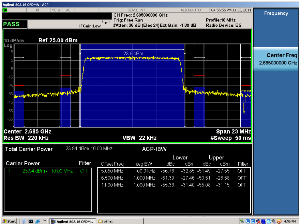
Plot 7-13. Adjacent Channel Power Plot (WiMAX Mode – High Channel - QPSK)
