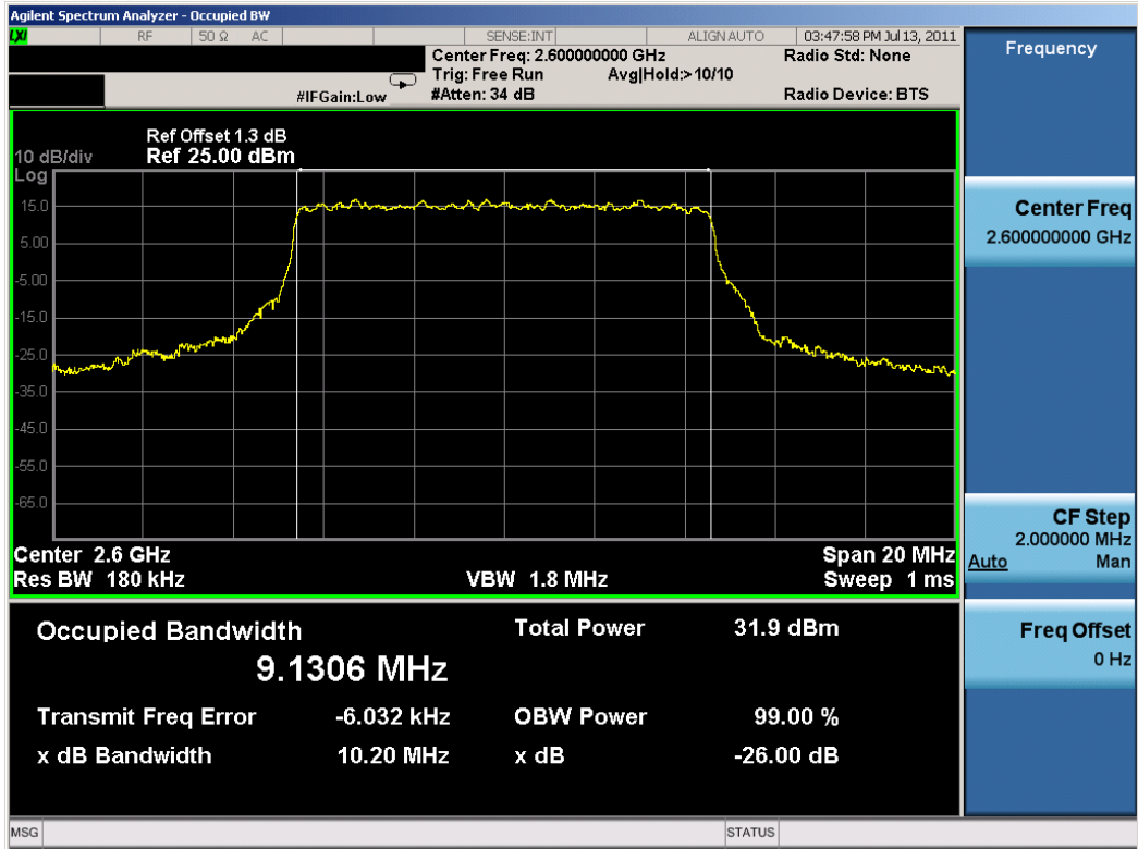
Plot 7-6. Occupied Bandwidth with PUSC 16QAM Modulation Plot (WiMAX Mode – Mid Channel)
