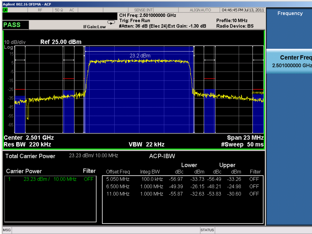
Plot 7-10. Adjacent Channel Power Plot (WiMAX Mode – Low Channel – 16QAM)
