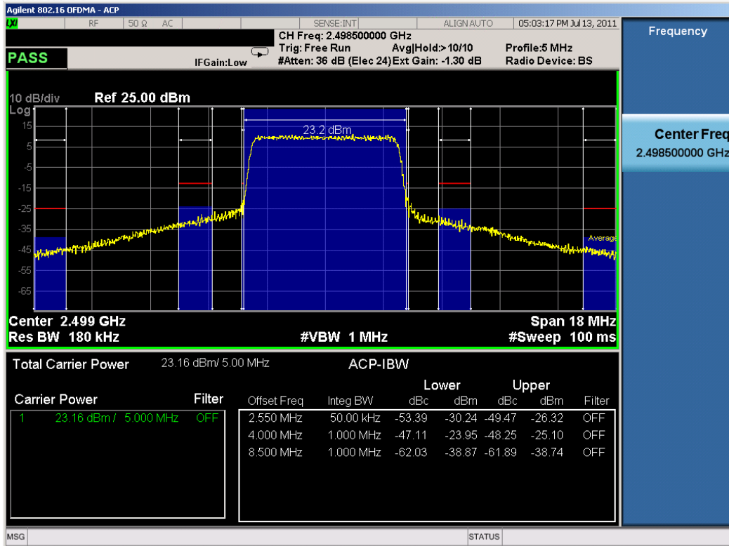
Plot 8-10. Adjacent Channel Power Plot (WiMAX Mode – Low Channel – 16QAM)
