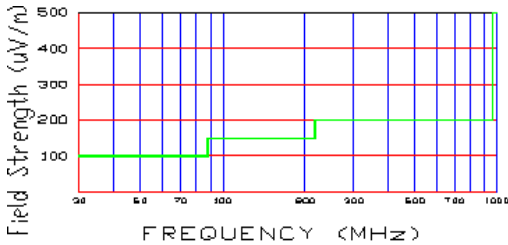
Figure 6-3. 3-Meter Limits
