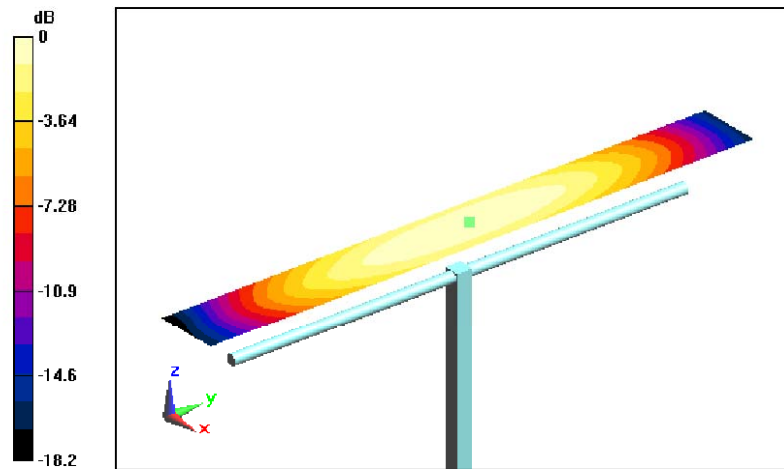
0 dB = 0.439A/m
