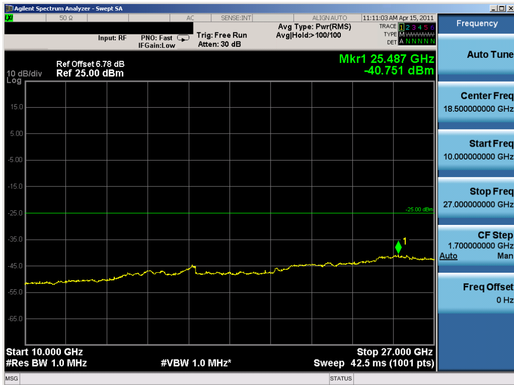
Plot 8-6. Conducted Spurious Plot (WiMAX – Mid Channel)
