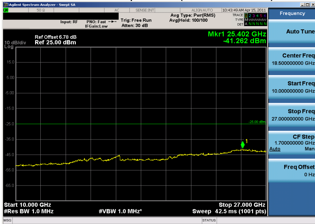
Plot 8-2. Conducted Spurious Plot (WiMAX – Low Channel)
