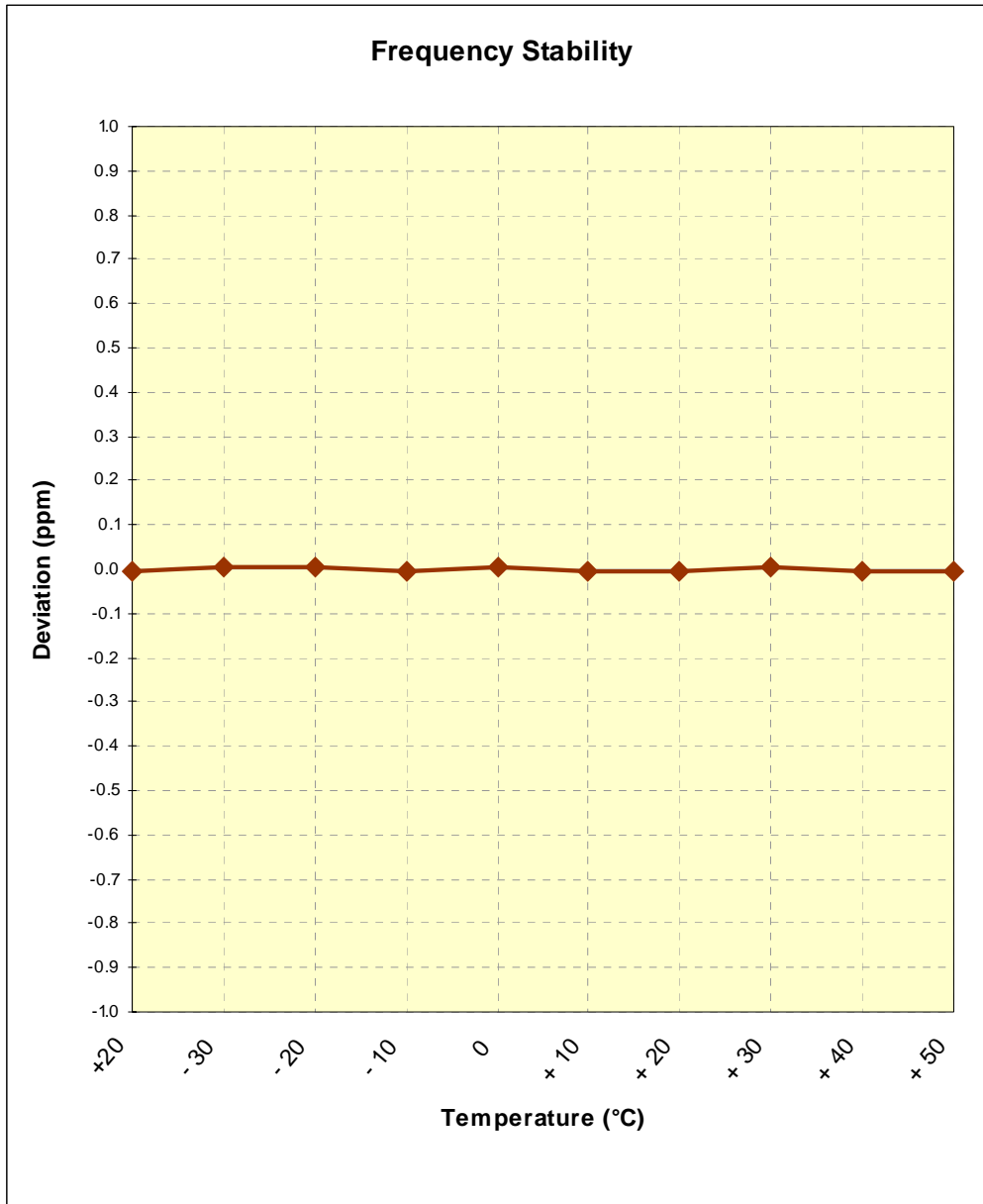
Figure 6-3. Frequency Stability Graph (WiMAX Mode)
