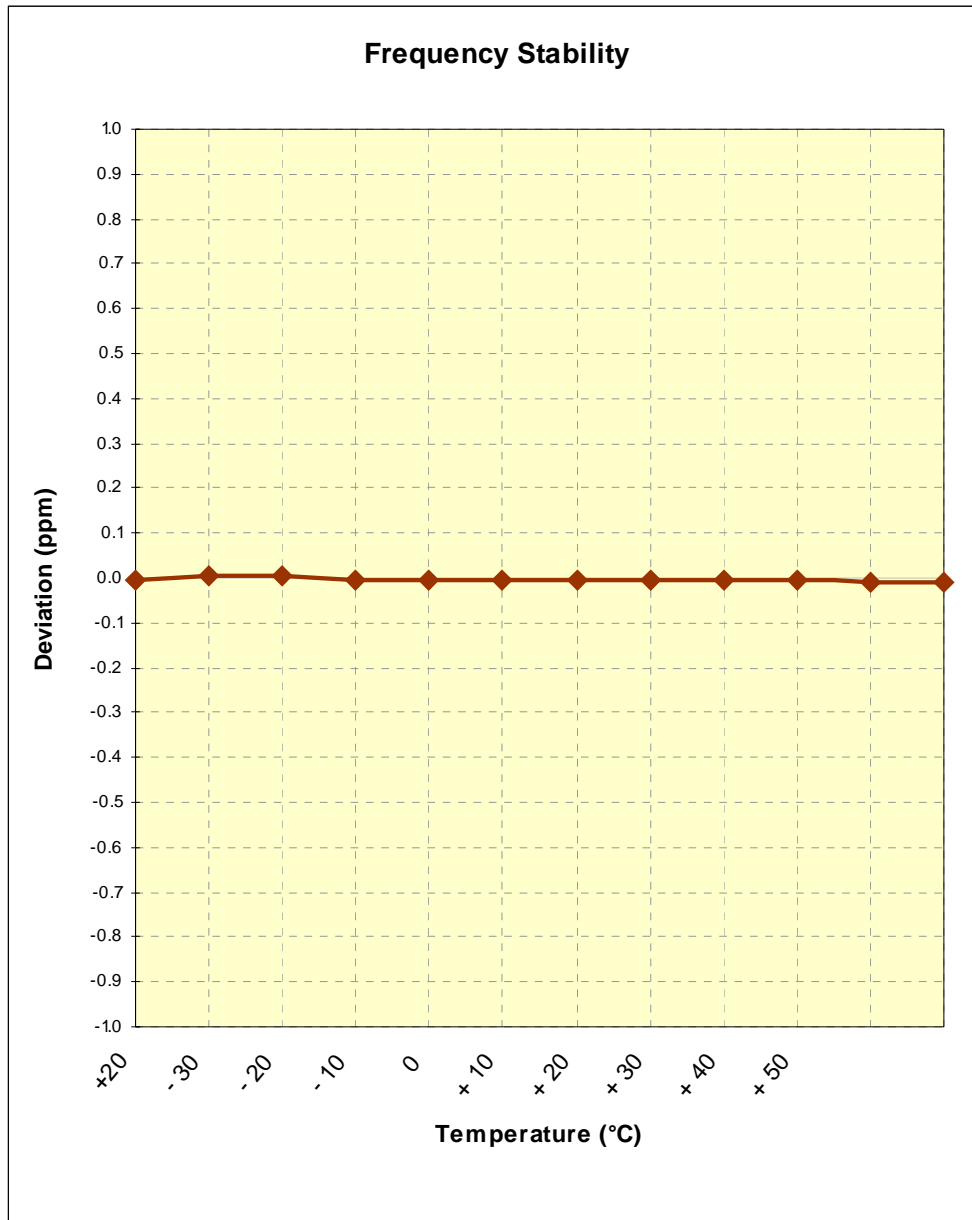
Figure 6-2. Frequency Stability Graph (WiMAX Mode)
