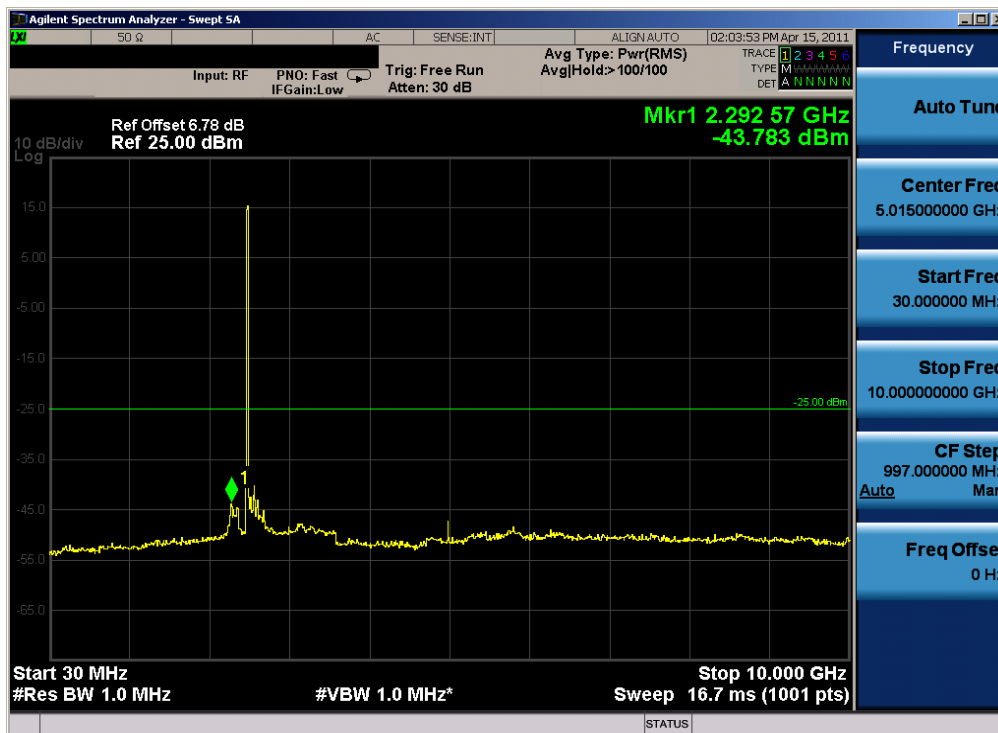
Plot 7-1. Conducted Spurious Plot (WiMAX – Low Channel)
