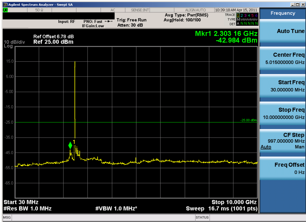
Plot 8-1. Conducted Spurious Plot (WiMAX – Low Channel)
