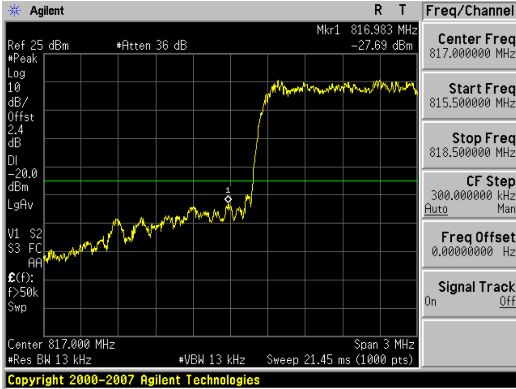
Plot 7-3. Channel Exterior Edge Plot (BC10 CDMA Ch. 476) - §90.691
