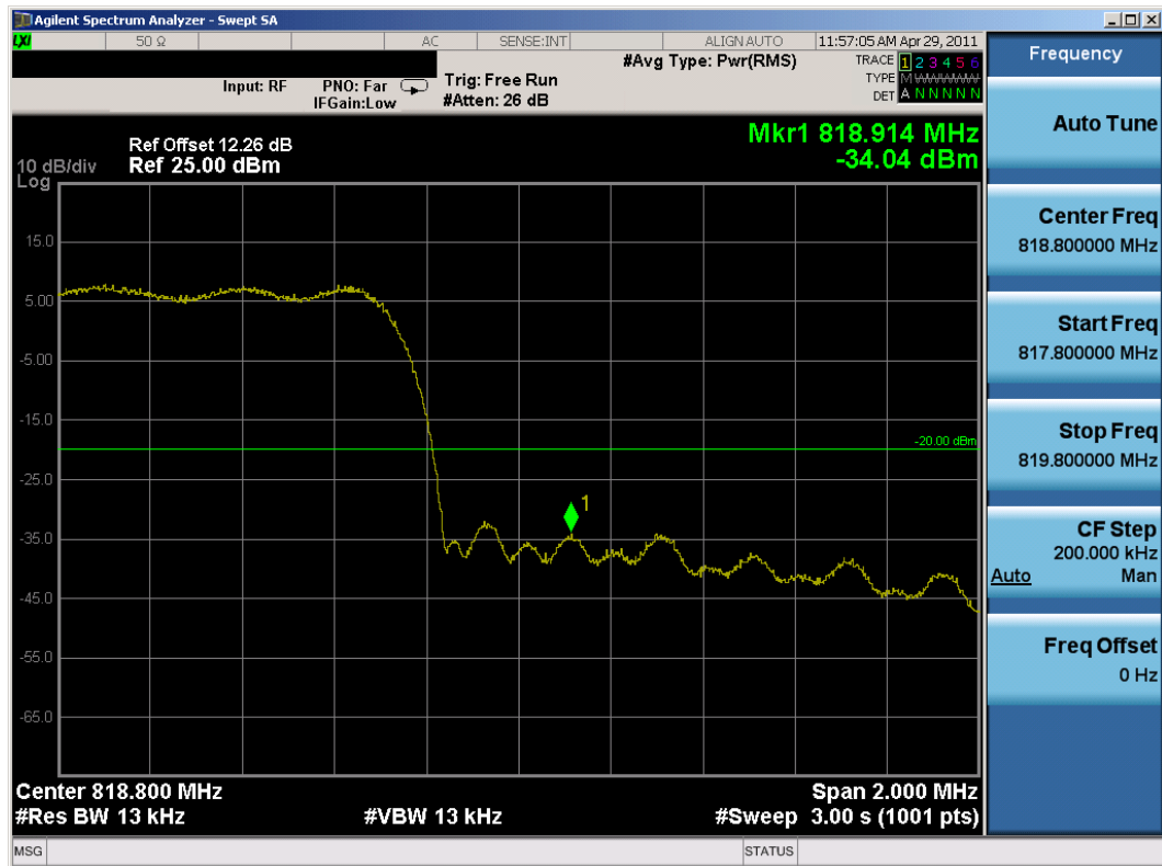
Plot 7-4. Channel Interior Edge Plot (BC10 CDMA Ch. 476) - §90.691
