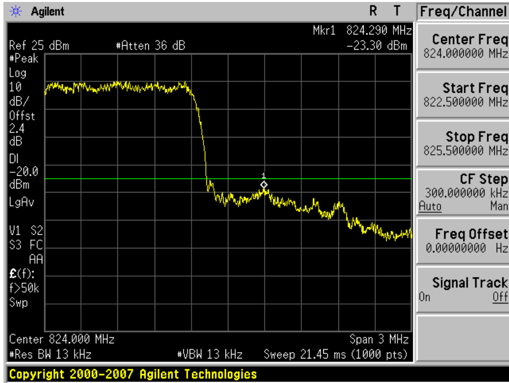
Plot 7-9. Channel Exterior Edge Plot (BC10 CDMA Ch. 684) - §90.691
