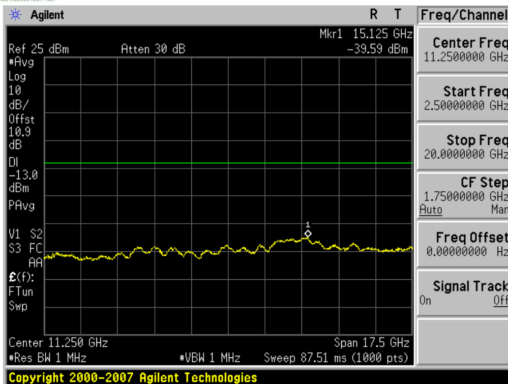
Plot 7-25. Spurious Plot (PCS (BC14) CDMA Mode – Ch. 1275)
