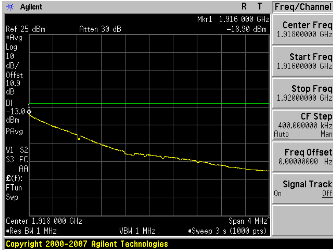
Plot 7-27. 4MHz Span Plot (PCS (BC14) CDMA Mode – Ch. 1275)
