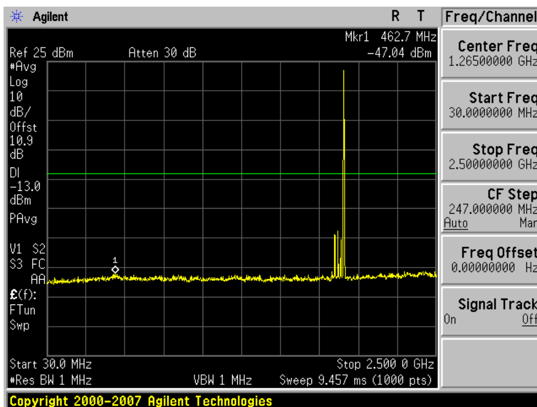
Plot 7-24. Conducted Spurious Plot (PCS (BC14) CDMA Mode – Ch. 1275)
