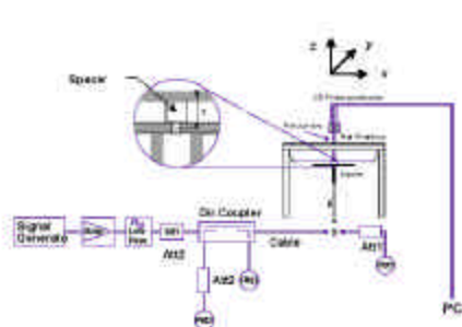
Figure 12.1 Dipole Validation Test Setup
