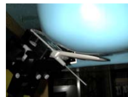
Figure 16. Left Head SAR Test Setup
