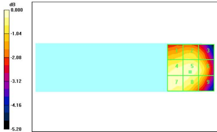
0 dB = 48.6V/m
