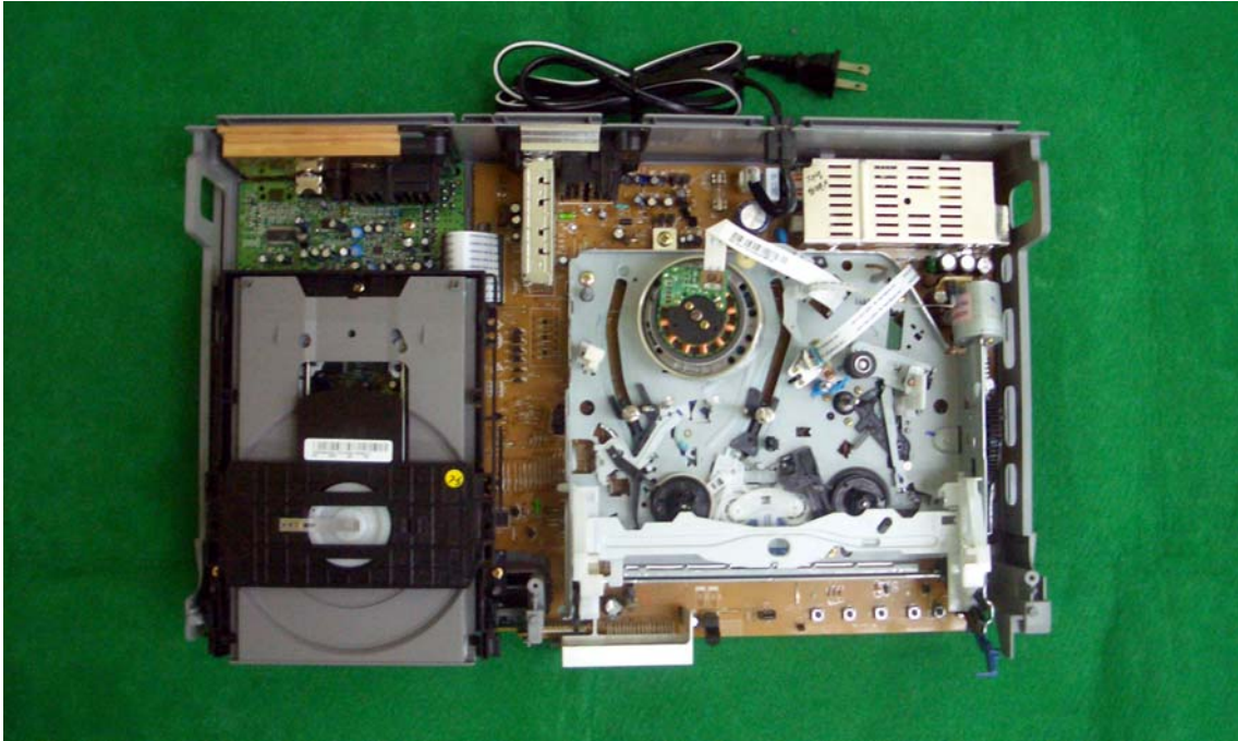
Front View – Front/Top cover open
