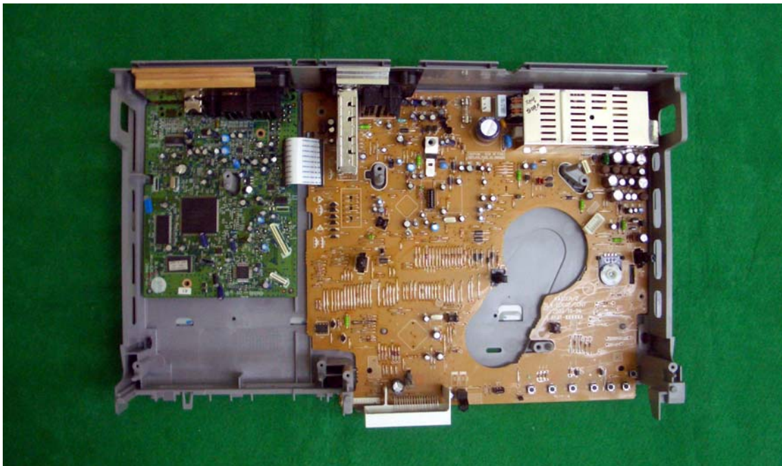
Top View – Top cover open
