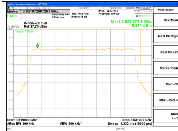
LTE B48 10MHz 64QAM Mid Channel
