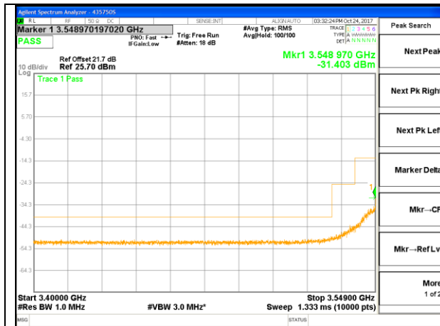
LTE B48 10MHz 64QAM Low Channel
