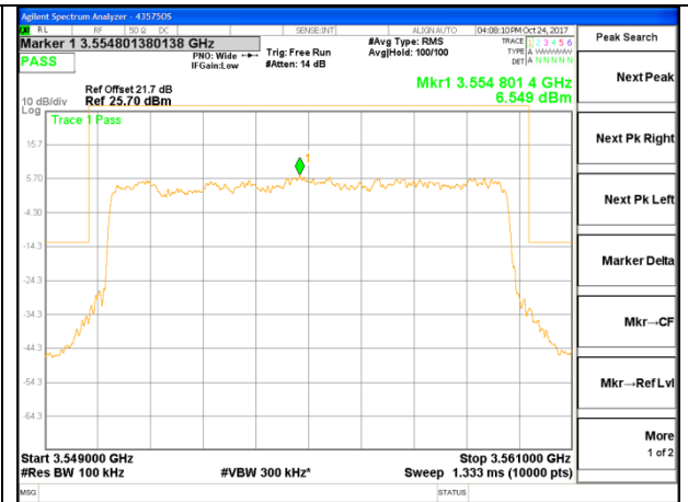
LTE B48 10MHz QPSK Low Channel
