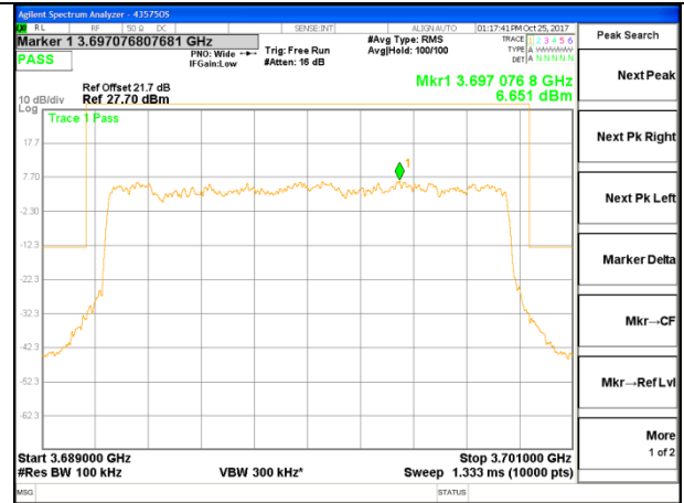
LTE B48 10MHz QPSK High Channel
