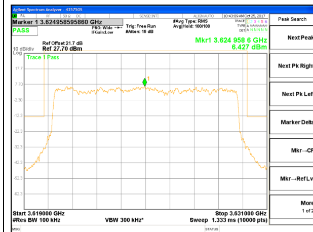
LTE B48 10MHz QPSK Mid Channel
