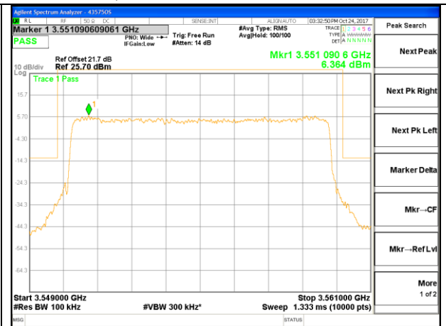
LTE B48 10MHz 64QAM Low Channel
