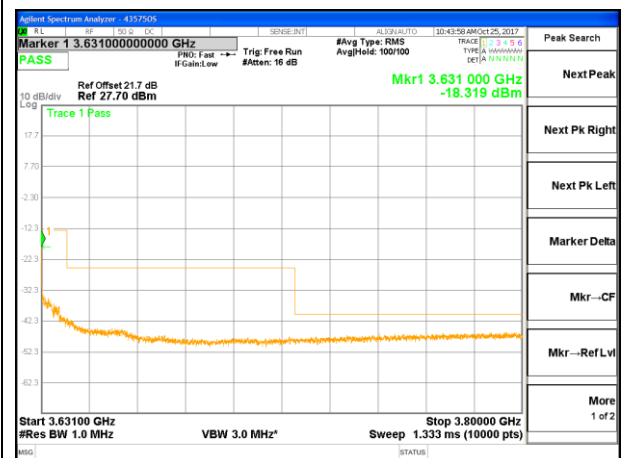
LTE B48 10MHz QPSK Mid Channel
