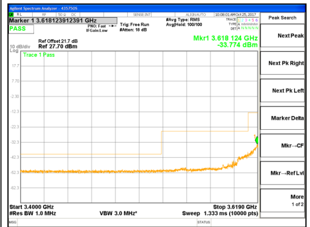
LTE B48 10MHz 64QAM Mid Channel
