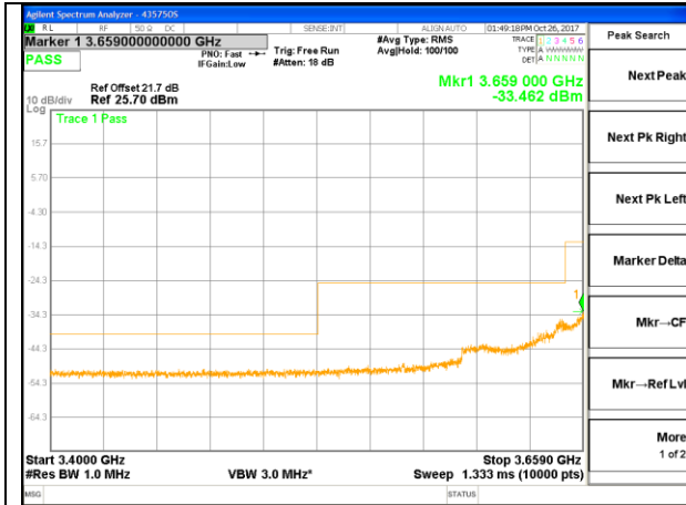
LTE B48 20MHz 64QAM High Channel
