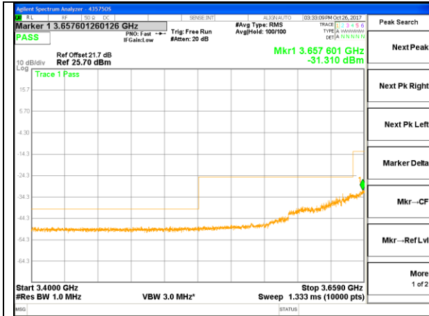
LTE B48 20MHz 16QAM High Channel
