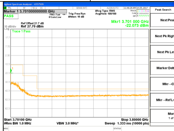
LTE B48 10MHz 16QAM High Channel
