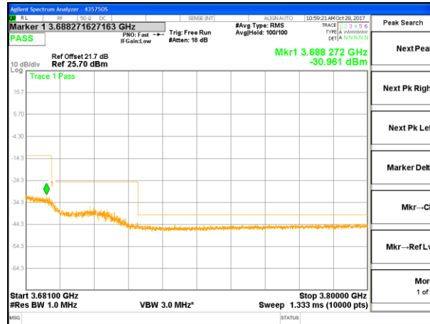
LTE B48 20MHz 16QAM High Channel
