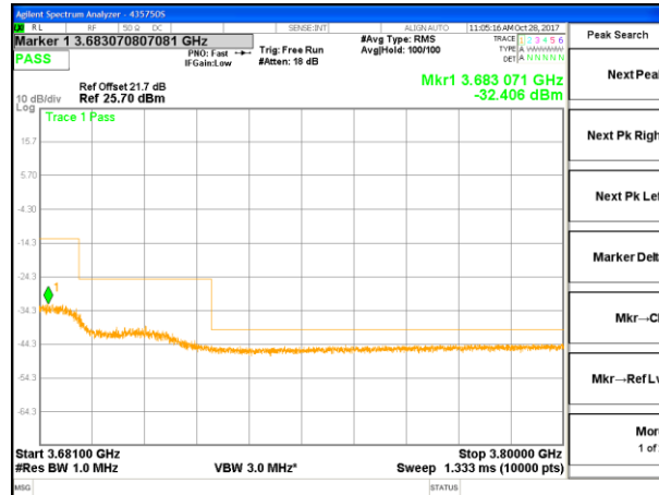
LTE B48 20MHz QPSK High Channel
