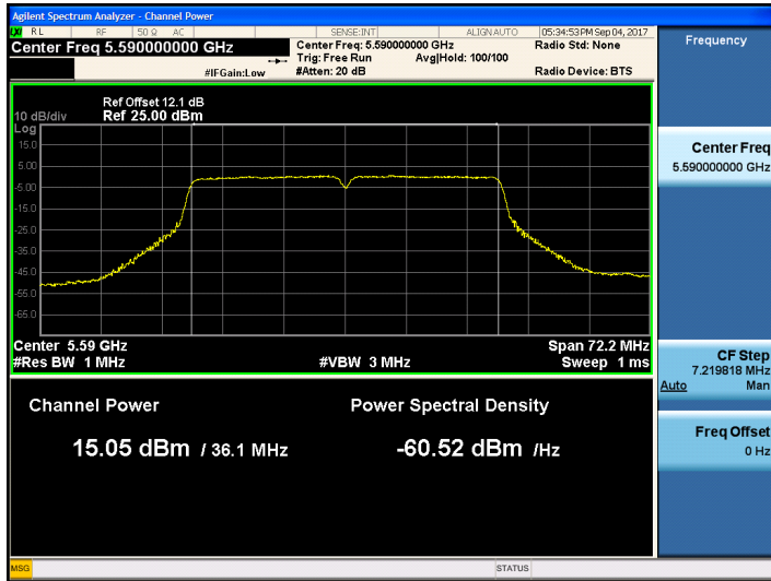
802.11ac_VHT40 UNII 2C BAND Average Power (5510 MHz ~5670 MHz) CH 118 MCS8
