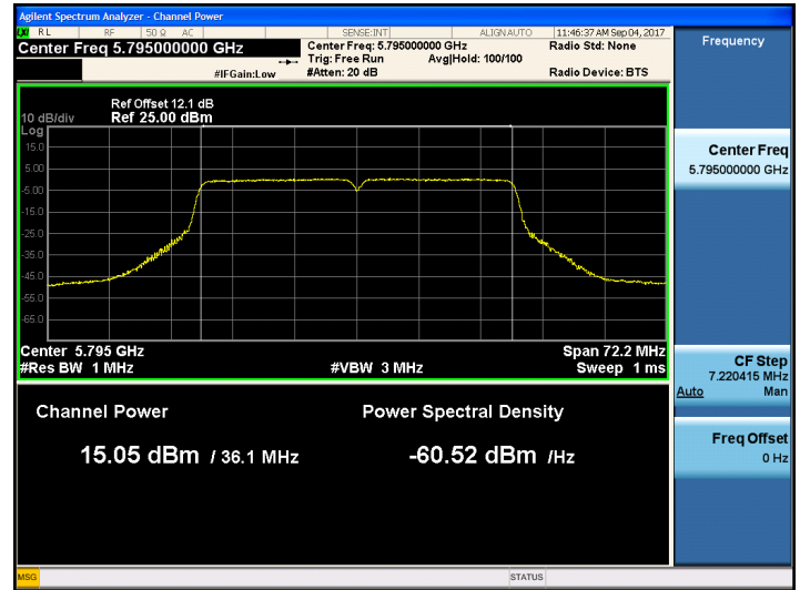
802.11n_HT40 UNII 3 BAND Average Power (5755 MHz ~5795 MHz) CH 159 MCS5
