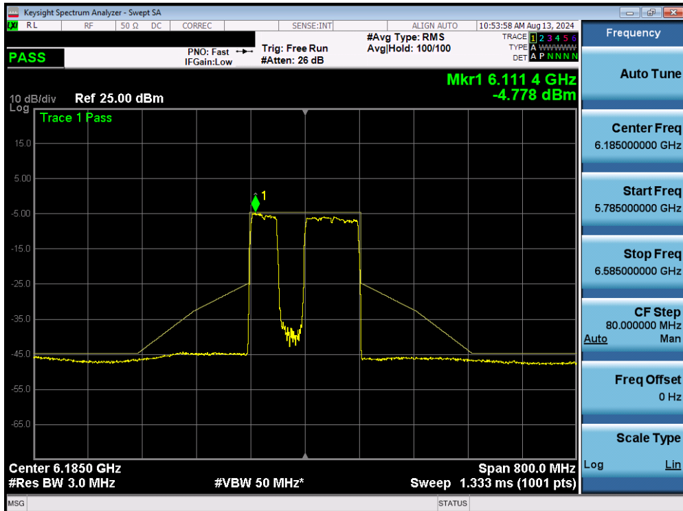
Plot 7-321. In Band Emissions MIMO ANT2 (160MHz BW 802.11be (996+484 Tones) (UNII Band 5) – Ch. 47)
