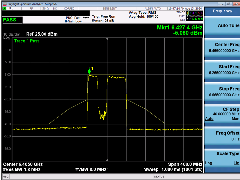
Plot 7-324. In Band Emissions MIMO ANT2 (80MHz BW 802.11be (484+242 Tones) (UNII Band 6) – Ch. 103)
