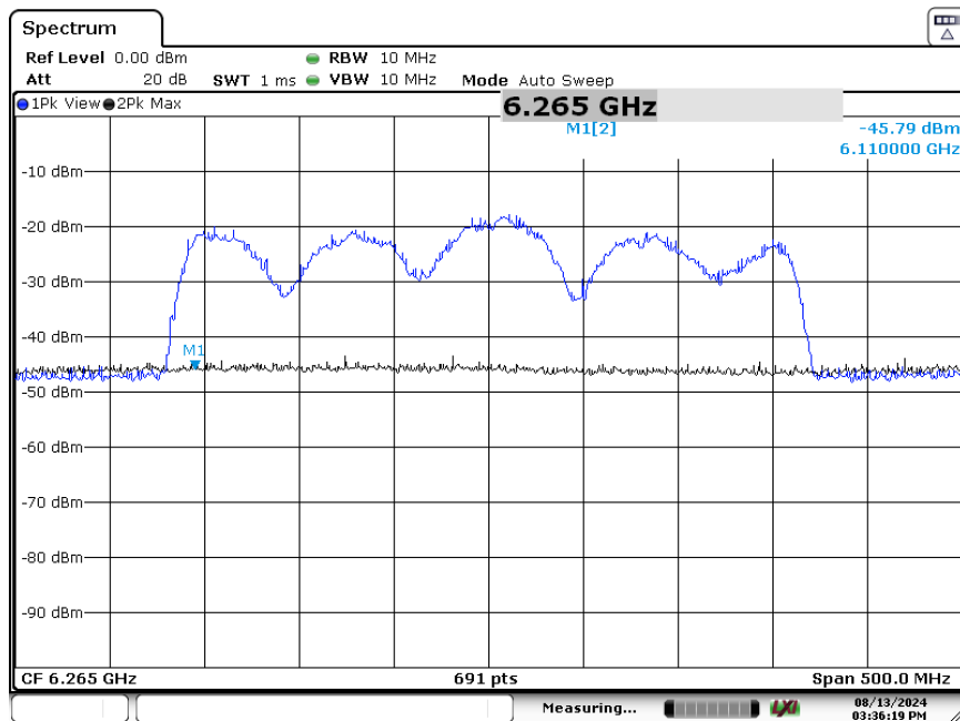
Plot 7-352. CBP 320MHz Channel - Injection Lower Edge – [6110 MHz]
