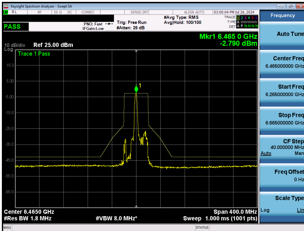
Plot 7-287. In Band Emissions Plot MIMO ANT2 (80MHz BW 802.11ax/be (26 Tones) (UNII Band 6) – Ch. 103)
