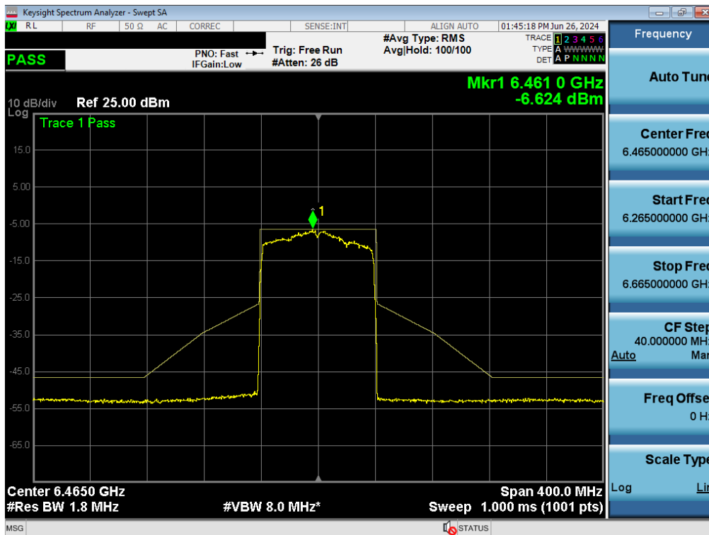
Plot 7-307. In Band Emissions Plot MIMO ANT2 (80MHz BW 802.11ax/be (Full Tones) (UNII Band 6) – Ch. 103)
