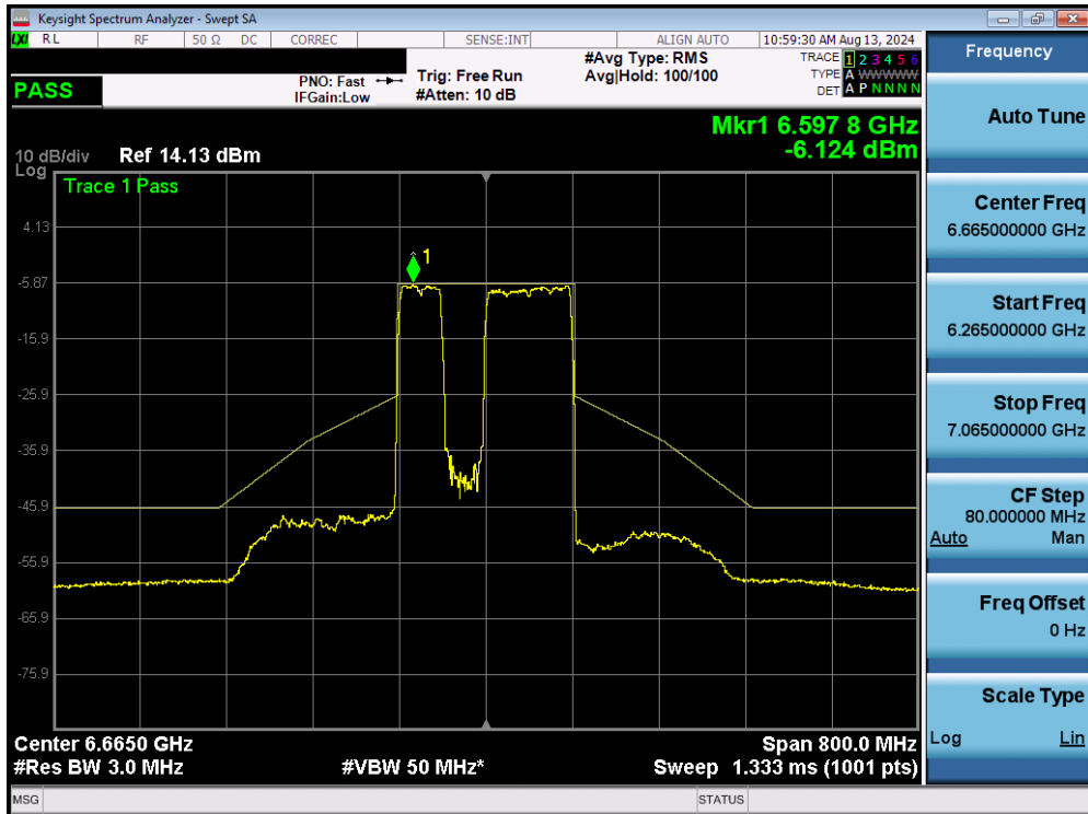
Plot 7-329. In Band Emissions MIMO ANT2 (160MHz BW 802.11be (996+484 Tones) (UNII Band 7) – Ch. 143)
