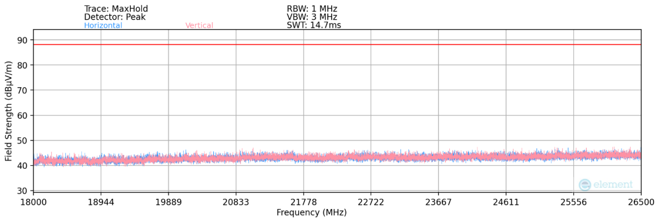
Plot 7-359. Radiated Spurious Plot 18GHz - 26.5GHz (802.11ax)
