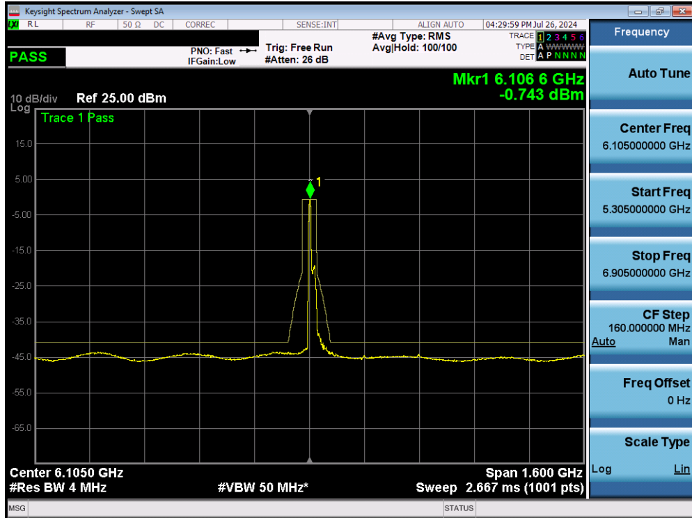
Plot 7-284. In Band Emissions Plot MIMO ANT2 (320MHz BW 802.11be (26 Tones) (UNII Band 5) – Ch. 31)
