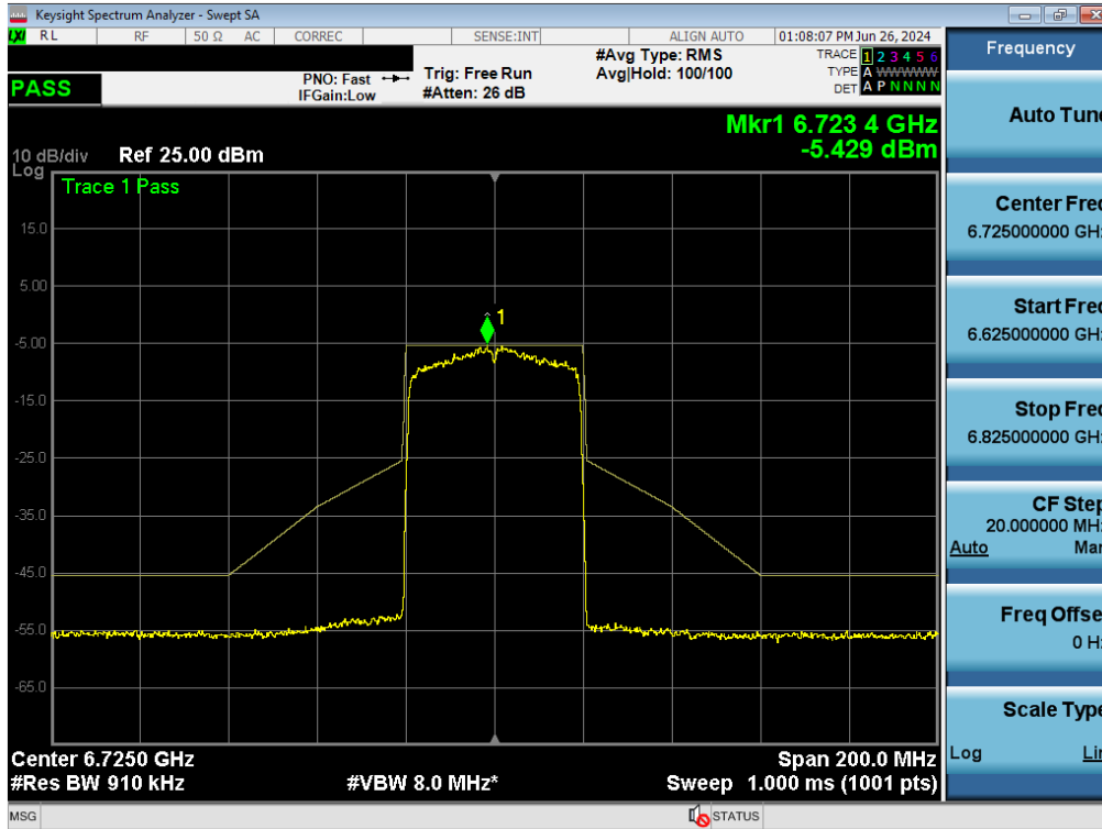
Plot 7-310. In Band Emissions Plot MIMO ANT2 (40MHz BW 802.11ax/be (Full Tones) (UNII Band 7) – Ch. 155)
