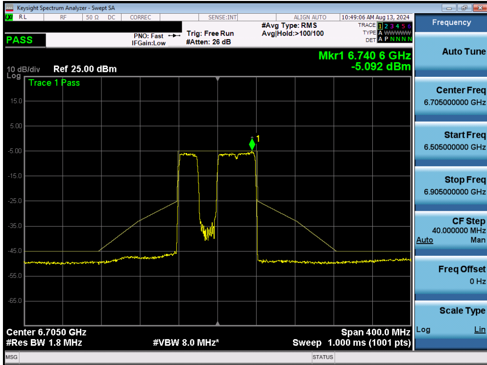
Plot 7-328. In Band Emissions MIMO ANT2 (80MHz BW 802.11be (484+242 Tones) (UNII Band 7) – Ch. 151)
