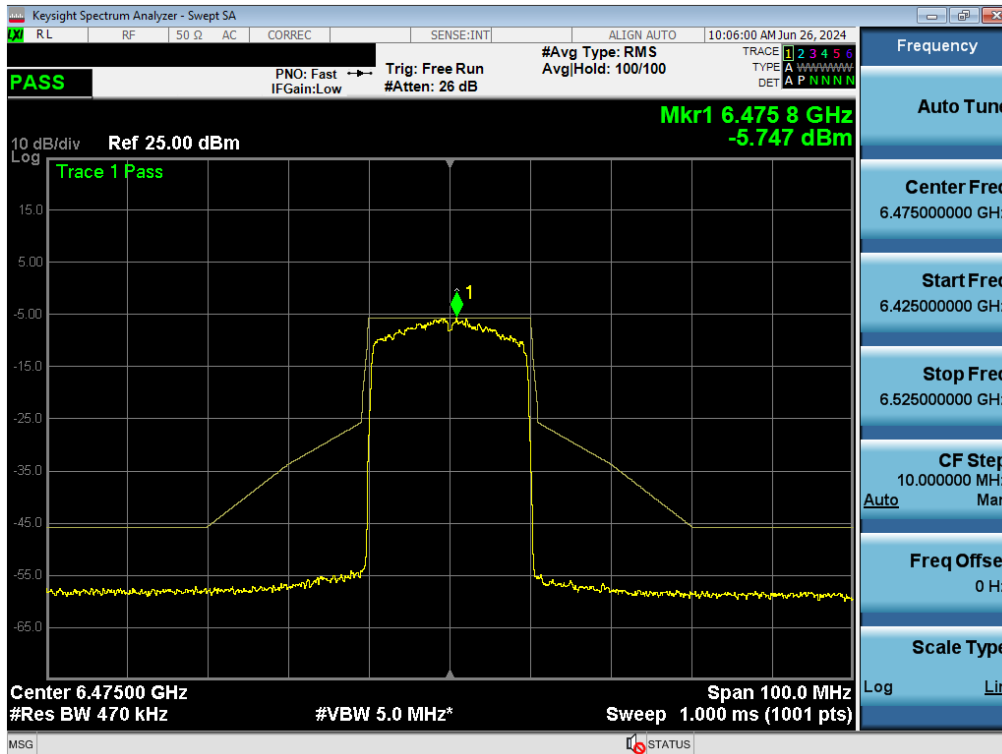
Plot 7-305. In Band Emissions Plot MIMO ANT2 (20MHz BW 802.11ax/be (Full Tones) (UNII Band 6) – Ch. 105)
