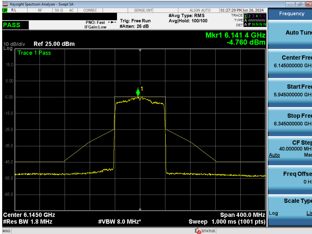
Plot 7-302. In Band Emissions Plot MIMO ANT2 (80MHz BW 802.11ax/be (Full Tones) (UNII Band 5) – Ch. 39)
