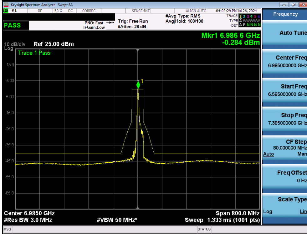
Plot 7-298. In Band Emissions Plot MIMO ANT2 (160MHz BW 802.11ax/be (26 Tones) (UNII Band 8) – Ch. 207
