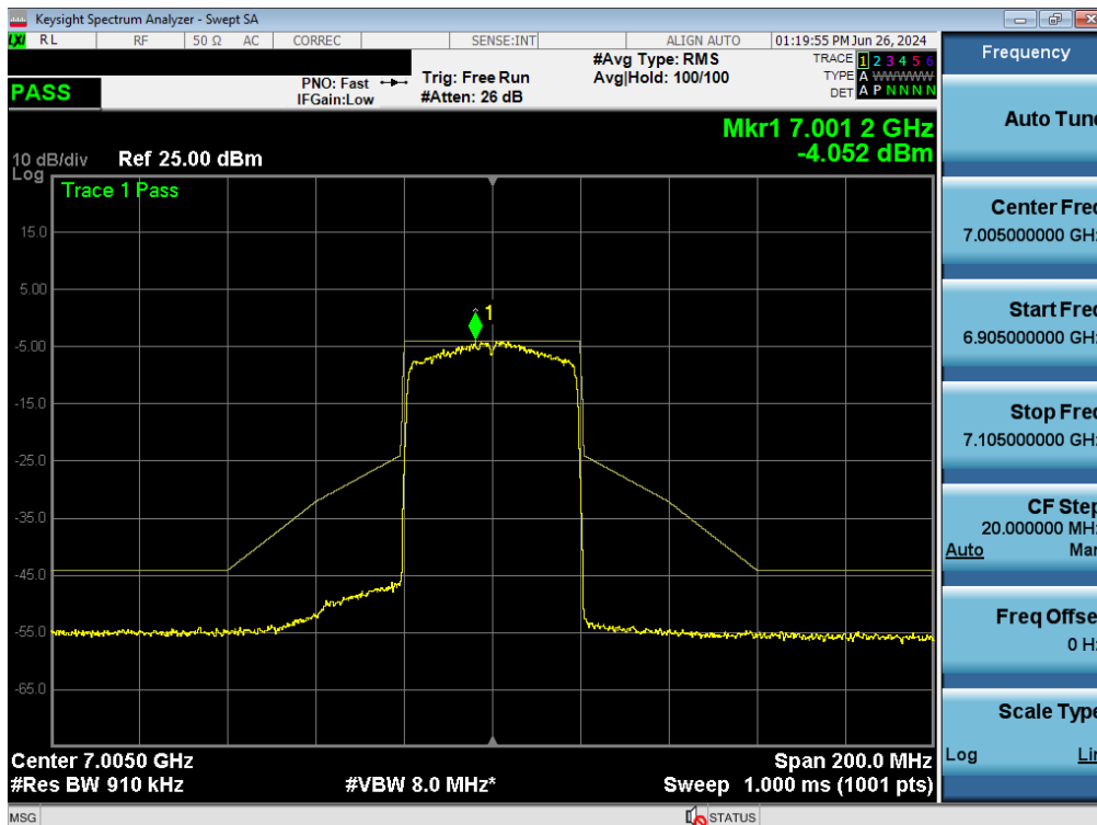
Plot 7-315. In Band Emissions Plot MIMO ANT2 (40MHz BW 802.11ax/be (Full Tones) (UNII Band 8) – Ch. 211)
