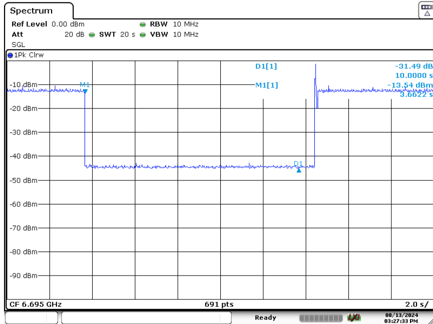
Plot 7-344. Contention Based Protocol Timing Plot (20MHz (UNII Band 7) – Ch. 149)
