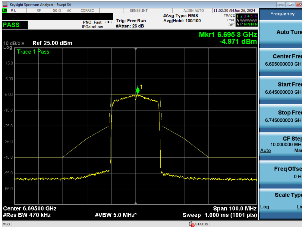
Plot 7-309. In Band Emissions Plot MIMO ANT2 (20MHz BW 802.11ax/be (Full Tones) (UNII Band 7) – Ch. 149)
