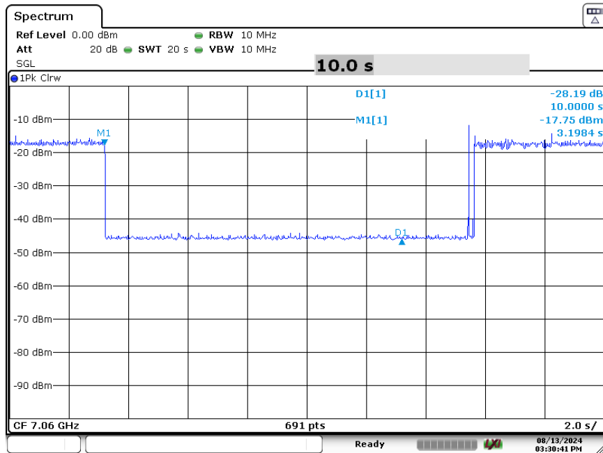
Plot 7-350. Contention Based Protocol Timing Plot (320MHz (UNII Band 8) – Ch. 191 Mid)
