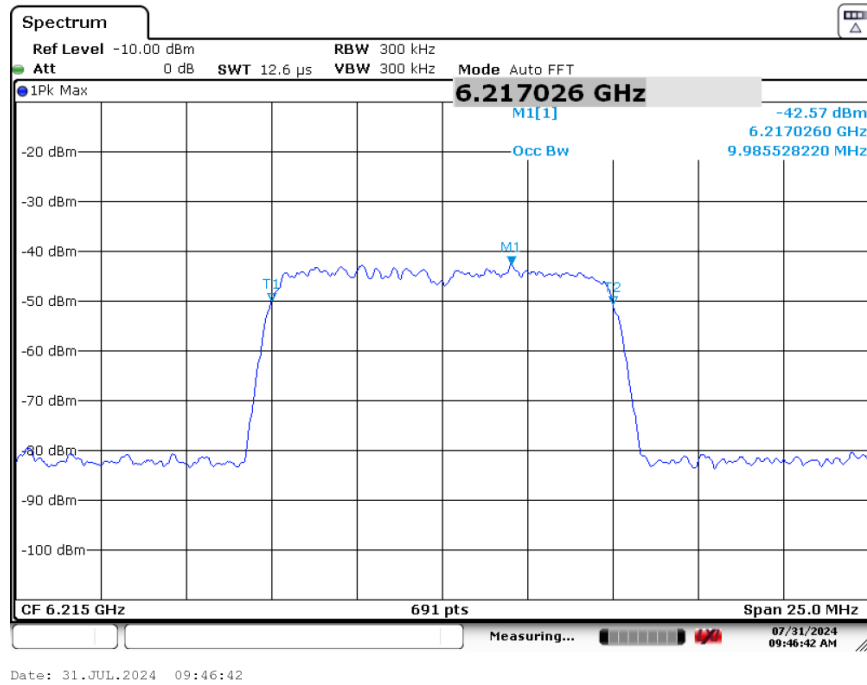
Plot 7-335. AWGN Signal (Demonstration)
