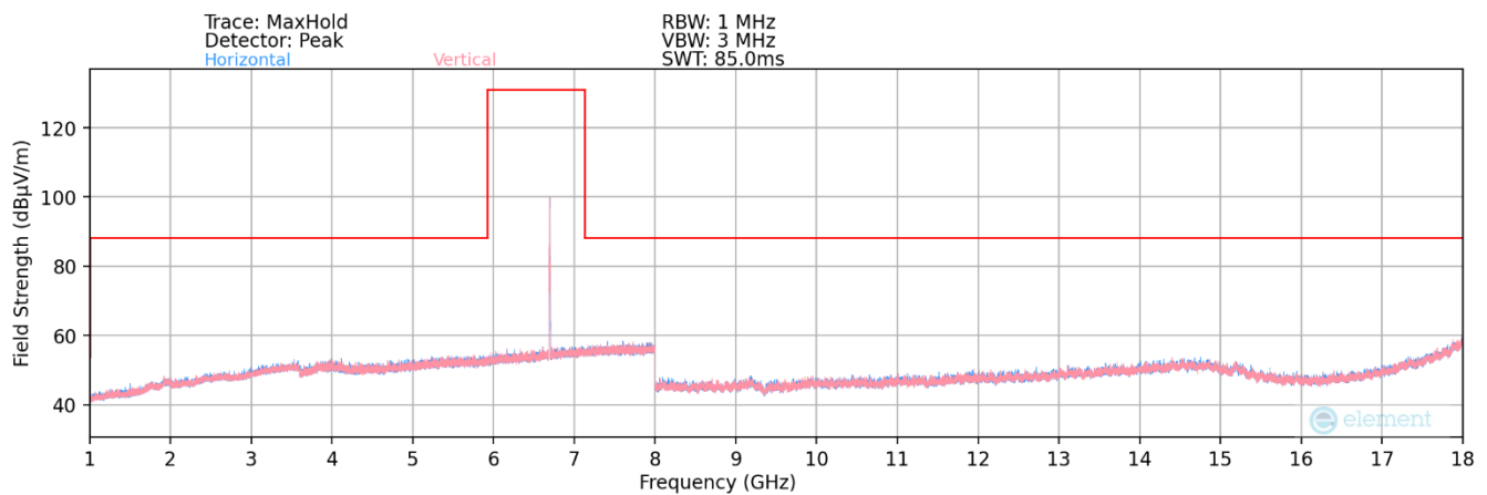
Plot 7-357. Radiated Spurious Plot 1GHz – 18GHz MIMO (802.11ax – UNII Band 7 Ch. 149)
