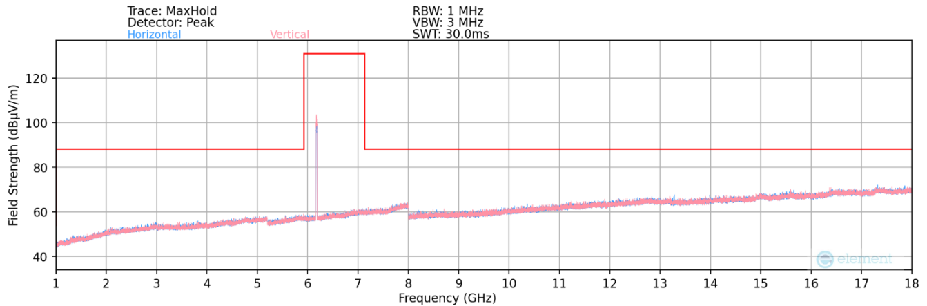
Plot 7-361. Radiated Spurious Plot 1GHz – 18GHz MIMO (802.11ax – UNII Band 5 Ch. 45)
