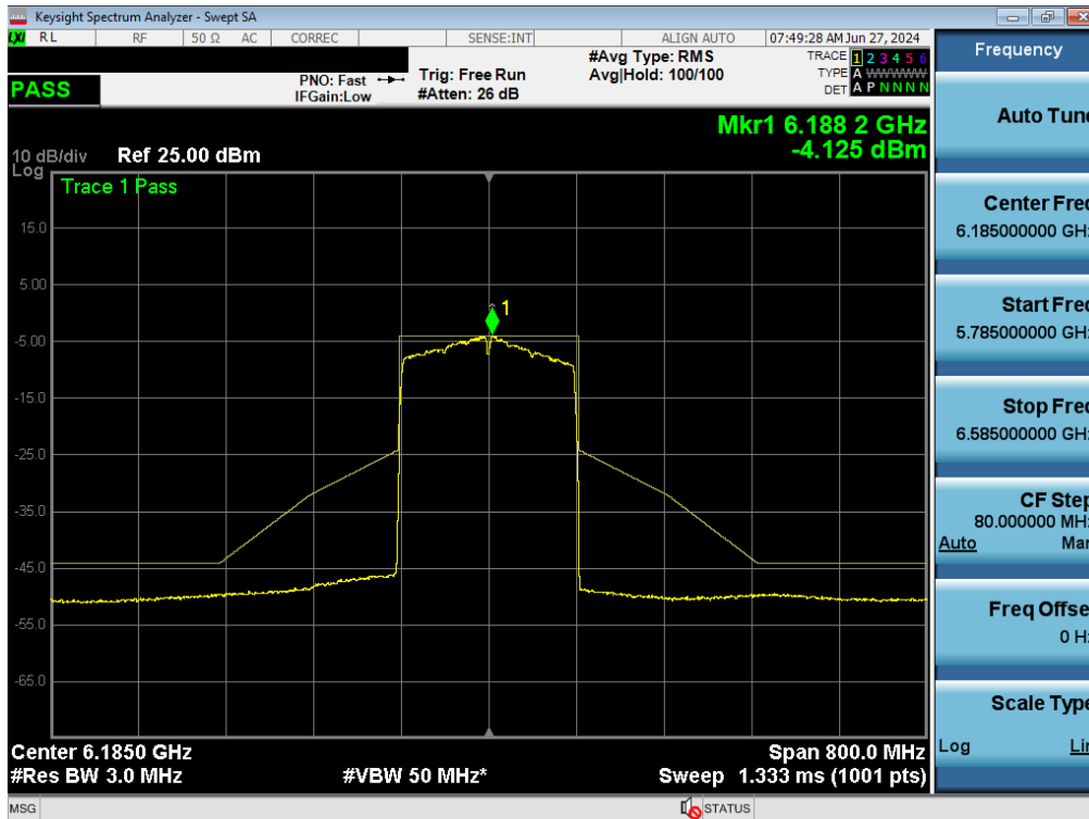
Plot 7-303. In Band Emissions Plot MIMO ANT2 (160MHz BW 802.11ax/be (Full Tones) (UNII Band 5) – Ch. 47)
