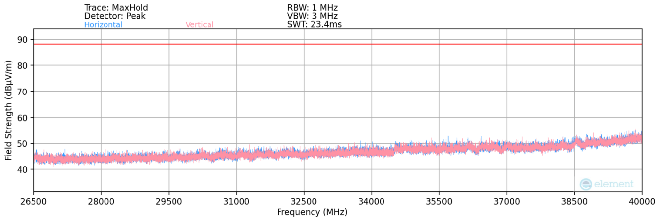
Plot 7-360. Radiated Spurious Plot 26.5GHz - 40GHz (802.11ax)
