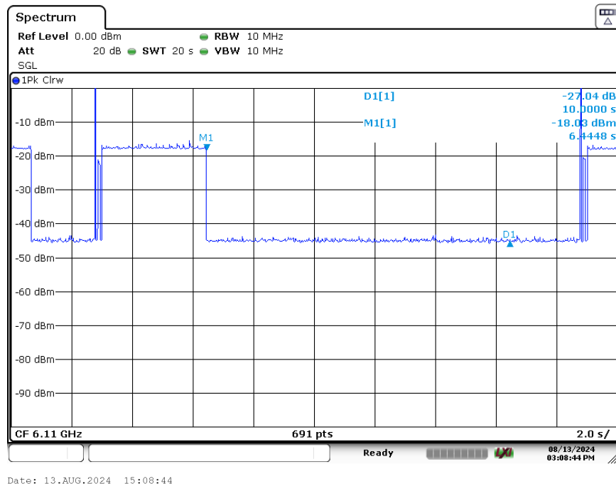
Plot 7-337. Contention Based Protocol Timing Plot (320MHz (UNII Band 5) – Ch. 31 Low)
