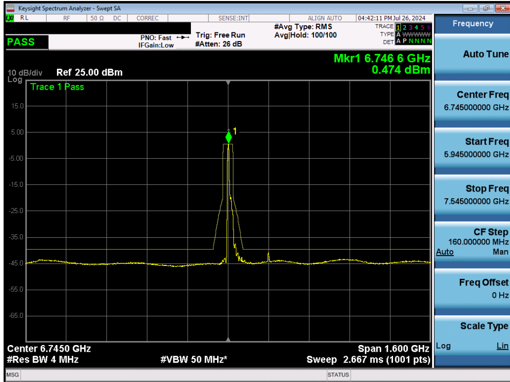
Plot 7-294. In Band Emissions Plot MIMO ANT2 (320MHz BW 802.11be (26 Tones) (UNII Band 7) – Ch. 159)
