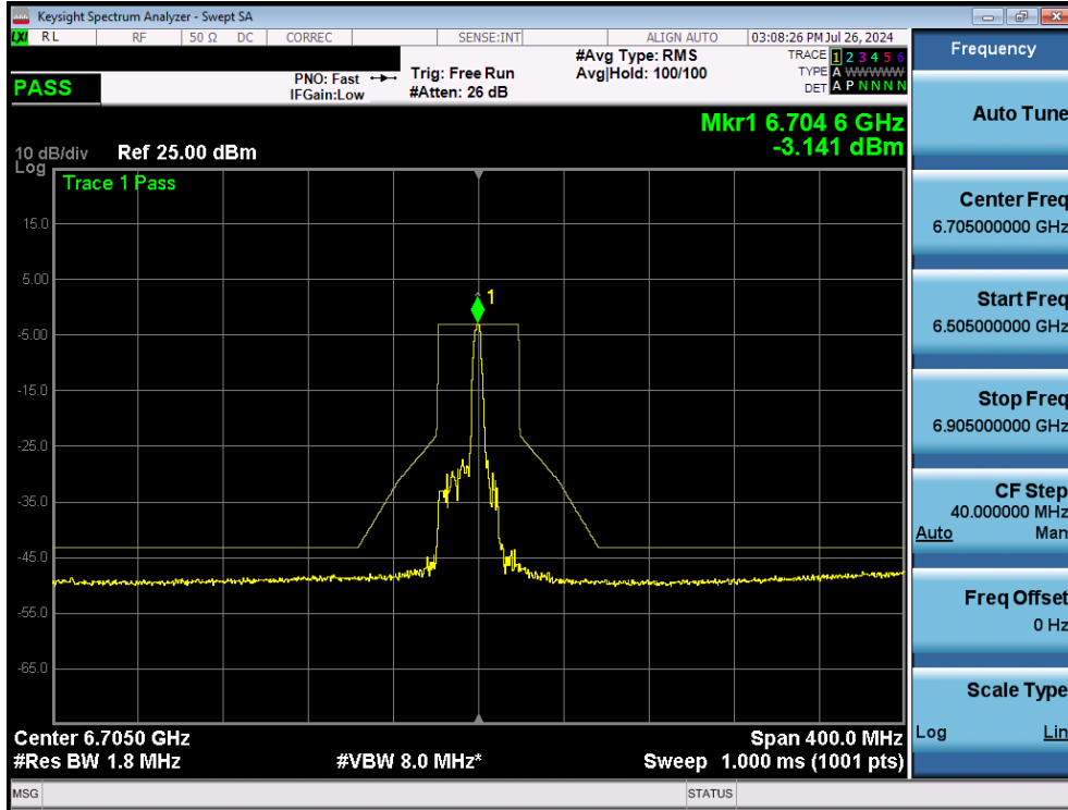
Plot 7-292. In Band Emissions Plot MIMO ANT2 (80MHz BW 802.11ax/be (26 Tones) (UNII Band 7) – Ch. 151)
