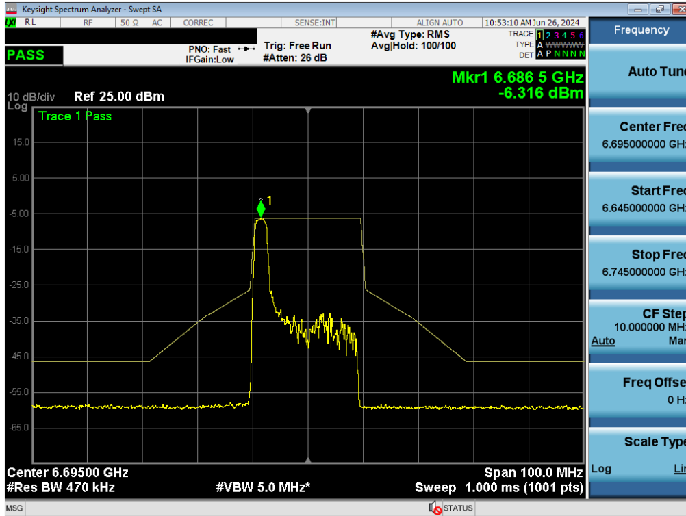
Plot 7-290. In Band Emissions Plot MIMO ANT2 (20MHz BW 802.11ax/be (26 Tones) (UNII Band 7) – Ch. 149)
