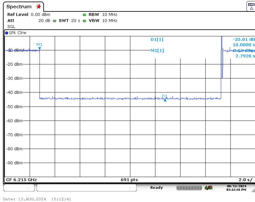
Plot 7-336. Contention Based Protocol Timing Plot (20MHz (UNII Band 5) – Ch. 53)
