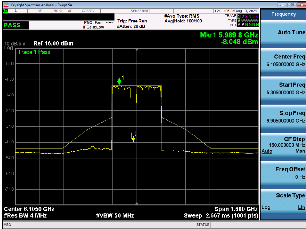
Plot 7-322. In Band Emissions MIMO ANT2 (320MHz BW 802.11be (2*996+484 Tones) (UNII Band 5) – Ch. 31)
