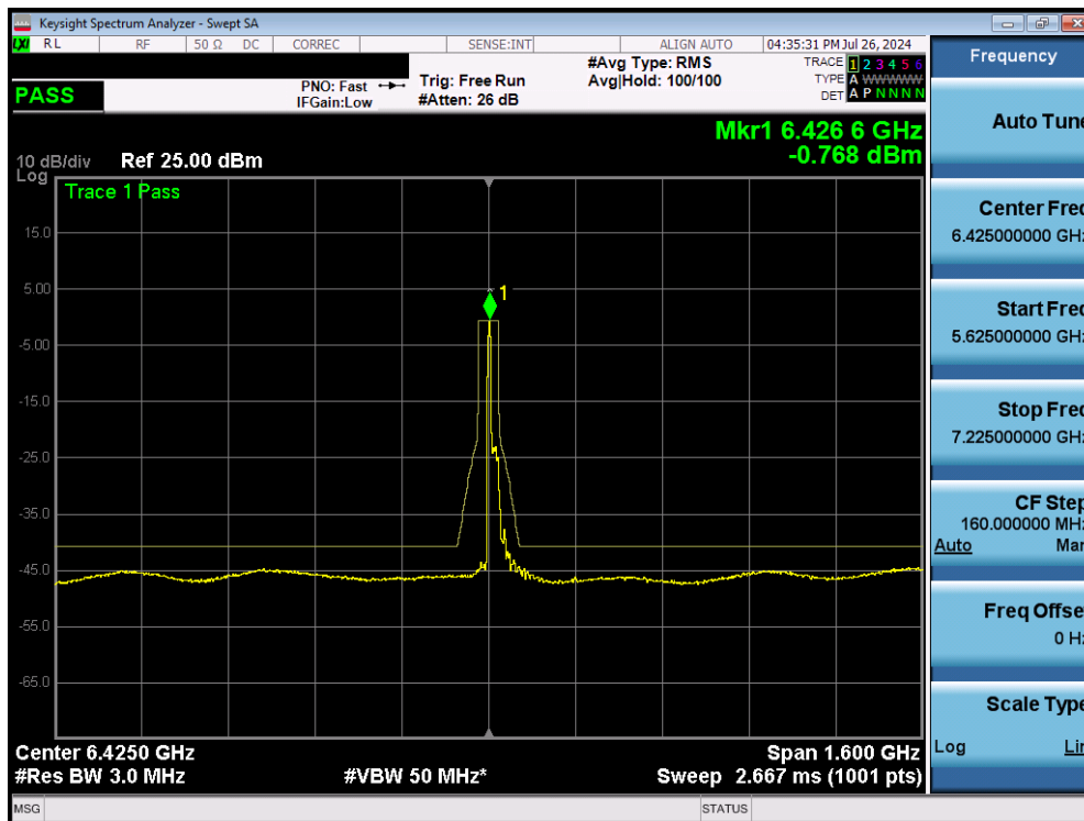
Plot 7-289. In Band Emissions Plot MIMO ANT2 (320MHz BW 802.11be (26 Tones) (UNII Band 6) – Ch. 95)
