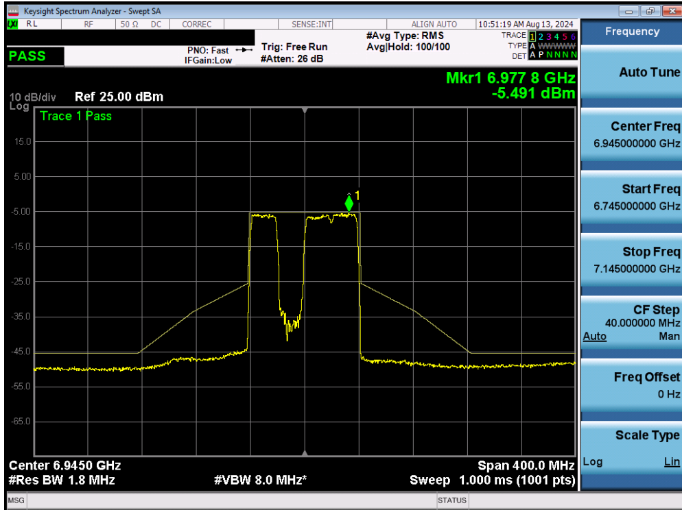
Plot 7-332. In Band Emissions MIMO ANT2 (80MHz BW 802.11be (484+242 Tones) (UNII Band 8) – Ch. 199)
