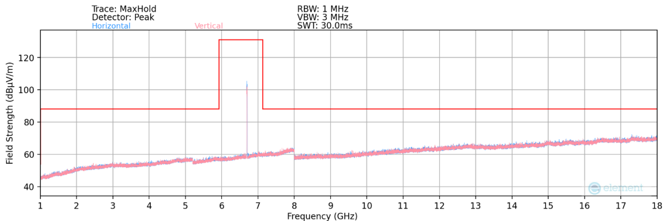
Plot 7-363. Radiated Spurious Plot 1GHz – 18GHz MIMO (802.11ax – UNII Band 7 Ch. 149)
