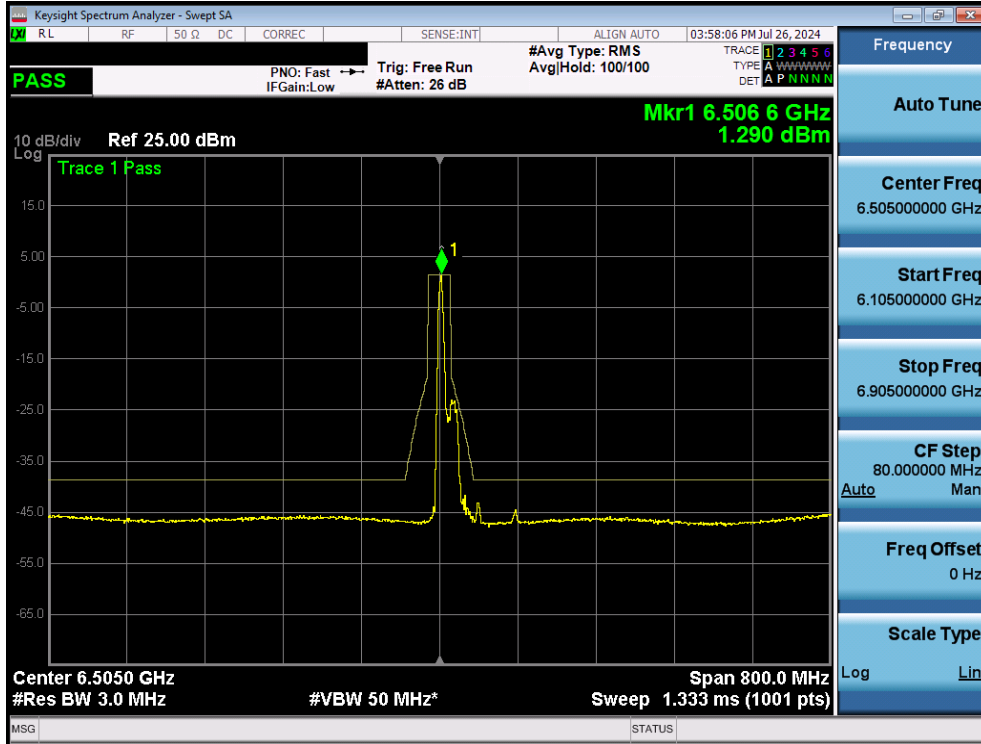
Plot 7-288. In Band Emissions Plot MIMO ANT2 (160MHz BW 802.11 ax/be (26 Tones) (UNII Band 6) – Ch. 111)
