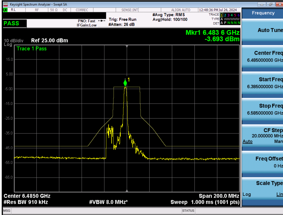
Plot 7-286. In Band Emissions Plot MIMO ANT2 (40MHz BW 802.11ax/be (26 Tones) (UNII Band 6) – Ch. 107)
