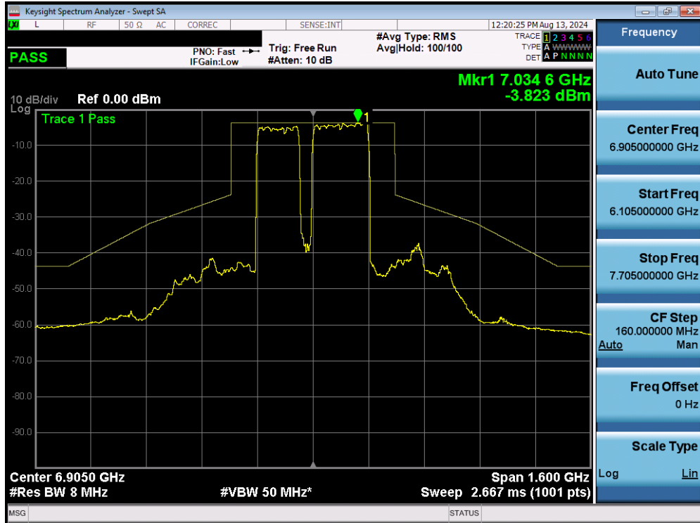
Plot 7-334. In Band Emissions MIMO ANT2 (320MHz BW 802.11be (2*996+484 Tones) (UNII Band 8) – Ch. 191)
