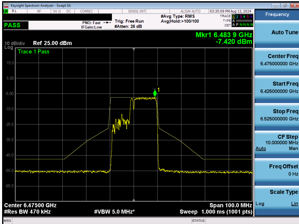
Plot 7-323. In Band Emissions MIMO ANT2 (20MHz BW 802.11be (106+26 Tones) (UNII Band 6) – Ch. 105)
