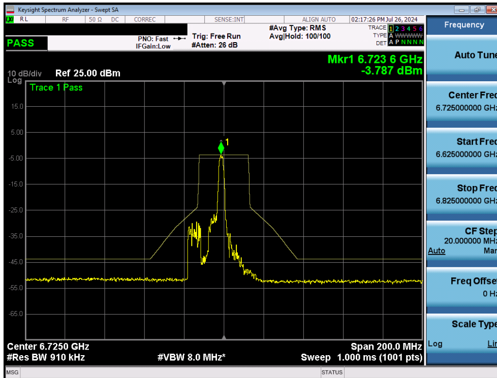
Plot 7-291. In Band Emissions Plot MIMO ANT2 (40MHz BW 802.11ax/be (26 Tones) (UNII Band 7) – Ch. 155)
