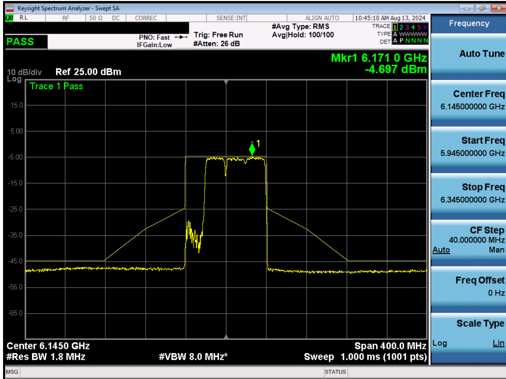
Plot 7-320. In Band Emissions MIMO ANT2 (80MHz BW 802.11be (484+242 Tones) (UNII Band 5) – Ch. 39)
