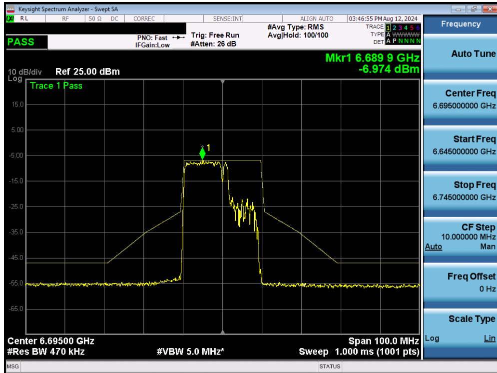
Plot 7-327. In Band Emissions MIMO ANT2 (20MHz BW 802.11be (106+26 Tones) (UNII Band 7) – Ch. 149)
