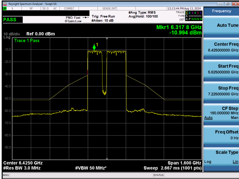
Plot 7-326. In Band Emissions MIMO ANT2 (320MHz BW 802.11be (2*996+484 Tones) (UNII Band 6) – Ch. 95)
