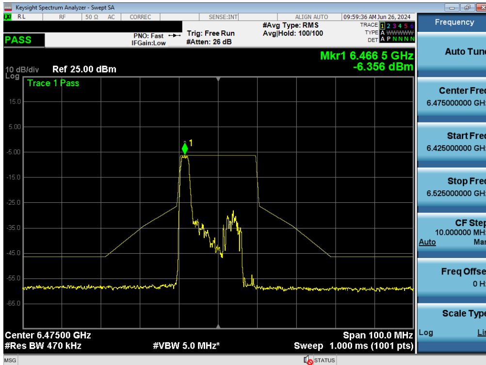
Plot 7-285. In Band Emissions Plot MIMO ANT2 (20MHz BW 802.11ax/be (26 Tones) (UNII Band 6) – Ch. 105)
