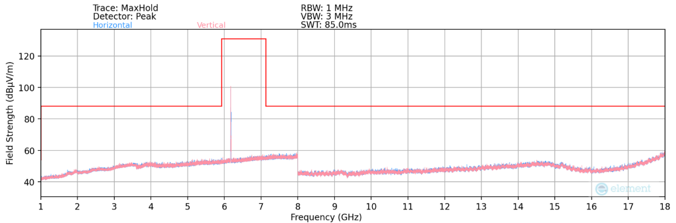
Plot 7-355. Radiated Spurious Plot 1GHz – 18GHz MIMO (802.11ax – UNII Band 5 Ch. 45)
