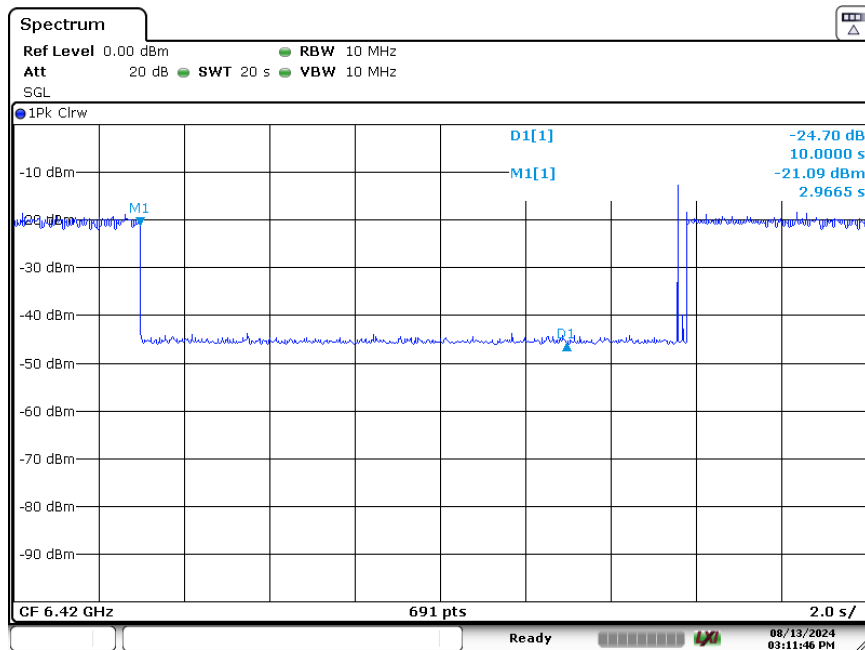
Plot 7-339. Contention Based Protocol Timing Plot (320MHz (UNII Band 5) – Ch. 31 High)
