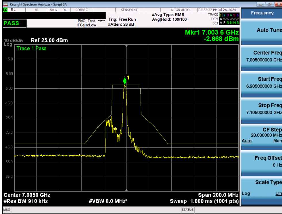
Plot 7-296. In Band Emissions Plot MIMO ANT2 (40MHz BW 802.11ax/be (26 Tones) (UNII Band 8) – Ch. 211)
