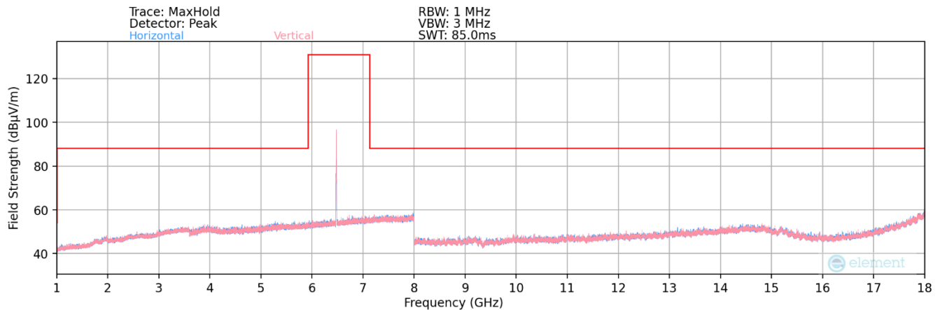
Plot 7-356. Radiated Spurious Plot 1GHz – 18GHz MIMO (802.11ax – UNII Band 6 Ch. 105)
