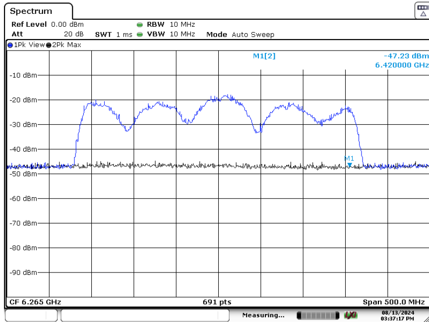
Plot 7-354. CBP 320MHz Channel - Injection Upper Edge – [6420 MHz]
