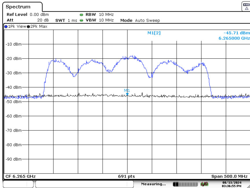
Plot 7-353. CBP 320MHz Channel - Injection Center – [6265 MHz]
