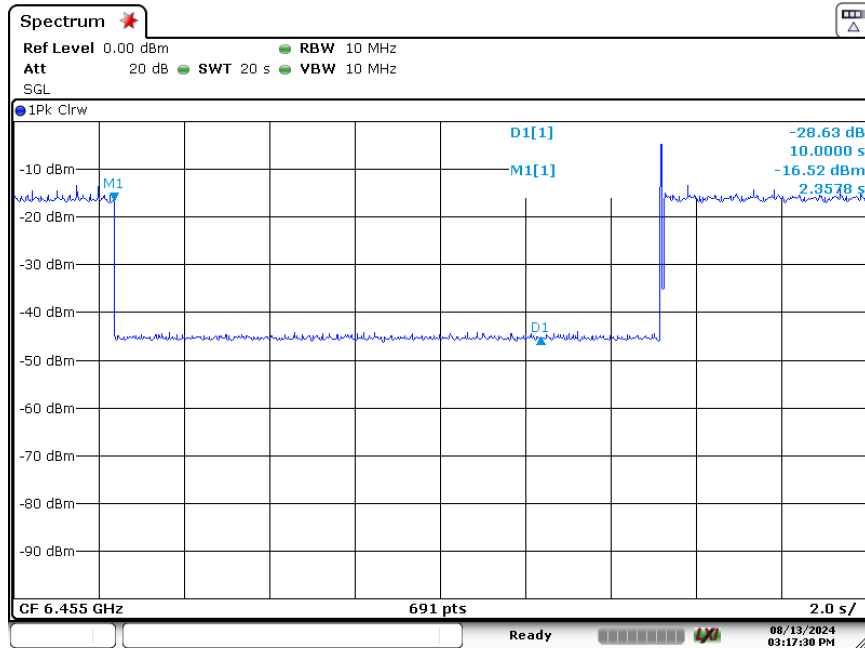
Plot 7-340. Contention Based Protocol Timing Plot (20MHz (UNII Band 6) – Ch. 101)
