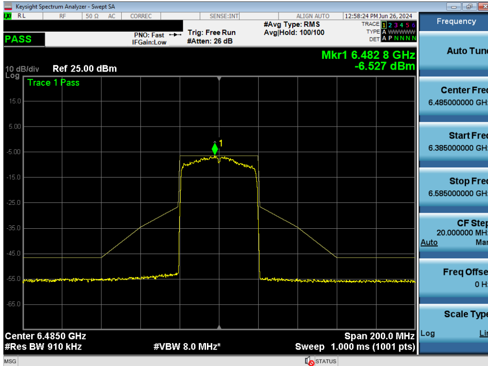
Plot 7-306. In Band Emissions Plot MIMO ANT2 (40MHz BW 802.11ax/be (Full Tones) (UNII Band 6) – Ch. 107)
