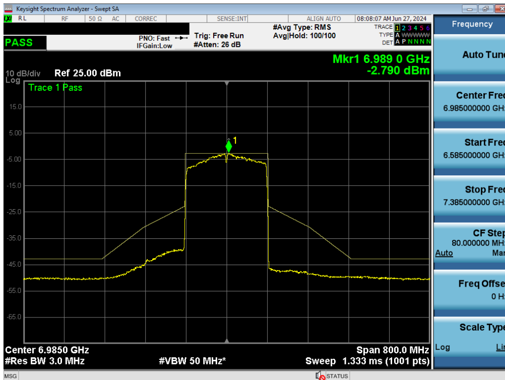
Plot 7-317. In Band Emissions Plot MIMO ANT2 (160MHz BW 802.11ax/be (Full Tones) (UNII Band 8) – Ch. 207)
