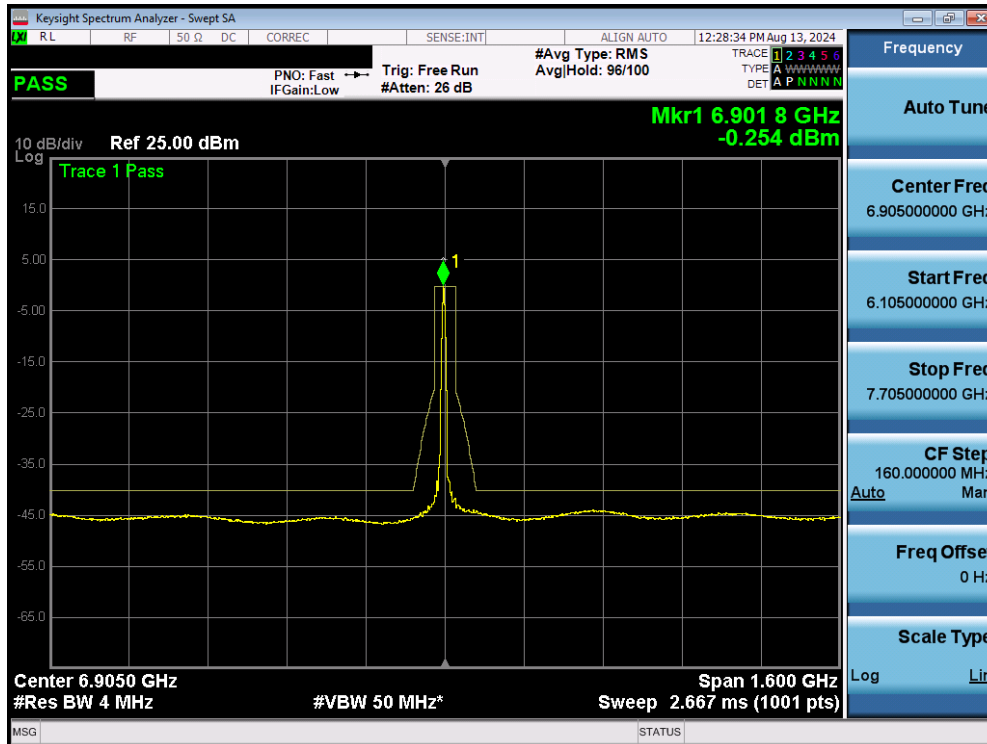
Plot 7-299. In Band Emissions Plot MIMO ANT2 (320MHz BW 802.11be (26 Tones) (UNII Band 8) – Ch. 191)
