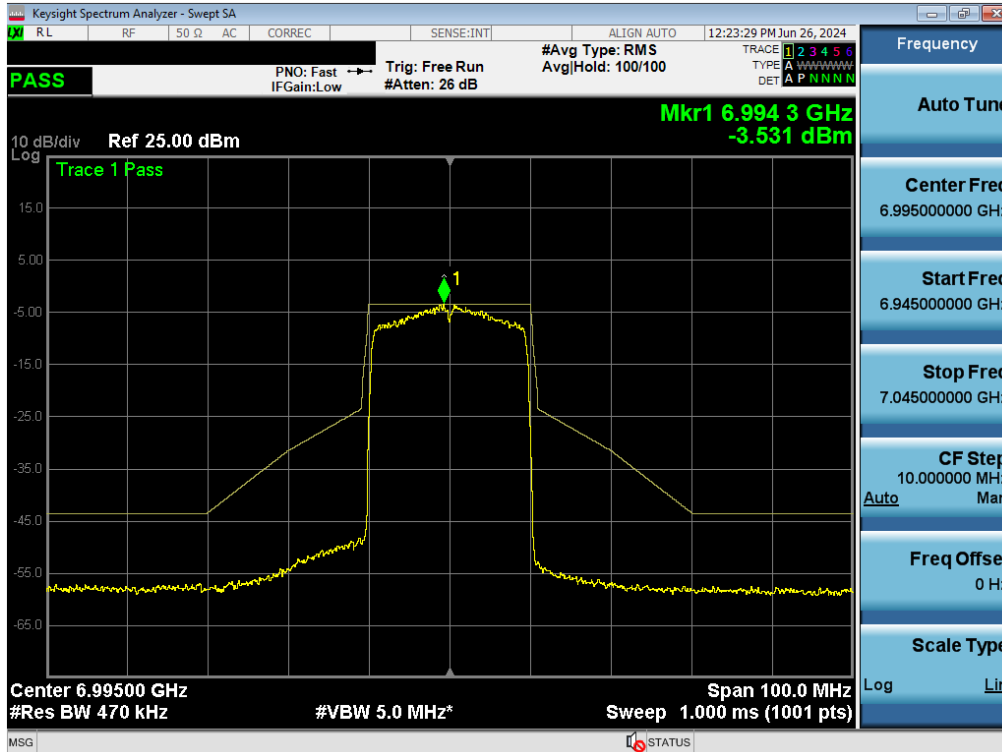
Plot 7-314. In Band Emissions Plot MIMO ANT2 (20MHz BW 802.11ax/be (Full Tones) (UNII Band 8) – Ch. 209)
