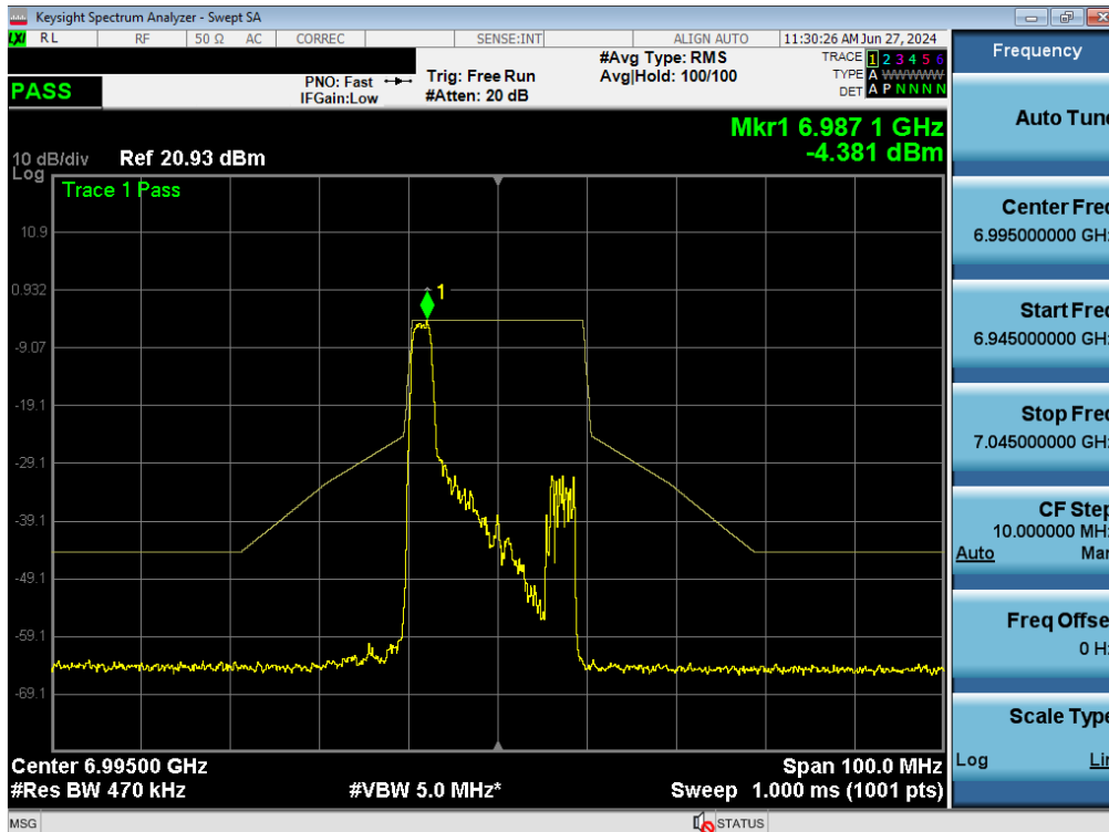
Plot 7-295. In Band Emissions Plot MIMO ANT2 (20MHz BW 802.11ax/be (26 Tones) (UNII Band 8) – Ch. 209)
