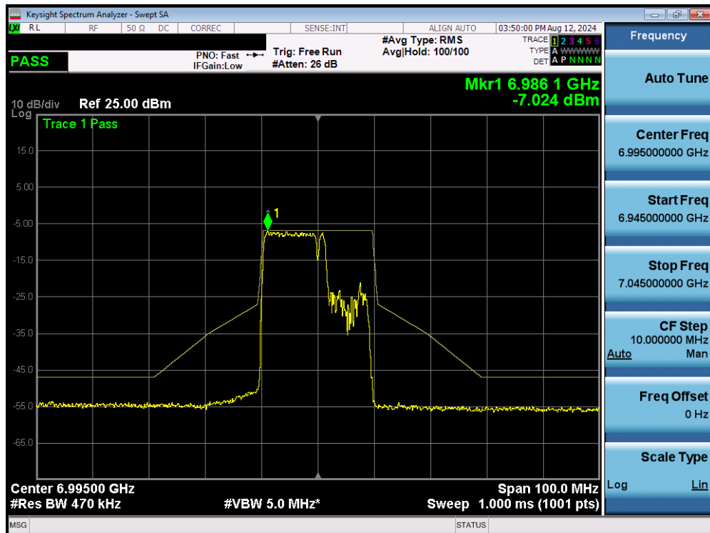
Plot 7-331. In Band Emissions MIMO ANT2 (20MHz BW 802.11be (106+26 Tones) (UNII Band 8) – Ch. 209)
