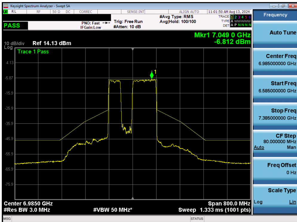
Plot 7-333. In Band Emissions MIMO ANT2 (160MHz BW 802.11be (996+484 Tones) (UNII Band 8) – Ch. 207)
