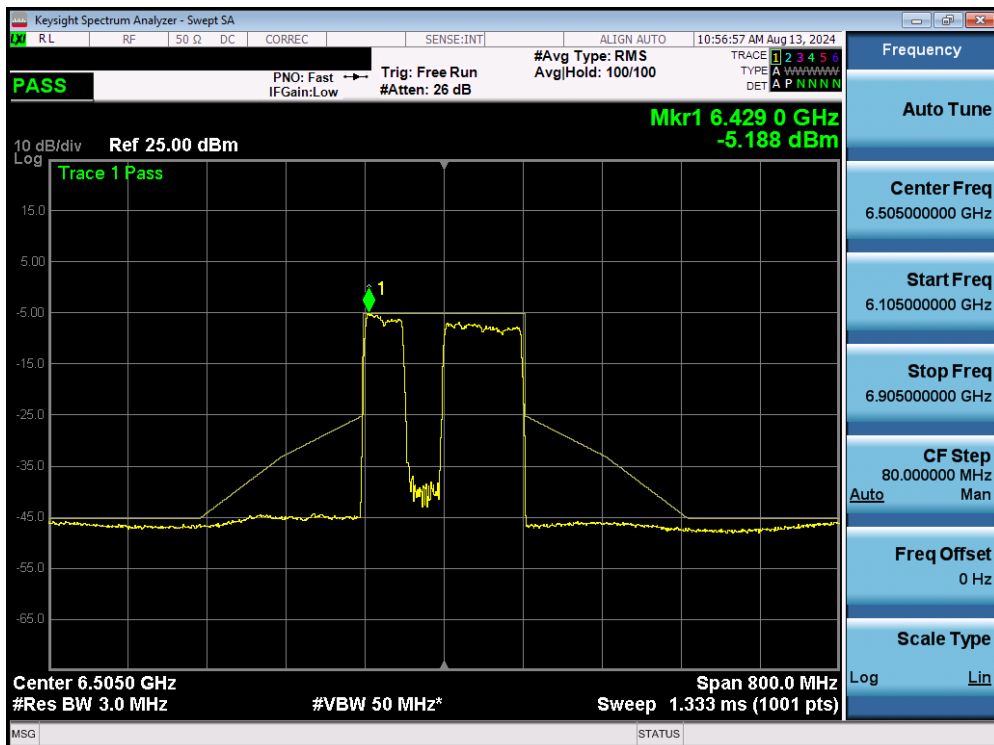
Plot 7-325. In Band Emissions MIMO ANT2 (160MHz BW 802.11be (996+484 Tones) (UNII Band 6) – Ch. 111)
