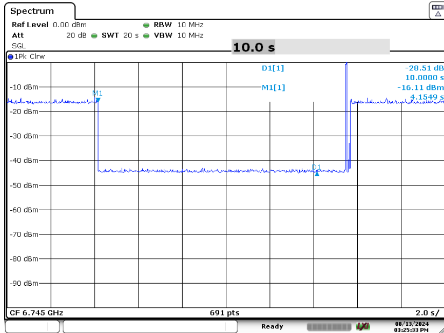
Plot 7-346. Contention Based Protocol Timing Plot (320MHz (UNII Band 7) – Ch. 159 Mid)
