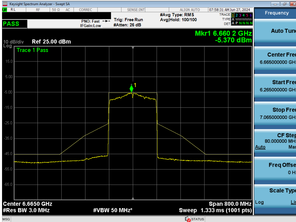
Plot 7-312. In Band Emissions Plot MIMO ANT2 (160MHz BW 802.11ax/be (Full Tones) (UNII Band 7) – Ch. 143)
