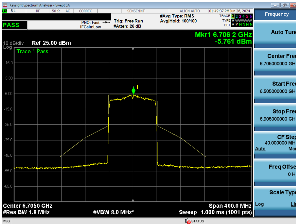
Plot 7-311. In Band Emissions Plot MIMO ANT2 (80MHz BW 802.11ax/be (Full Tones) (UNII Band 7) – Ch. 151)
