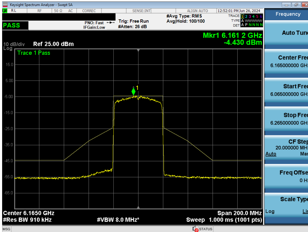
Plot 7-301. In Band Emissions Plot MIMO ANT2 (40MHz BW 802.11ax/be (Full Tones) (UNII Band 5) – Ch. 43)
