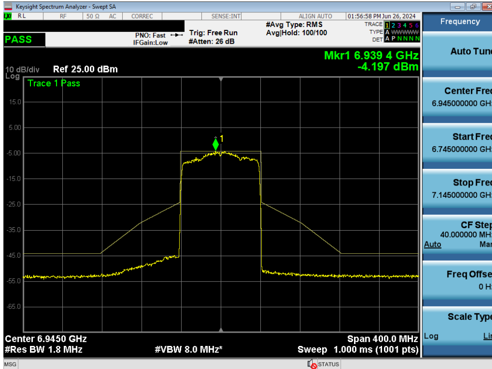
Plot 7-316. In Band Emissions Plot MIMO ANT2 (80MHz BW 802.11ax/be (Full Tones) (UNII Band 8) – Ch. 199)
