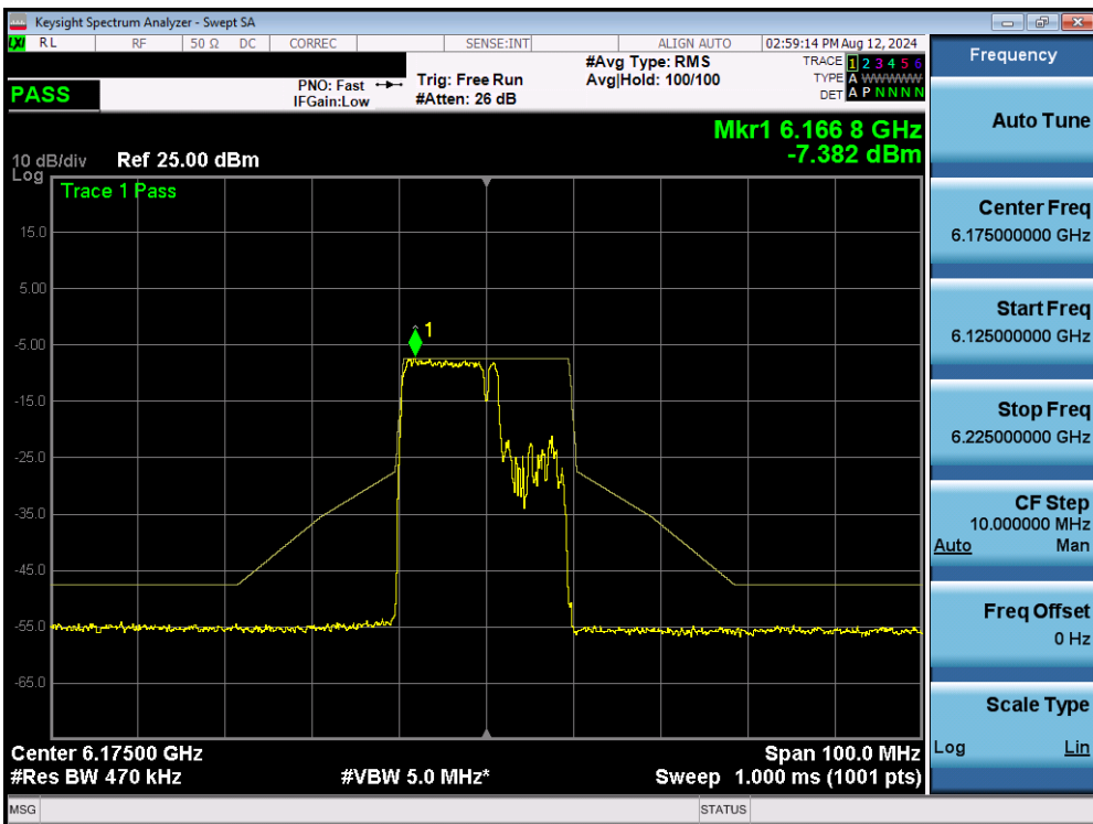
Plot 7-319. In Band Emissions MIMO ANT2 (20MHz BW 802.11be (106+26 Tones) (UNII Band 5) – Ch. 45)
