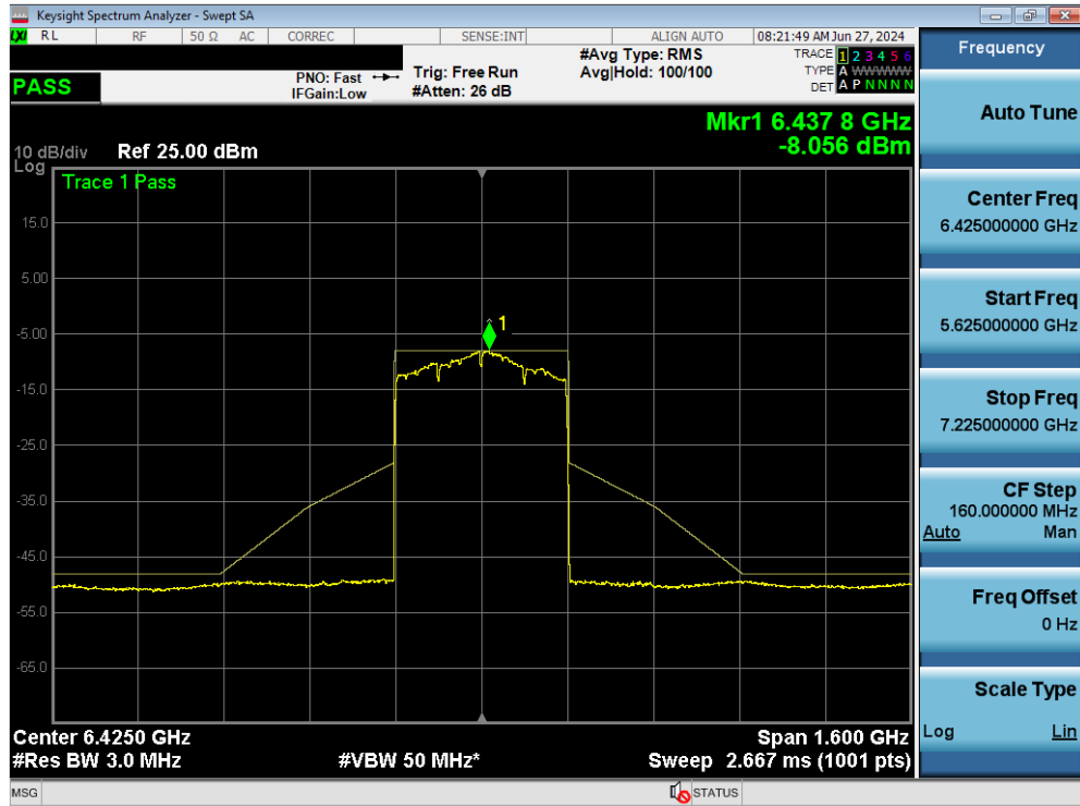
Plot 7-308. In Band Emissions Plot MIMO ANT2 (320MHz BW 802.11be (Full Tones) (UNII Band 6) – Ch. 95)
