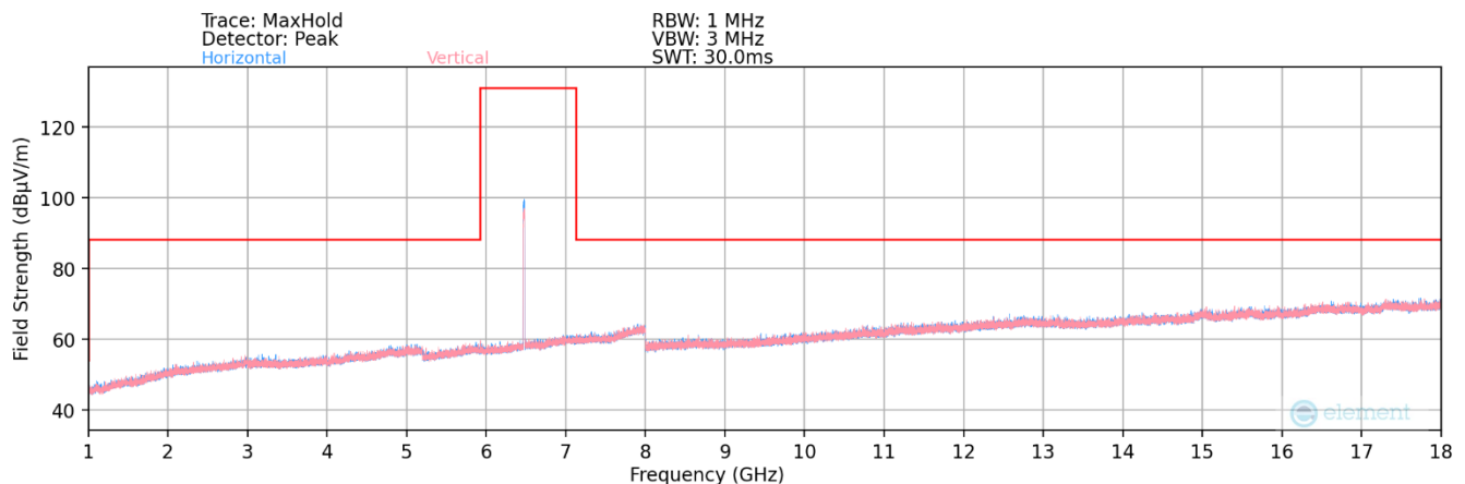
Plot 7-362. Radiated Spurious Plot 1GHz – 18GHz MIMO (802.11ax – UNII Band 6 Ch. 105)
