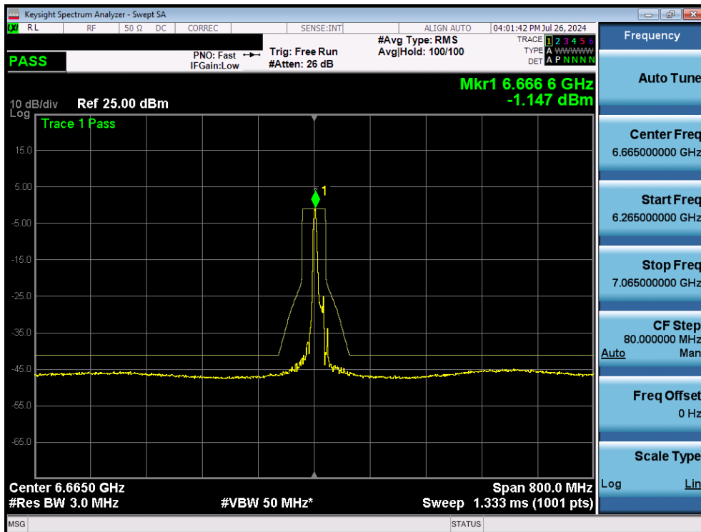
Plot 7-293. In Band Emissions Plot MIMO ANT2 (160MHz BW 802.11ax/be (26 Tones) (UNII Band 7) – Ch. 143)
