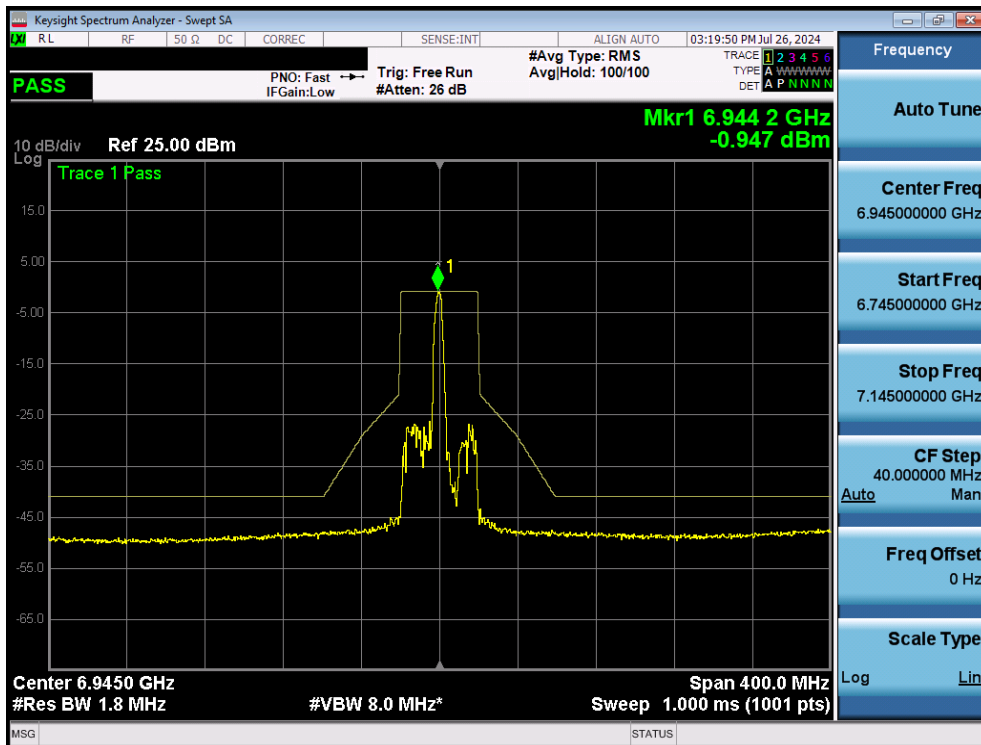
Plot 7-297. In Band Emissions Plot MIMO ANT2 (80MHz BW 802.11ax/be (26 Tones) (UNII Band 8) – Ch. 199)
