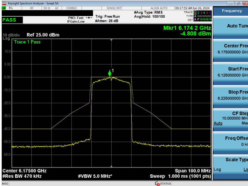
Plot 7-300. In Band Emissions Plot MIMO ANT2 (20MHz BW 802.11ax/be (Full Tones) (UNII Band 5) – Ch. 45)
