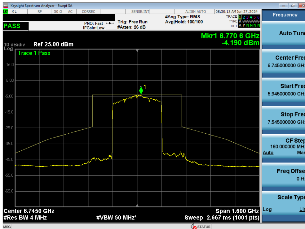
Plot 7-313. In Band Emissions Plot MIMO ANT2 (320MHz BW 802.11be (Full Tones) (UNII Band 7) – Ch. 159)
