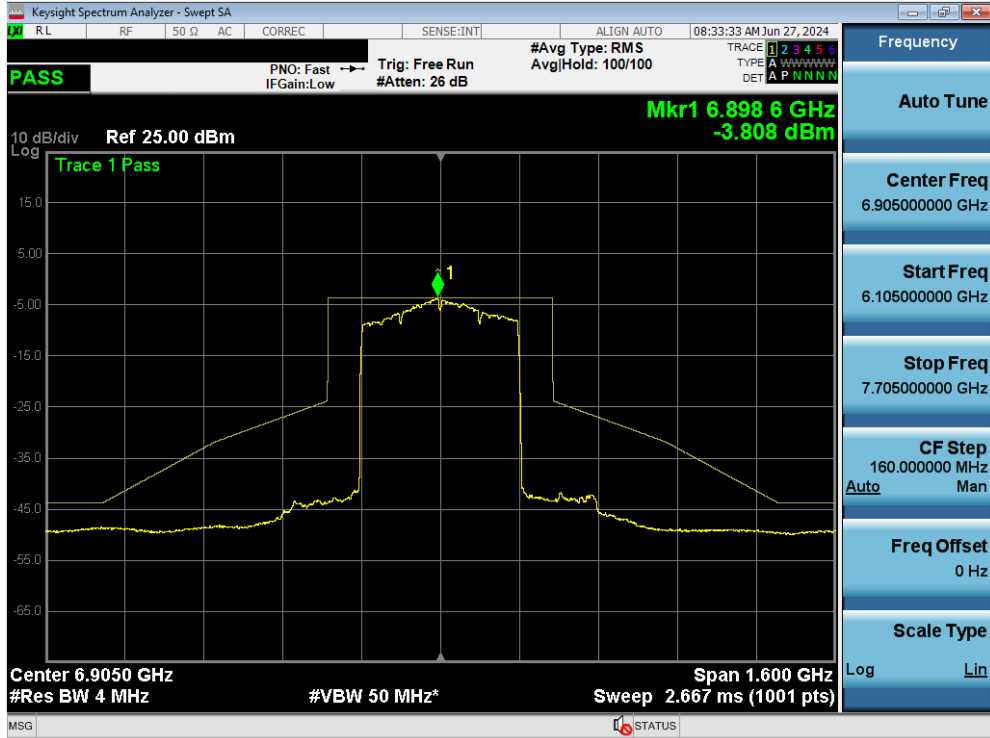
Plot 7-318. In Band Emissions Plot MIMO ANT2 (320MHz BW 802.11be (Full Tones) (UNII Band 8) – Ch. 191)
