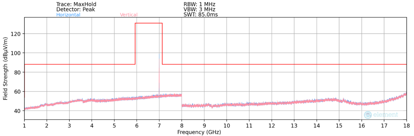
Plot 7-358. Radiated Spurious Plot 1GHz – 18GHz MIMO (802.11ax – UNII Band 8 Ch. 209)
