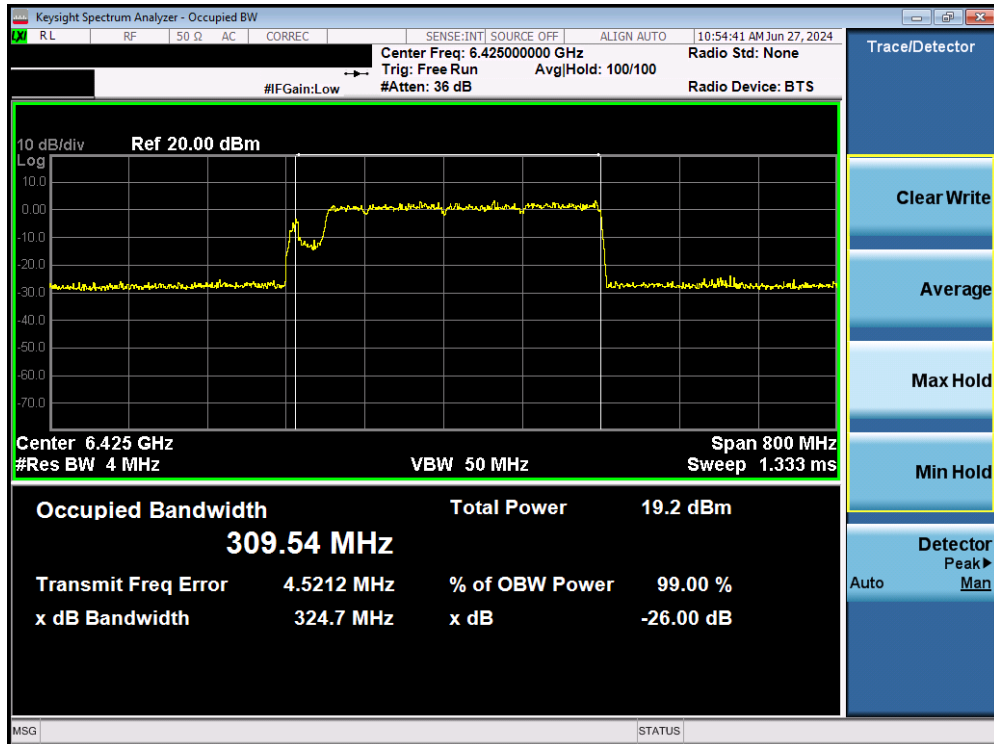
Plot 7-48. Occupied Bandwidth Plot MIMO ANT1 (320MHz BW 802.11be (3*996+484 Tones) (UNII Band 6) – Ch. 95)
