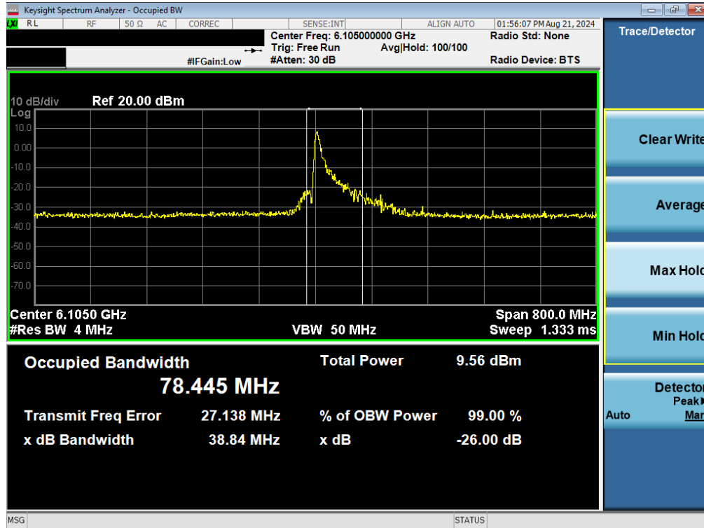
Plot 7-61. Occupied Bandwidth Plot MIMO ANT2 (320MHz BW 802.11be (26 Tones) (UNII Band 5) – Ch. 31)
