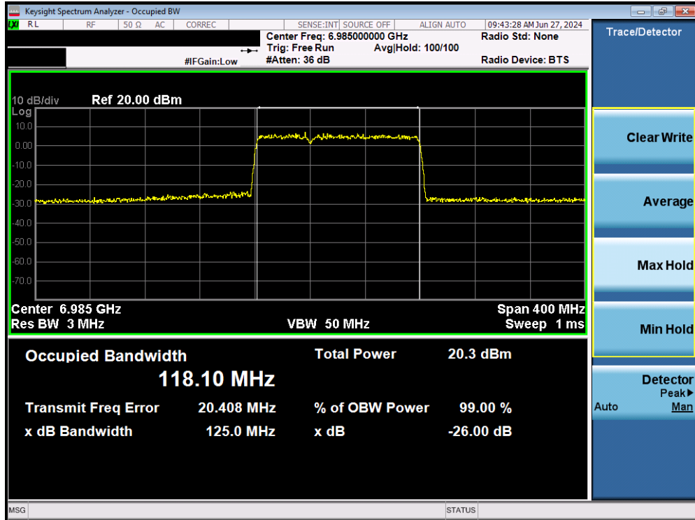
Plot 7-55. Occupied Bandwidth Plot MIMO ANT1 (160MHz BW 802.11be (996+484 Tones) (UNII Band 8) – Ch. 207)
