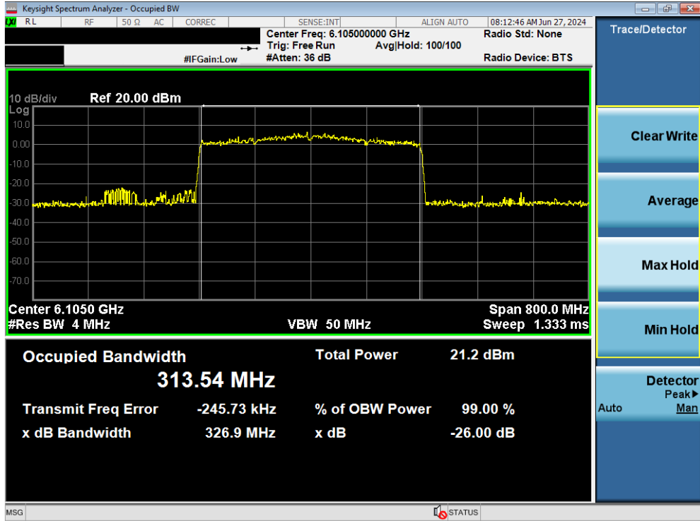
Plot 7-81. Occupied Bandwidth Plot MIMO ANT2 (320MHz BW 802.11be (Full Tones) (UNII Band 5) – Ch. 31)
