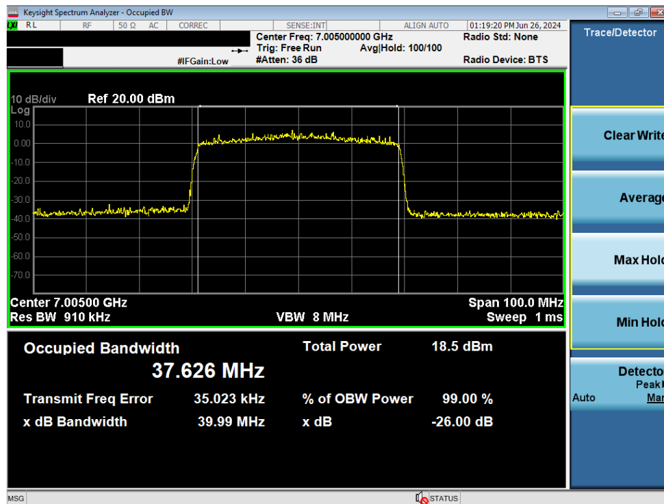
Plot 7-93. Occupied Bandwidth Plot MIMO ANT2 (40MHz BW 802.11ax (Full Tones) (UNII Band 8) – Ch. 211)
