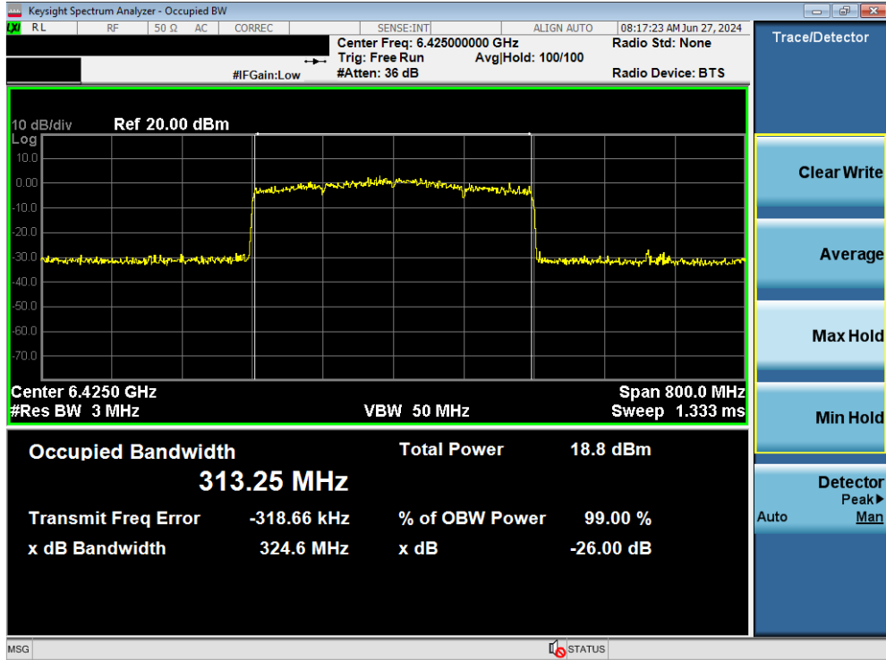
Plot 7-86. Occupied Bandwidth Plot MIMO ANT2 (320MHz BW 802.11be (Full Tones) (UNII Band 6) – Ch. 95)
