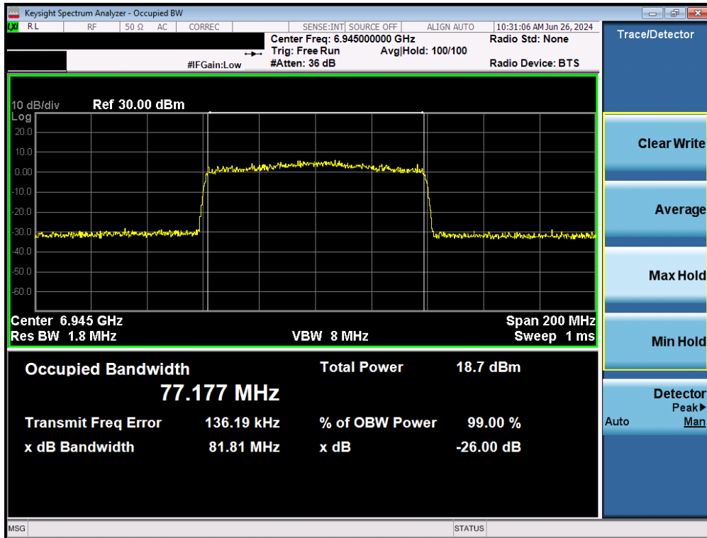
Plot 7-38. Occupied Bandwidth Plot MIMO ANT1 (80MHz BW 802.11ax/be (Full Tones) (UNII Band 8) – Ch. 199)
