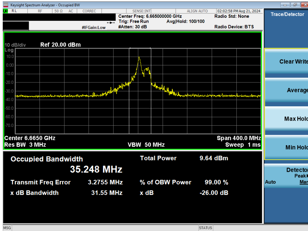
Plot 7-70. Occupied Bandwidth Plot MIMO ANT2 (160MHz BW 802.11ax/be (26 Tones) (UNII Band 7) – Ch. 143)
