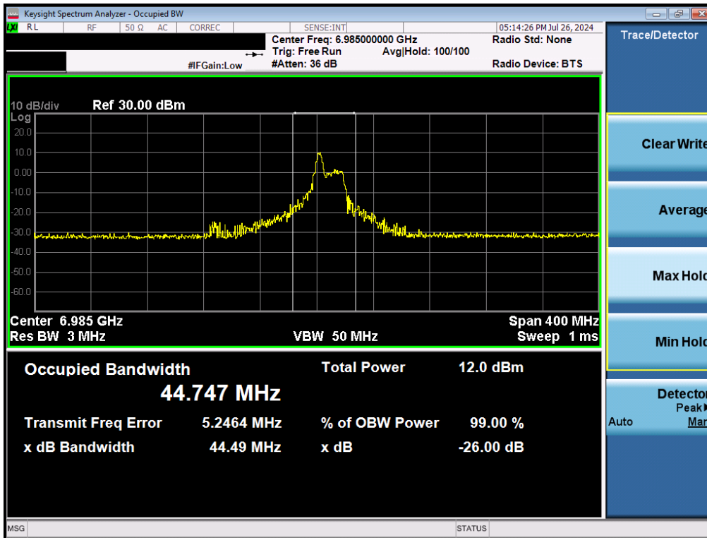
Plot 7-19. Occupied Bandwidth Plot MIMO ANT1 (160MHz BW 802.11ax/be (26 Tones) (UNII Band 8) – Ch. 207)
