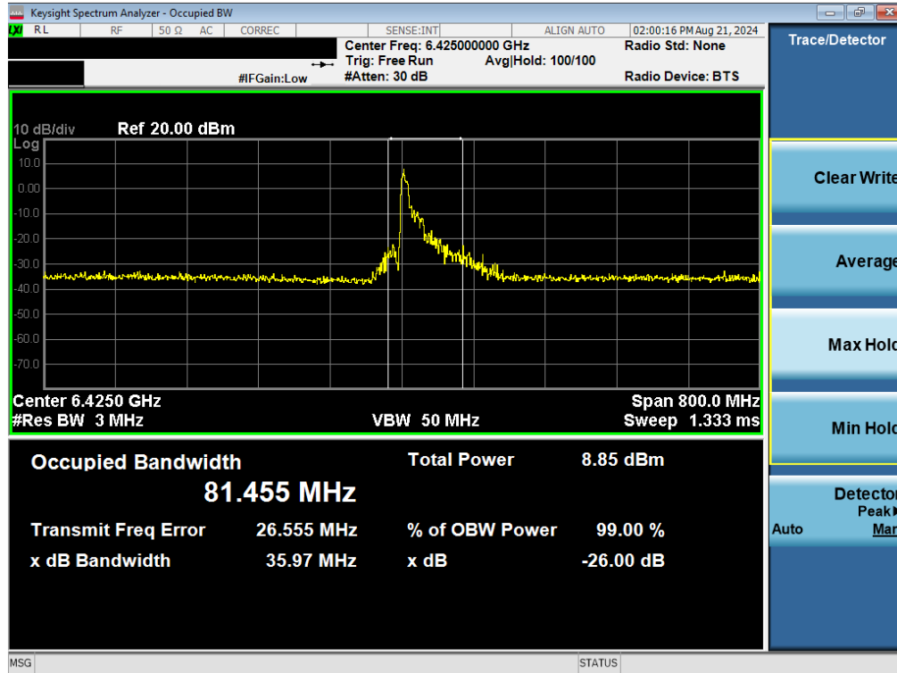
Plot 7-66. Occupied Bandwidth Plot MIMO ANT2 (320MHz BW 802.11be (26 Tones) (UNII Band 6) – Ch. 95)
