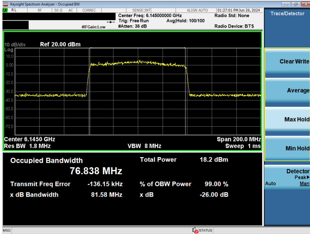
Plot 7-79. Occupied Bandwidth Plot MIMO ANT2 (80MHz BW 802.11ax/be (Full Tones) (UNII Band 5) – Ch. 39)
