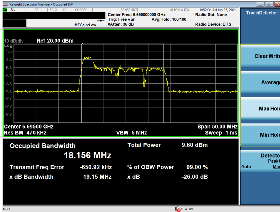
Plot 7-67. Occupied Bandwidth Plot MIMO ANT2 (20MHz BW 802.11 ax/be (26 Tones) (UNII Band 7) – Ch. 149)
