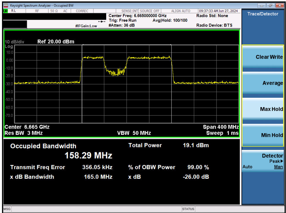
Plot 7-51. Occupied Bandwidth Plot MIMO ANT1 (160MHz BW 802.11be (996+484 Tones) (UNII Band 7) – Ch. 143)
