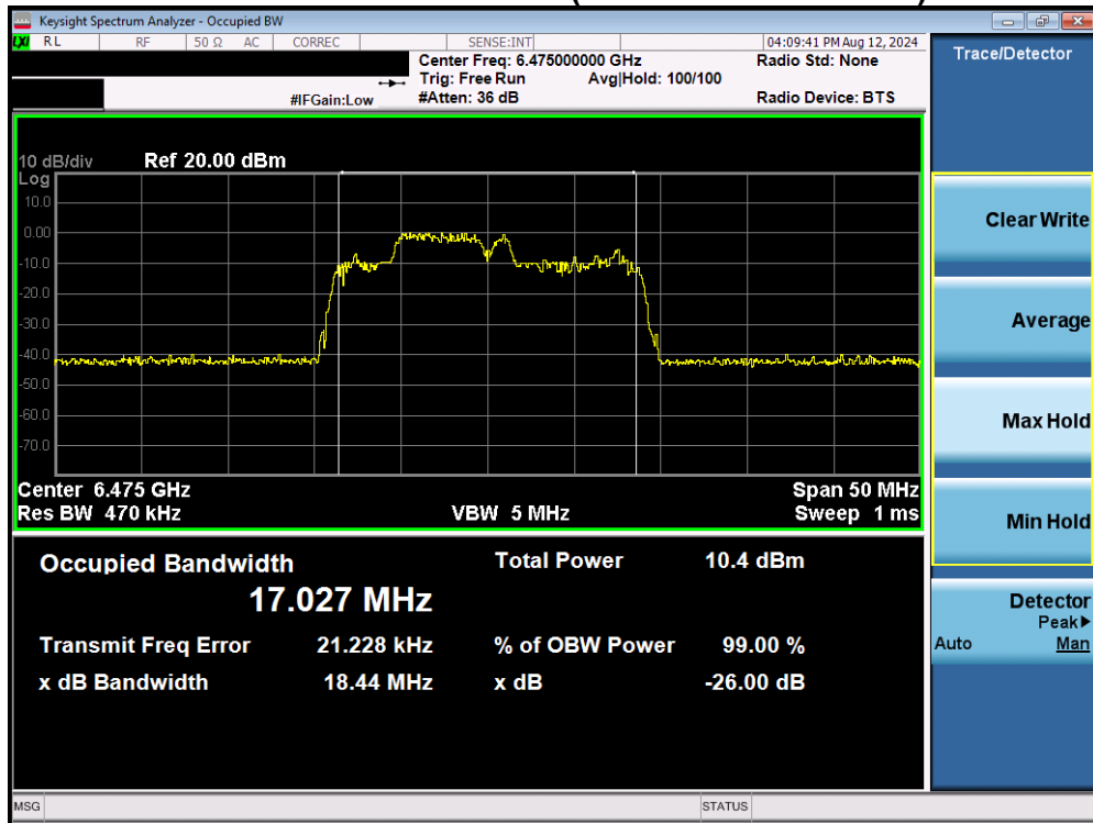
Plot 7-45. Occupied Bandwidth Plot MIMO ANT1 (20MHz BW 802.11be (52+26 Tones) (UNII Band 6) – Ch. 105)
