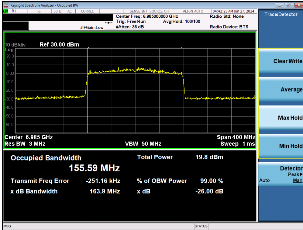
Plot 7-39. Occupied Bandwidth Plot MIMO ANT1 (160MHz BW 802.11ax/be (Full Tones) (UNII Band 8) – Ch. 207)
