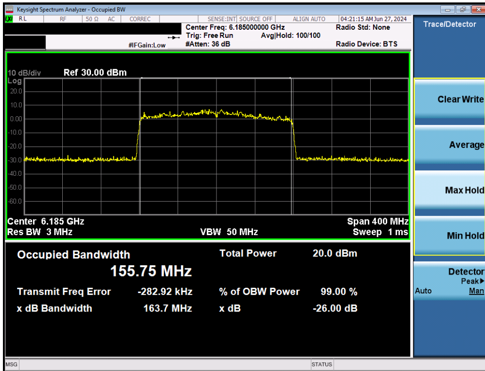
Plot 7-24. Occupied Bandwidth Plot MIMO ANT1 (160MHz BW 802.11 ax/be (Full Tones) (UNII Band 5) – Ch. 47)
