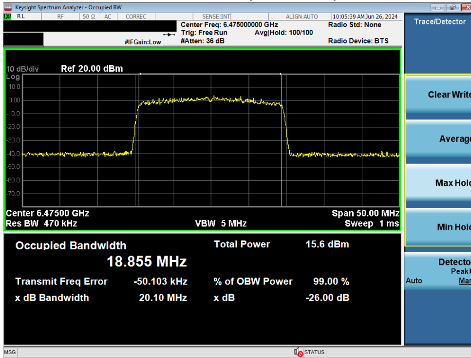
Plot 7-82. Occupied Bandwidth Plot MIMO ANT2 (20MHz BW 802.11ax/be (Full Tones) (UNII Band 6) – Ch. 105)
