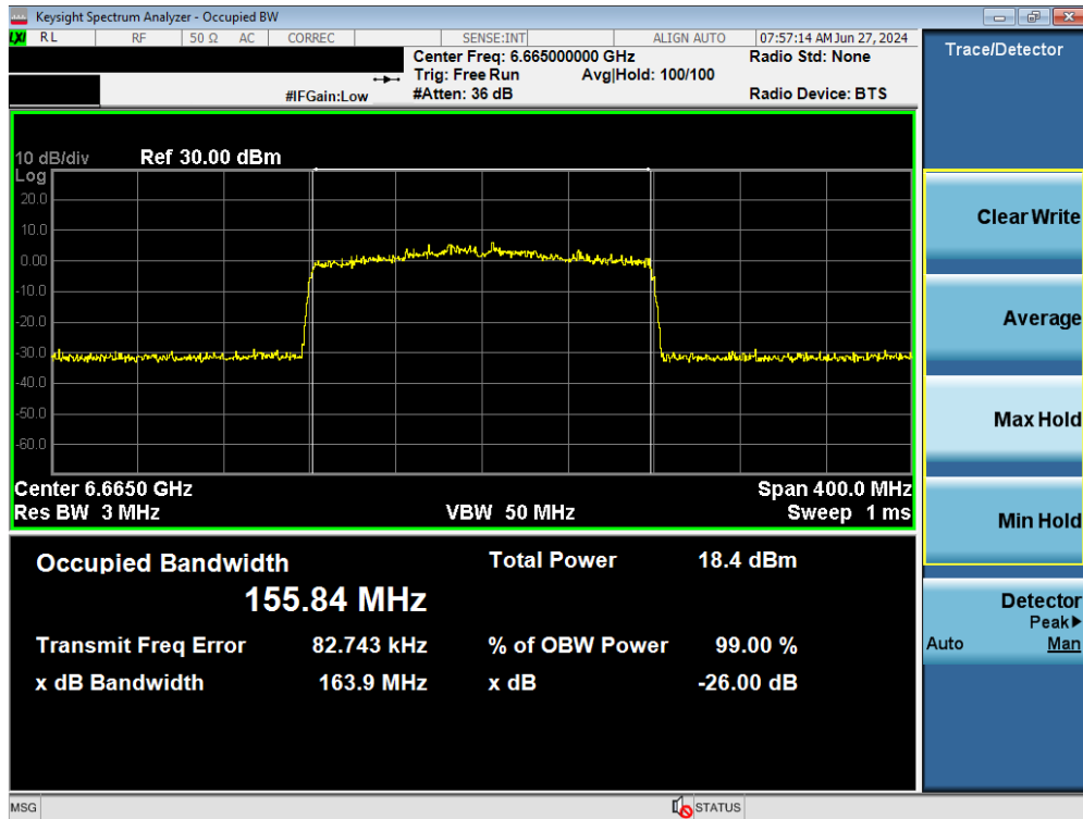
Plot 7-90. Occupied Bandwidth Plot MIMO ANT2 (160MHz BW 802.11ax/be (Full Tones) (UNII Band 7) – Ch. 143)
