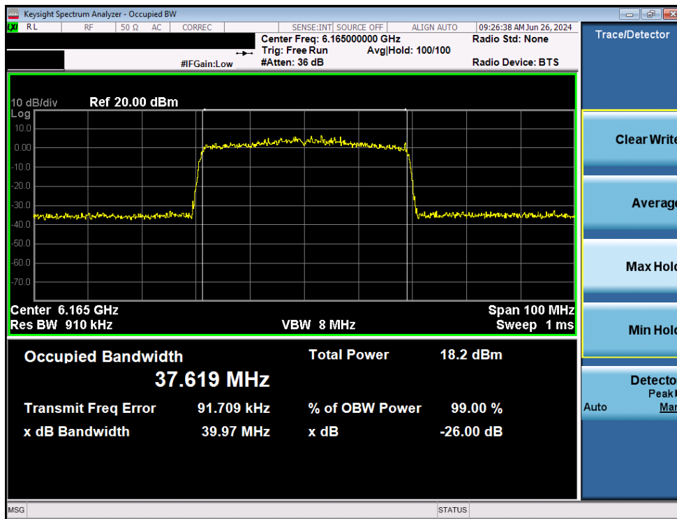
Plot 7-22. Occupied Bandwidth Plot MIMO ANT1 (40MHz BW 802.11 ax/be (Full Tones) (UNII Band 5) – Ch. 43)
