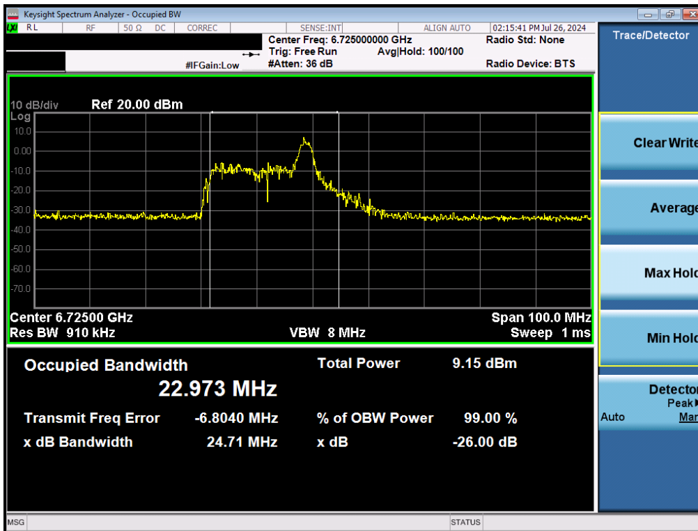
Plot 7-68. Occupied Bandwidth Plot MIMO ANT2 (40MHz BW 802.11 ax/be (26 Tones) (UNII Band 7) – Ch. 155)
