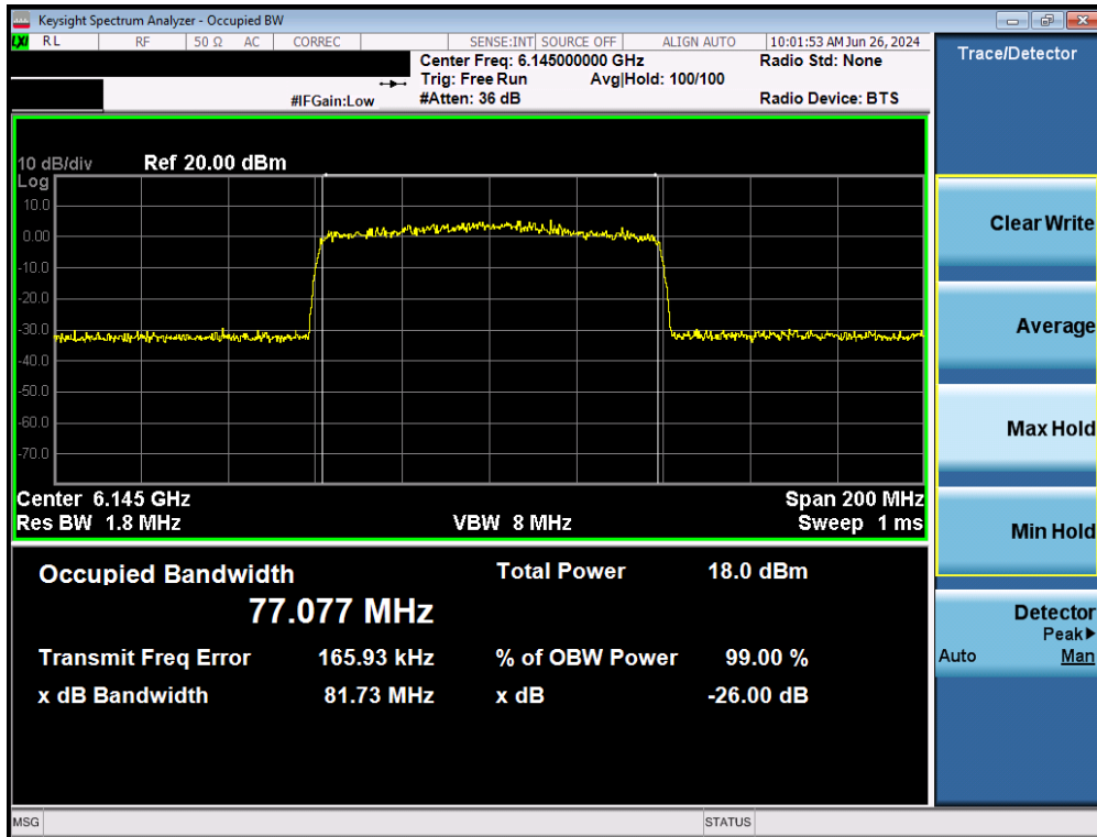
Plot 7-23. Occupied Bandwidth Plot MIMO ANT1 (80MHz BW 802.11 ax/be (Full Tones) (UNII Band 5) – Ch. 39)
