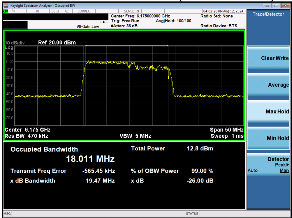
Plot 7-41. Occupied Bandwidth Plot MIMO ANT1 (20MHz BW 802.11be (106+26 Tones) (UNII Band 5) – Ch. 45)
