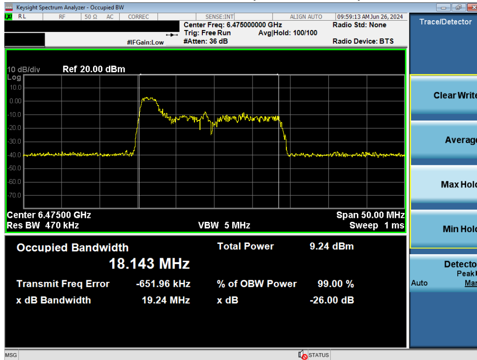
Plot 7-62. Occupied Bandwidth Plot MIMO ANT2 (20MHz BW 802.11 ax/be (26 Tones) (UNII Band 6) – Ch. 105)
