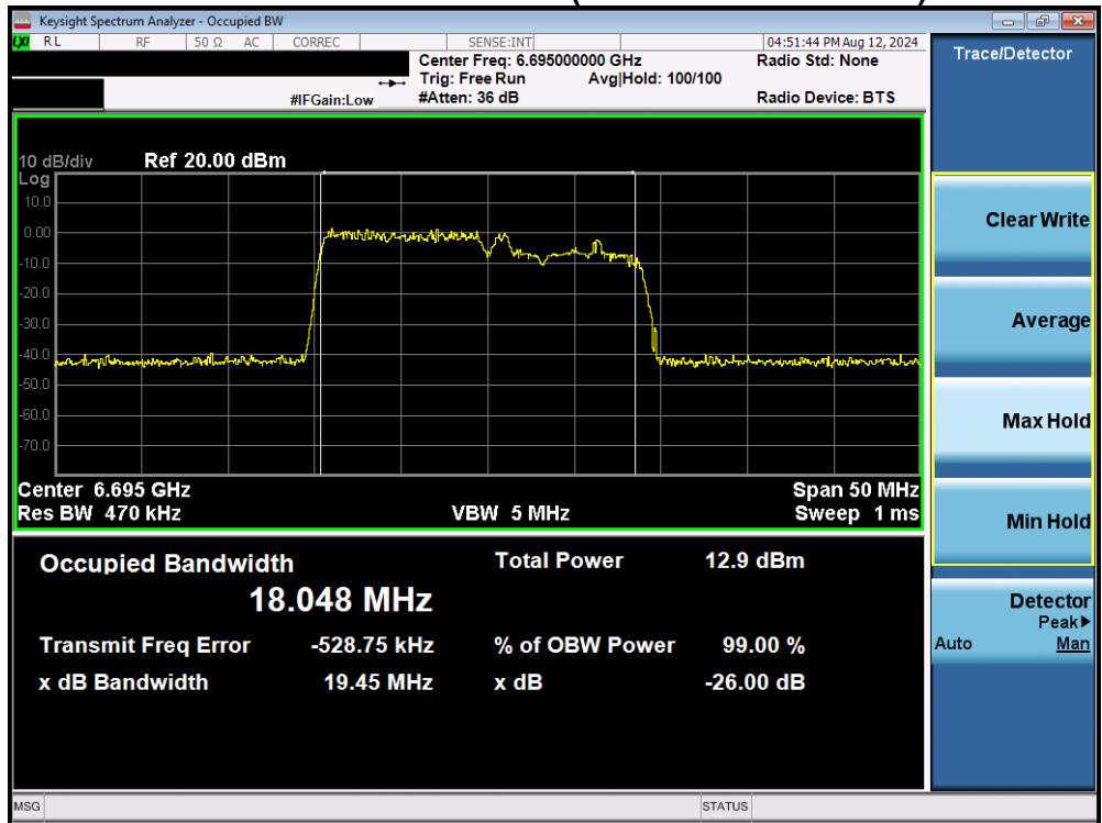
Plot 7-49. Occupied Bandwidth Plot MIMO ANT1 (20MHz BW 802.11be (106+26 Tones) (UNII Band 7) – Ch. 149)
