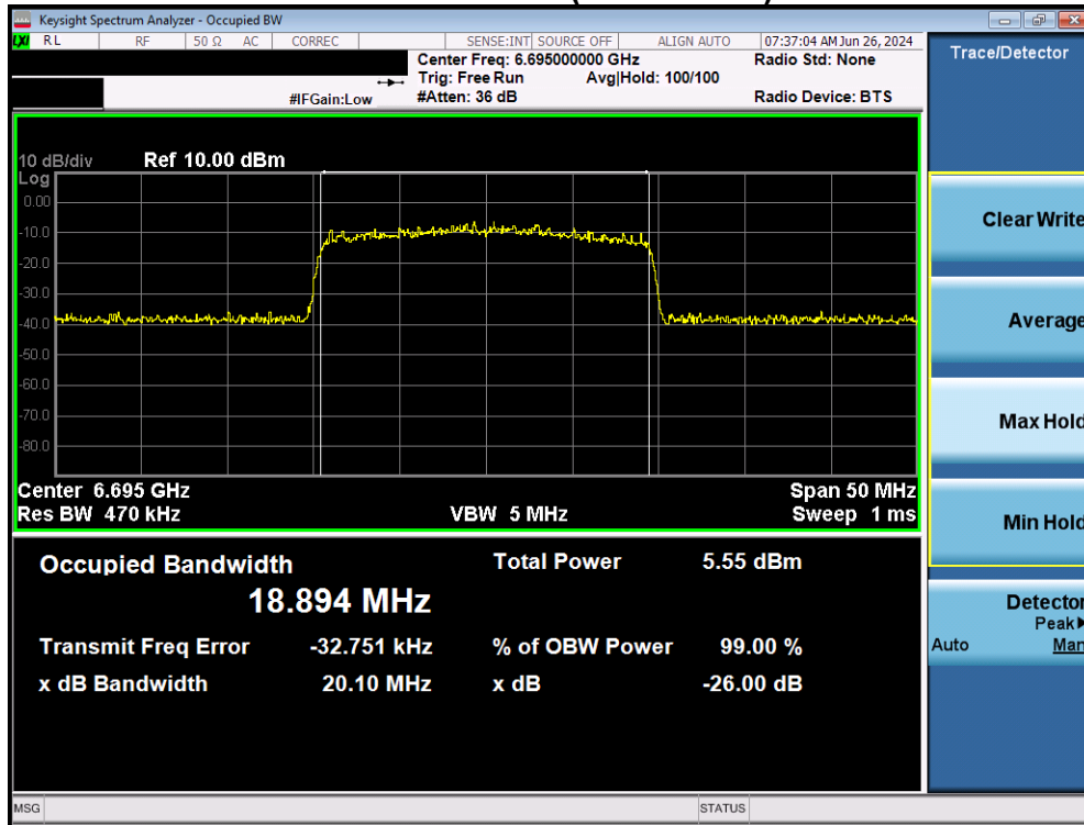
Plot 7-31. Occupied Bandwidth Plot MIMO ANT1 (20MHz BW 802.11ax/be (Full Tones) (UNII Band 7) – Ch. 149)
