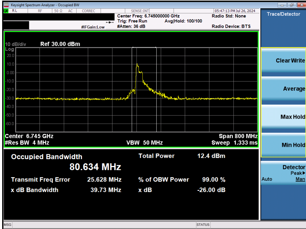
Plot 7-15. Occupied Bandwidth Plot MIMO ANT1 (320MHz BW 802.11be (26 Tones) (UNII Band 7) – Ch. 159)
