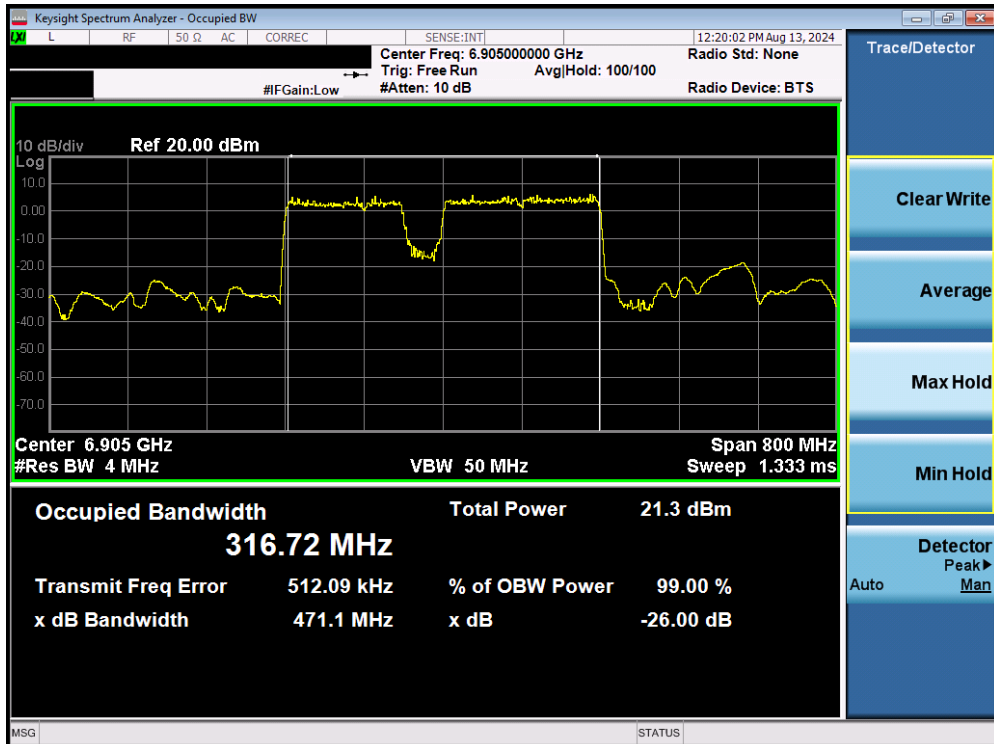
Plot 7-56. Occupied Bandwidth Plot MIMO ANT1 (320MHz BW 802.11be (3*996+484 Tones) (UNII Band 8) – Ch. 191)
