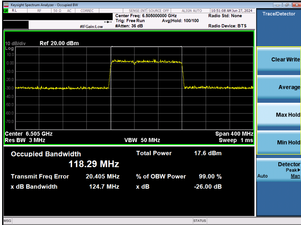
Plot 7-47. Occupied Bandwidth Plot MIMO ANT1 (160MHz BW 802.11be (996+484 Tones) (UNII Band 6) – Ch. 111)
