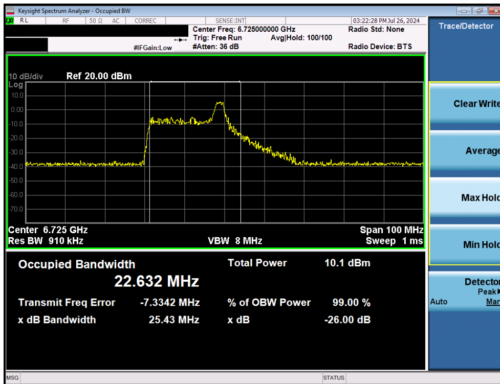
Plot 7-12. Occupied Bandwidth Plot MIMO ANT1 (40MHz BW 802.11 ax/be (26 Tones) (UNII Band 7) – Ch. 155)
