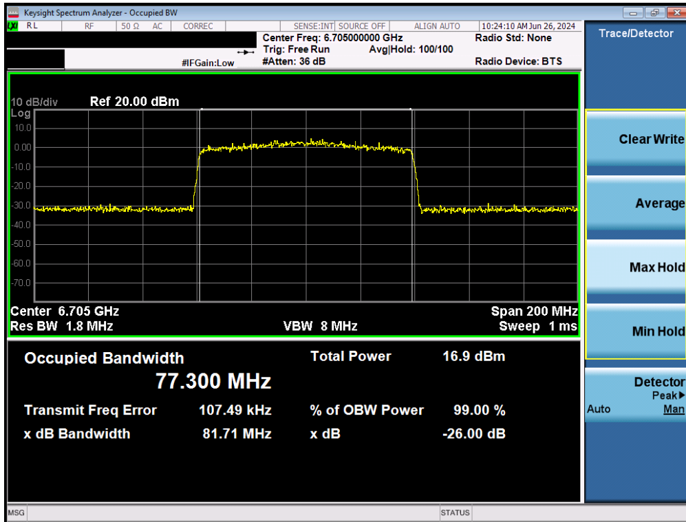
Plot 7-33. Occupied Bandwidth Plot MIMO ANT1 (80MHz BW 802.11ax/be (Full Tones) (UNII Band 7) – Ch. 151)
