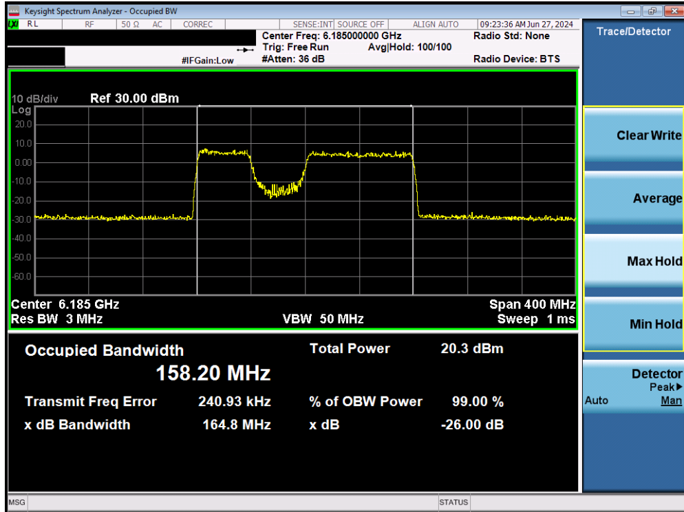
Plot 7-43. Occupied Bandwidth Plot MIMO ANT1 (160MHz BW 802.11be (996+484 Tones) (UNII Band 5) – Ch. 47)
