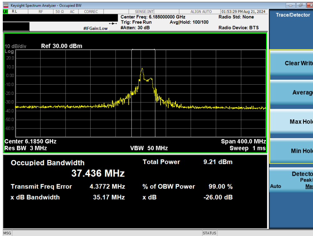
Plot 7-60. Occupied Bandwidth Plot MIMO ANT2 (160MHz BW 802.11ax (26 Tones) (UNII Band 5) – Ch. 47)
