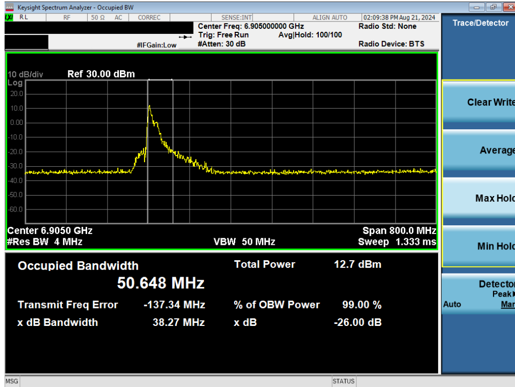
Plot 7-76. Occupied Bandwidth Plot MIMO ANT2 (320MHz BW 802.11be (26 Tones) (UNII Band 8) – Ch. 191)
