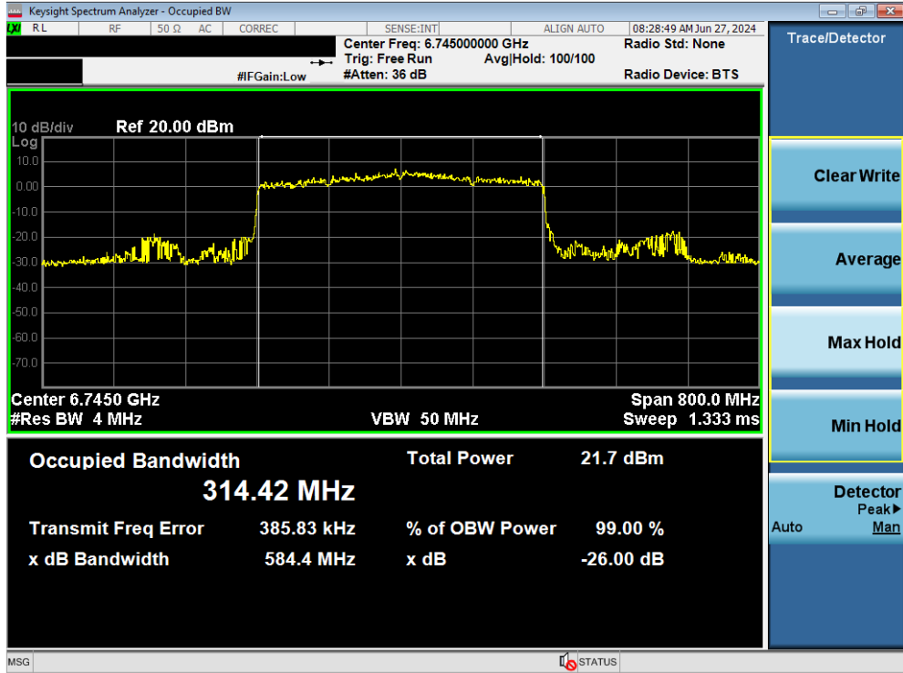
Plot 7-91. Occupied Bandwidth Plot MIMO ANT2 (320MHz BW 802.11be (Full Tones) (UNII Band 7) – Ch. 159)
