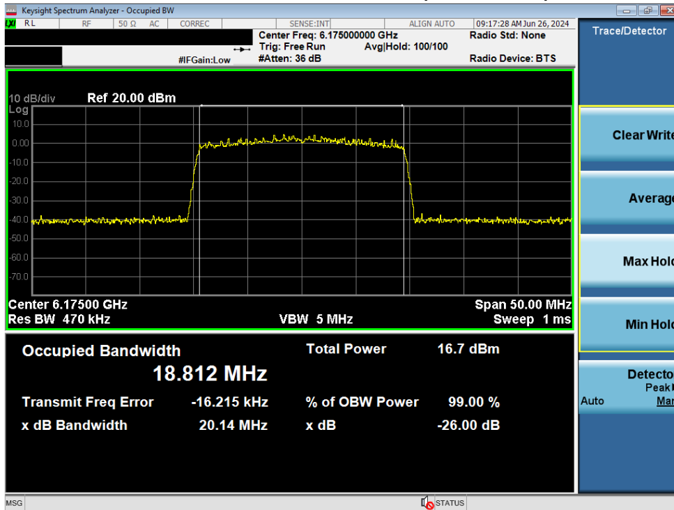
Plot 7-77. Occupied Bandwidth Plot MIMO ANT2 (20MHz BW 802.11 ax/be (Full Tones) (UNII Band 5) – Ch. 45)
