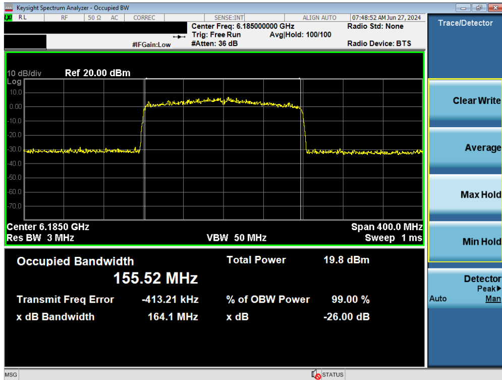
Plot 7-80. Occupied Bandwidth Plot MIMO ANT2 (160MHz BW 802.11ax/be (Full Tones) (UNII Band 5) – Ch. 47)
