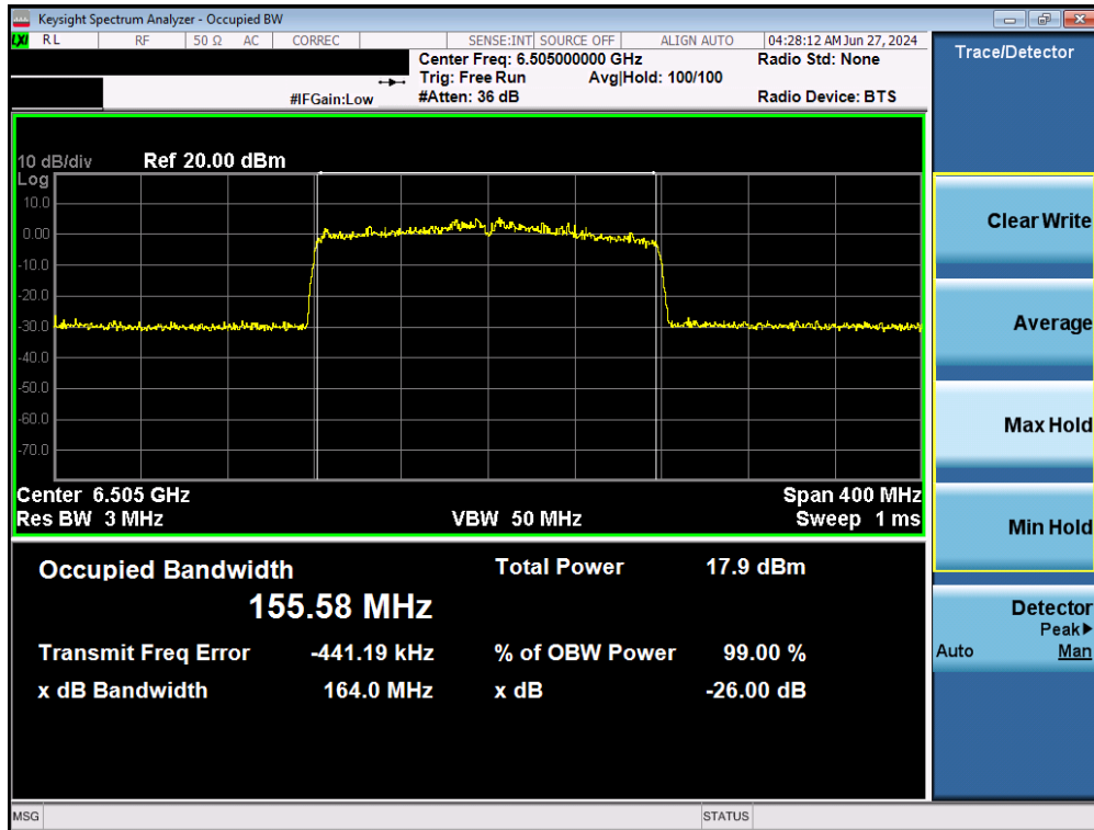
Plot 7-29. Occupied Bandwidth Plot MIMO ANT1 (160MHz BW 802.11ax/be (Full Tones) (UNII Band 6) – Ch. 111)
