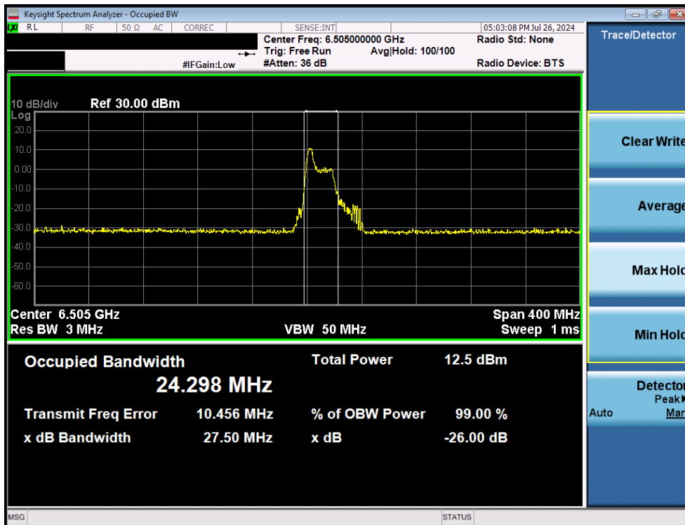
Plot 7-9. Occupied Bandwidth Plot MIMO ANT1 (160MHz BW 802.11ax/be (26 Tones) (UNII Band 6) – Ch. 111)
