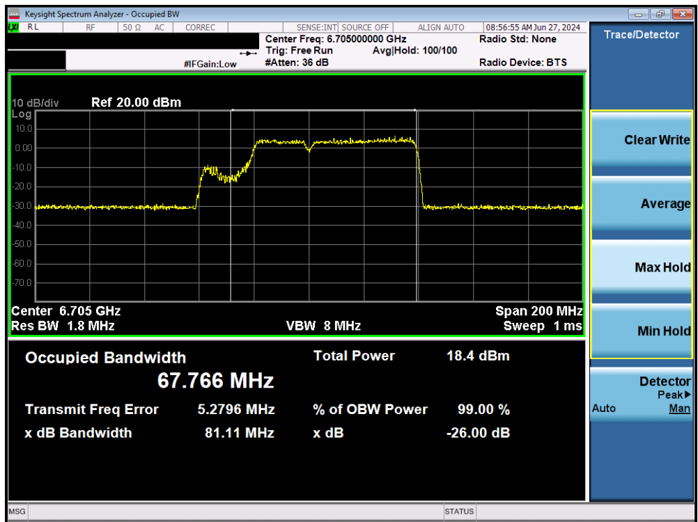
Plot 7-50. Occupied Bandwidth Plot MIMO ANT1 (80MHz BW 802.11be (484+242 Tones) (UNII Band 7) – Ch. 151)
