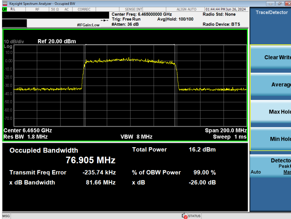
Plot 7-84. Occupied Bandwidth Plot MIMO ANT2 (80MHz BW 802.11ax/be (Full Tones) (UNII Band 6) – Ch. 103)
