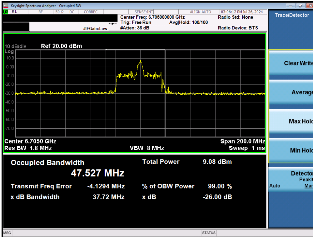
Plot 7-69. Occupied Bandwidth Plot MIMO ANT2 (80MHz BW 802.11ax/be (26 Tones) (UNII Band 7) – Ch. 151)
