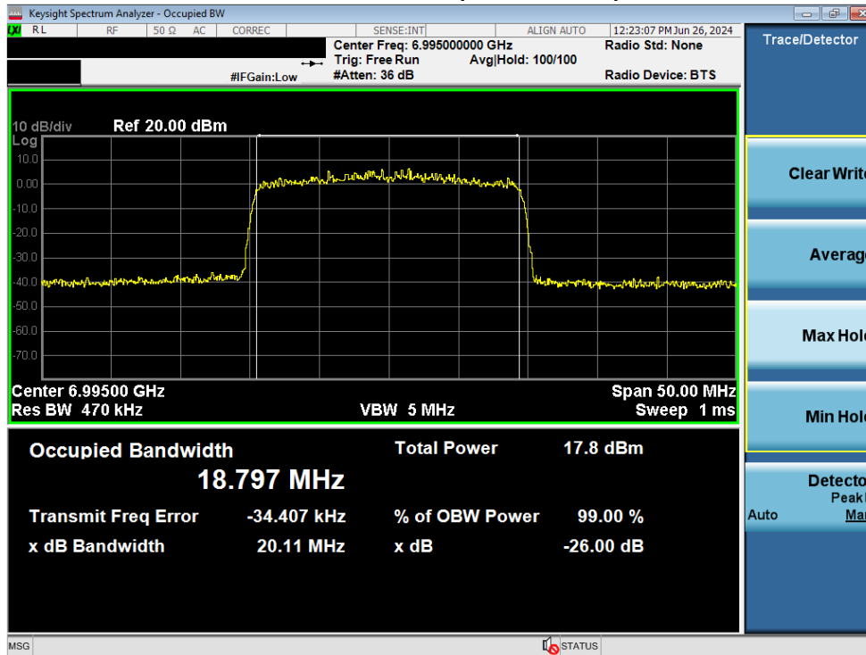
Plot 7-92. Occupied Bandwidth Plot MIMO ANT2 (20MHz BW 802.11ax (Full Tones) (UNII Band 8) – Ch. 209)
