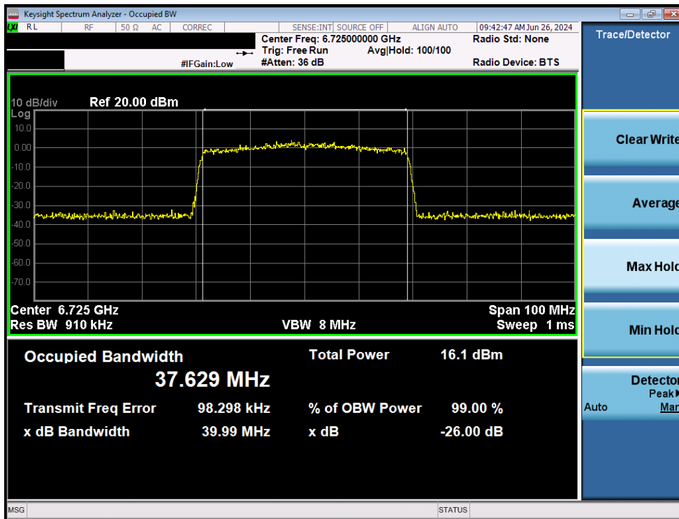
Plot 7-32. Occupied Bandwidth Plot MIMO ANT1 (40MHz BW 802.11ax/be (Full Tones) (UNII Band 7) – Ch. 155)
