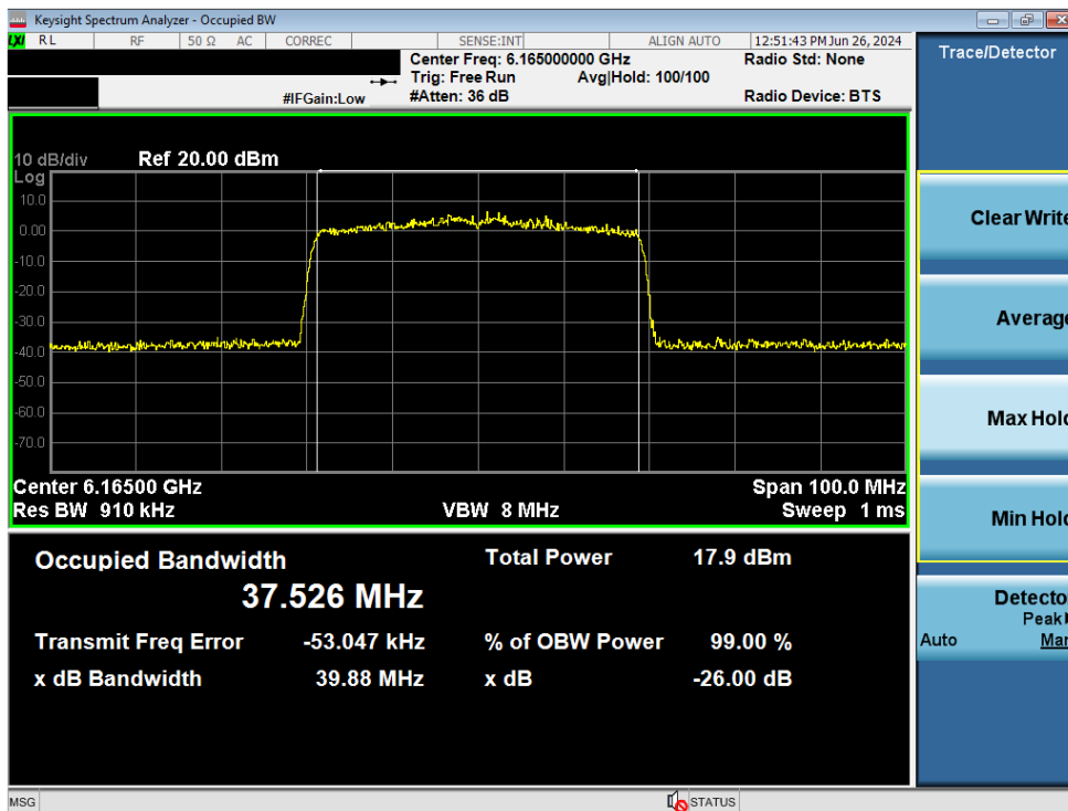
Plot 7-78. Occupied Bandwidth Plot MIMO ANT2 (40MHz BW 802.11 ax/be (Full Tones) (UNII Band 5) – Ch. 43)
