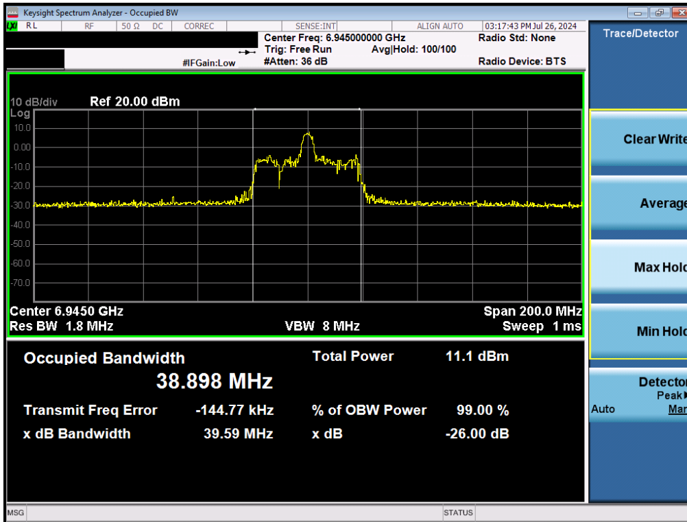
Plot 7-74. Occupied Bandwidth Plot MIMO ANT2 (80MHz BW 802.11ax/be (26 Tones) (UNII Band 8) – Ch. 199)
