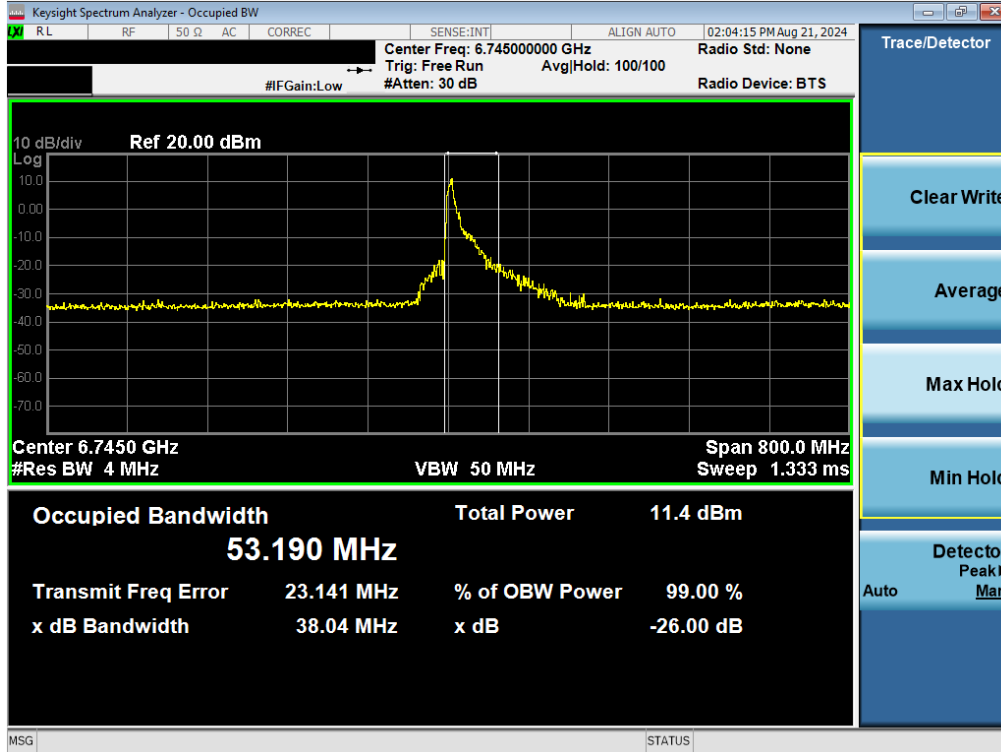
Plot 7-71. Occupied Bandwidth Plot MIMO ANT2 (320MHz BW 802.11be (26 Tones) (UNII Band 7) – Ch. 159)
