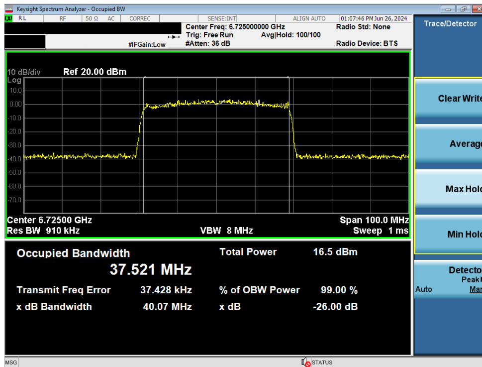
Plot 7-88. Occupied Bandwidth Plot MIMO ANT2 (40MHz BW 802.11ax/be (Full Tones) (UNII Band 7) – Ch. 155)
