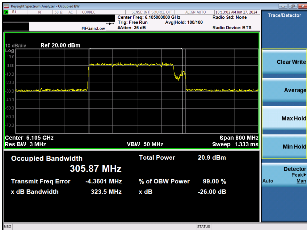
Plot 7-44. Occupied Bandwidth Plot MIMO ANT1 (320MHz BW 802.11be (3*996+484 Tones) (UNII Band 5) – Ch. 31)
