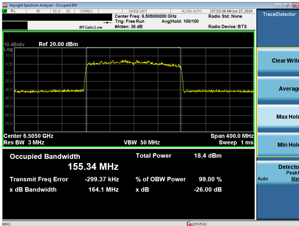
Plot 7-85. Occupied Bandwidth Plot MIMO ANT2 (160MHz BW 802.11ax/be (Full Tones) (UNII Band 6) – Ch. 111)
