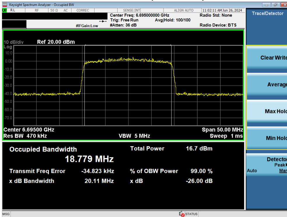
Plot 7-87. Occupied Bandwidth Plot MIMO ANT2 (20MHz BW 802.11ax/be (Full Tones) (UNII Band 7) – Ch. 149)
