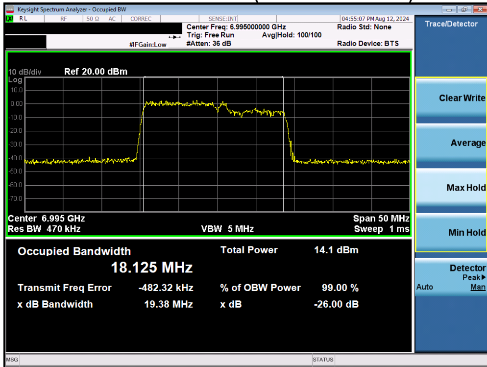
Plot 7-53. Occupied Bandwidth Plot MIMO ANT1 (20MHz BW 802.11be (106+26 Tones) (UNII Band 8) – Ch. 209)
