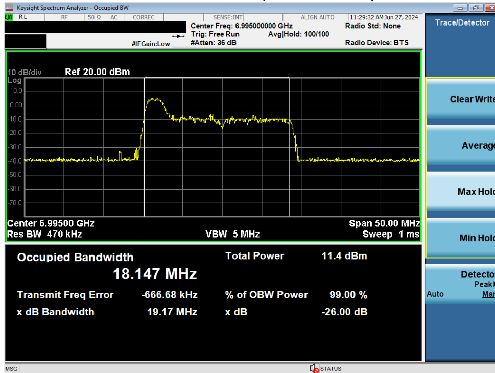
Plot 7-72. Occupied Bandwidth Plot MIMO ANT2 (20MHz BW 802.11 ax/be (26 Tones) (UNII Band 8) – Ch. 209)
