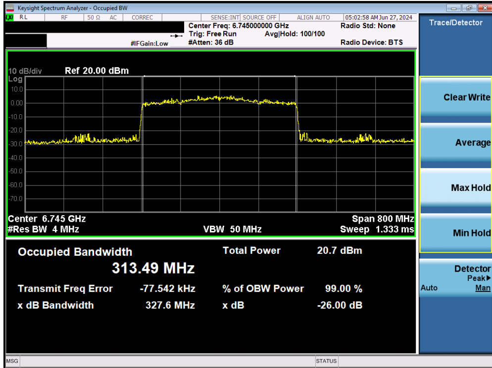
Plot 7-35. Occupied Bandwidth Plot MIMO ANT1 (320MHz BW 802.11be (Full Tones) (UNII Band 7) – Ch. 159)
