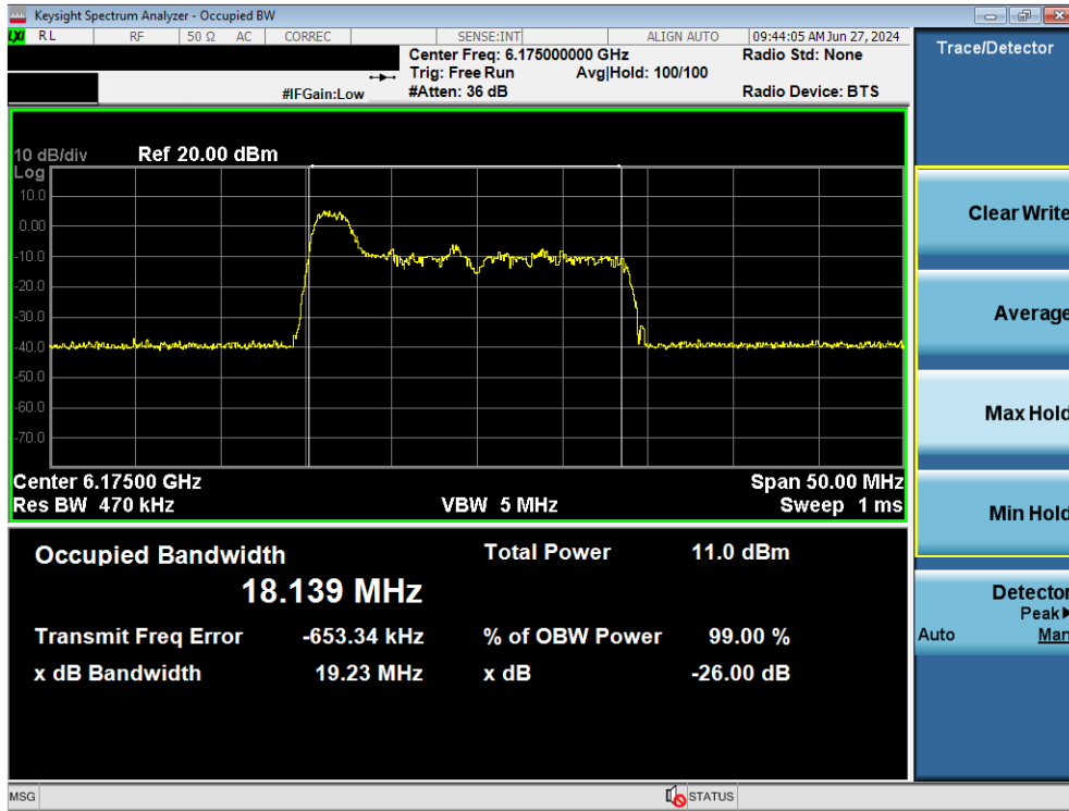
Plot 7-57. Occupied Bandwidth Plot MIMO ANT2 (20MHz BW 802.11ax/be (26 Tones) (UNII Band 5) – Ch. 45)
