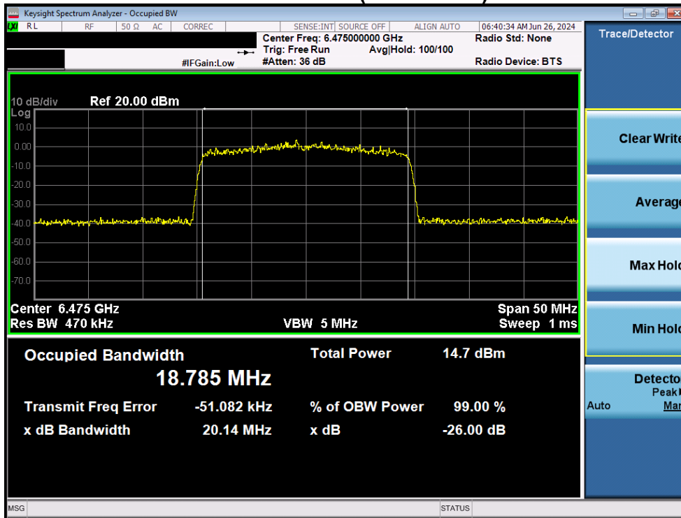
Plot 7-26. Occupied Bandwidth Plot MIMO ANT1 (20MHz BW 802.11ax/be (Full Tones) (UNII Band 6) – Ch. 105)
