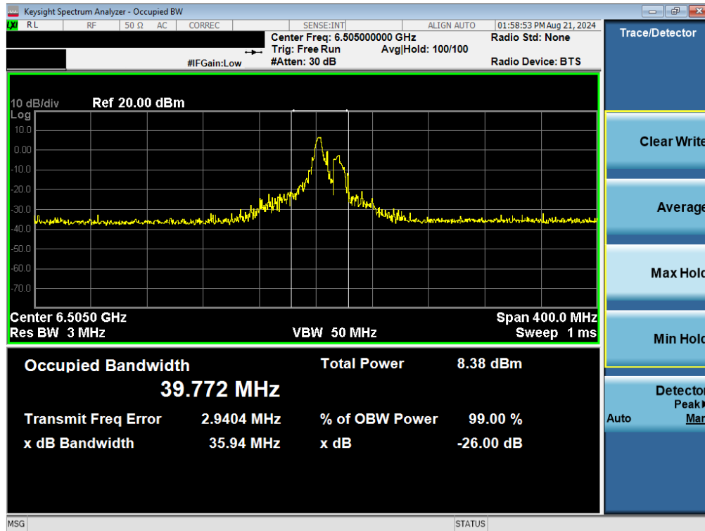
Plot 7-65. Occupied Bandwidth Plot MIMO ANT2 (160MHz BW 802.11ax/be (26 Tones) (UNII Band 6) – Ch. 111)
