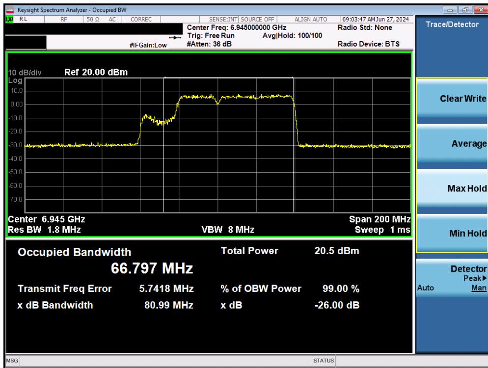
Plot 7-54. Occupied Bandwidth Plot MIMO ANT1 (80MHz BW 802.11be (484+242 Tones) (UNII Band 8) – Ch. 199)
