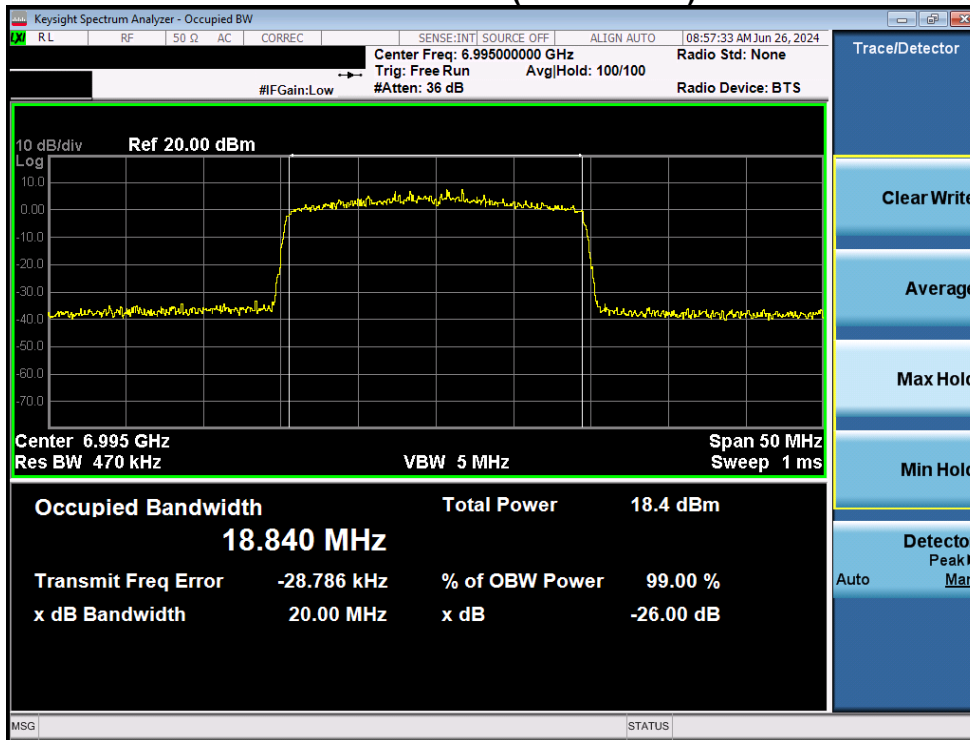
Plot 7-36. Occupied Bandwidth Plot MIMO ANT1 (20MHz BW 802.11ax/be (Full Tones) (UNII Band 8) – Ch. 209)
