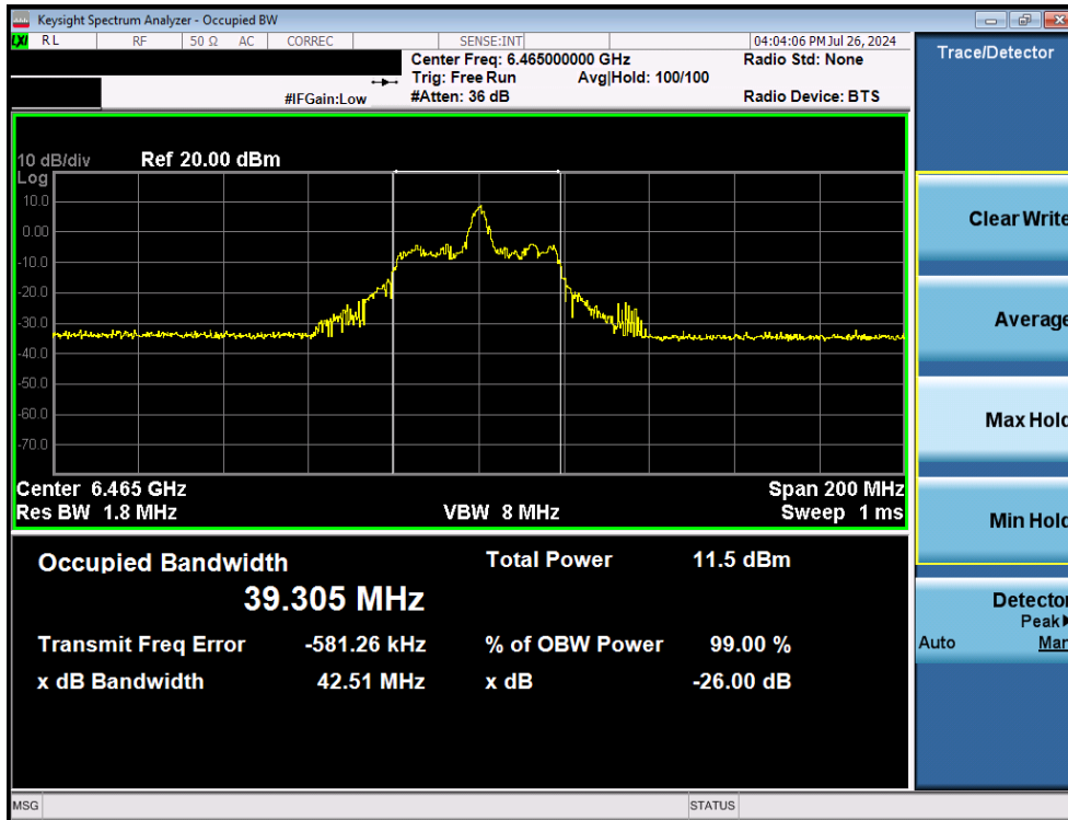
Plot 7-8. Occupied Bandwidth Plot MIMO ANT1 (80MHz BW 802.11ax/be (26 Tones) (UNII Band 6) – Ch. 103)
