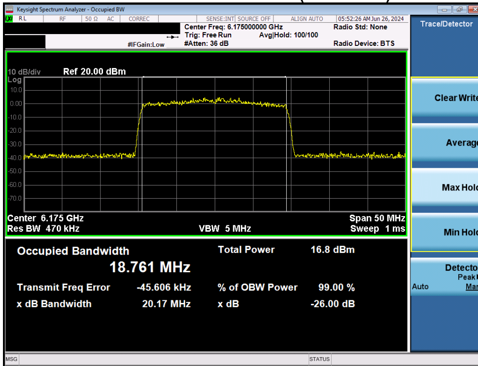
Plot 7-21. Occupied Bandwidth Plot MIMO ANT1 (20MHz BW 802.11 ax/be (Full Tones) (UNII Band 5) – Ch. 45)
