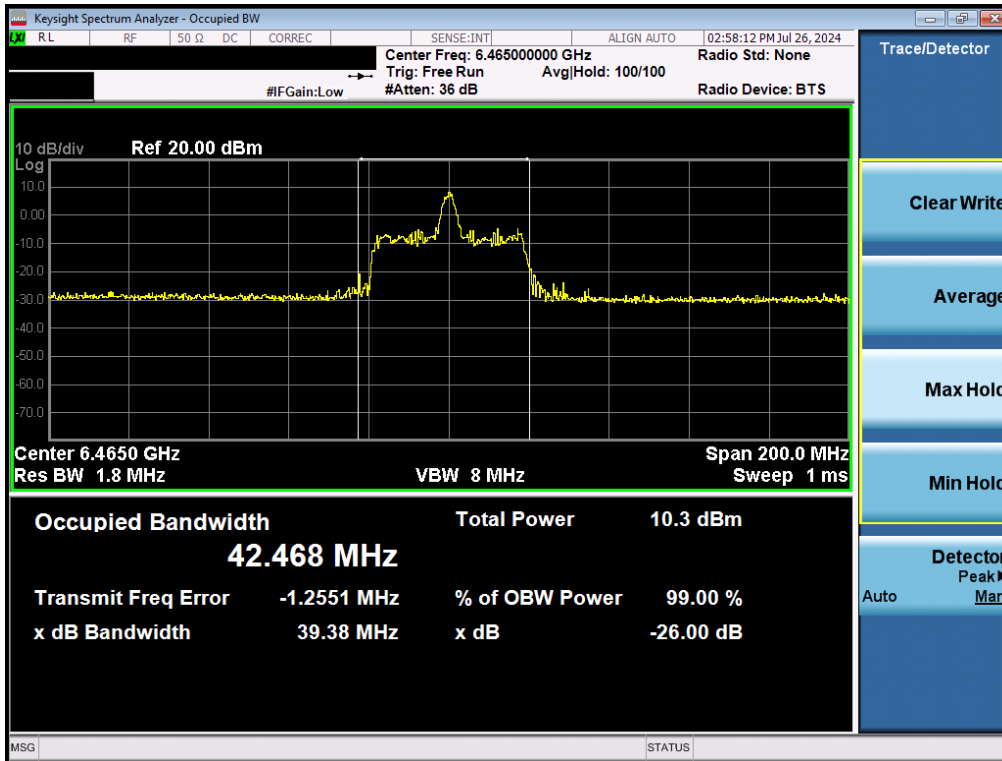
Plot 7-64. Occupied Bandwidth Plot MIMO ANT2 (80MHz BW 802.11ax/be (26 Tones) (UNII Band 6) – Ch. 103)
