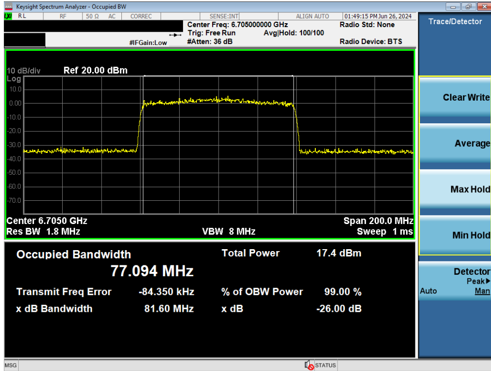
Plot 7-89. Occupied Bandwidth Plot MIMO ANT2 (80MHz BW 802.11ax/be (Full Tones) (UNII Band 7) – Ch. 151)
