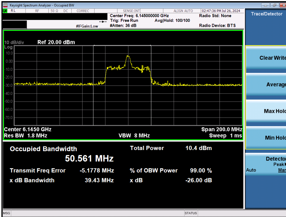
Plot 7-59. Occupied Bandwidth Plot MIMO ANT2 (80MHz BW 802.11ax/be (26 Tones) (UNII Band 5) – Ch. 39)
