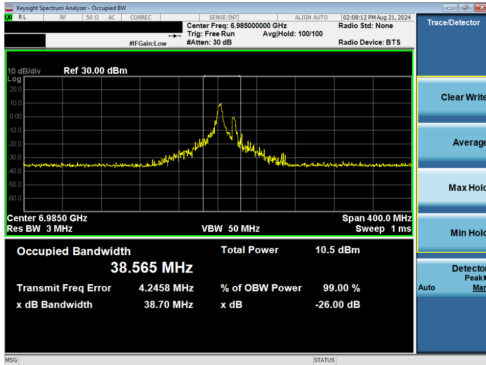
Plot 7-75. Occupied Bandwidth Plot MIMO ANT2 (160MHz BW 802.11ax/be (26 Tones) (UNII Band 8) – Ch. 207)
