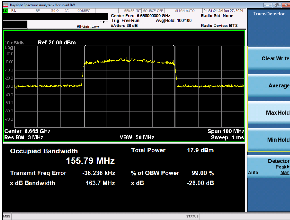
Plot 7-34. Occupied Bandwidth Plot MIMO ANT1 (160MHz BW 802.11ax/be (Full Tones) (UNII Band 7) – Ch. 143)
