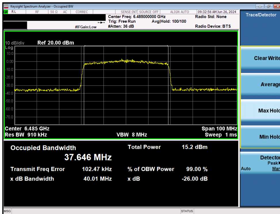
Plot 7-27. Occupied Bandwidth Plot MIMO ANT1 (40MHz BW 802.11ax/be (Full Tones) (UNII Band 6) – Ch. 107)
