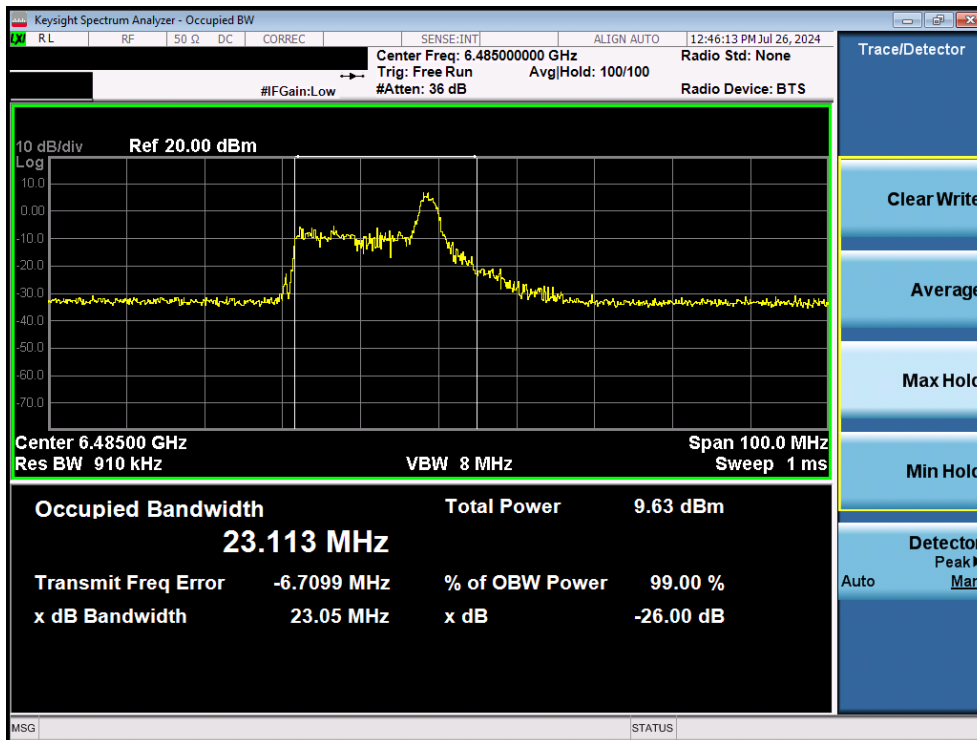
Plot 7-63. Occupied Bandwidth Plot MIMO ANT2 (40MHz BW 802.11 ax/be (26 Tones) (UNII Band 6) – Ch. 107)
