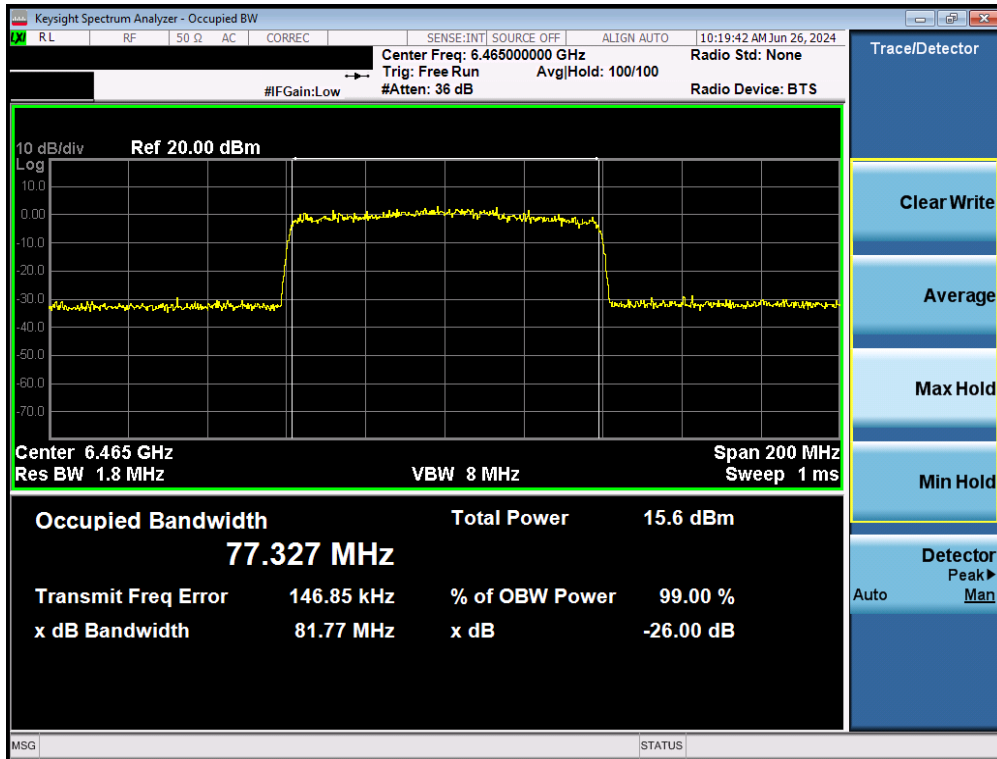
Plot 7-28. Occupied Bandwidth Plot MIMO ANT1 (80MHz BW 802.11ax/be (Full Tones) (UNII Band 6) – Ch. 103)
