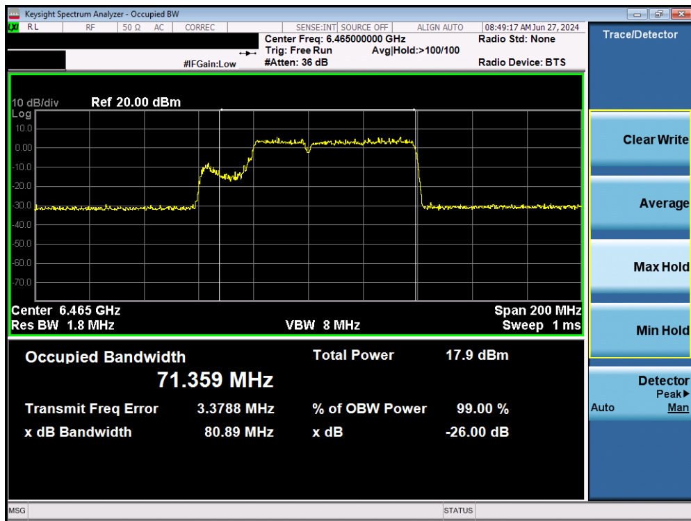
Plot 7-46. Occupied Bandwidth Plot MIMO ANT1 (80MHz BW 802.11be (484+242 Tones) (UNII Band 6) – Ch. 103)
