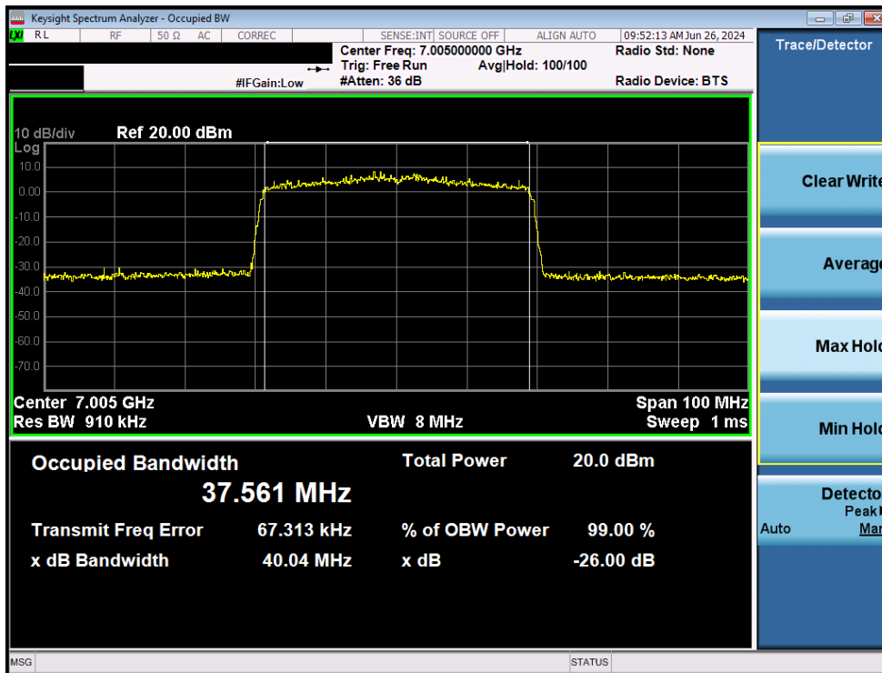
Plot 7-37. Occupied Bandwidth Plot MIMO ANT1 (40MHz BW 802.11ax/be (Full Tones) (UNII Band 8) – Ch. 211)
