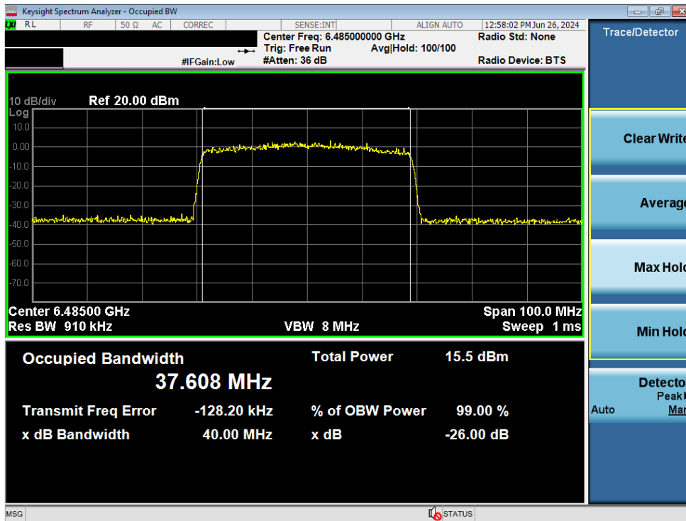
Plot 7-83. Occupied Bandwidth Plot MIMO ANT2 (40MHz BW 802.11ax/be (Full Tones) (UNII Band 6) – Ch. 107)
