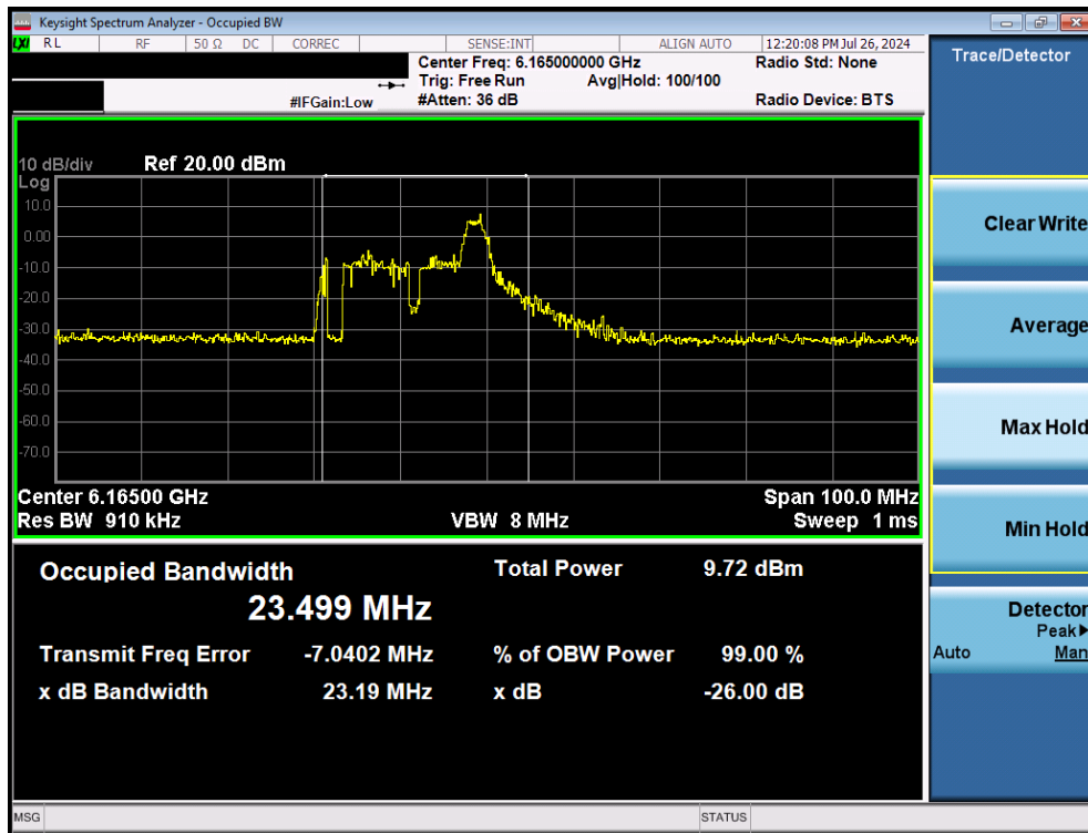
Plot 7-58. Occupied Bandwidth Plot MIMO ANT2 (40MHz BW 802.11ax/be (26 Tones) (UNII Band 5) – Ch. 43)
