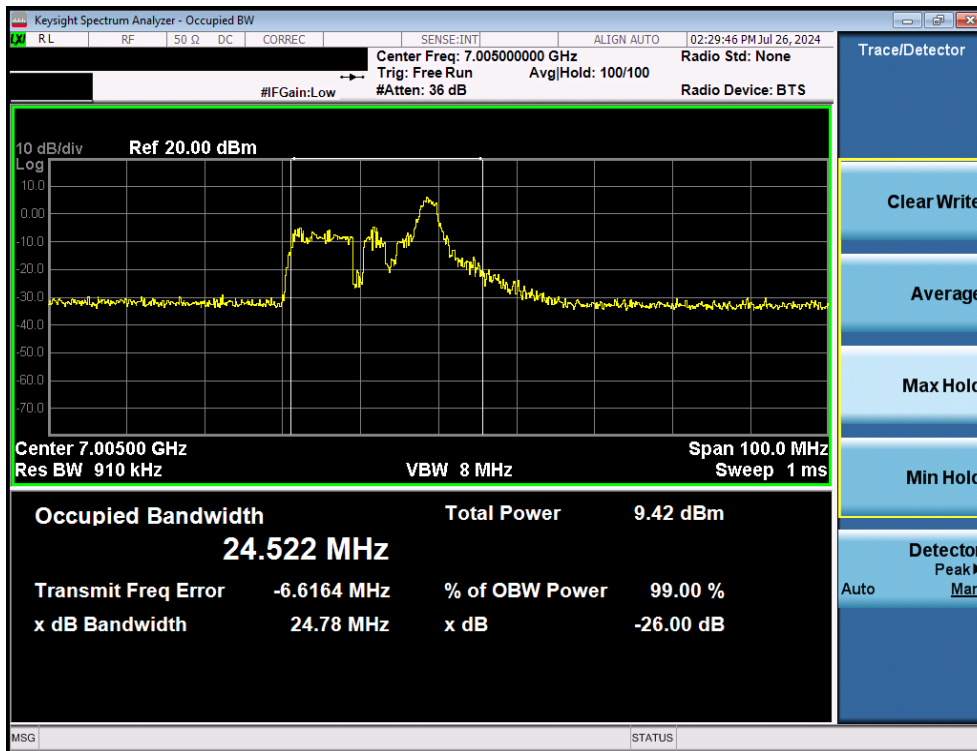
Plot 7-73. Occupied Bandwidth Plot MIMO ANT2 (40MHz BW 802.11 ax/be (26 Tones) (UNII Band 8) – Ch. 211)
