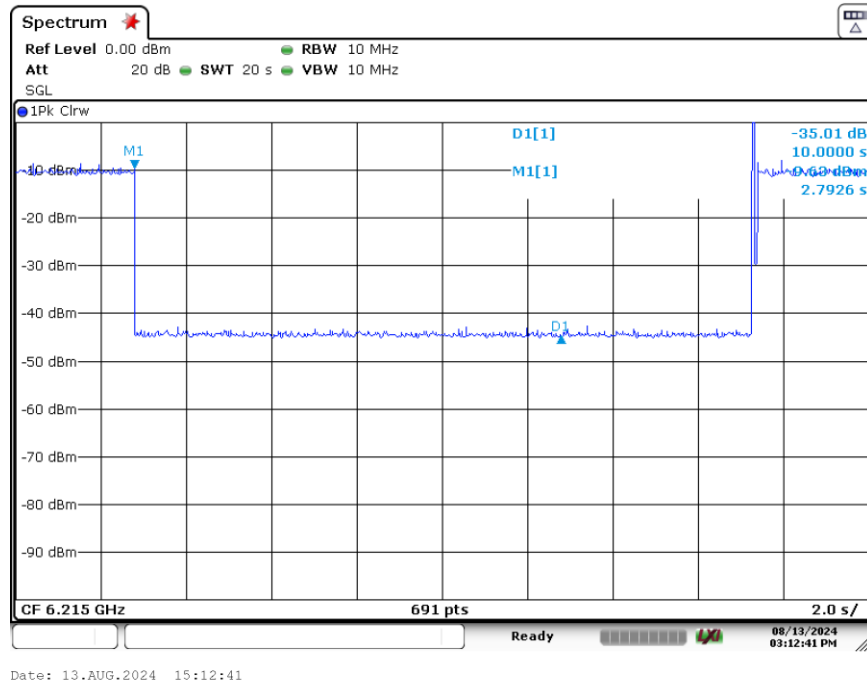
Plot 7-216. Contention Based Protocol Timing Plot (20MHz (UNII Band 5) – Ch. 53)
