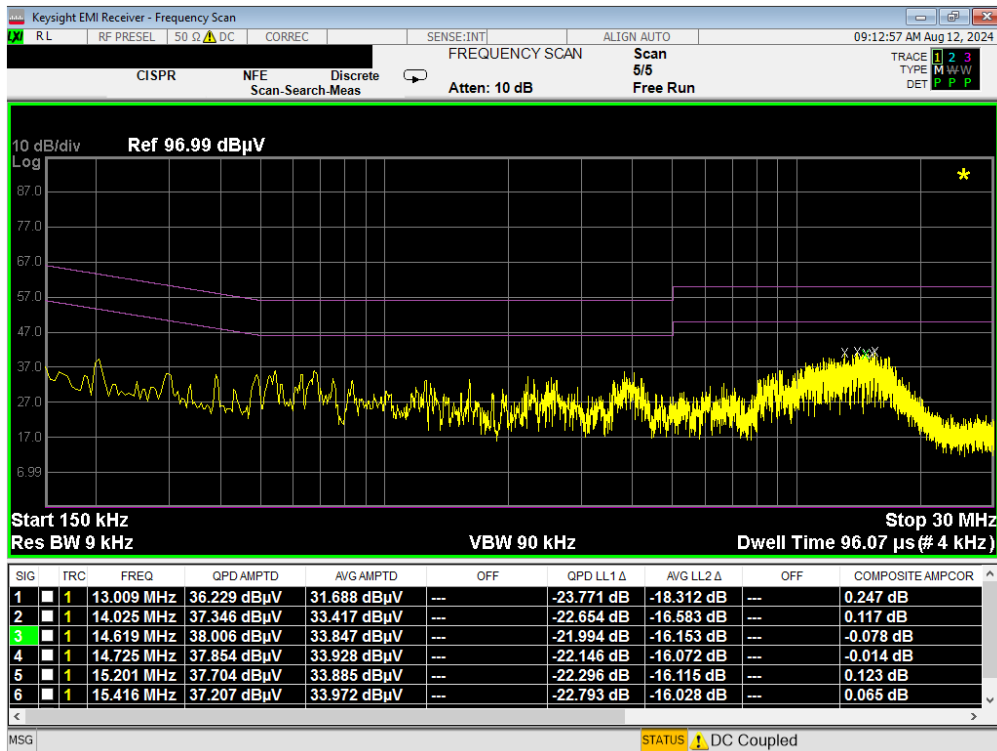
Plot 7-263. Line Conducted Plot with 802.11a UNII Band 5 (N)
