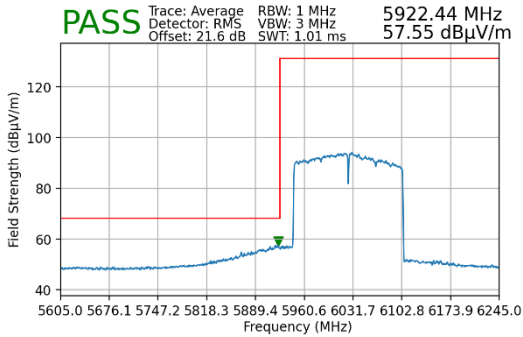
Plot 7-254. Radiated Lower Band Edge Plot MIMO (Average – UNII Band 5)
