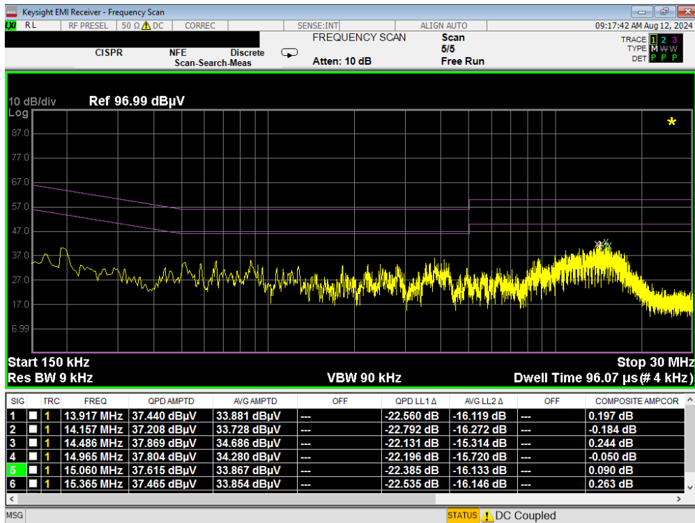
Plot 7-265. Line Conducted Plot with 802.11a UNII Band 6 (N)
