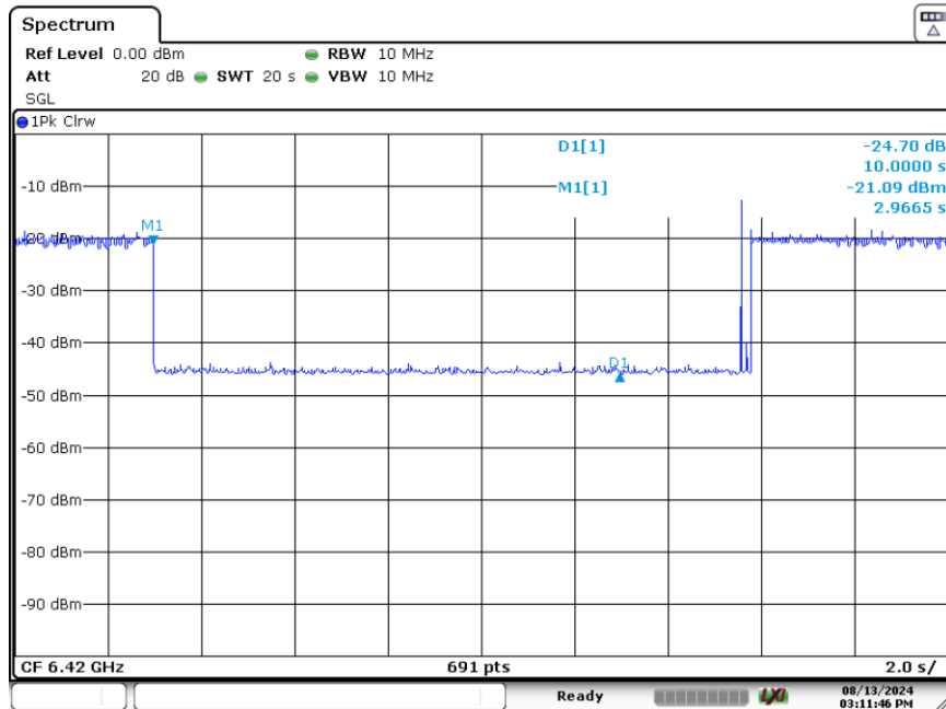
Plot 7-219. Contention Based Protocol Timing Plot (320MHz (UNII Band 5) – Ch. 31 High)
