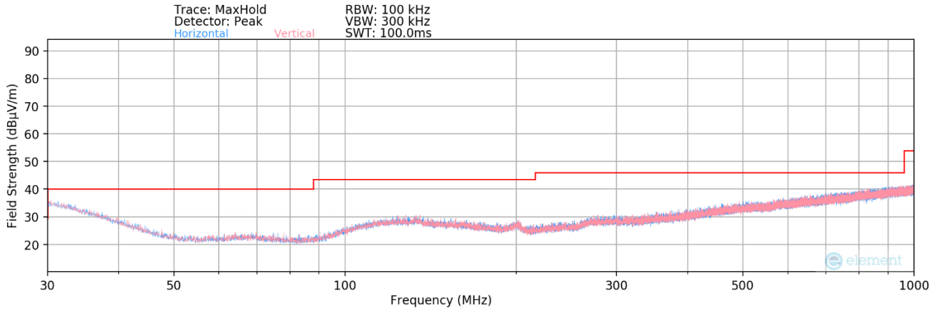
Plot 7-235. Radiated Spurious Plot below 1GHz MIMO (802.11a)
