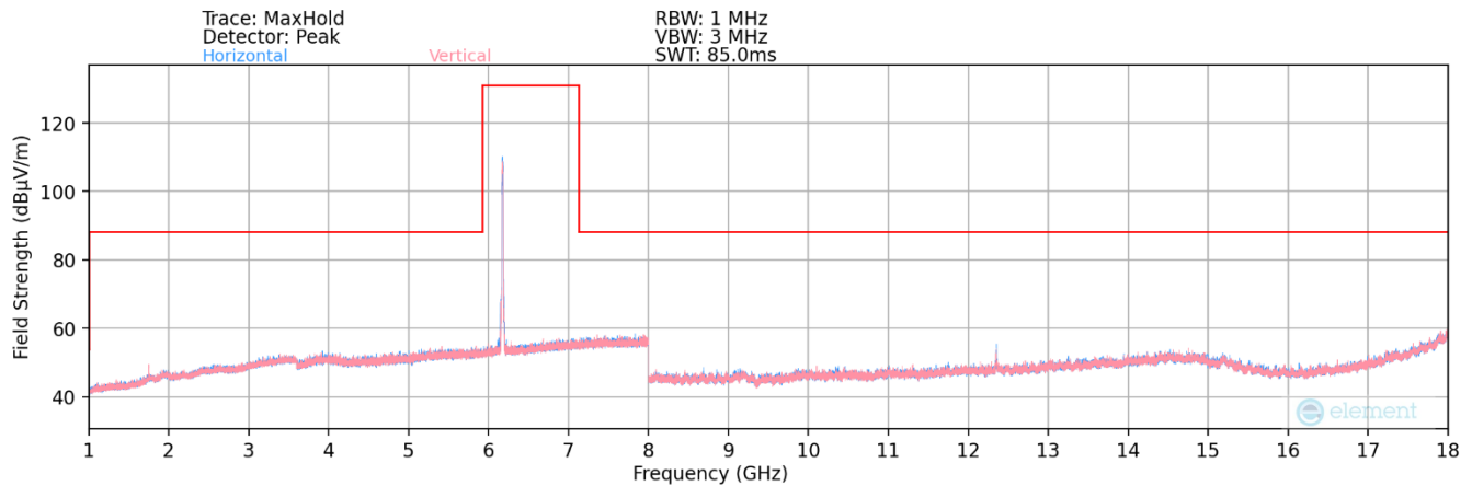
Plot 7-236. Radiated Spurious Plot 1GHz – 18GHz MIMO (802.11a – UNII Band 5 Ch. 45 – LPI/SP)
