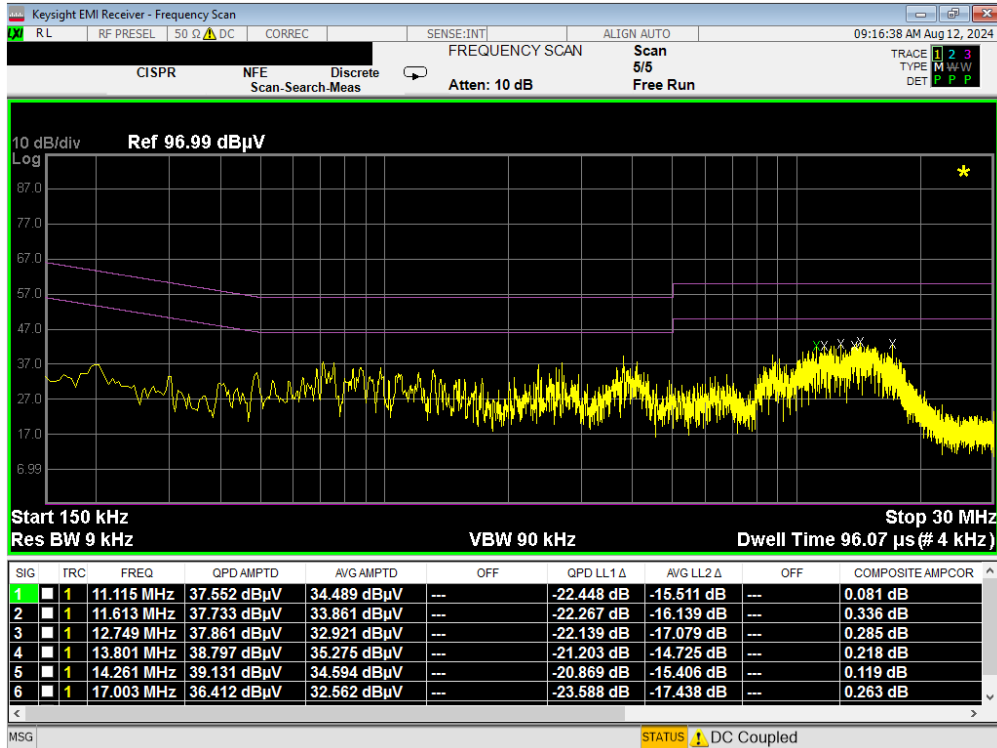
Plot 7-264. Line Conducted Plot with 802.11a UNII Band 6 (L1)
