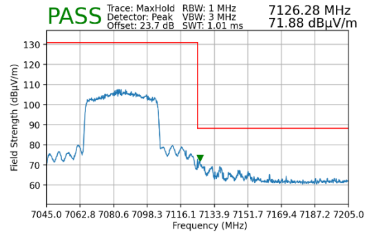
Plot 7-249. Radiated Upper Band Edge Plot MIMO (Peak – UNII Band 8)
