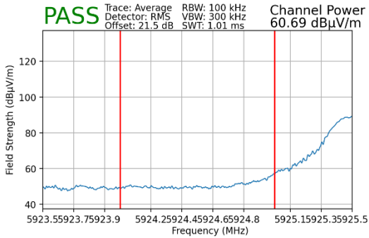
Plot 7-242. Radiated Lower Band Edge Plot MIMO (Average – UNII Band 5)
