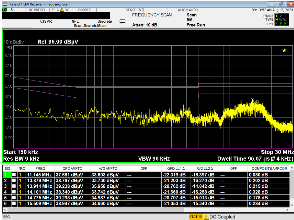
Plot 7-262. Line Conducted Plot with 802.11a UNII Band 5 (L1)
