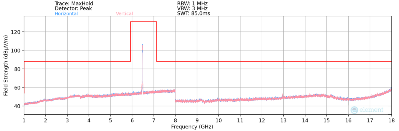
Plot 7-237. Radiated Spurious Plot 1GHz – 18GHz MIMO (802.11a – UNII Band 6 Ch. 105 – LPI)
