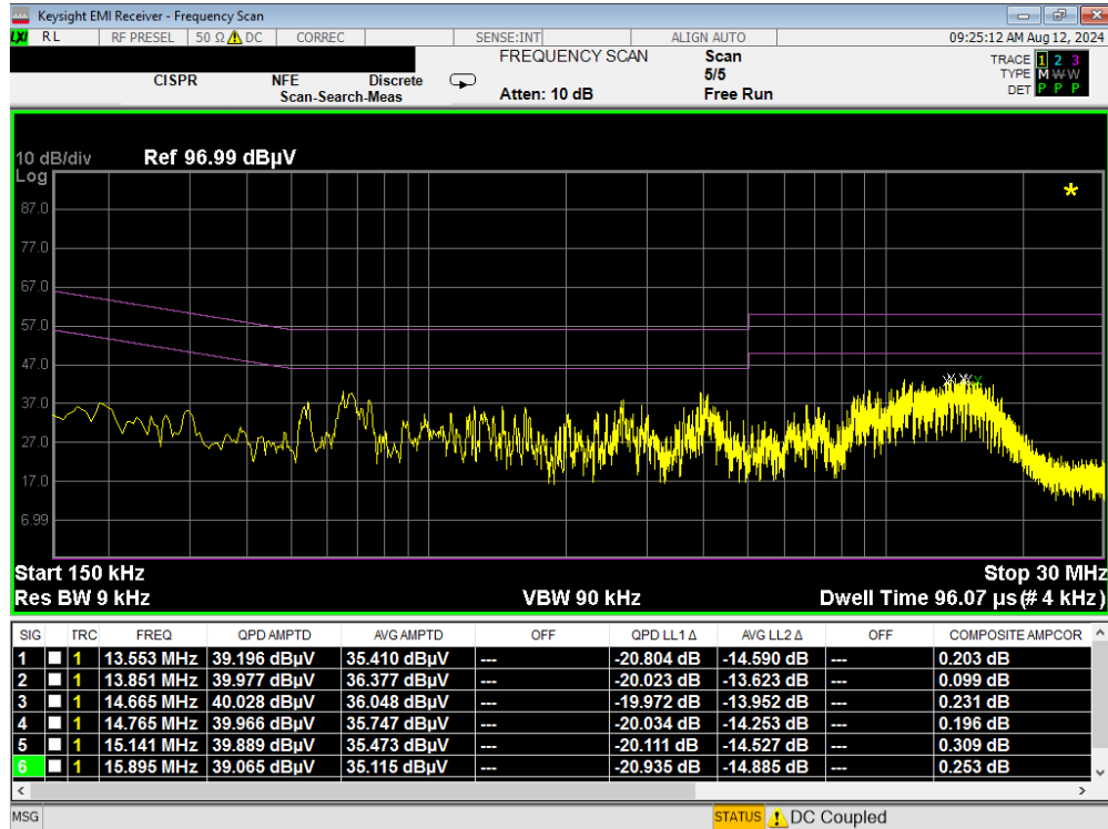
Plot 7-268. Line Conducted Plot with 802.11a UNII Band 8 (L1)
