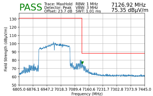
Plot 7-257. Radiated Upper Band Edge Plot MIMO (Peak – UNII Band 8)
