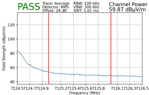
Plot 7-244. Radiated Upper Band Edge Plot MIMO (Average – UNII Band 8)
