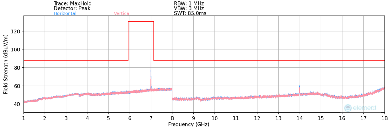
Plot 7-239. Radiated Spurious Plot 1GHz – 18GHz MIMO (802.11a – U Band 8 Ch. 209 – LPI)
