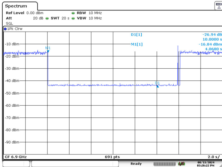
Plot 7-227. Contention Based Protocol Timing Plot (320MHz (UNII Band 7) – Ch. 159 High)
