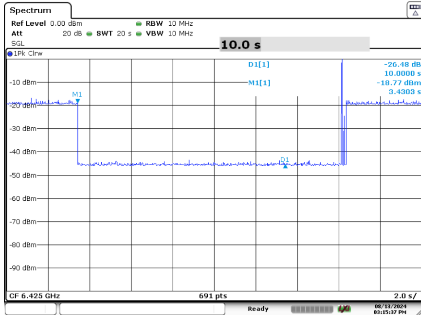
Plot 7-222. Contention Based Protocol Timing Plot (320MHz (UNII Band 6) – Ch. 95 Mid)
