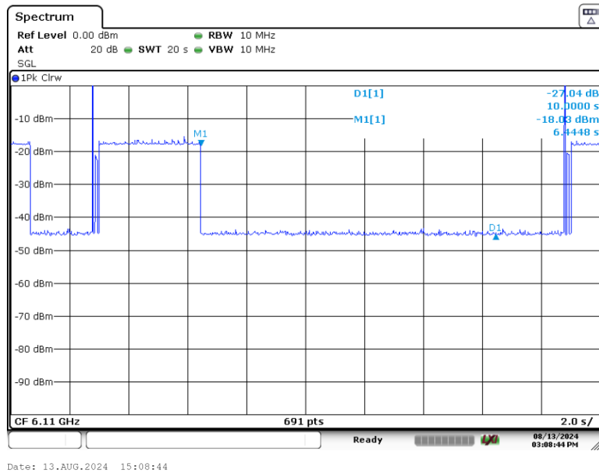
Plot 7-217. Contention Based Protocol Timing Plot (320MHz (UNII Band 5) – Ch. 31 Low)
