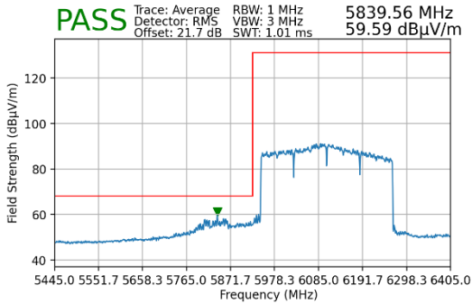
Plot 7-258. Radiated Lower Band Edge Plot MIMO (Average – UNII Band 5)
