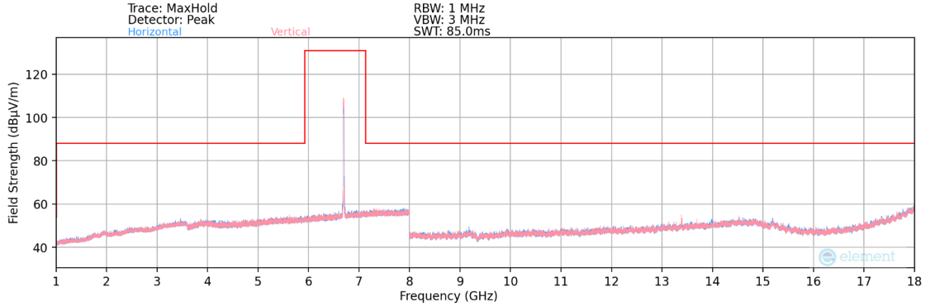
Plot 7-238. Radiated Spurious Plot 1GHz – 18GHz MIMO (802.11a – UNII Band 7 Ch. 149 – LPI/SP)
