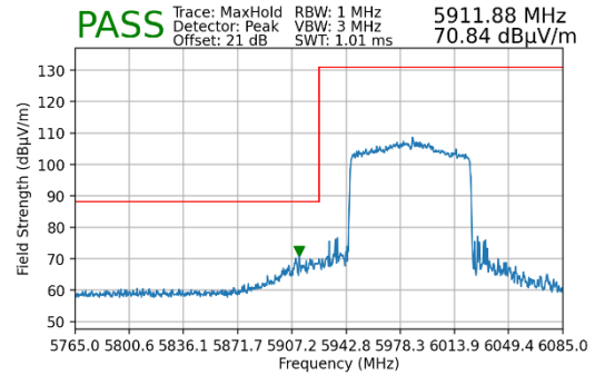
Plot 7-251. Radiated Lower Band Edge Plot MIMO (Peak – UNII Band 5)
