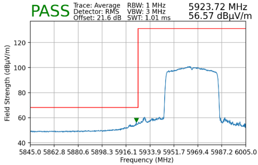
Plot 7-246. Radiated Lower Band Edge Plot MIMO (Average – UNII Band 5)
