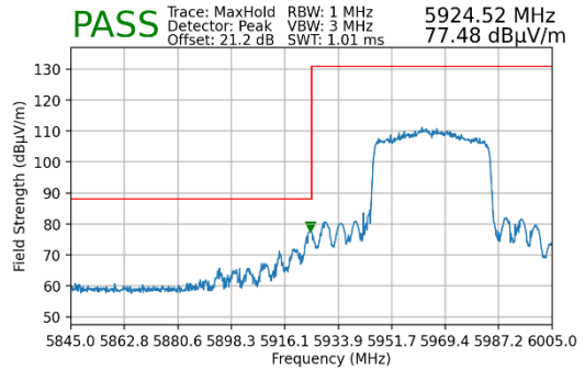
Plot 7-247. Radiated Lower Band Edge Plot MIMO (Peak – UNII Band 5)
