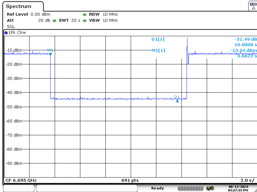
Plot 7-224. Contention Based Protocol Timing Plot (20MHz (UNII Band 7) – Ch. 149)
