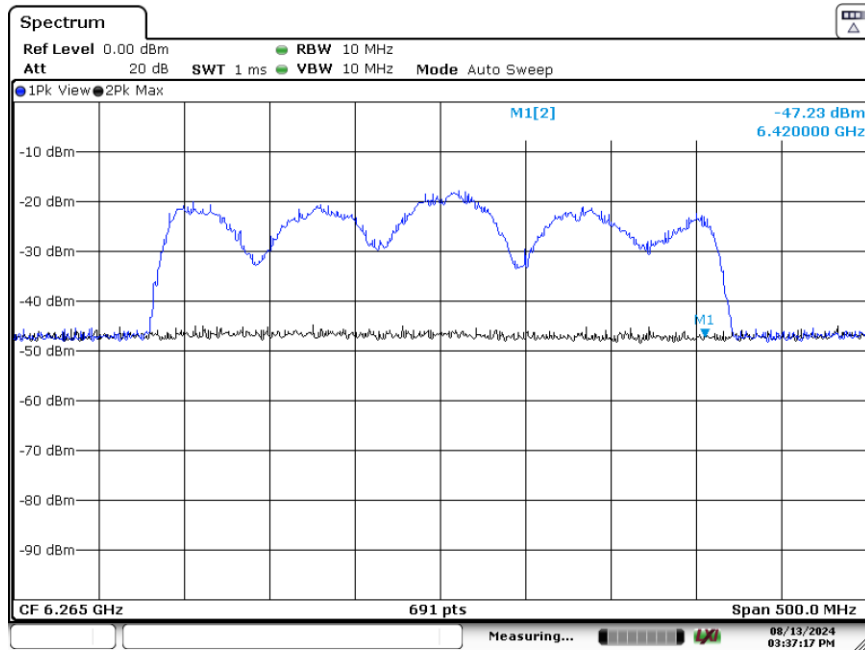
Plot 7-234. CBP 320MHz Channel - Injection Upper Edge – [6420 MHz]
