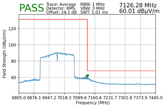
Plot 7-256. Radiated Upper Band Edge Plot MIMO (Average – UNII Band 8)
