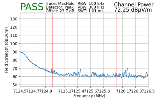
Plot 7-245. Radiated Upper Band Edge Plot MIMO (Peak – UNII Band 8)
