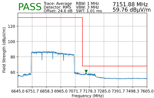
Plot 7-260. Radiated Upper Band Edge Plot MIMO (Average – UNII Band 8)
