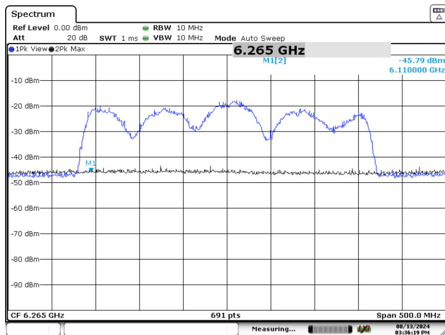
Plot 7-232. CBP 320MHz Channel - Injection Lower Edge – [6110 MHz]
