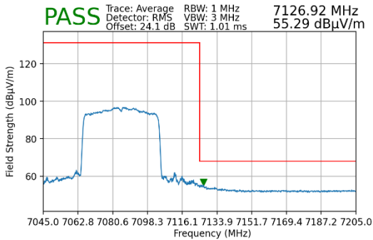
Plot 7-248. Radiated Upper Band Edge Plot MIMO (Average – UNII Band 8)
