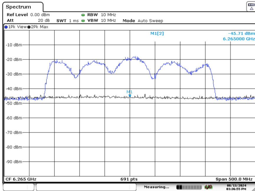
Plot 7-233. CBP 320MHz Channel - Injection Center – [6265 MHz]
