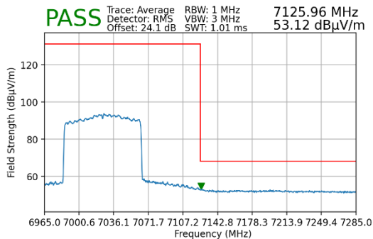
Plot 7-252. Radiated Upper Band Edge Plot MIMO (Average – UNII Band 8)
