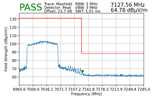
Plot 7-253. Radiated Upper Band Edge Plot MIMO (Peak – UNII Band 8)
