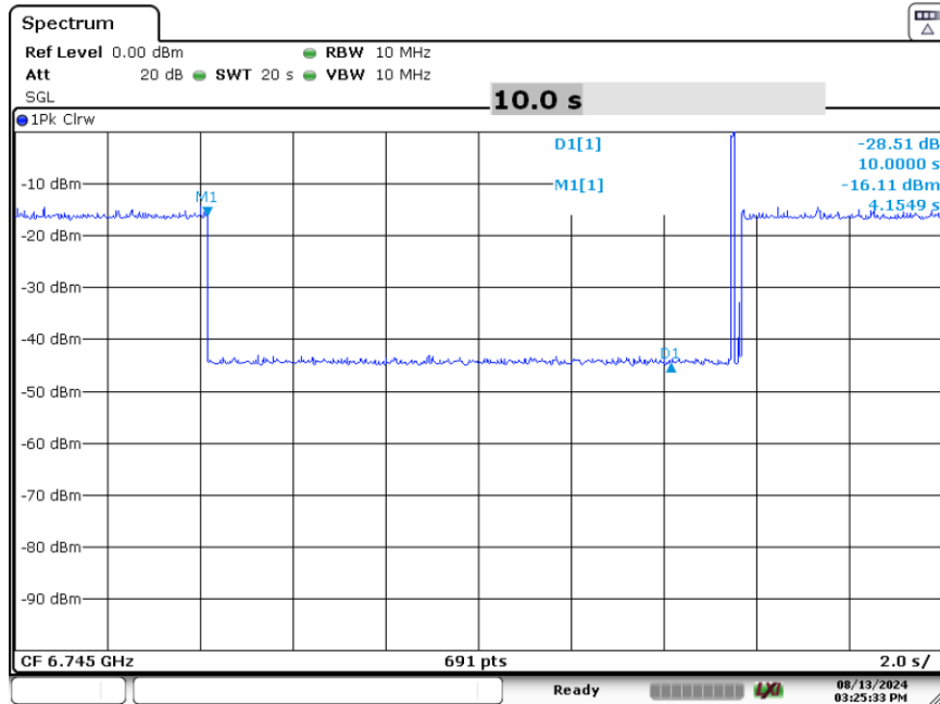
Plot 7-226. Contention Based Protocol Timing Plot (320MHz (UNII Band 7) – Ch. 159 Mid)
