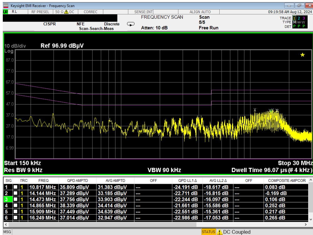
Plot 7-267. Line Conducted Plot with 802.11a UNII Band 7 (N)
