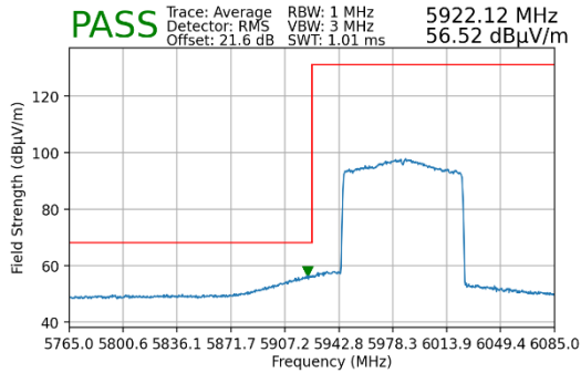
Plot 7-250. Radiated Lower Band Edge Plot MIMO (Average – UNII Band 5)
