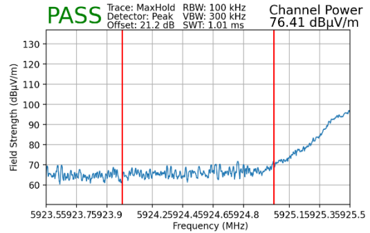
Plot 7-243. Radiated Lower Band Edge Plot MIMO (Peak – UNII Band 5)
