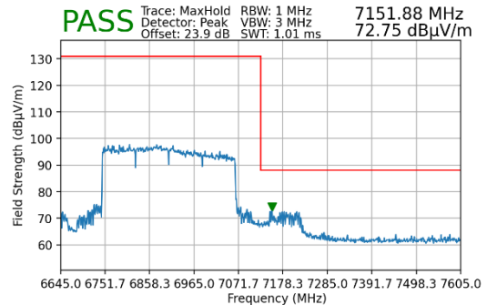
Plot 7-261. Radiated Upper Band Edge Plot MIMO (Peak – UNII Band 8)
