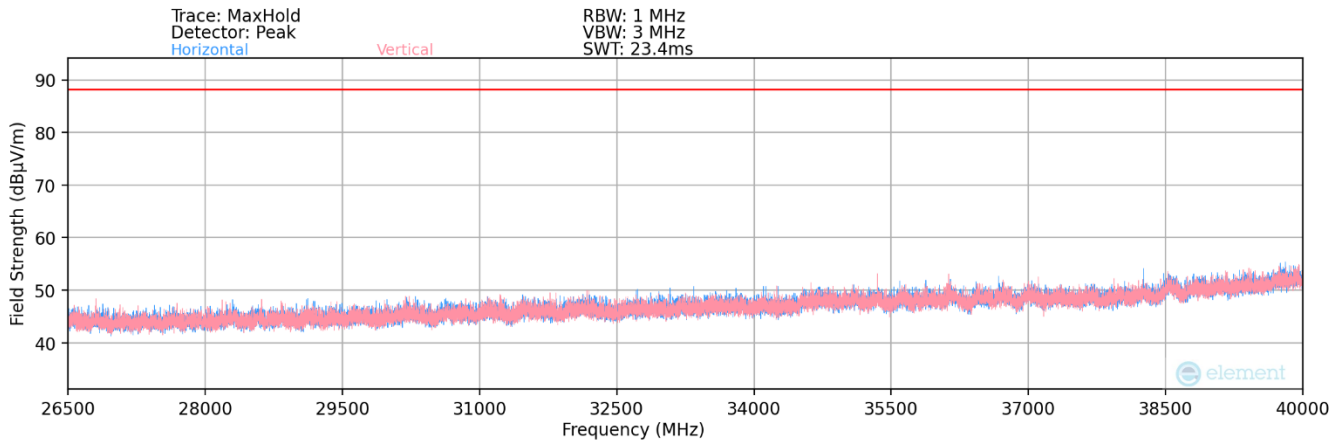
Plot 7-241. Radiated Spurious Plot 26.5GHz - 40GHz (802.11a)
