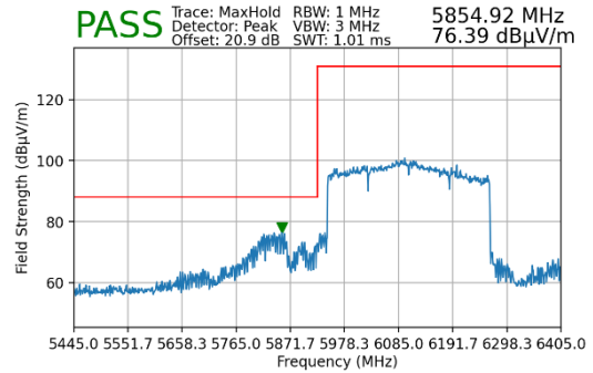
Plot 7-259. Radiated Lower Band Edge Plot MIMO (Peak – UNII Band 5)
