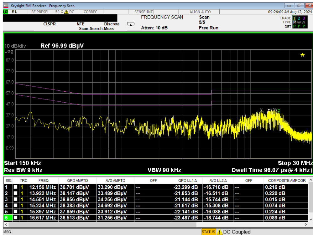
Plot 7-269. Line Conducted Plot with 802.11a UNII Band 8 (N)
