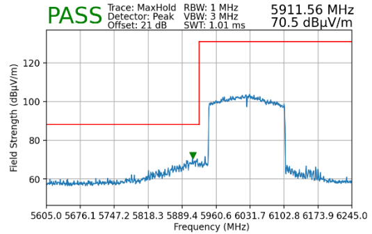
Plot 7-255. Radiated Lower Band Edge Plot MIMO (Peak – UNII Band 5)
