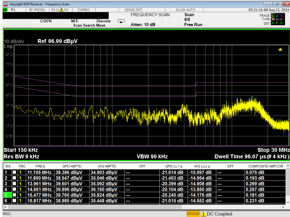
Plot 7-266. Line Conducted Plot with 802.11a UNII Band 7 (L1)
