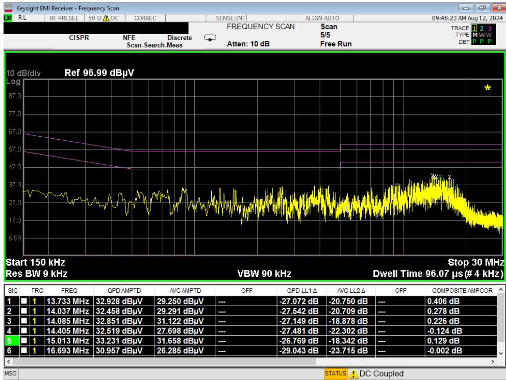
Plot 7-98. Line-Conducted Test Plot (N)
