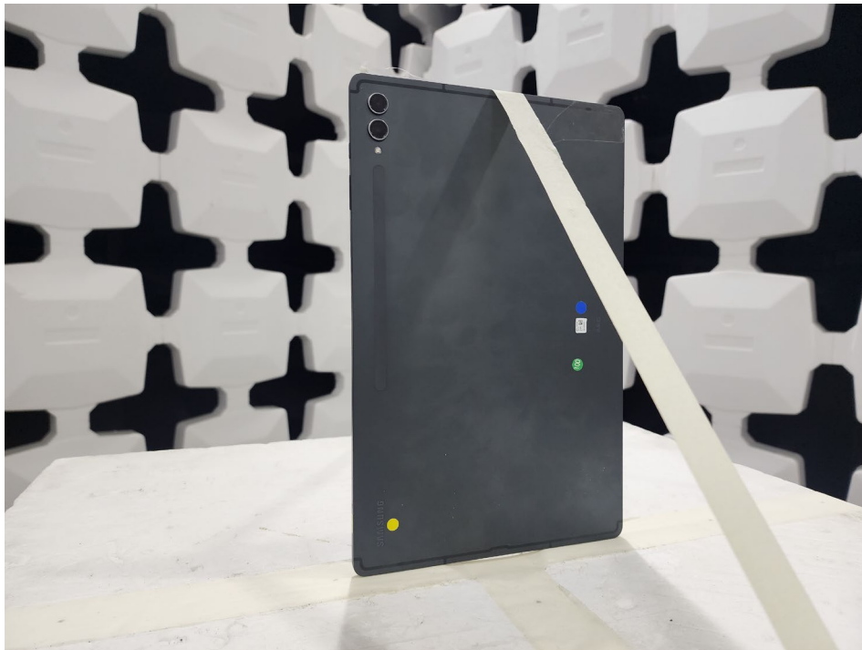
Figure 6. Test Setup – Z Position – 1GHz-18GHz
