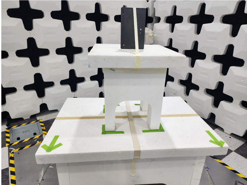
Figure 5. Test Setup – Z Position – 1GHz-18GHz
