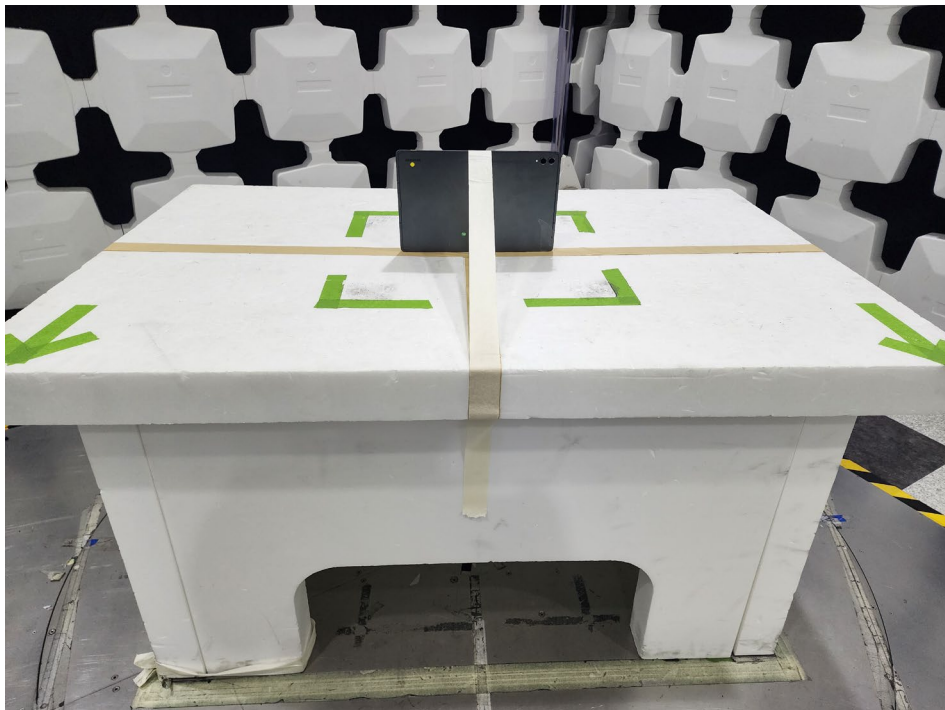
Figure 8. Test Setup – Y Position – 30MHz-1GHz
