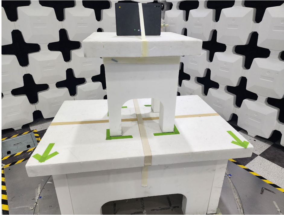
Figure 3. Test Setup – Y Position – 1GHz-18GHz
