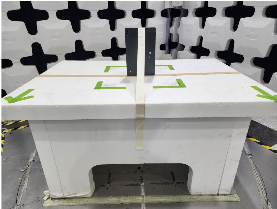
Figure 9. Test Setup – Z Position – 30MHz-1GHz
