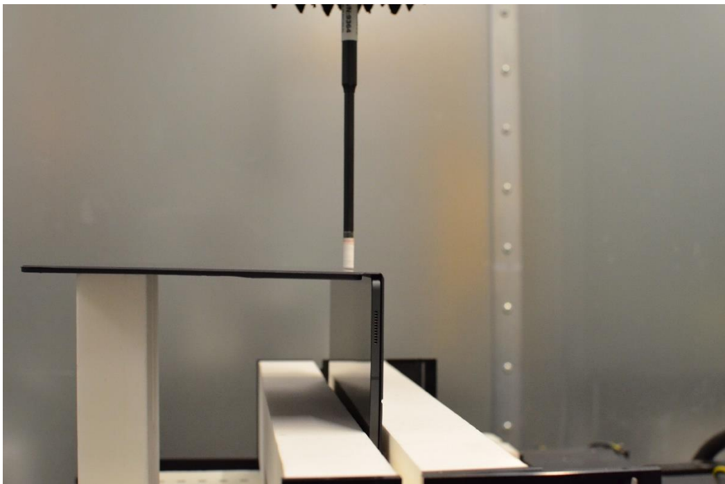
Figure G-34 Near Field Power Density Test Setup Photo – Laptop, Bottom edge at 2mm with Keyboard (Variant 1) – WIFI MIMO
