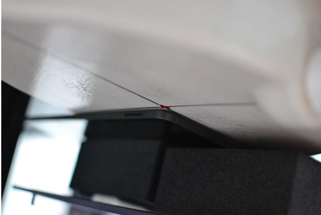
Figure G-3 SAR Test Setup Photo – Tablet, Back side at 0mm – WIFI MIMO (Peak 1)
