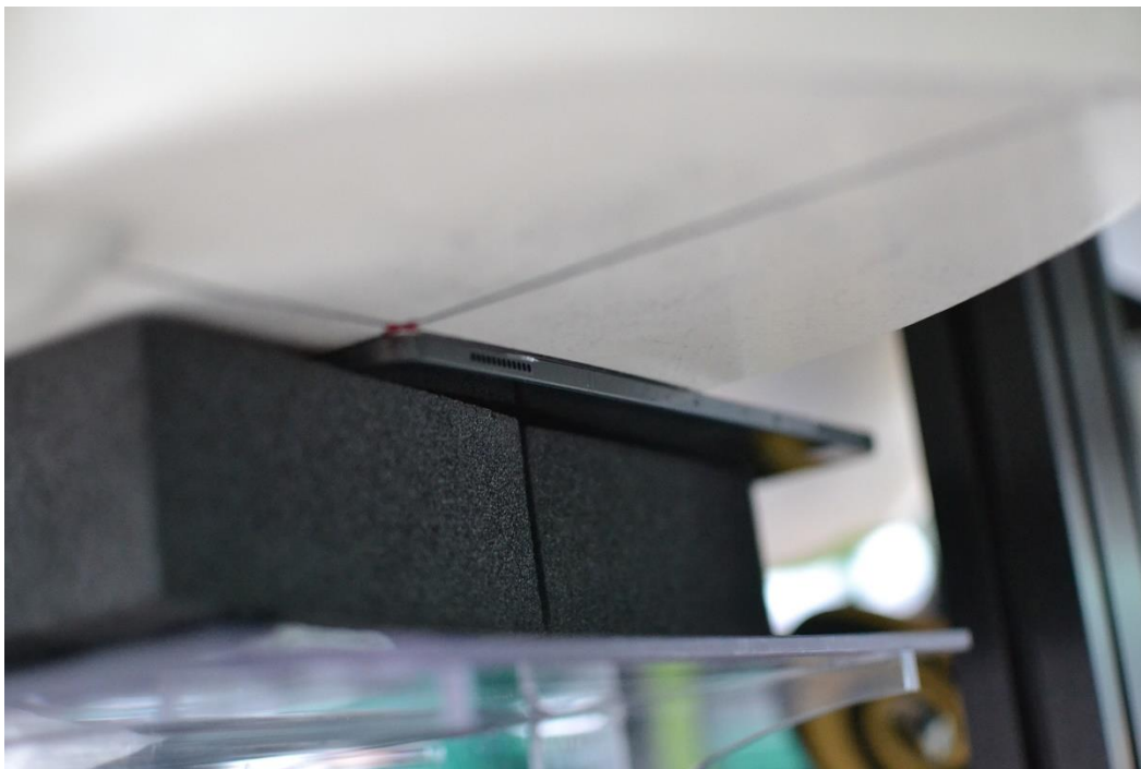
Figure G-4 SAR Test Setup Photo – Tablet, Back side at 0mm – WIFI MIMO (Peak 2)
