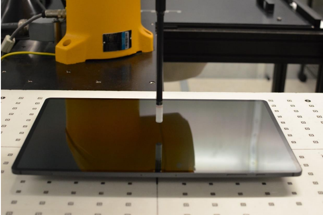
Figure G-25 Near Field Power Density Test Setup Photo – Tablet, Front side at 15mm – WIFI MIMO
