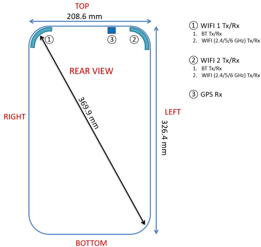
Figure G-1 DUT Antenna Locations
