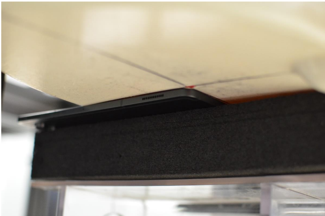
Figure G-10 SAR Test Setup Photo – Tablet, Front side at 0mm – WIFI MIMO (Peak 2)
