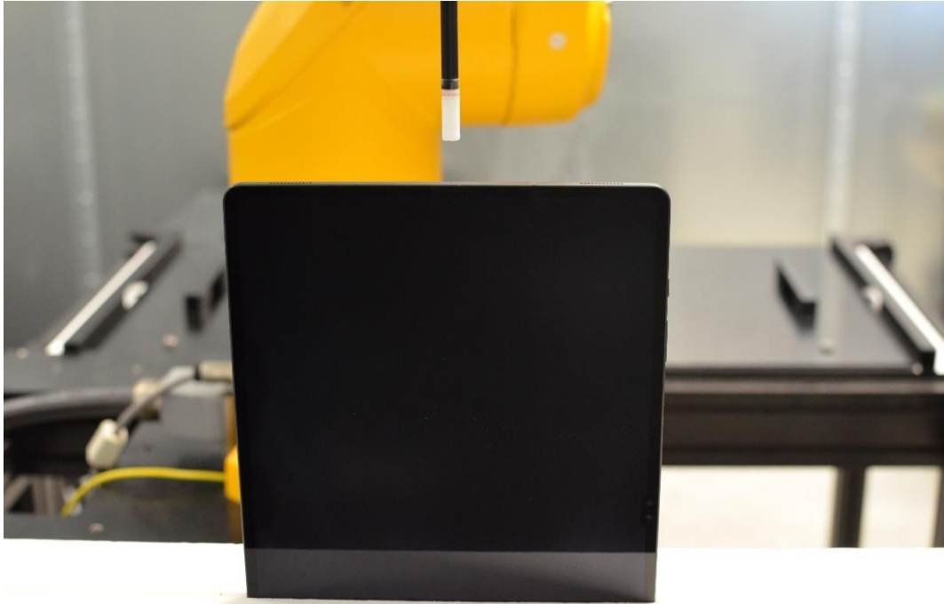
Figure G-27 Near Field Power Density Test Setup Photo – Tablet, Top edge at 19mm – WIFI MIMO
