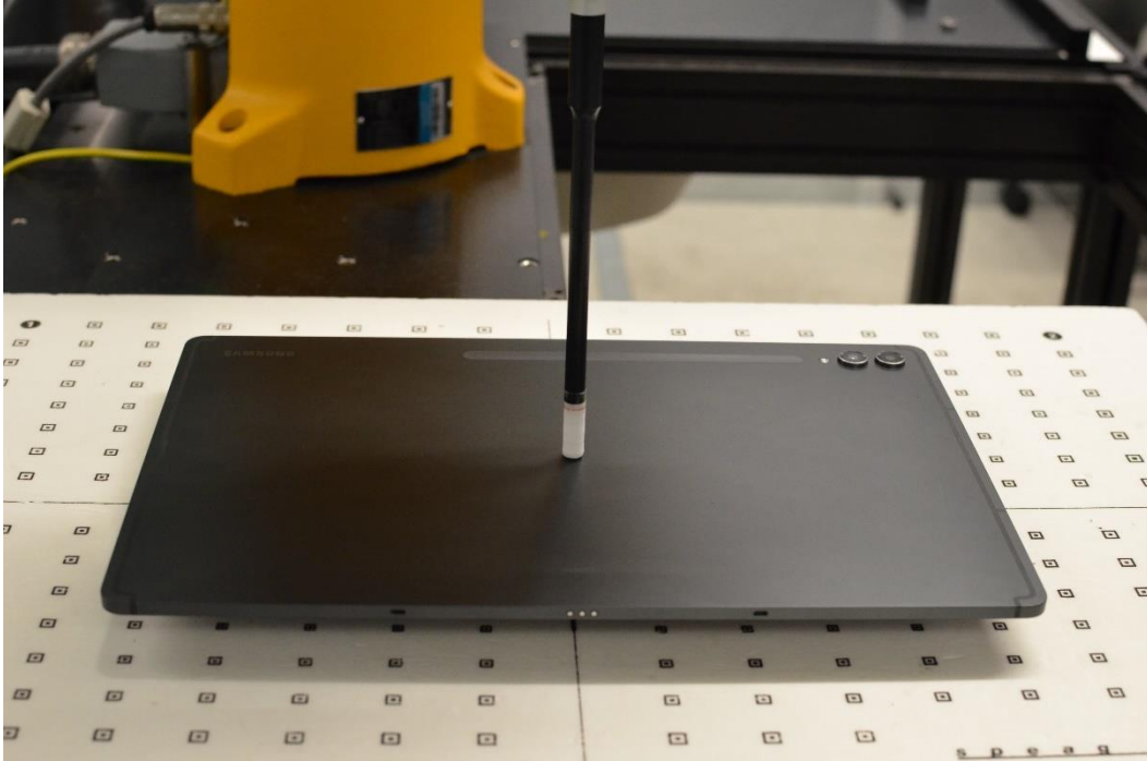
Figure G-21 Near Field Power Density Test Setup Photo – Tablet, Back side at 2mm – WIFI MIMO
