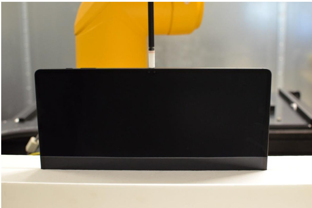
Figure G-28 Near Field Power Density Test Setup Photo – Tablet, Right edge at 2mm – WIFI MIMO
