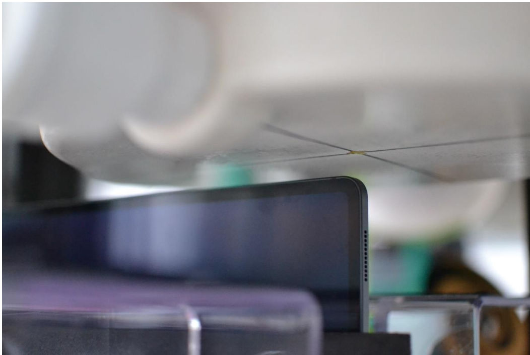
Figure G-18 SAR Test Setup Photo – Tablet, Left Edge at 9mm – WIFI MIMO
