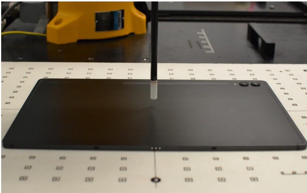
Figure G-22 Near Field Power Density Test Setup Photo – Tablet, Back side at 8.84mm – WIFI MIMO
