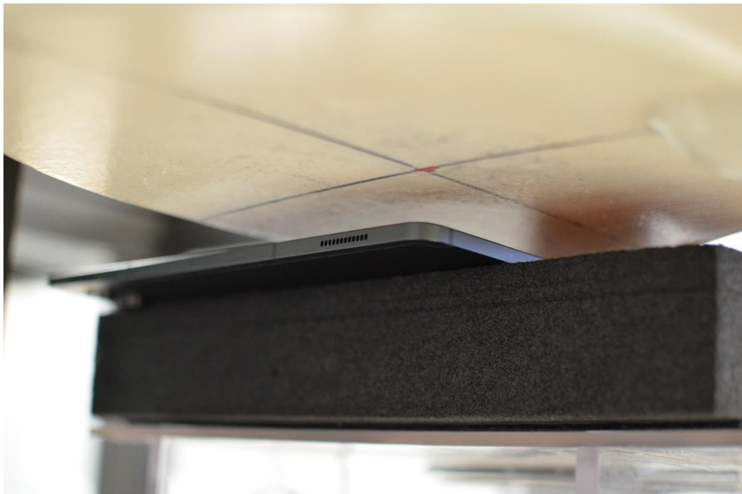
Figure G-12 SAR Test Setup Photo – Tablet, Front side at 15mm – WIFI MIMO (Peak 2)
