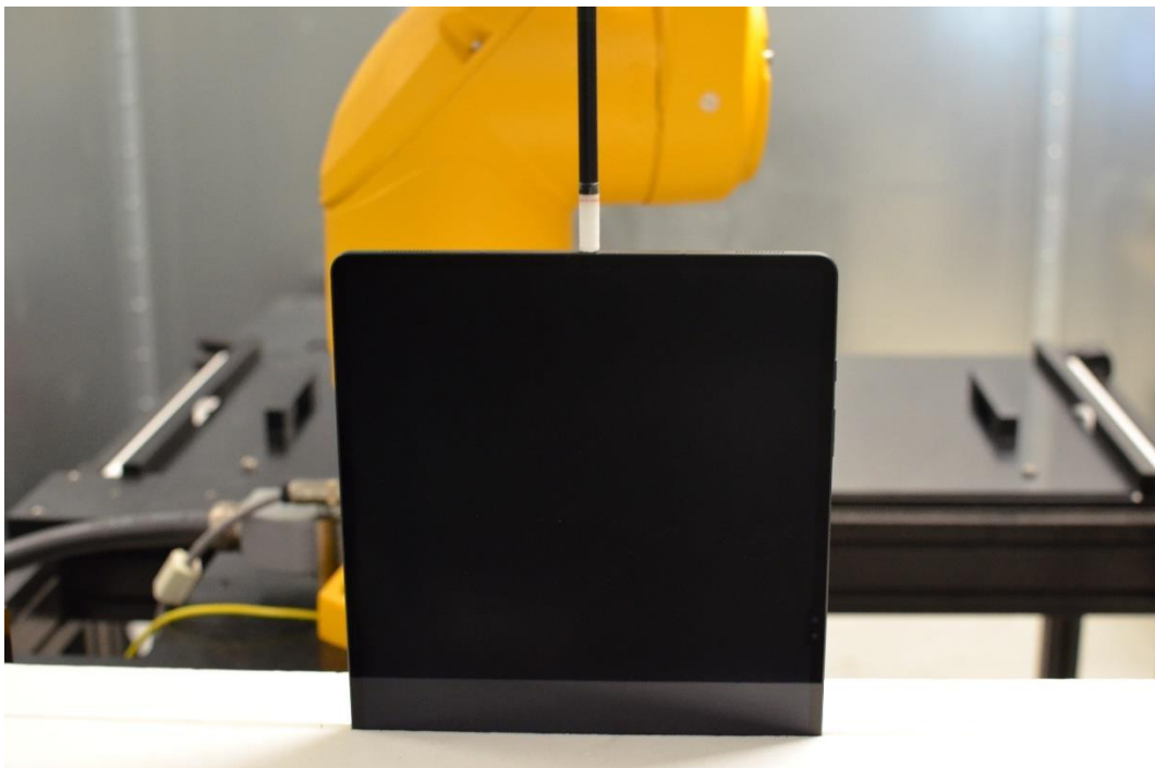
Figure G-26 Near Field Power Density Test Setup Photo – Tablet, Top edge at 2mm – WIFI MIMO
