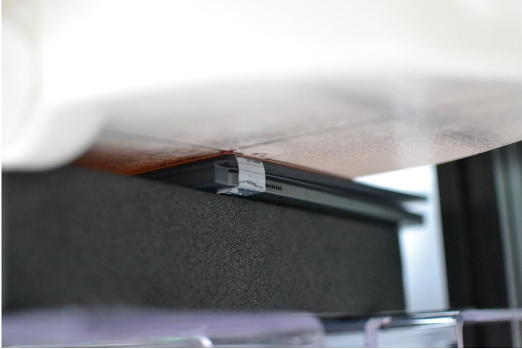
SAR Test Setup Photo 7 – Back side with Keyboard (Variant 2) at 0mm for WIFI/BT Antenna 2 and WIFI MIMO (Peak 2)
