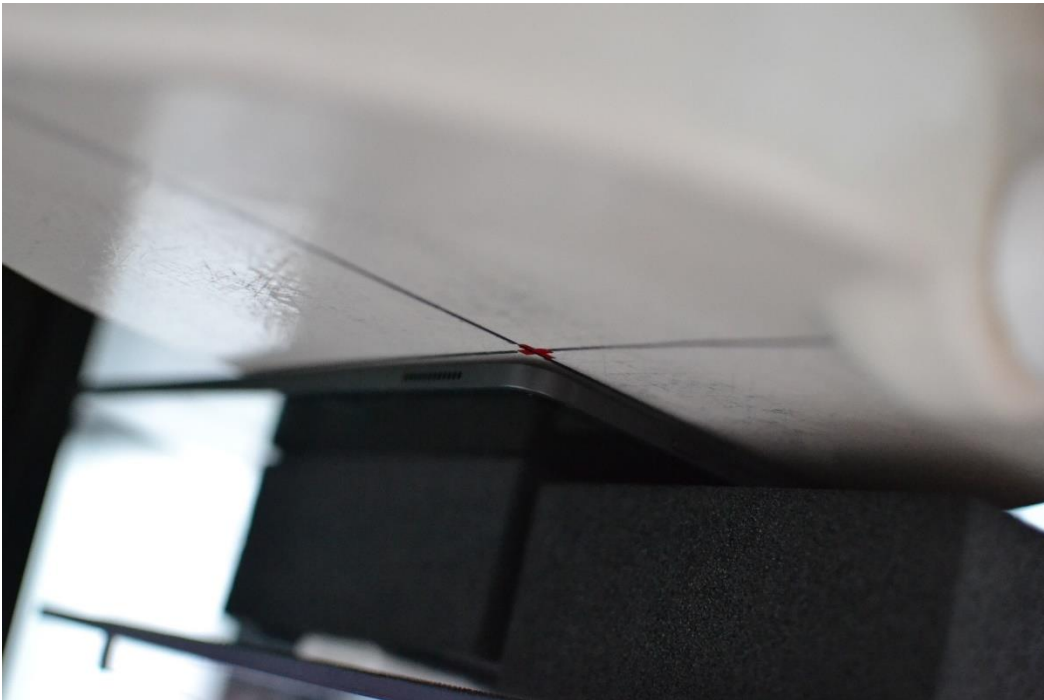
SAR Test Setup Photo 4 – Back side at 0mm for BT Antenna 1 and WIFI MIMO (Peak 1)
