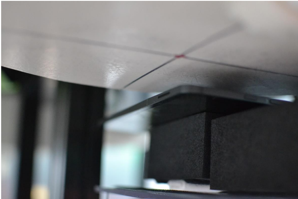
SAR Test Setup Photo 2 – Back side at 15mm for WIFI MIMO (Peak 1)
