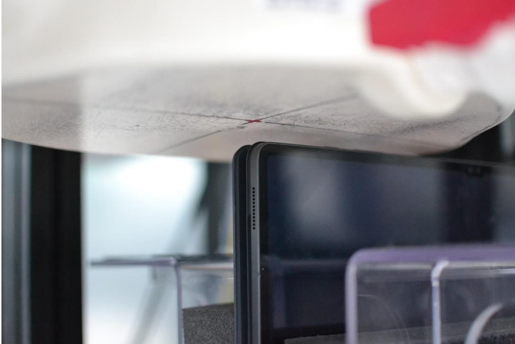
SAR Test Setup Photo 15 – Right Edge with Keyboard (Variant 2) at 7mm for BT Antenna 1 and WIFI MIMO
