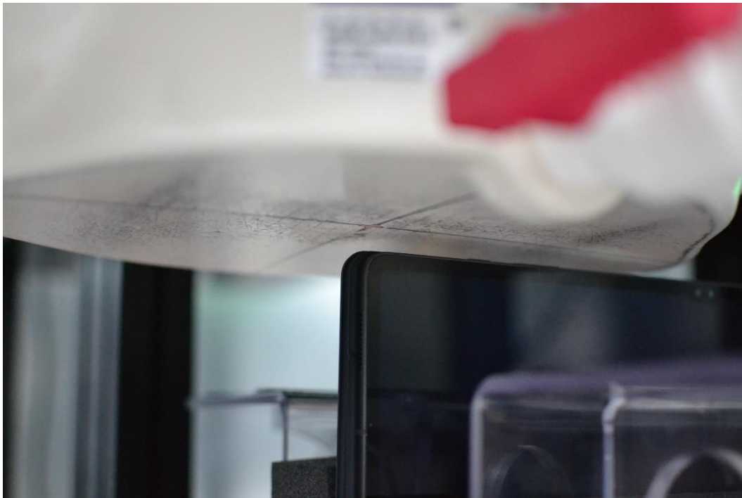
SAR Test Setup Photo 14 – Right Edge with Keyboard (Variant 1) at 7mm for BT Antenna 1 and WIFI MIMO
