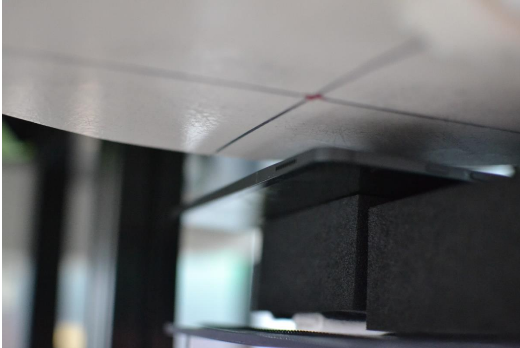
SAR Test Setup Photo 1 – Back side at 16mm for BT Antenna 1
