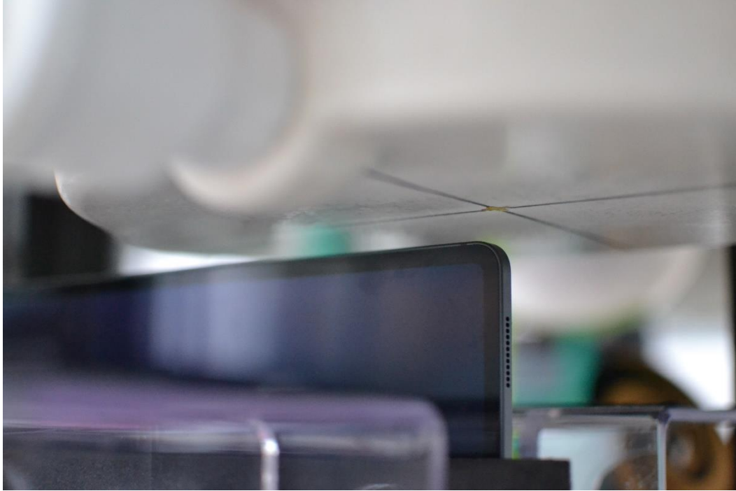
SAR Test Setup Photo 17 – Left Edge at 9mm for WIFI/BT Antenna 2 and WIFI MIMO
