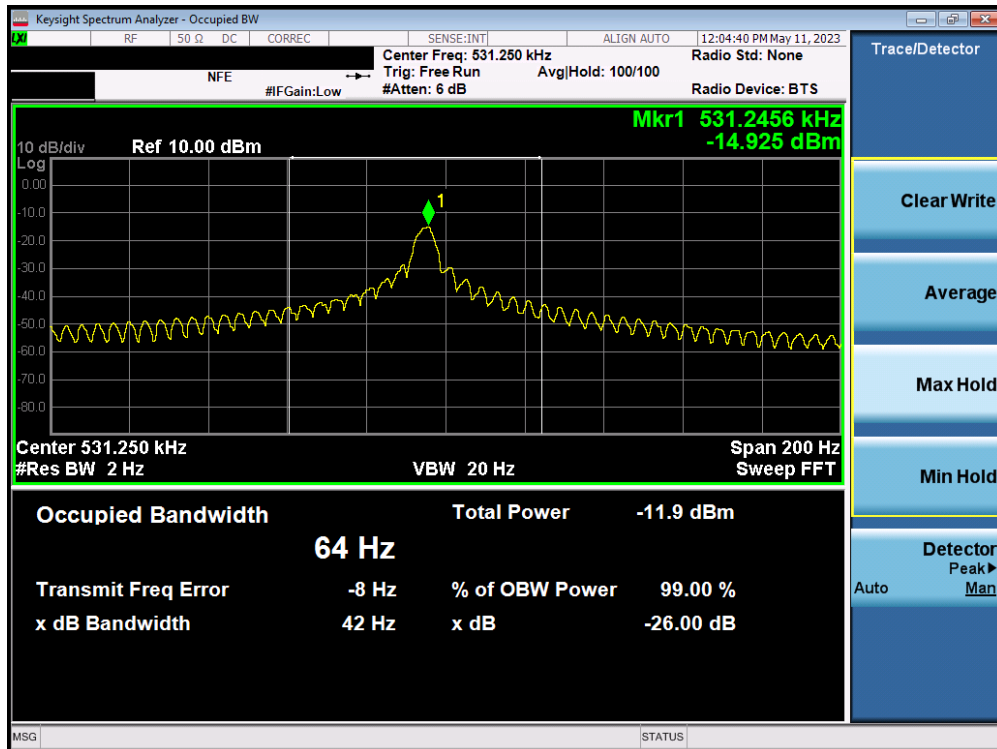
Plot 7-4. Occupied Bandwidth Measurement _ Click
