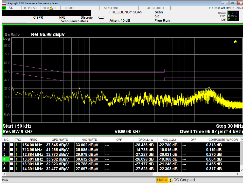
Plot 7-31. Line-Conducted Test Plot (L1) - Click
