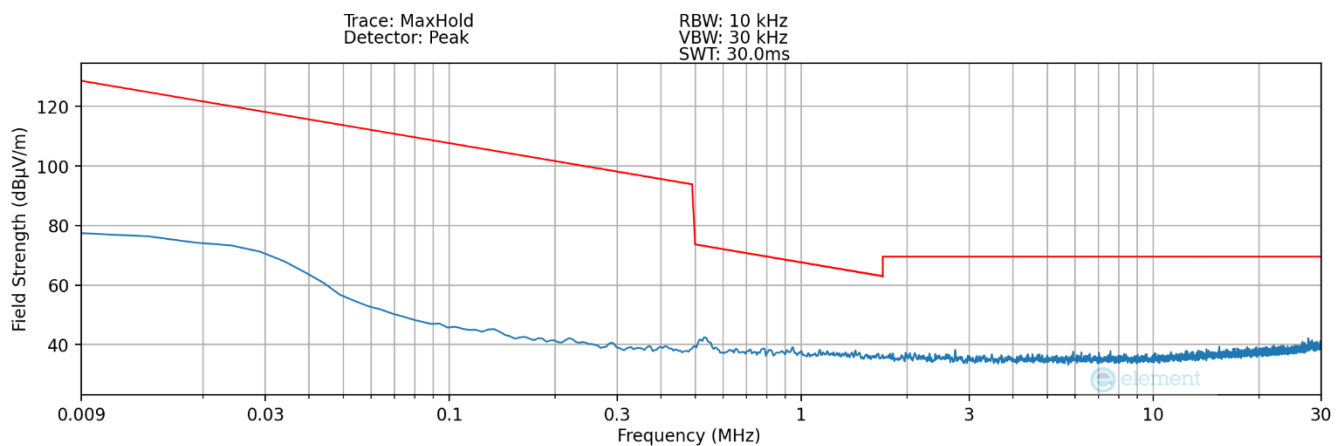
Plot 7-9. Radiated Spurious Plot 9kHz – 30MHz (Pol. Z – Device to Pen WPT) _ SPEN Detection 1
