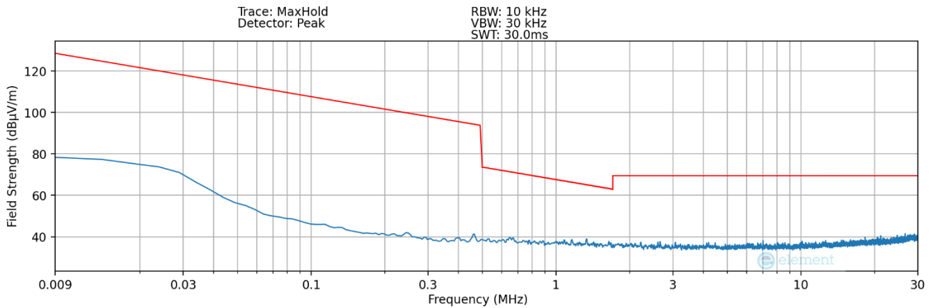
Plot 7-23 Radiated Spurious Plot 9kHz – 30MHz (Pol. Y – Digitizer – Keyboard Cover Detect)
