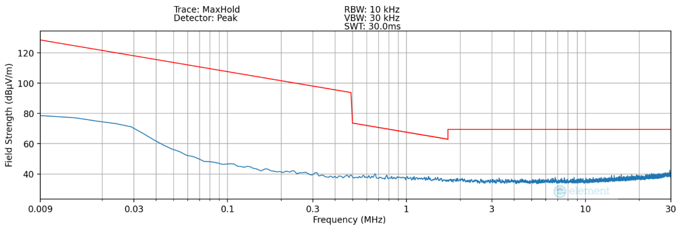
Plot 7-24. Radiated Spurious Plot 9kHz – 30MHz (Pol. Z – Digitizer – Keyboard Cover Detect)
