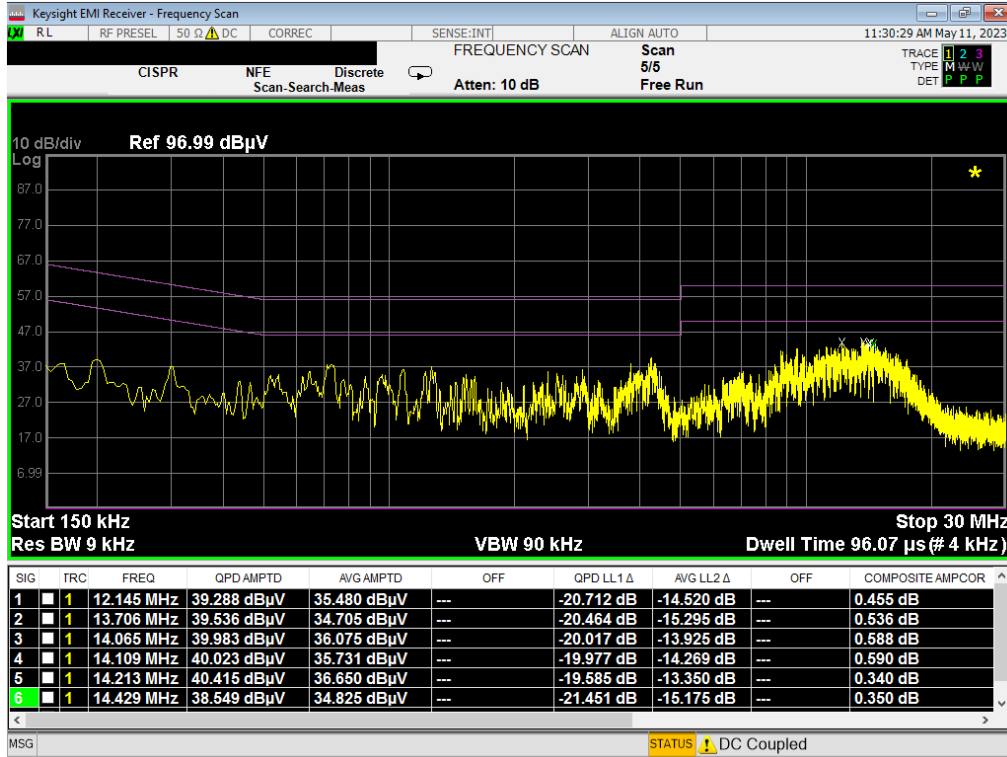
Plot 7-29. Line-Conducted Test Plot (L1) - Hover
