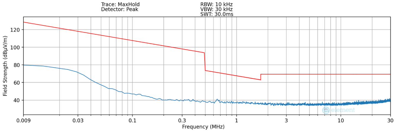
Plot 7-22. Radiated Spurious Plot 9kHz – 30MHz (Pol. X – Digitizer – Keyboard Cover Detect)
