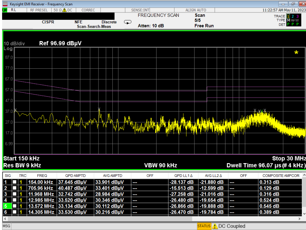
Plot 7-33. Line-Conducted Test Plot (L1) - Eraser
