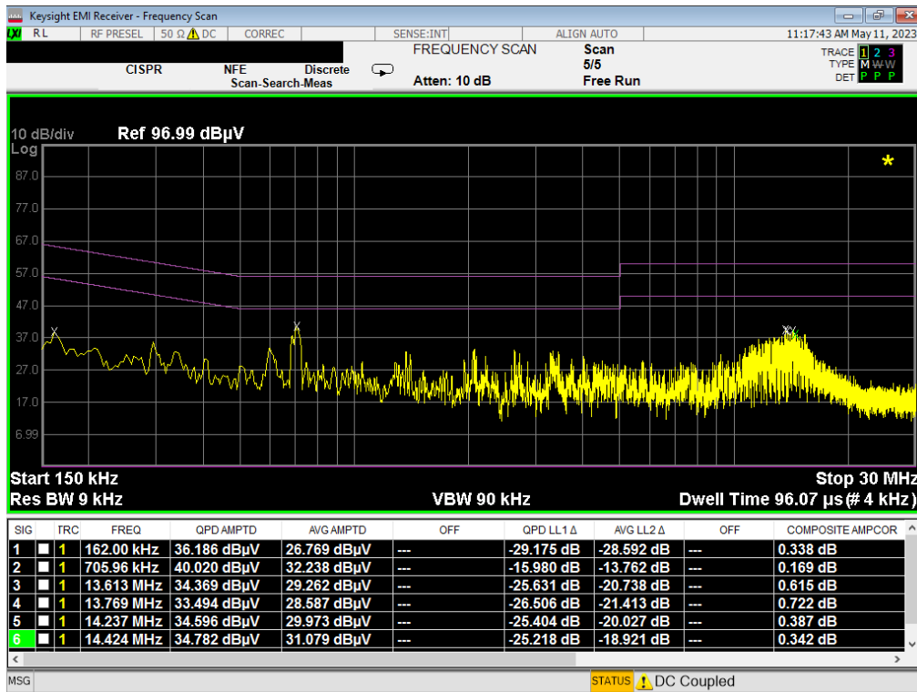
Plot 7-36. Line-Conducted Test Plot (N) - Keyboard Cover Detect
