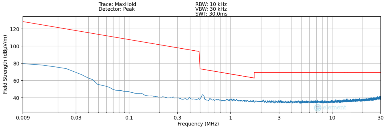
Plot 7-16. Radiated Spurious Plot 9kHz – 30MHz (Pol. X – Digitizer – Click)
