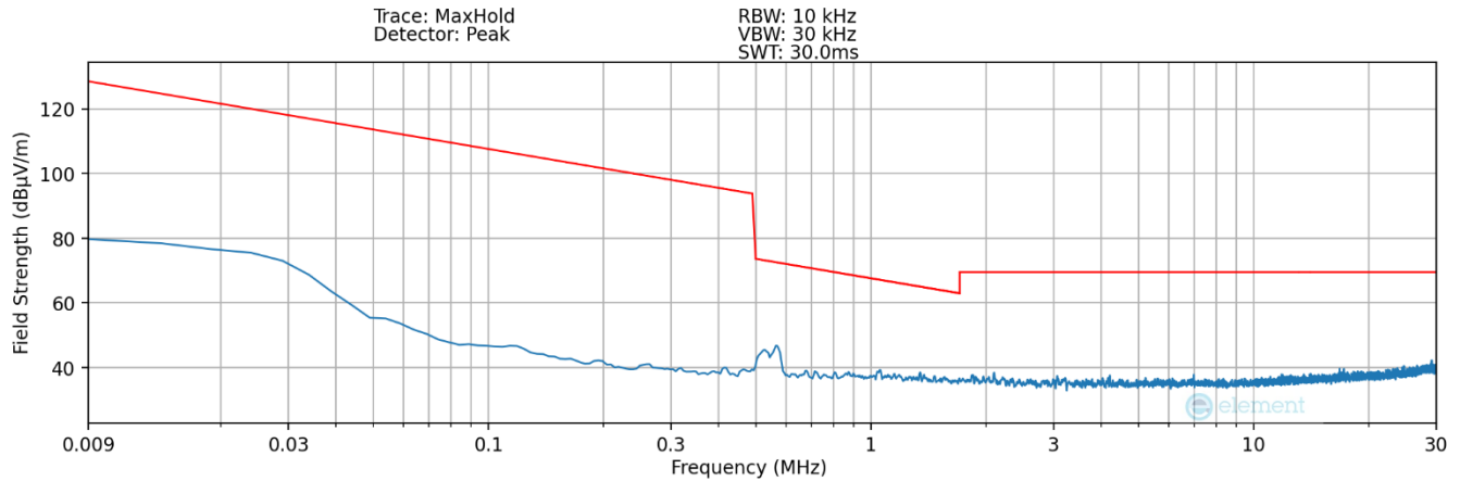
Plot 7-7. Radiated Spurious Plot 9kHz – 30MHz (Pol. X – Device to Pen WPT) _ SPEN Detection 1
