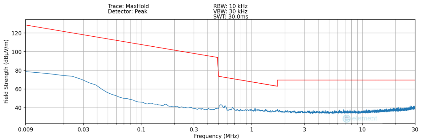
Plot 7-11 Radiated Spurious Plot 9kHz – 30MHz (Pol. Y – Device to Pen WPT) _ SPEN Detection 2
