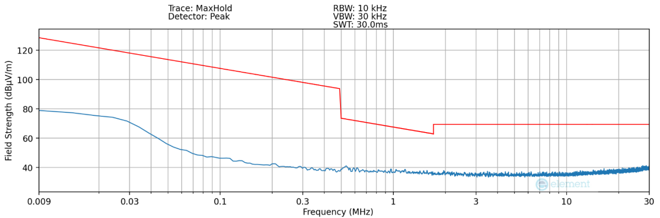
Plot 7-17 Radiated Spurious Plot 9kHz – 30MHz (Pol. Y – Digitizer – Click)
