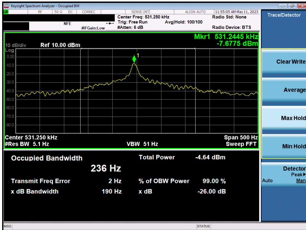
Plot 7-2. Occupied Bandwidth Measurement _ SPEN Detection 2
