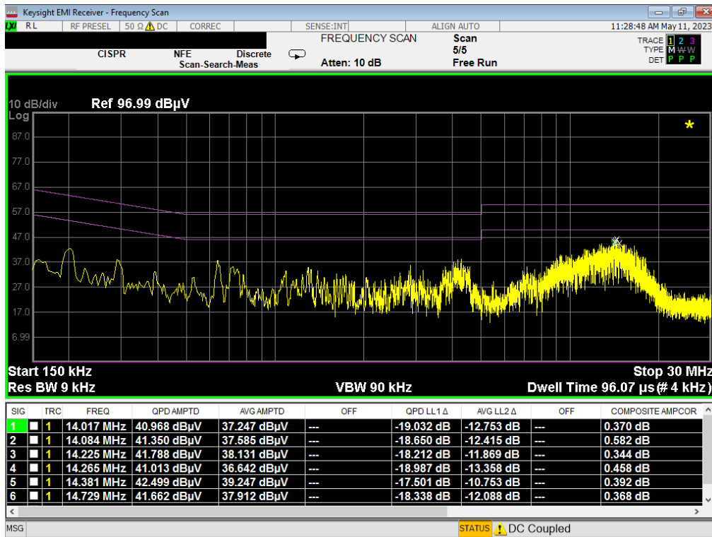
Plot 7-30. Line-Conducted Test Plot (N) - Hover
