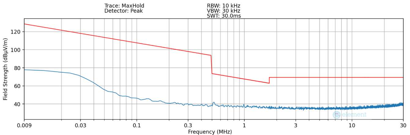
Plot 7-18. Radiated Spurious Plot 9kHz – 30MHz (Pol. Z – Digitizer – Click)
