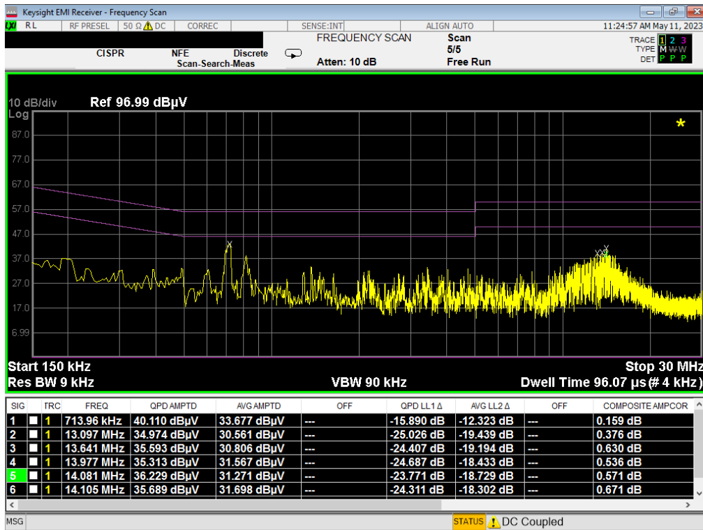
Plot 7-34. Line-Conducted Test Plot (N) - Eraser
