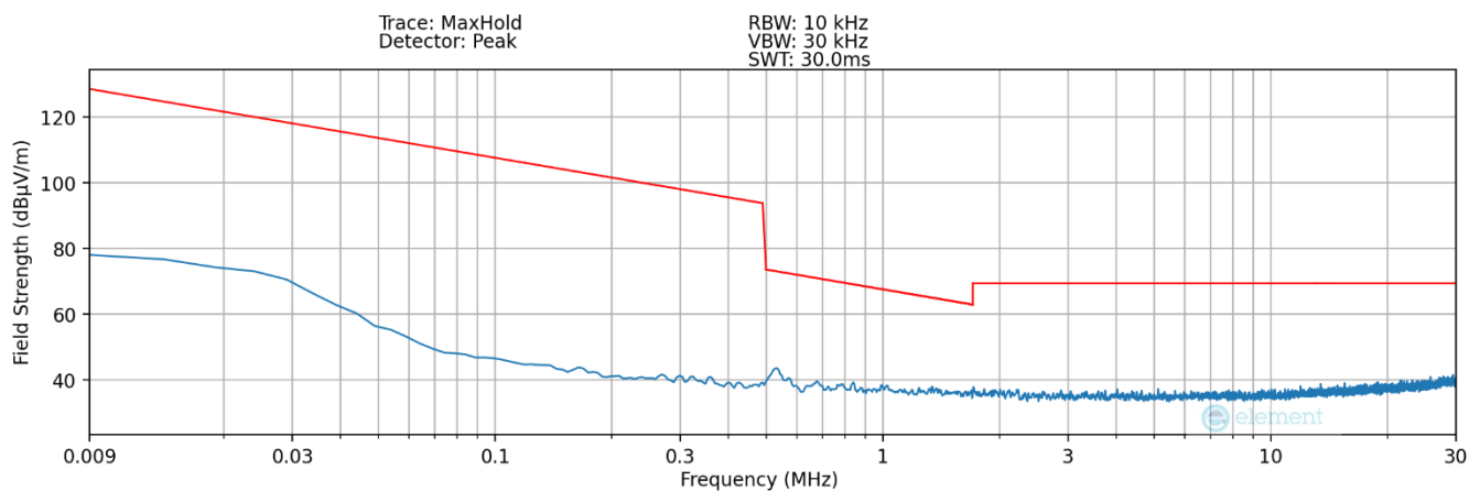
Plot 7-12. Radiated Spurious Plot 9kHz – 30MHz (Pol. Z – Device to Pen WPT) _ SPEN Detection 2
