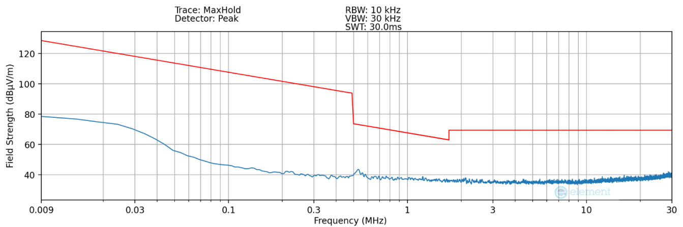
Plot 7-8 Radiated Spurious Plot 9kHz – 30MHz (Pol. Y – Device to Pen WPT) _ SPEN Detection 1
