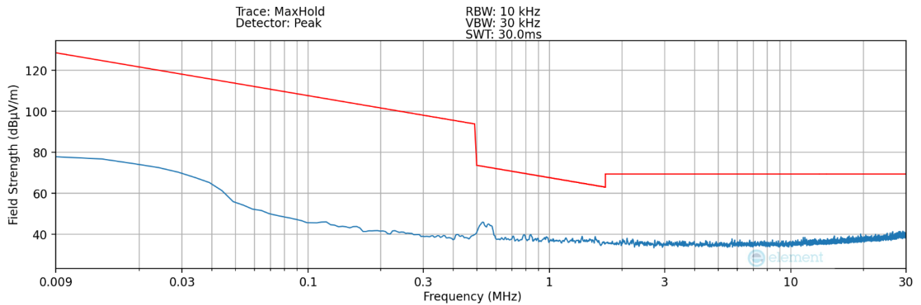
Plot 7-10. Radiated Spurious Plot 9kHz – 30MHz (Pol. X – Device to Pen WPT) _ SPEN Detection 2
