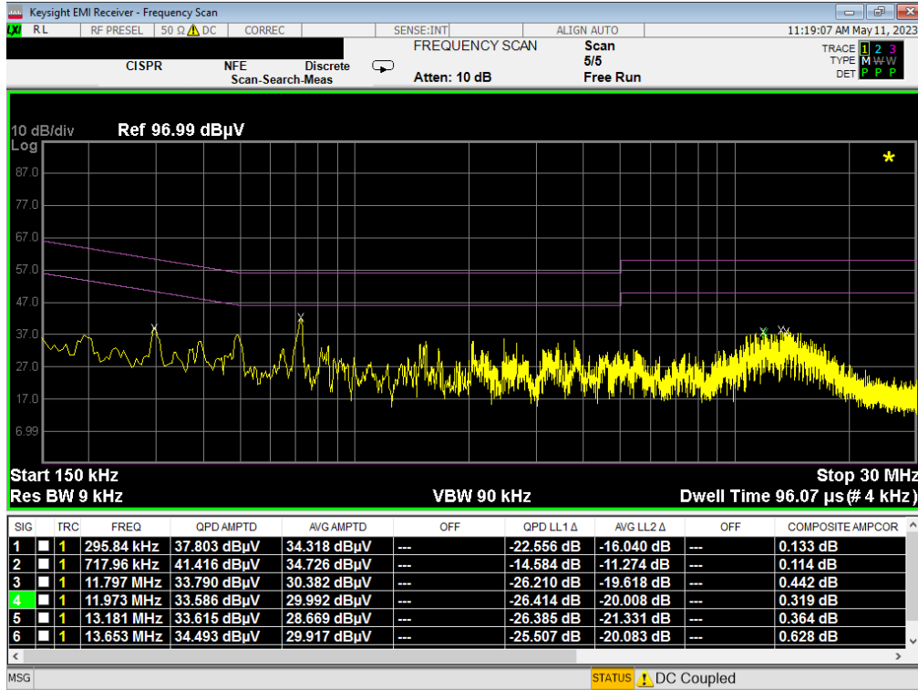
Plot 7-35. Line-Conducted Test Plot (L1) - Keyboard Cover Detect
