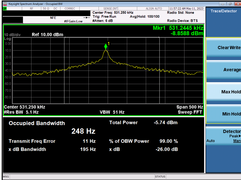
Plot 7-1. Occupied Bandwidth Measurement _ SPEN Detection 1
