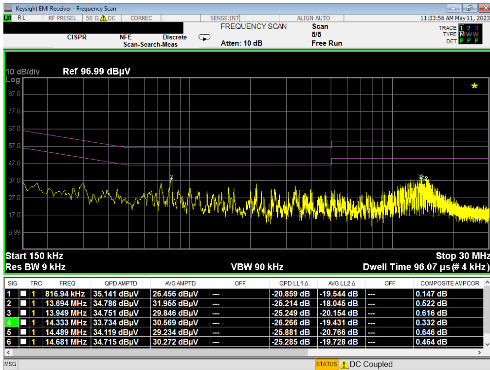
Plot 7-32. Line-Conducted Test Plot (N) - Click
