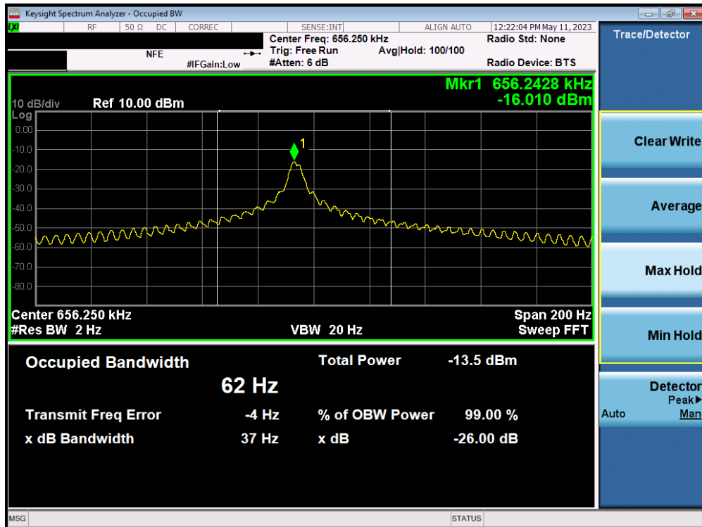
Plot 7-6. Occupied Bandwidth Measurement _ Keyboard Cover Detect
