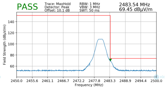
Plot 7-102. Radiated Restricted Upper Band Edge Measurement (Peak) – ANT1
