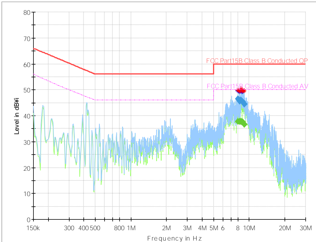
Plot 7-107. Line Conducted Plot with Bluetooth LE (N)
